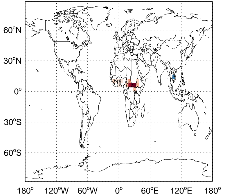
v11-02f-Run1 - v11-02e-Run1 SO2 biomass emissions for Jan
