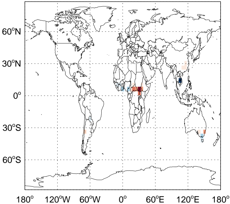
v11-02f-Run1 - v11-02e-Run0 SO2 biomass emissions for Jan
