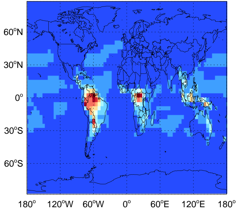
ACET biogenic emissions for Jan
