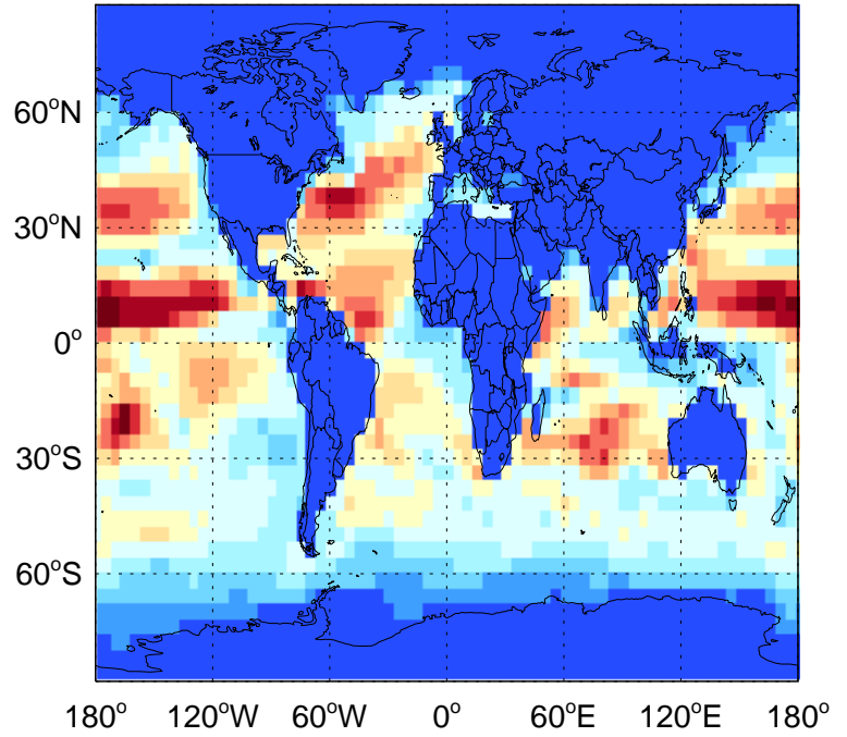
ACET ocean source emissions for Jan
