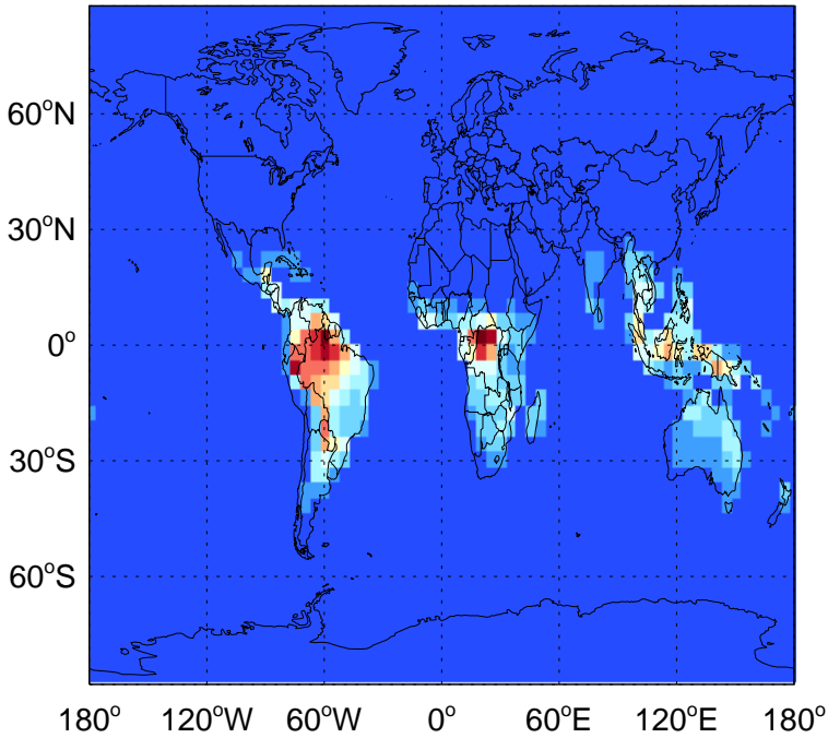
ACET direct emissions for Jan
