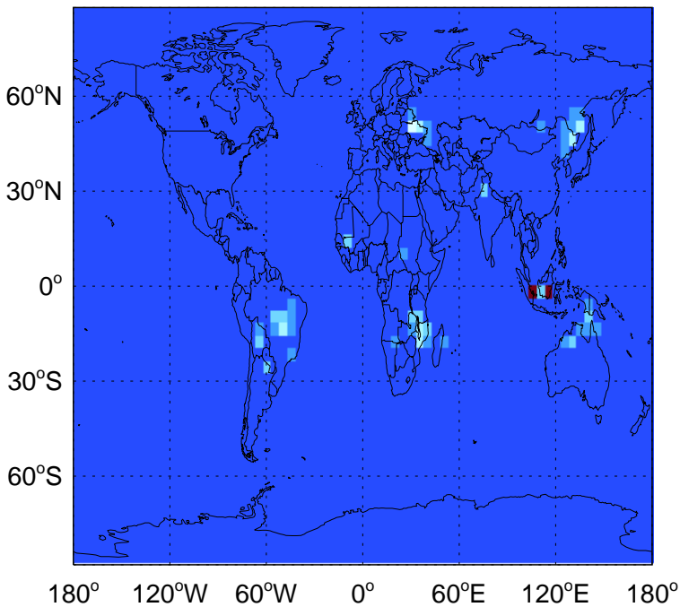
ALK4 biomass emissions for Oct
