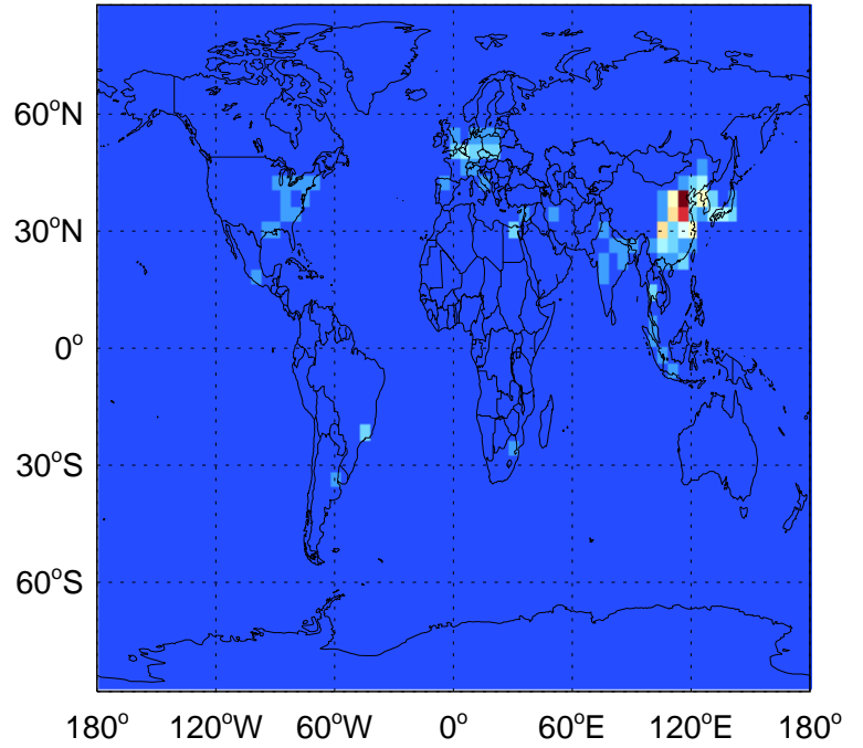
BC column anthro emissions for Apr
