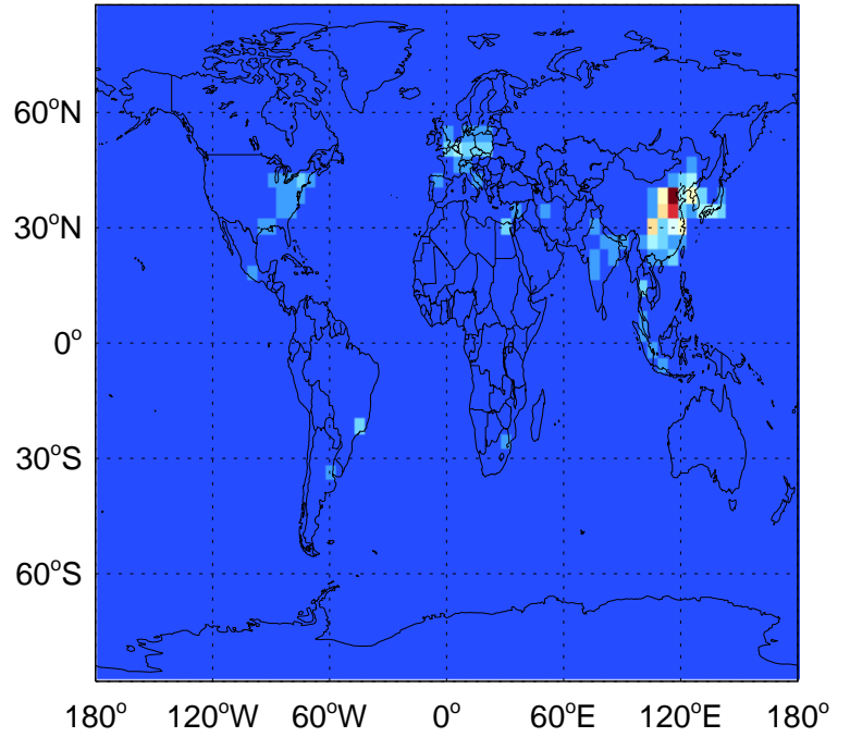
BC column anthro emissions for Jan
