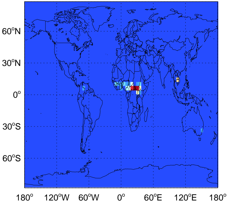
BC biomass emissions for Jan
