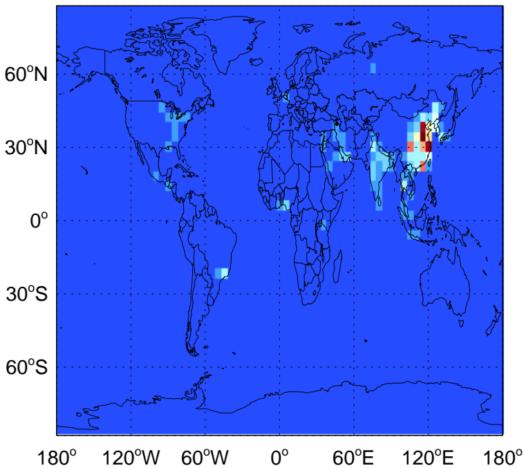
BC column anthro emissions for Oct
