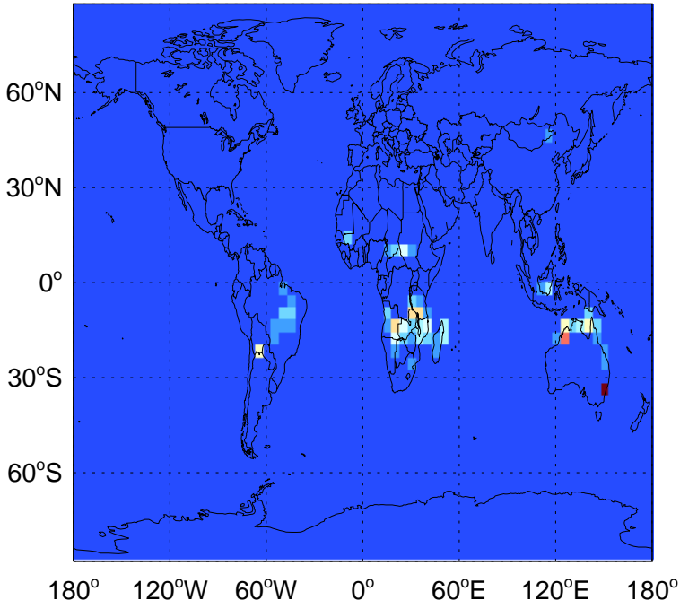
BC biomass emissions for Oct
