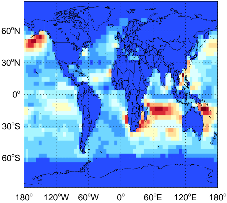
DMS biogenic emissions for Oct
