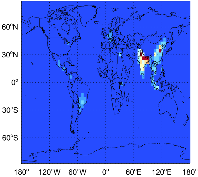
NH3 column anthro emissions for Jan
