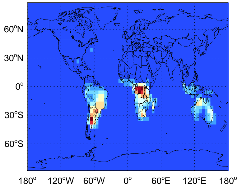
NO column lightning emissions for Jan
