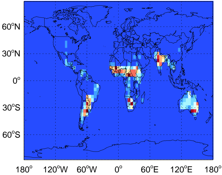
NO soil emissions for Jan
