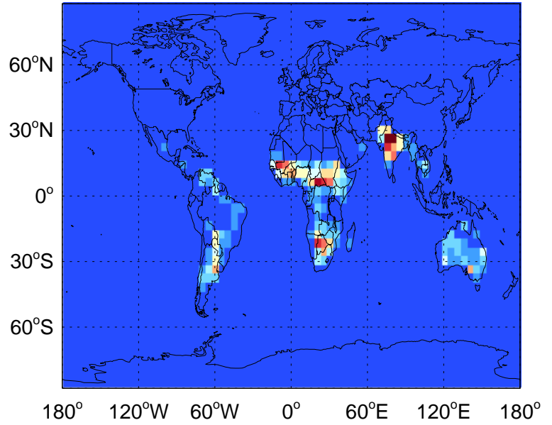
NO soil emissions for Jan
