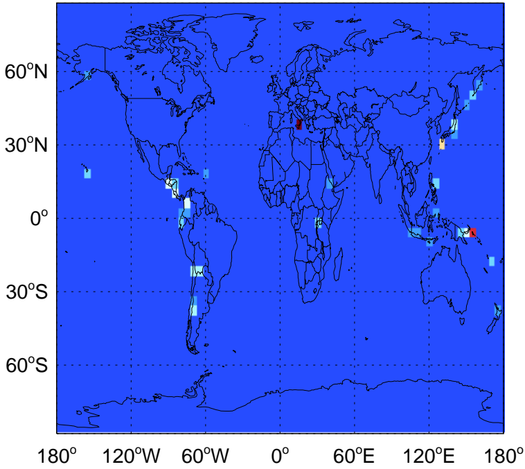
SO2 column nonerup volc emissions for Jan
