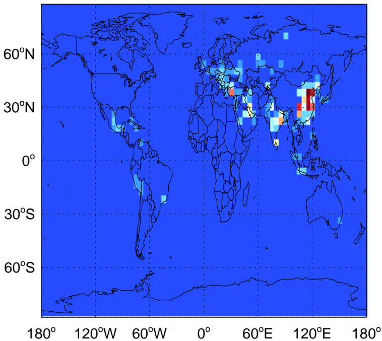
SO4 column anth+biof emissions for Oct
