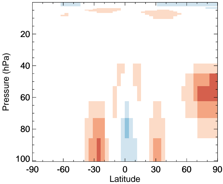
H2O2 - Strat zonal mean abs diff for Jan
