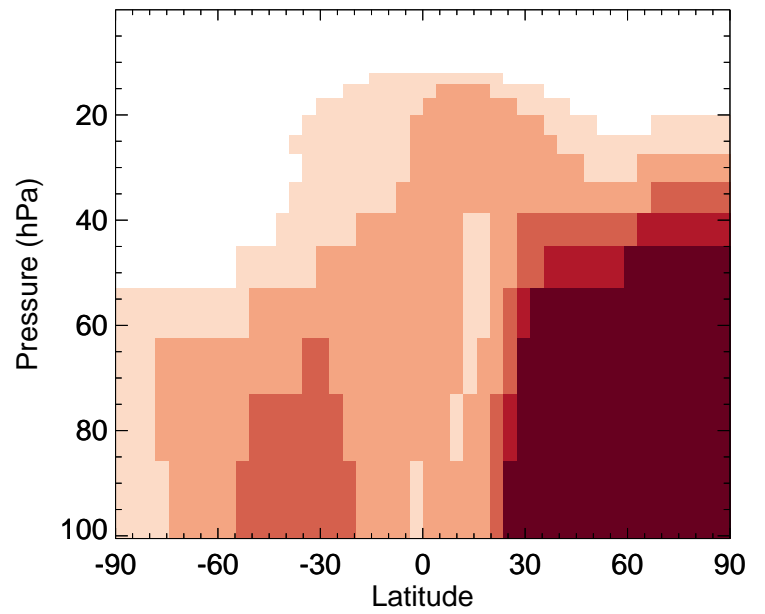
OCPI - Strat zonal mean % diff for Jan
