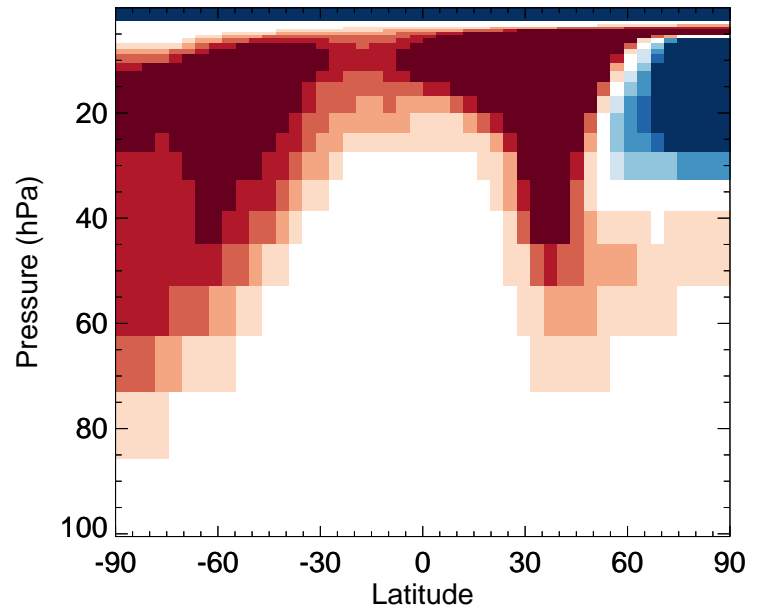
H2O2 - Strat zonal mean % diff for Jan
