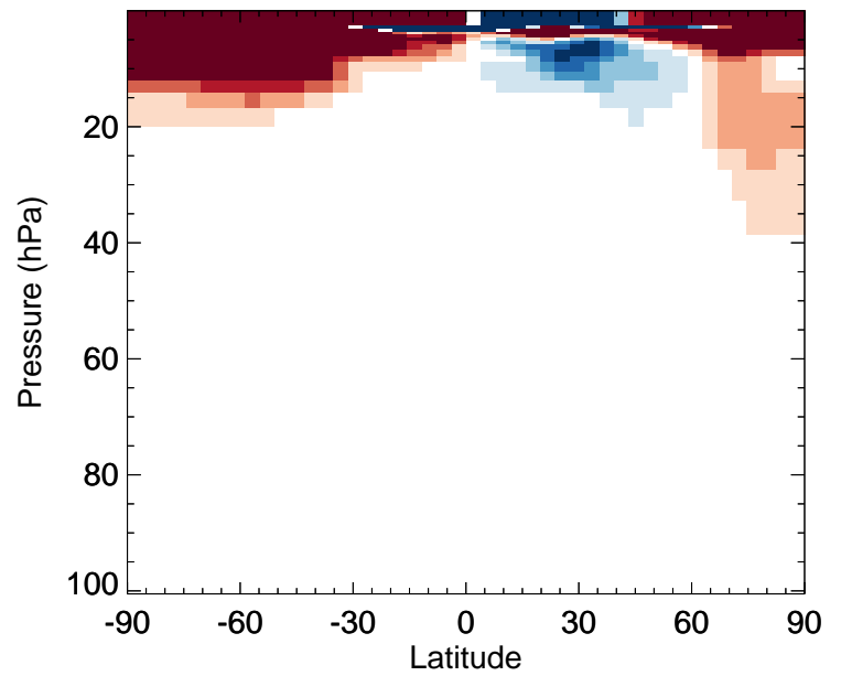
CFC11 - Strat zonal mean % diff for Jan
