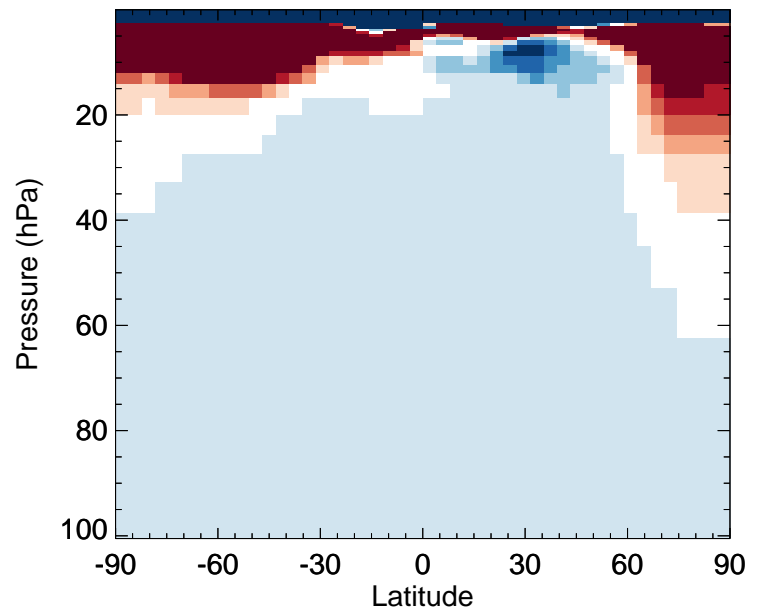
H2402 - Strat zonal mean % diff for Jan
