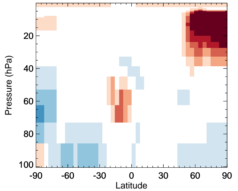
BrCl - Strat zonal mean % diff for Jan
