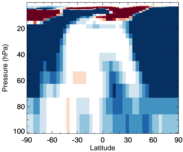
HNO 4 - Strat zonal mean abs diff for Jan
