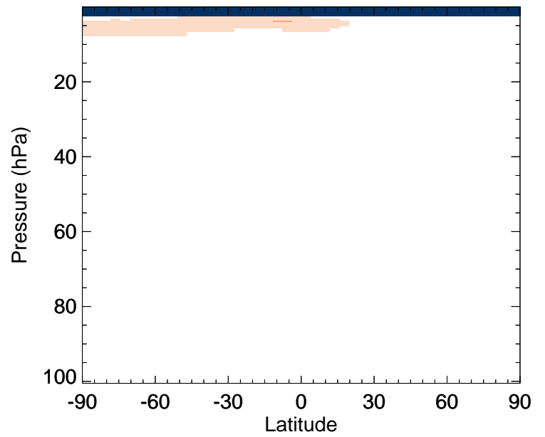
H2402 - Strat zonal mean % diff for Jan
