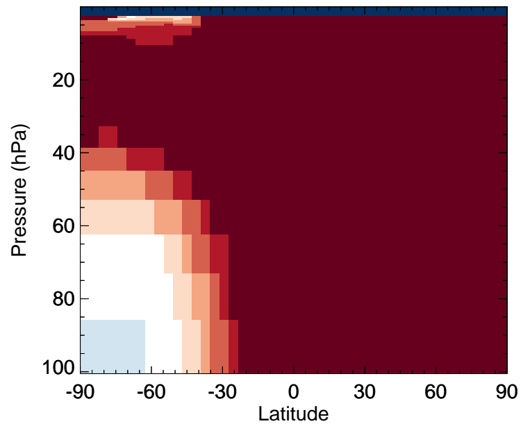
C2H6 - Strat zonal mean % diff for Jan
