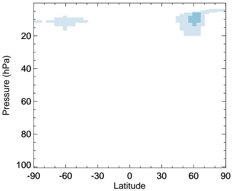
BrNO3 - Strat zonal mean abs diff for Jan
