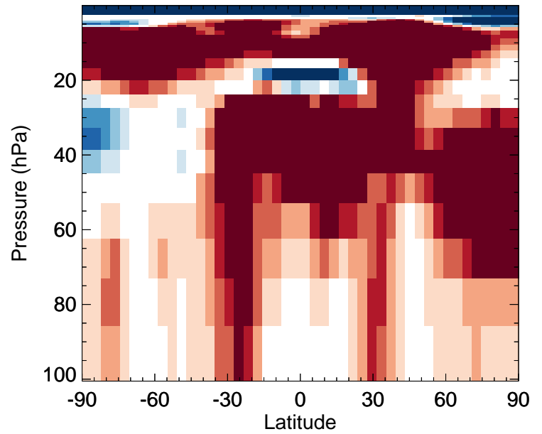
H2O2 - Strat zonal mean % diff for Jan
