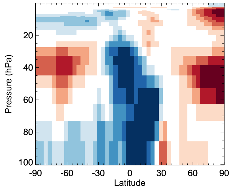
OCPI - Strat zonal mean % diff for Jan
