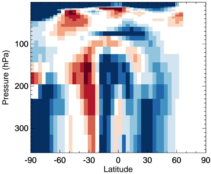
OH - Strat zonal mean abs diff for Jan
