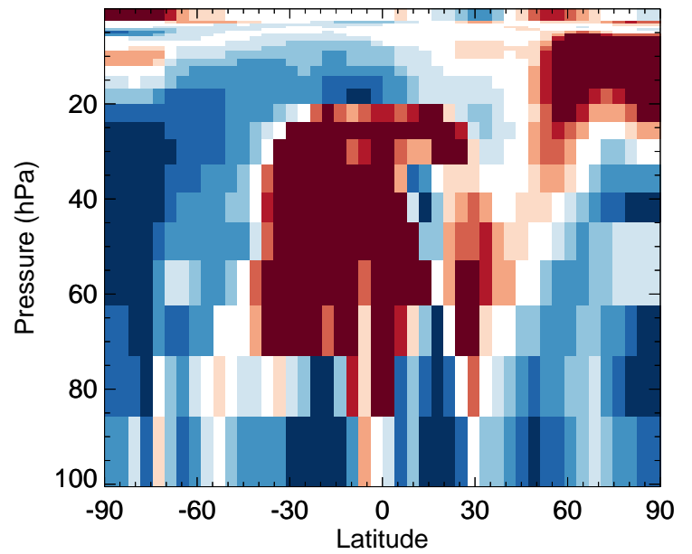
BrCl - Strat zonal mean % diff for Jan
