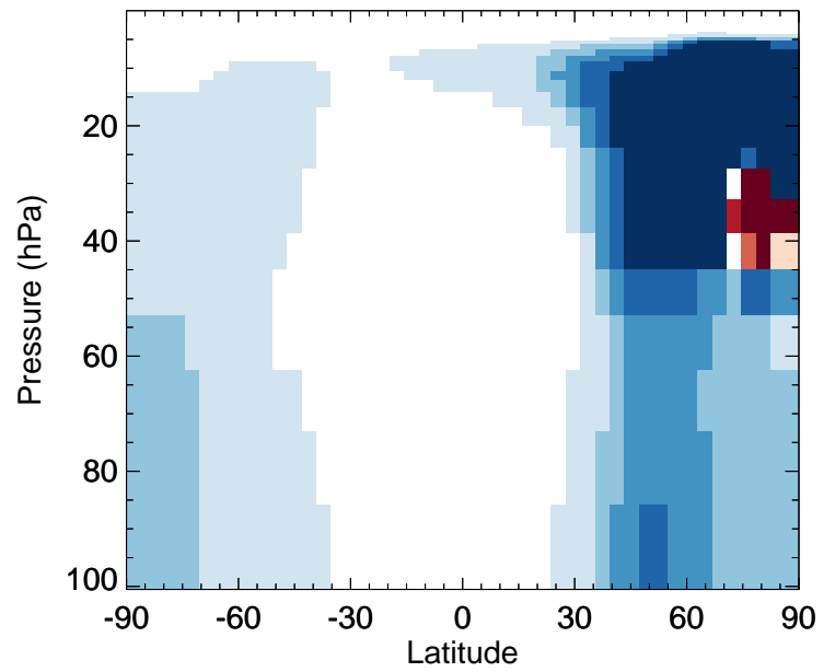
BrNO3 - Strat zonal mean % diff for Jan
