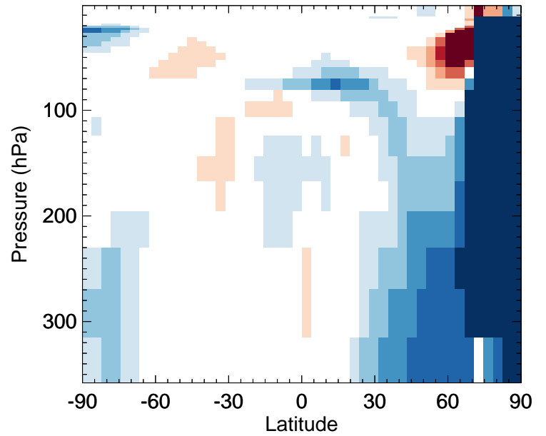
OH - Strat zonal mean % diff for Jan
