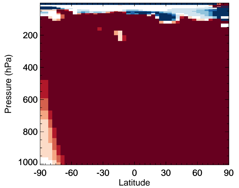
v11-02f-Run1 / v11-02e-Run1 RIPD - Zonal mean % diff for Apr
