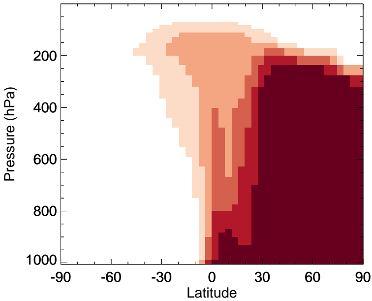
v11-02f-Run1 - v11-02e-Run0 C2H6 - Zonal mean abs diff for Apr
