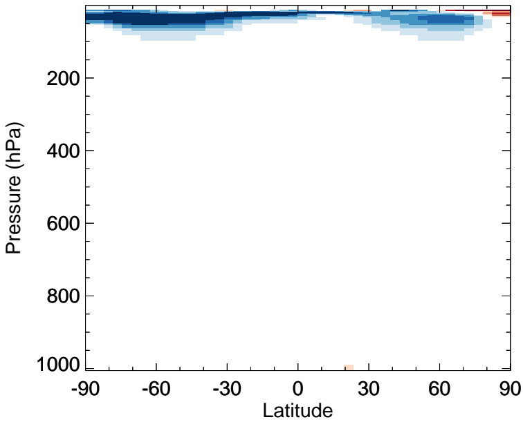
v11-02f-Run1 - v11-02e-Run0 NO 2 - Zonal mean abs diff for Apr
