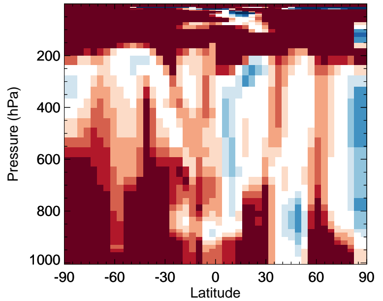
v11-02f-Run1 / v11-02e-Run0 MGLY - Zonal mean % diff for Apr
