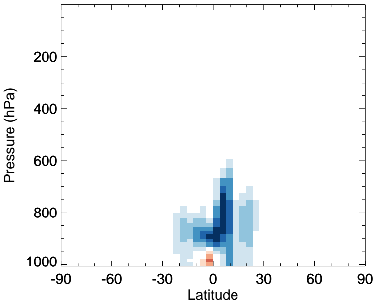
v11-02f-Run1 - v11-02e-Run0 MVK - Zonal mean abs diff for Apr
