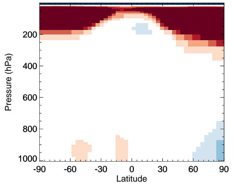
v11-02f-Run1 / v11-02e-Run1 H2O2 - Zonal mean % diff for Apr
