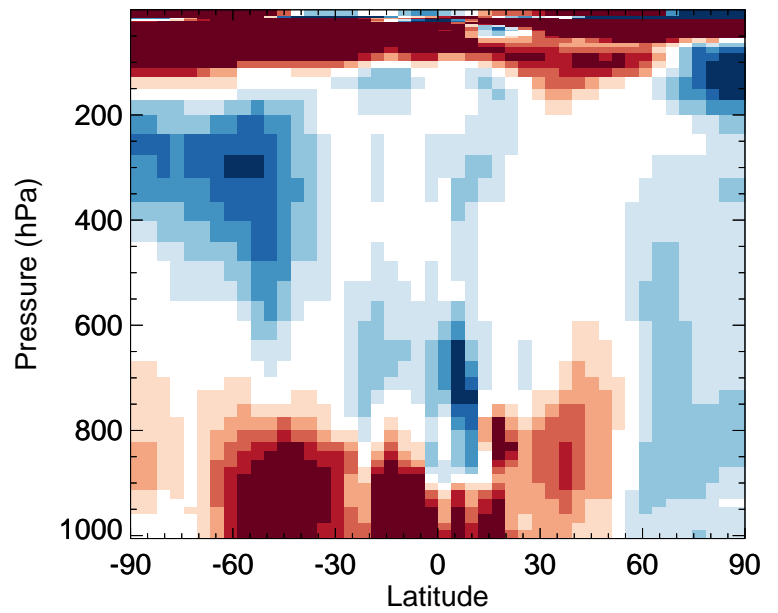
v11-02f-Run1 / v11-02e-Run0 PAN - Zonal mean % diff for Apr
