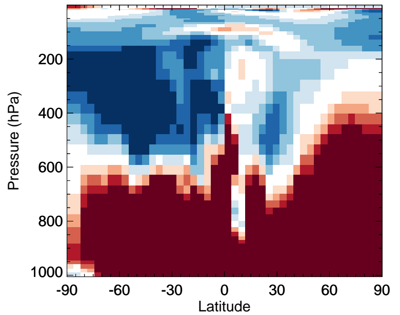
v11-02f-Run1 / v11-02e-Run0 TSOA0 - Zonal mean % diff for Apr
