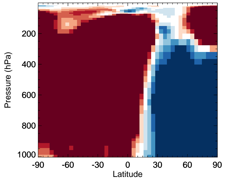
v11-02f-Run1 / v11-02e-Run0 ASOG1 - Zonal mean % diff for Apr
