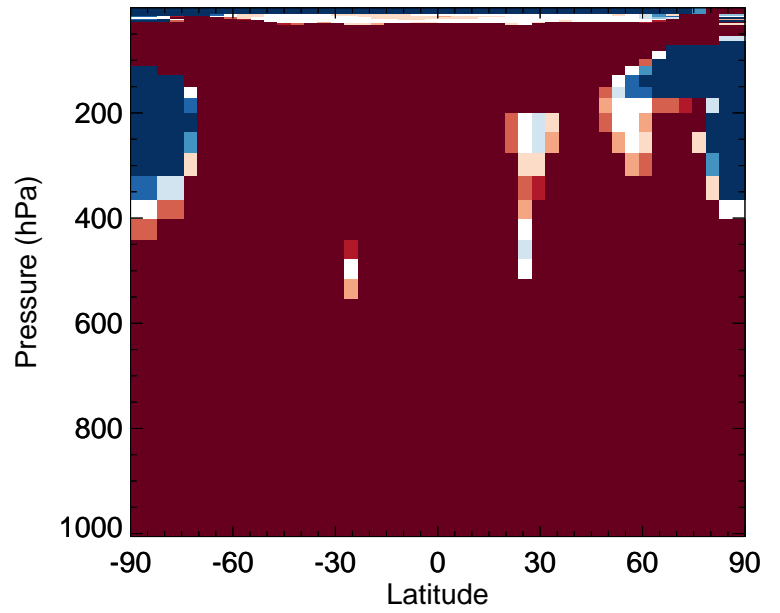
v11-02f-Run1 / v11-02e-Run0 IPMN - Zonal mean % diff for Apr
