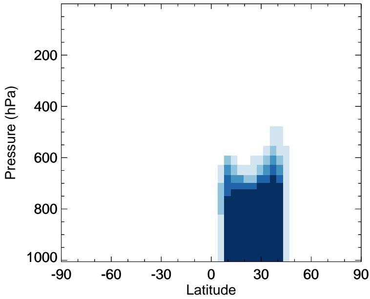
v11-02f-Run1 - v11-02e-Run0 DST3 - Zonal mean abs diff for Apr
