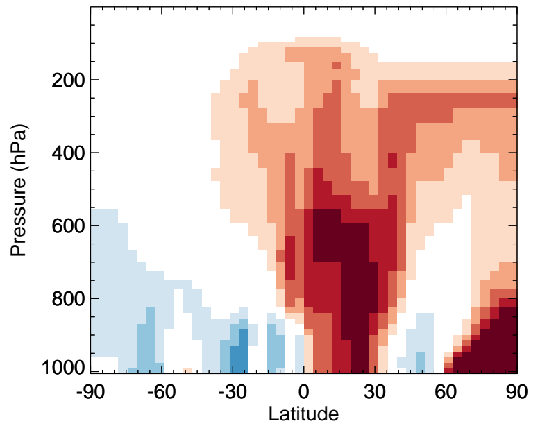
v11-02f-Run1 / v11-02e-Run1 BCPI - Zonal mean % diff for Apr
