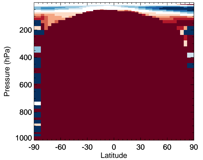
v11-02f-Run1 / v11-02e-Run1 MTPO - Zonal mean % diff for Apr
