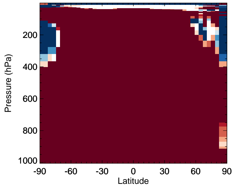
v11-02f-Run1 / v11-02e-Run0 MVK - Zonal mean % diff for Apr
