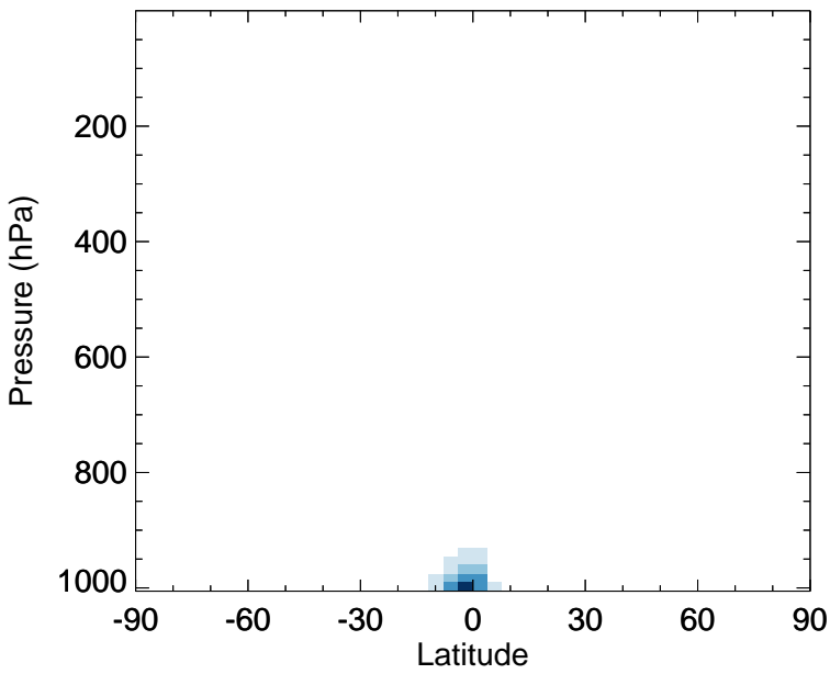
v11-02f-Run1 - v11-02e-Run1 MTPA - Zonal mean abs diff for Apr
