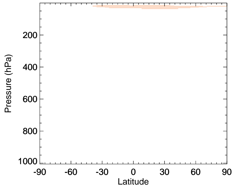
v11-02f-Run1 / v11-02e-Run1 CH2Br2 - Zonal mean % diff for Apr
