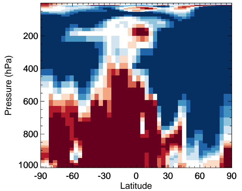
v11-02f-Run1 / v11-02e-Run0 ASOA2 - Zonal mean % diff for Apr
