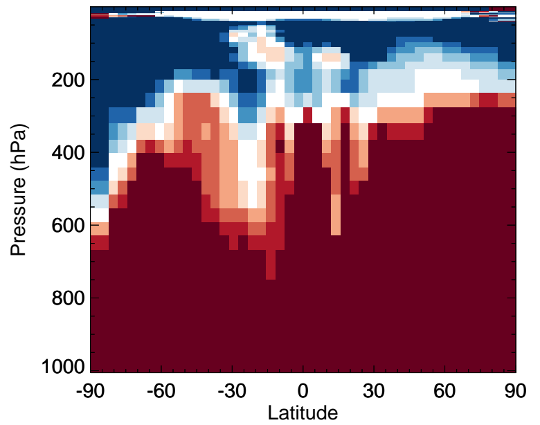
v11-02f-Run1 / v11-02e-Run1 MACR - Zonal mean % diff for Apr
