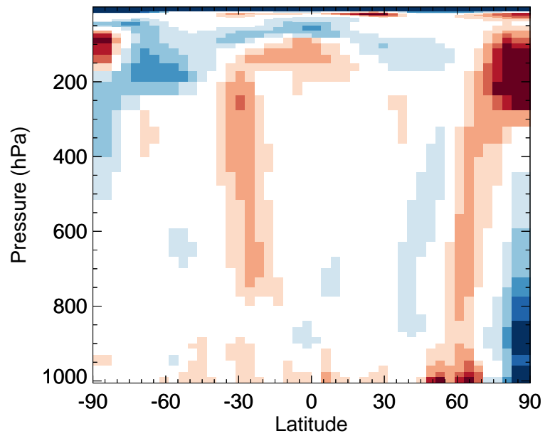
v11-02f-Run1 / v11-02e-Run0 CH 2 O - Zonal mean % diff for Apr
