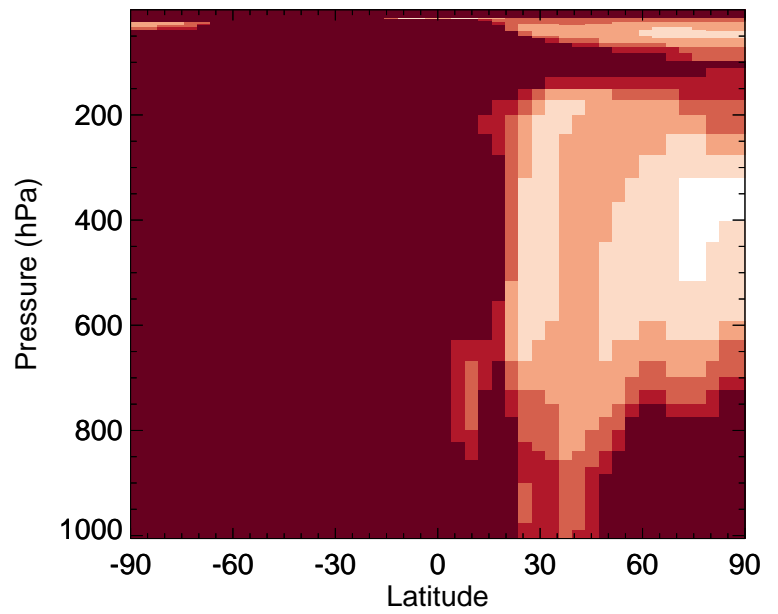
v11-02f-Run1 / v11-02e-Run1 R4N2 - Zonal mean % diff for Apr
