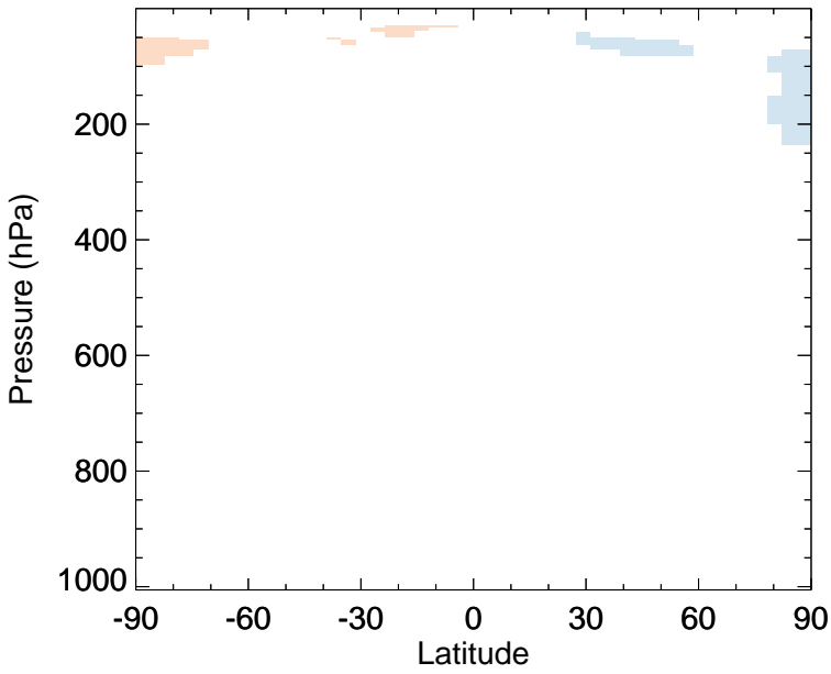
v11-02f-Run1 - v11-02e-Run0 CFC11 - Zonal mean abs diff for Apr
