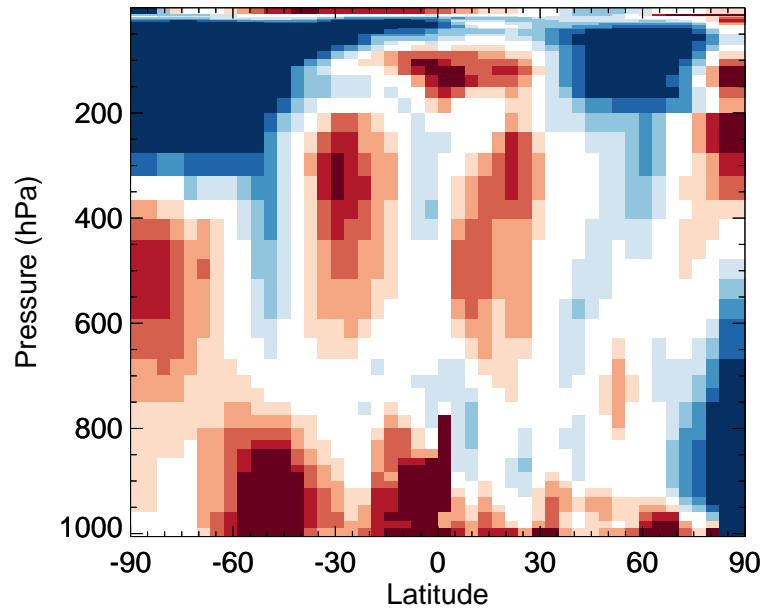
v11-02f-Run1 / v11-02e-Run0 NO 2 - Zonal mean % diff for Apr
