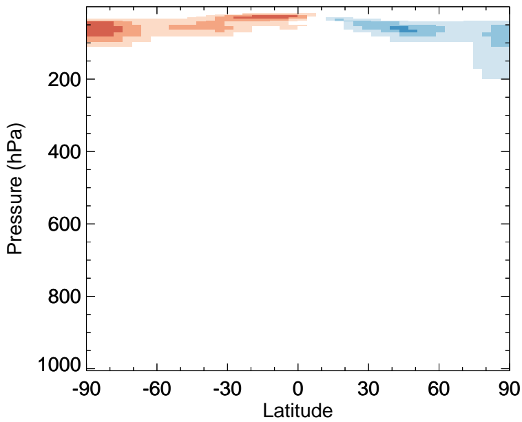
v11-02f-Run1 - v11-02e-Run0 OCS - Zonal mean abs diff for Apr
