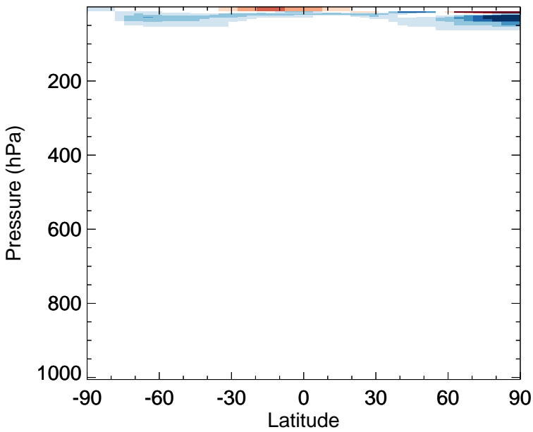
v11-02f-Run1 - v11-02e-Run0 NO - Zonal mean abs diff for Apr
