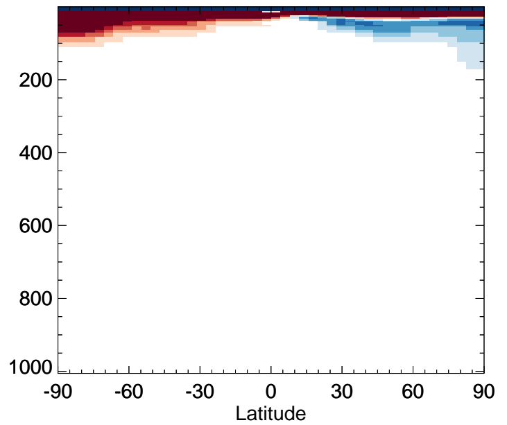
v11-02f-Run1 / v11-02e-Run0 OCS - Zonal mean % diff for Apr
