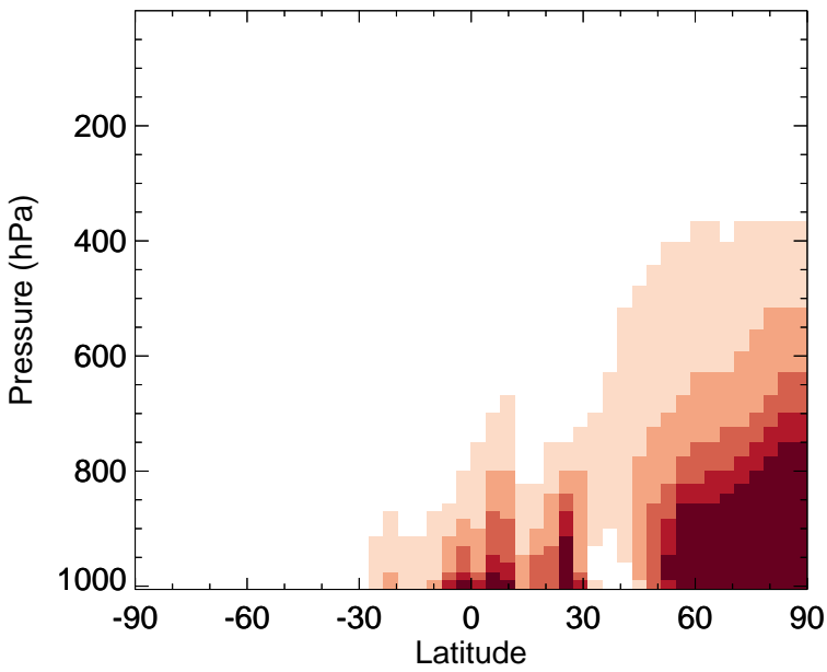
v11-02f-Run1 - v11-02e-Run1 ALK4 - Zonal mean abs diff for Apr
