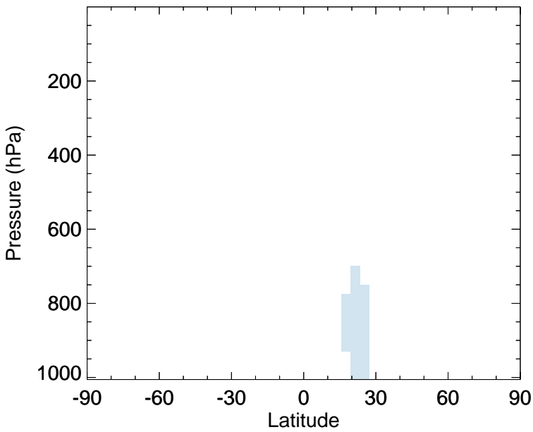
v11-02f-Run1 - v11-02e-Run0 SOAGX - Zonal mean abs diff for Apr
