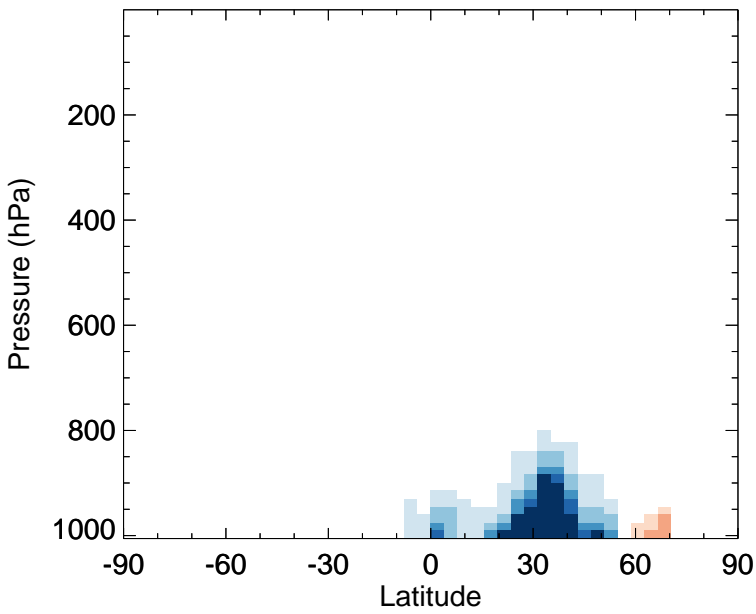
v11-02f-Run1 - v11-02e-Run1 XYLE - Zonal mean abs diff for Apr
