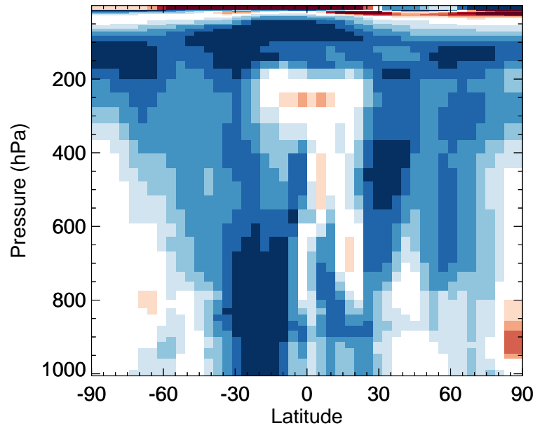
v11-02f-Run1 / v11-02e-Run0 SO4 - Zonal mean % diff for Apr
