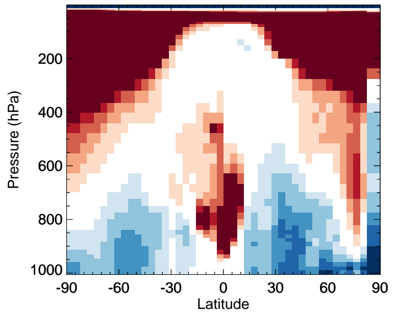
v11-02f-Run1 / v11-02e-Run1 OCIO - Zonal mean % diff for Apr
