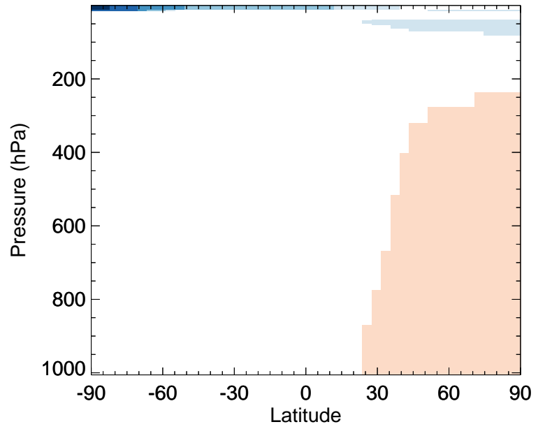
v11-02f-Run1 / v11-02e-Run1 CO - Zonal mean % diff for Apr
