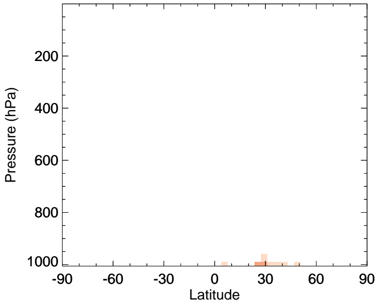
v11-02f-Run1 - v11-02e-Run0 SOAP - Zonal mean abs diff for Apr
