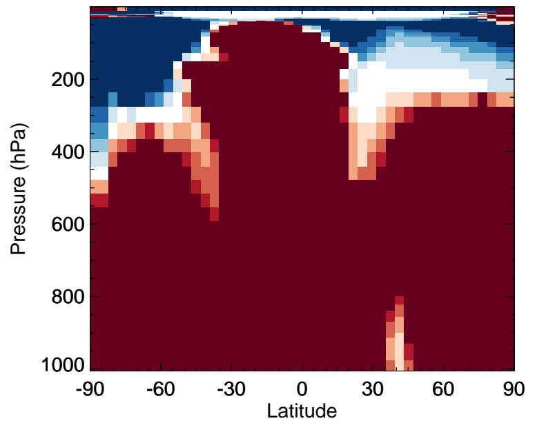
v11-02f-Run1 / v11-02e-Run1 PRPE - Zonal mean % diff for Apr
