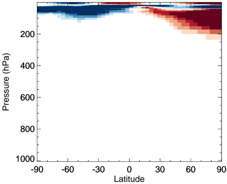
v11-02f-Run1 - v11-02e-Run0 HCl - Zonal mean abs diff for Apr
