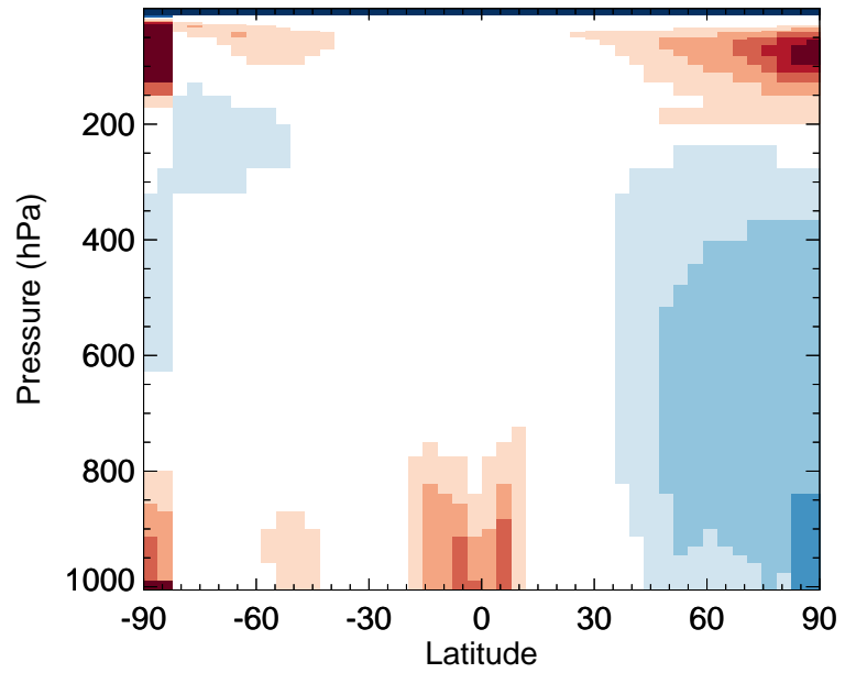
v11-02f-Run1 / v11-02e-Run1 OH - Zonal mean % diff for Apr
