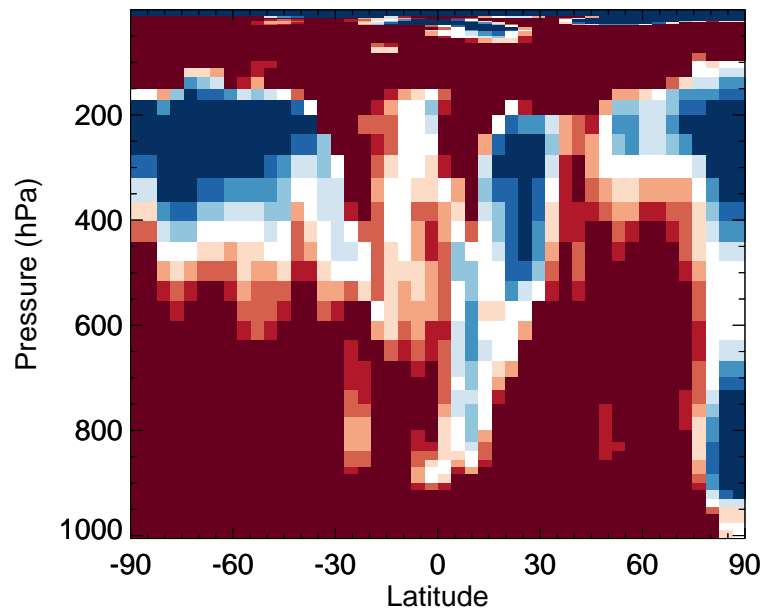
v11-02f-Run1 / v11-02e-Run0 HCOOH - Zonal mean % diff for Apr
