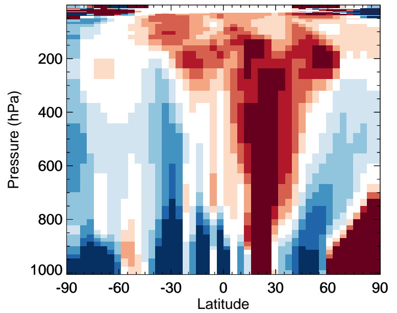
v11-02f-Run1 / v11-02e-Run1 BCPO - Zonal mean % diff for Apr
