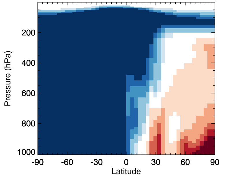
v11-02f-Run1 / v11-02e-Run1 SOAME - Zonal mean % diff for Apr
