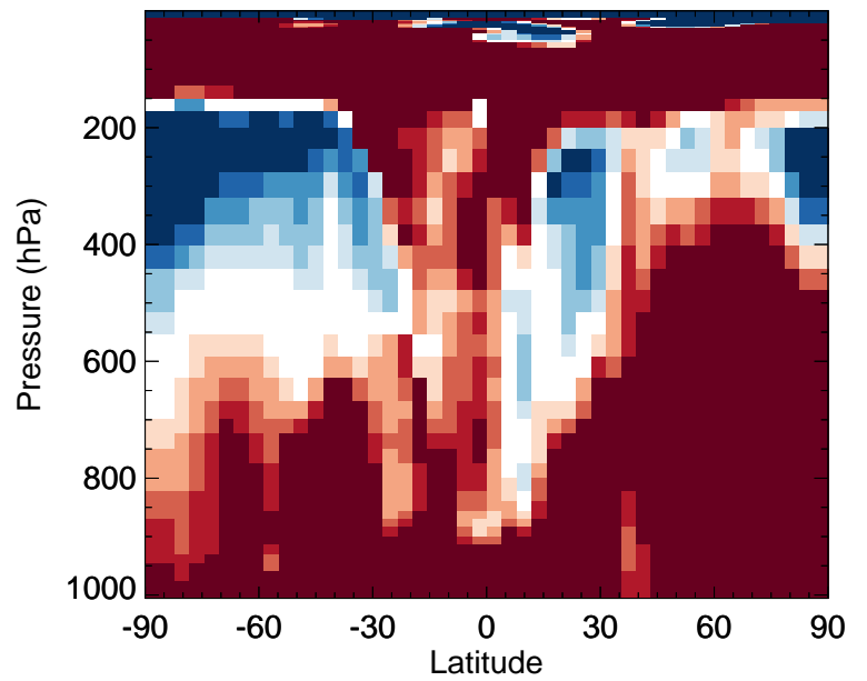
v11-02f-Run1 / v11-02e-Run0 HAC - Zonal mean % diff for Apr
