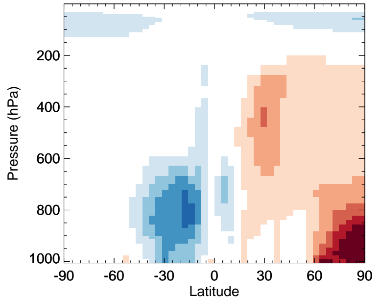
v11-02f-Run1 / v11-02e-Run1 SO 2 - Zonal mean % diff for Apr
