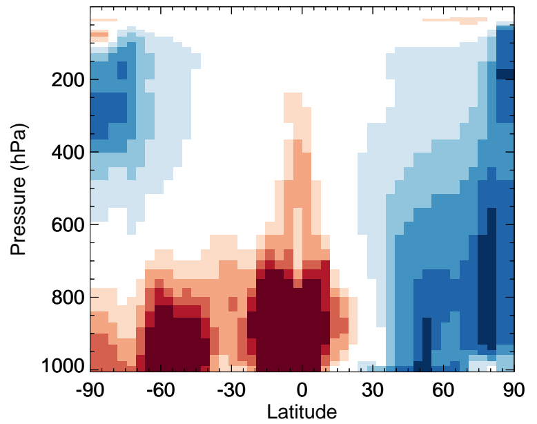
v11-02f-Run1 / v11-02e-Run1 NO3 - Zonal mean % diff for Apr
