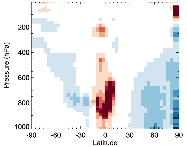
v11-02f-Run1 / v11-02e-Run1 BrCl - Zonal mean % diff for Apr
