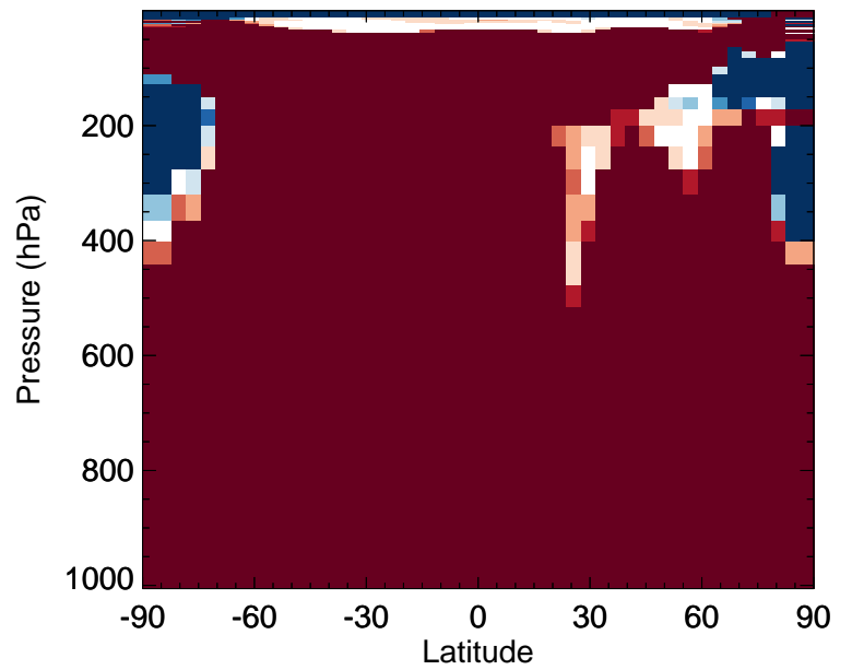
v11-02f-Run1 / v11-02e-Run0 MACR - Zonal mean % diff for Apr
