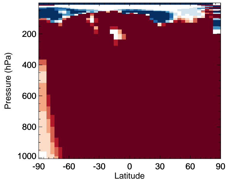
v11-02f-Run1 / v11-02e-Run1 RIPA - Zonal mean % diff for Apr
