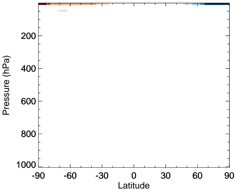
v11-02f-Run1 - v11-02e-Run1 ClO - Zonal mean abs diff for Apr
