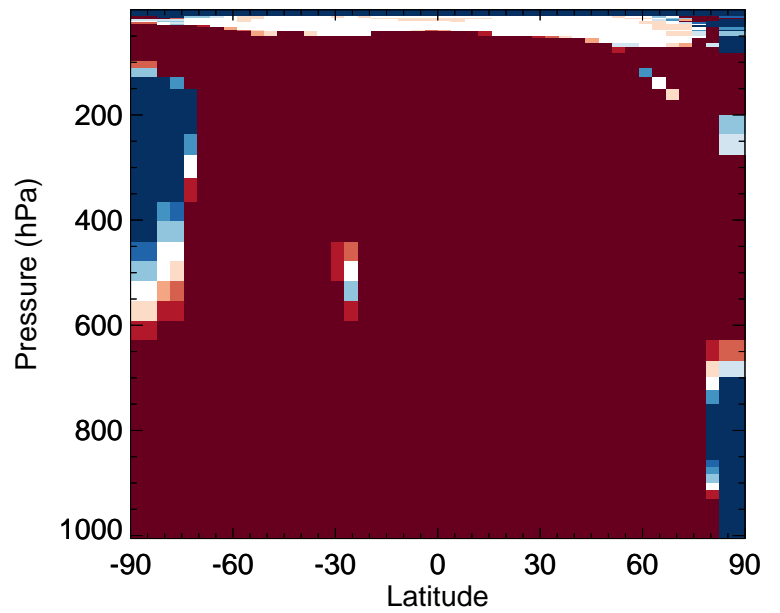
v11-02f-Run1 / v11-02e-Run0 ETHLN - Zonal mean % diff for Apr
