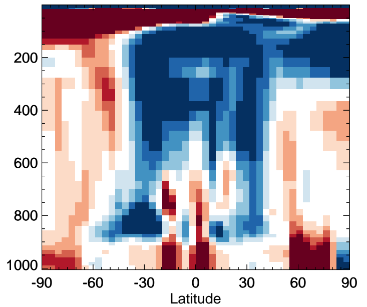
v11-02f-Run1 / v11-02e-Run0 SALA - Zonal mean % diff for Apr
