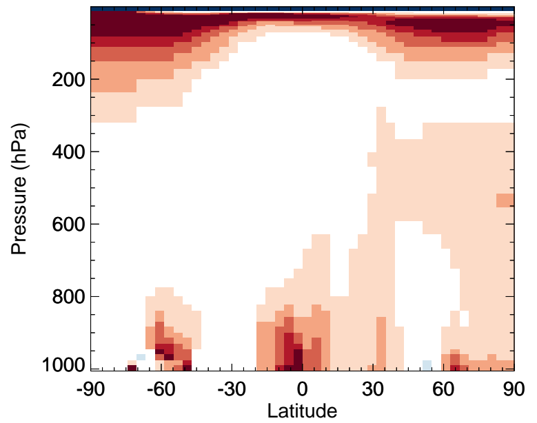
v11-02f-Run1 / v11-02e-Run1 HNO 3 - Zonal mean % diff for Apr
