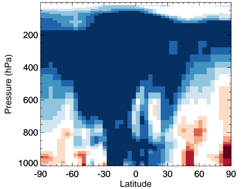
v11-02f-Run1 / v11-02e-Run0 NH4 - Zonal mean % diff for Apr
