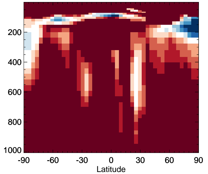
v11-02f-Run1 / v11-02e-Run0 RCHO - Zonal mean % diff for Apr
