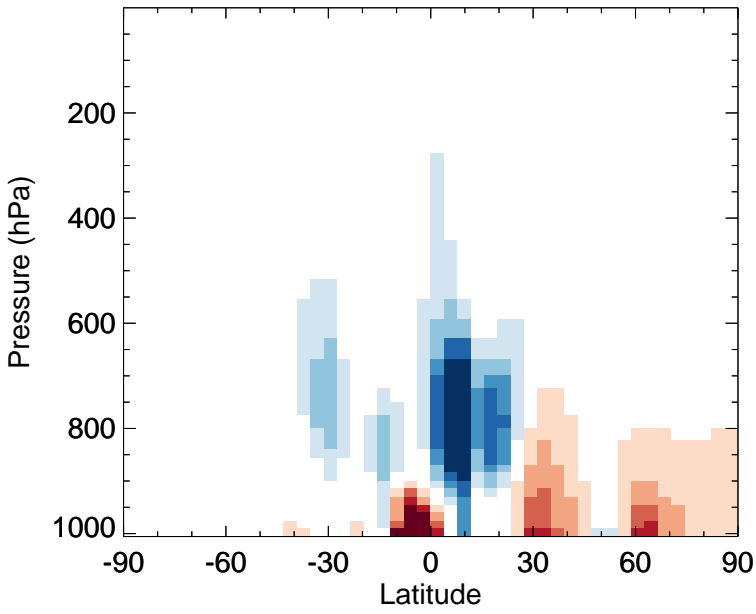
v11-02f-Run1 - v11-02e-Run1 MEK - Zonal mean abs diff for Apr
