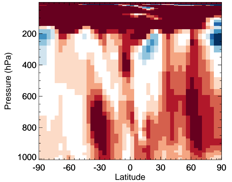
v11-02f-Run1 / v11-02e-Run0 MAP - Zonal mean % diff for Apr
