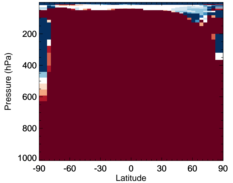
v11-02f-Run1 / v11-02e-Run0 MOBA - Zonal mean % diff for Apr
