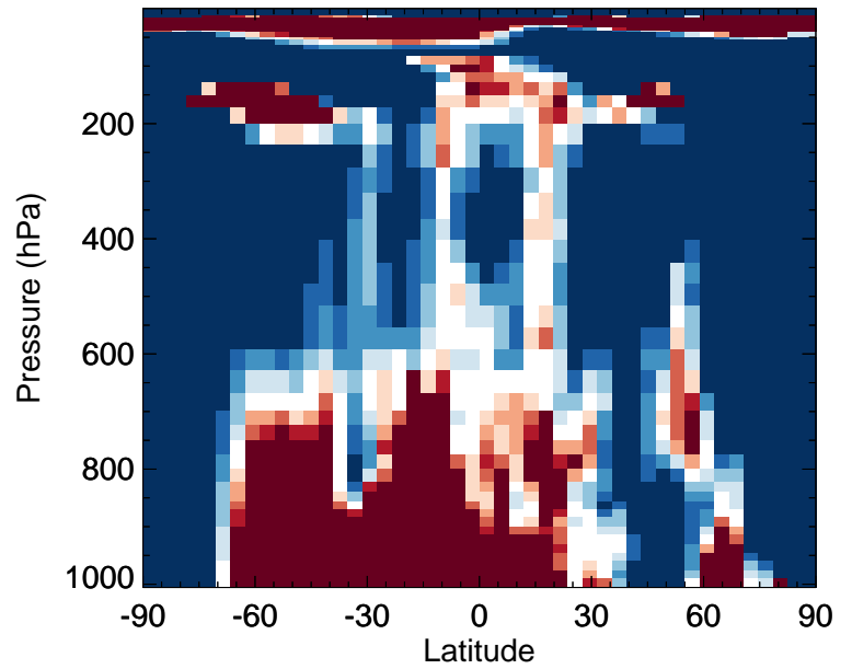
v11-02f-Run1 / v11-02e-Run0 ClNO 2 - Zonal mean % diff for Apr
