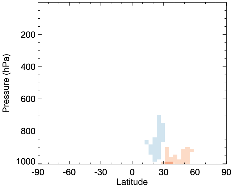
v11-02f-Run1 - v11-02e-Run0 NH4 - Zonal mean abs diff for Apr
