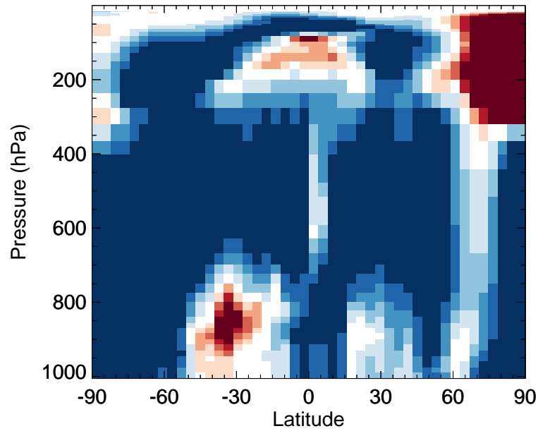
v11-02f-Run1 / v11-02e-Run0 ISOG1 - Zonal mean % diff for Apr
