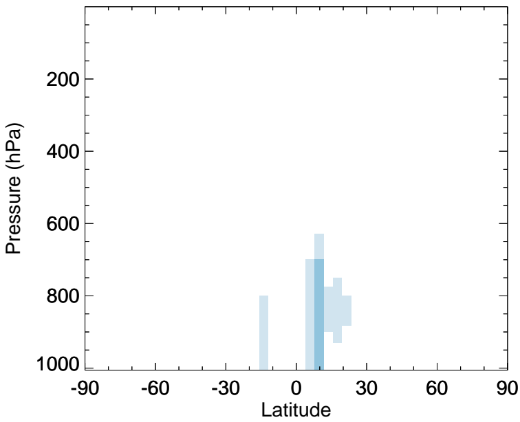
v11-02f-Run1 - v11-02e-Run1 GLYC - Zonal mean abs diff for Apr
