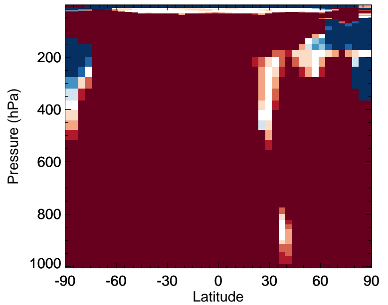
v11-02f-Run1 / v11-02e-Run0 PRPE - Zonal mean % diff for Apr
