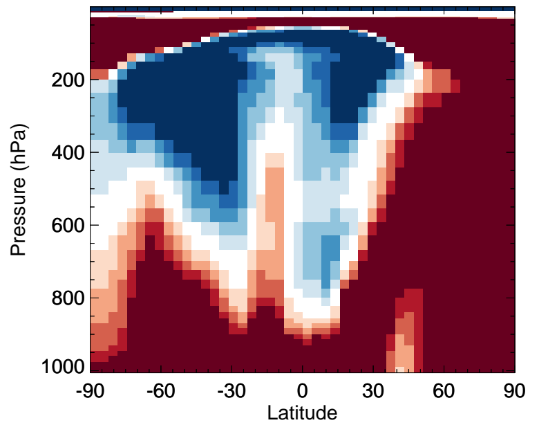
v11-02f-Run1 / v11-02e-Run1 HAC - Zonal mean % diff for Apr
