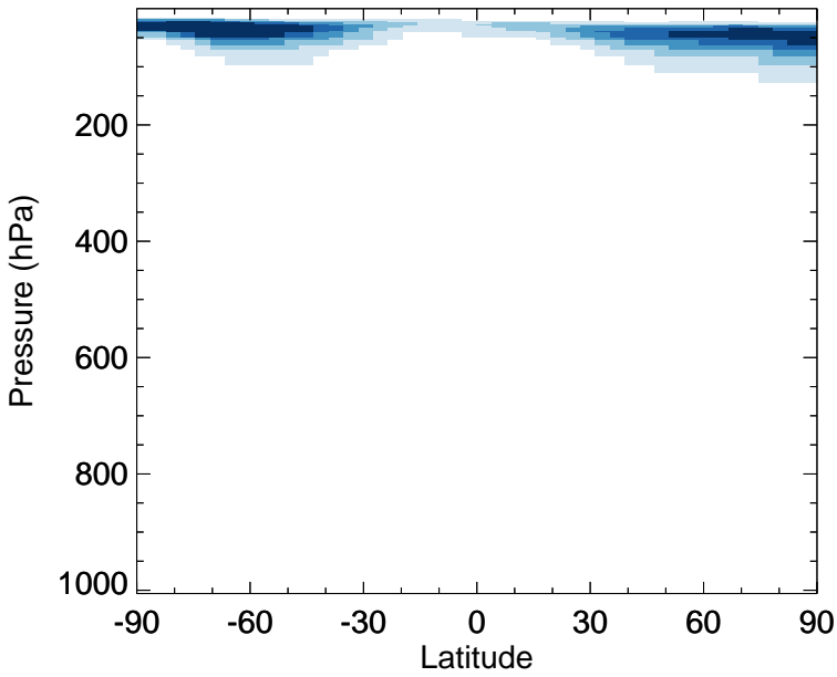
v11-02f-Run1 - v11-02e-Run1 NO 2 - Zonal mean abs diff for Apr
