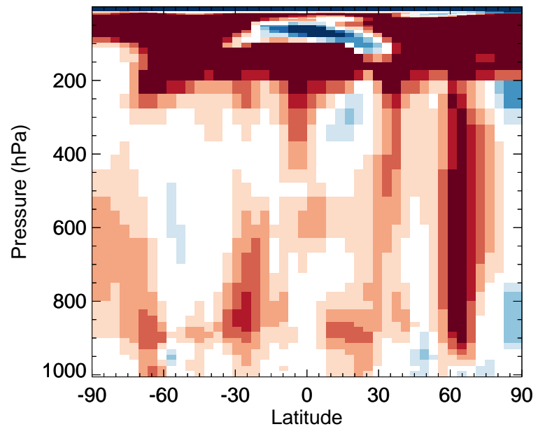
v11-02f-Run1 / v11-02e-Run0 H2O2 - Zonal mean % diff for Apr
