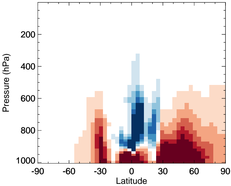
v11-02f-Run1 - v11-02e-Run0 MEK - Zonal mean abs diff for Apr
