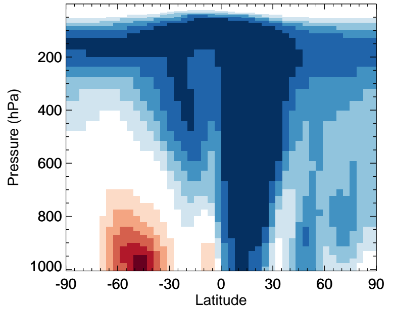
v11-02f-Run1 / v11-02e-Run1 ISN1OA - Zonal mean % diff for Apr
