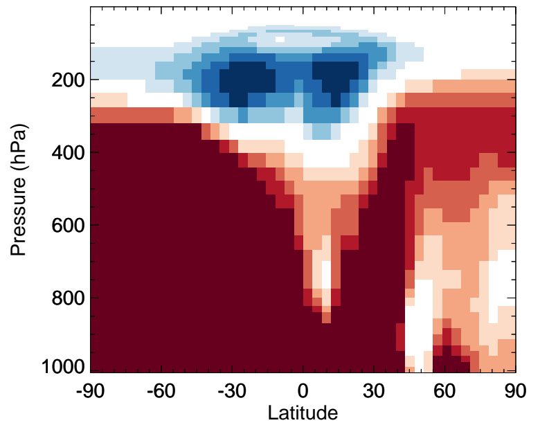
v11-02f-Run1 / v11-02e-Run1 TSOA3 - Zonal mean % diff for Apr
