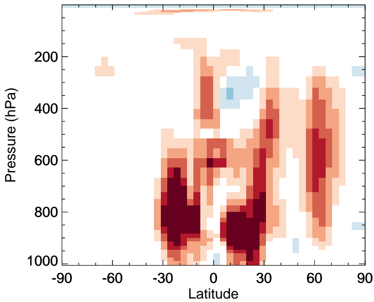
v11-02f-Run1 - v11-02e-Run0 H2O2 - Zonal mean abs diff for Apr
