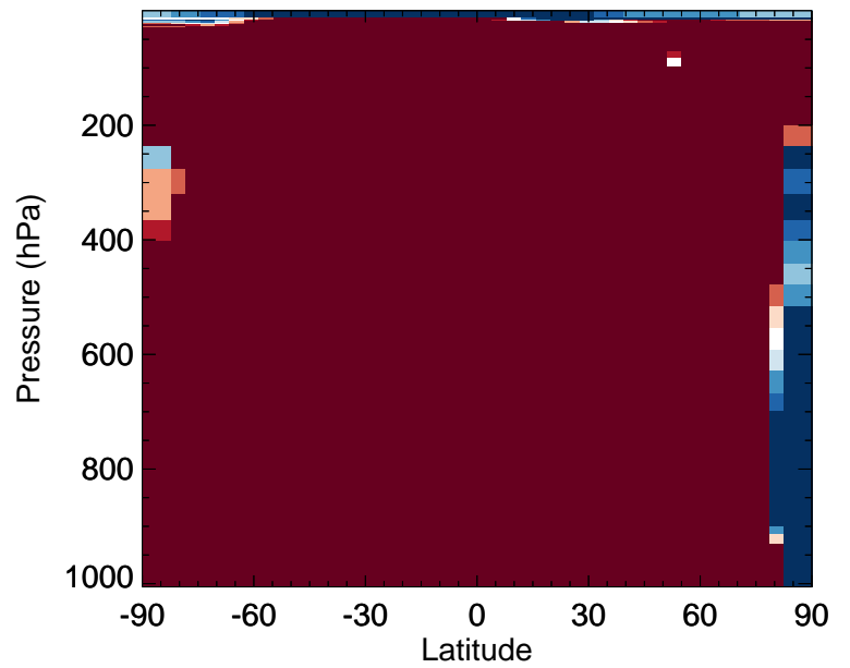
v11-02f-Run1 / v11-02e-Run0 ISN1OG - Zonal mean % diff for Apr
