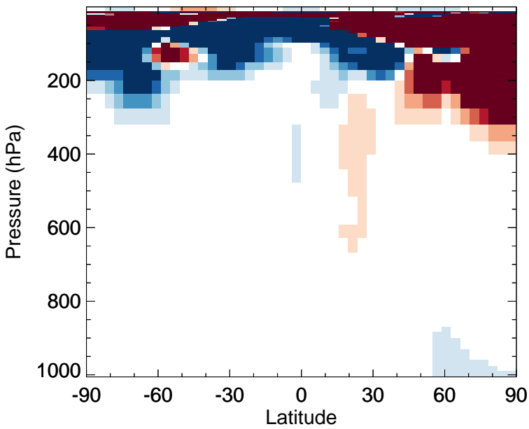
v11-02f-Run1 - v11-02e-Run0 O3 - Zonal mean abs diff for Apr
