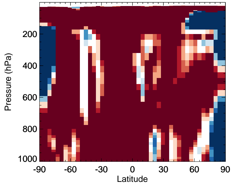
v11-02f-Run1 / v11-02e-Run0 SOAP - Zonal mean % diff for Apr
