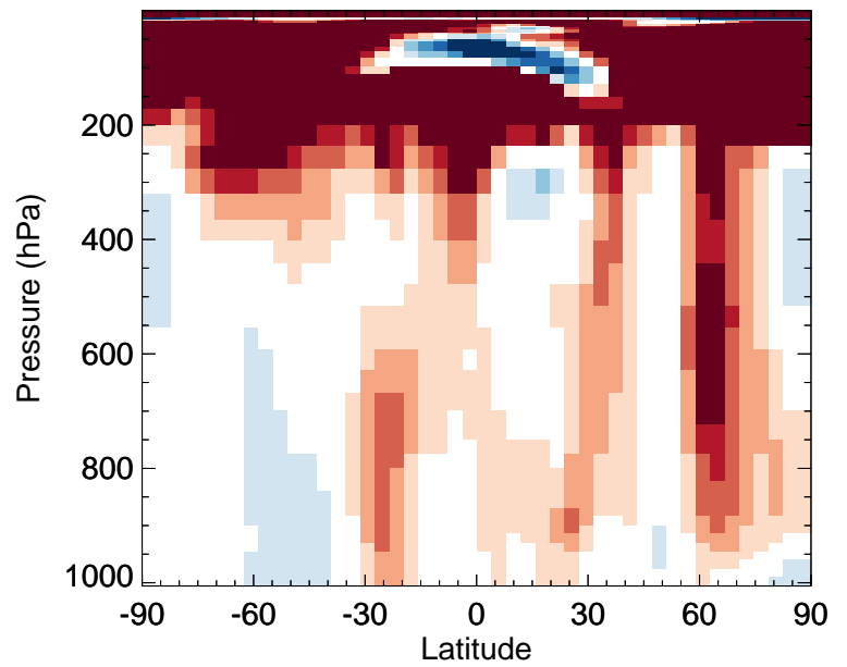
v11-02f-Run1 / v11-02e-Run0 MP - Zonal mean % diff for Apr
