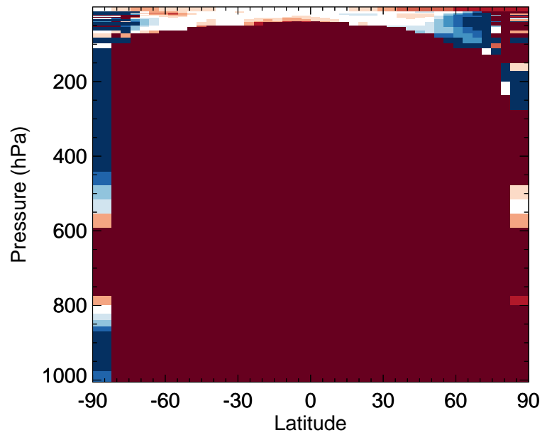
v11-02f-Run1 / v11-02e-Run0 MTPA - Zonal mean % diff for Apr
