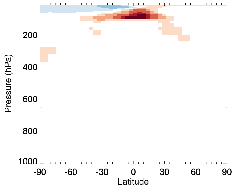
v11-02f-Run1 / v11-02e-Run1 SALC - Zonal mean % diff for Apr
