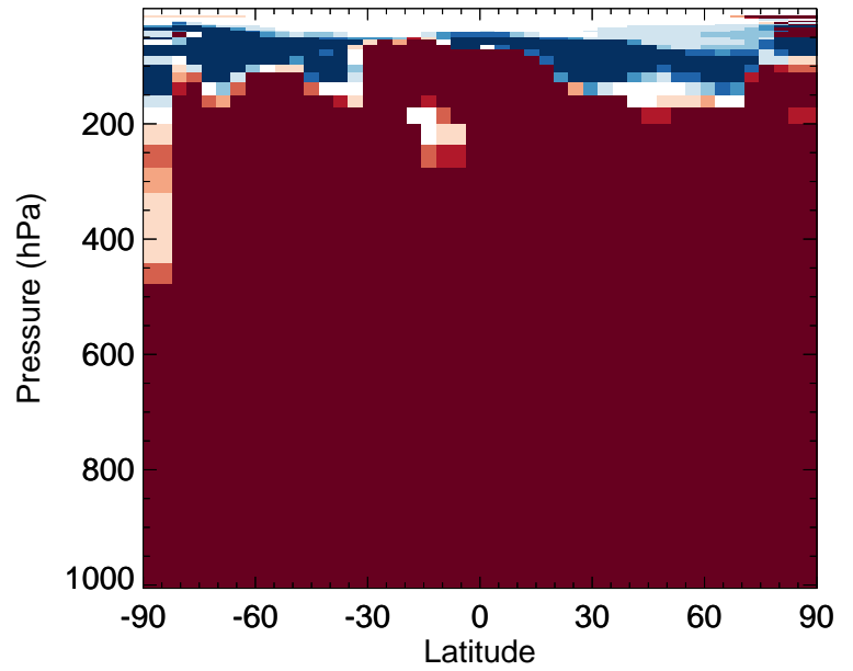
v11-02f-Run1 / v11-02e-Run1 MOBA - Zonal mean % diff for Apr
