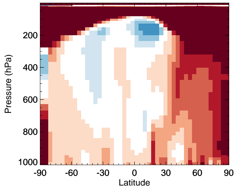
v11-02f-Run1 / v11-02e-Run1 ACTA - Zonal mean % diff for Apr
