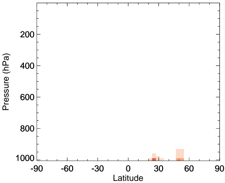
v11-02f-Run1 - v11-02e-Run0 OCPO - Zonal mean abs diff for Apr
