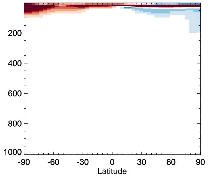
v11-02f-Run1 / v11-02e-Run0 CFC12 - Zonal mean % diff for Apr
