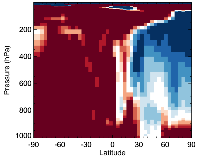
v11-02f-Run1 / v11-02e-Run0 GLYX - Zonal mean % diff for Apr
