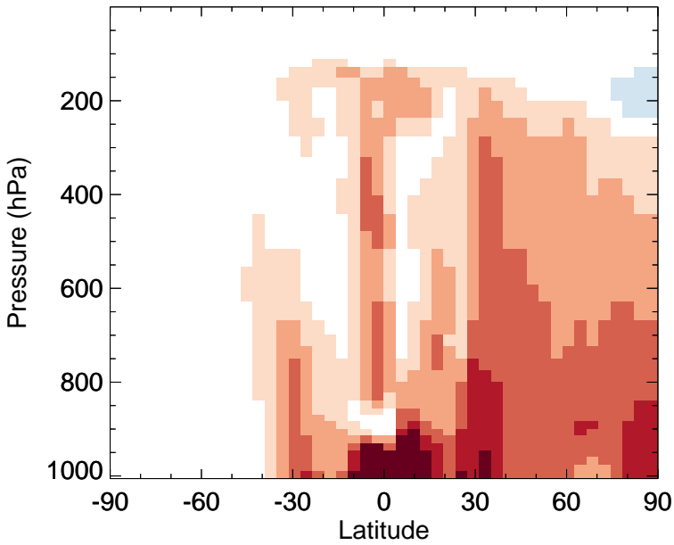
v11-02f-Run1 - v11-02e-Run0 ACET - Zonal mean abs diff for Apr
