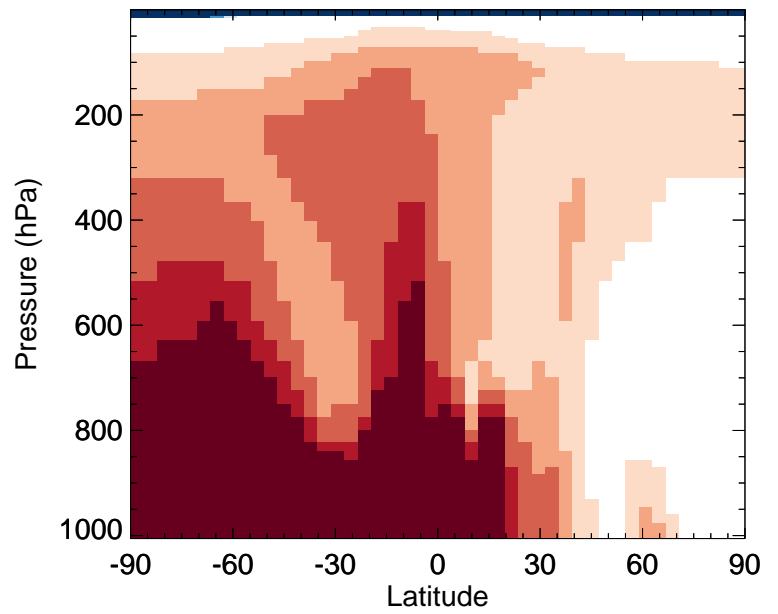
v11-02f-Run1 / v11-02e-Run1 PPN - Zonal mean % diff for Apr
