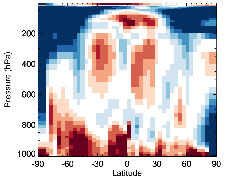
v11-02f-Run1 / v11-02e-Run0 NO - Zonal mean % diff for Apr
