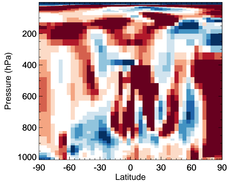
v11-02f-Run1 / v11-02e-Run0 SO 2 - Zonal mean % diff for Apr
