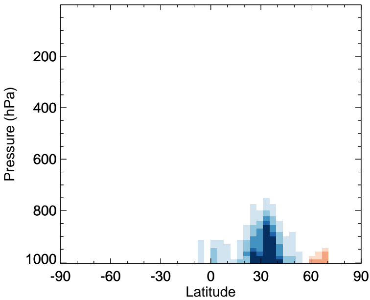
v11-02f-Run1 - v11-02e-Run0 XYLE - Zonal mean abs diff for Apr
