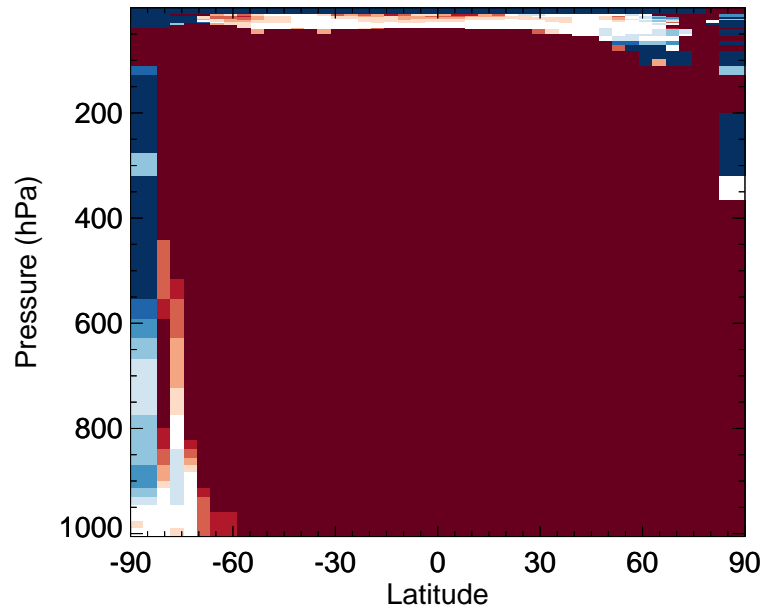
v11-02f-Run1 / v11-02e-Run0 ISOP - Zonal mean % diff for Apr
