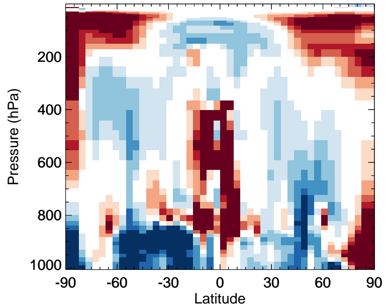
v11-02f-Run1 / v11-02e-Run0 BrO - Zonal mean % diff for Apr
