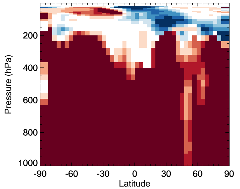
v11-02f-Run1 / v11-02e-Run1 ISN1OG - Zonal mean % diff for Apr
