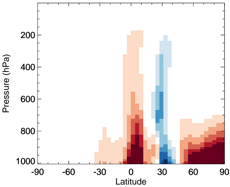
v11-02f-Run1 - v11-02e-Run1 BENZ - Zonal mean abs diff for Apr
