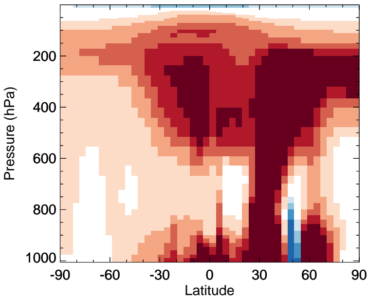
v11-02f-Run1 - v11-02e-Run1 PPN - Zonal mean abs diff for Apr
