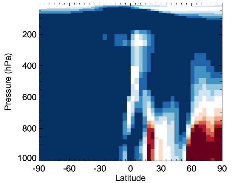
v11-02f-Run1 / v11-02e-Run0 SOAIE - Zonal mean % diff for Apr
