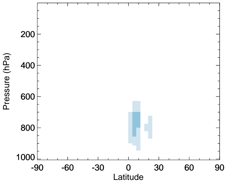
v11-02f-Run1 - v11-02e-Run0 HAC - Zonal mean abs diff for Apr
