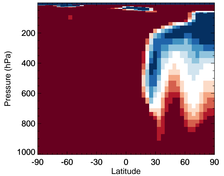
v11-02f-Run1 / v11-02e-Run0 BENZ - Zonal mean % diff for Apr
