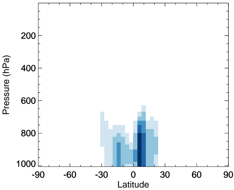
v11-02f-Run1 - v11-02e-Run1 MVK - Zonal mean abs diff for Apr
