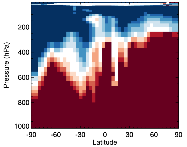
v11-02f-Run1 / v11-02e-Run1 IPMN - Zonal mean % diff for Apr
