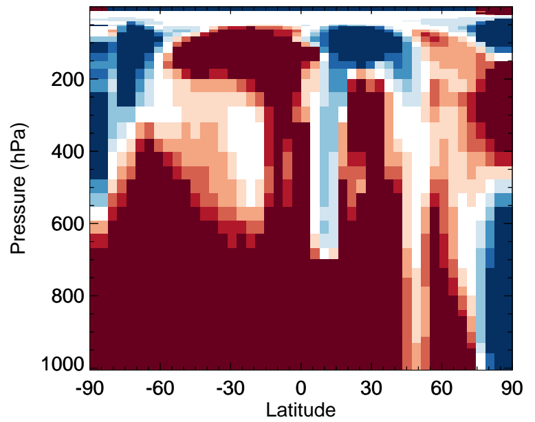
v11-02f-Run1 / v11-02e-Run1 NPMN - Zonal mean % diff for Apr
