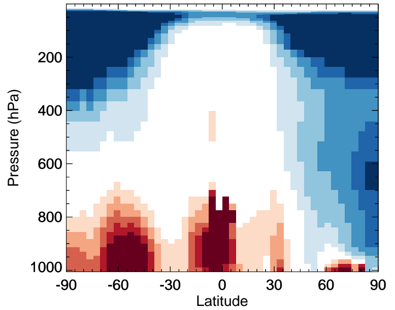
v11-02f-Run1 / v11-02e-Run1 NO 2 - Zonal mean % diff for Apr
