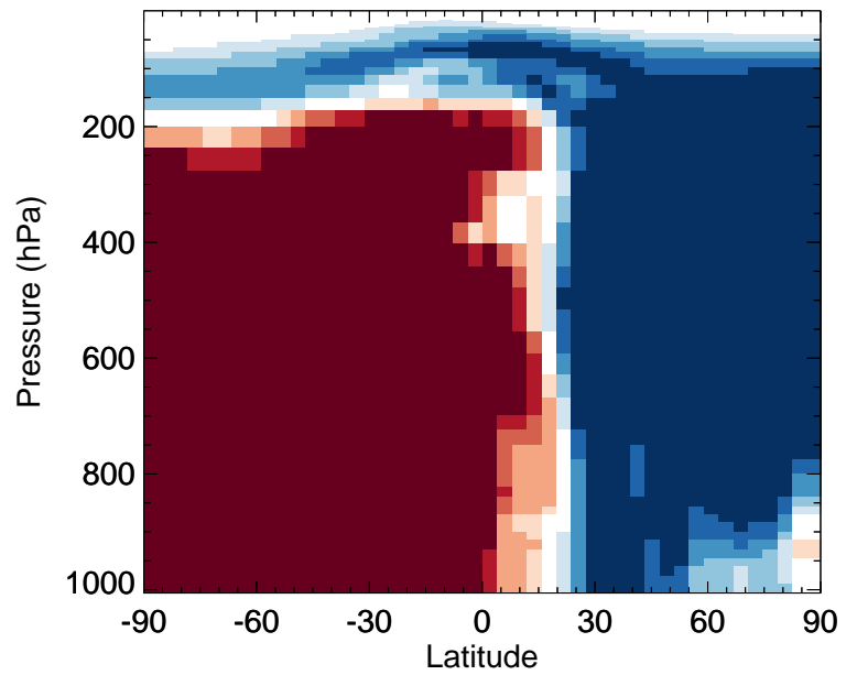
v11-02f-Run1 / v11-02e-Run0 ASOAN - Zonal mean % diff for Apr
