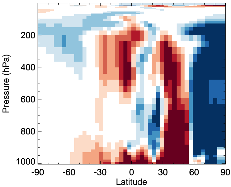
v11-02f-Run1 - v11-02e-Run0 PPN - Zonal mean abs diff for Apr
