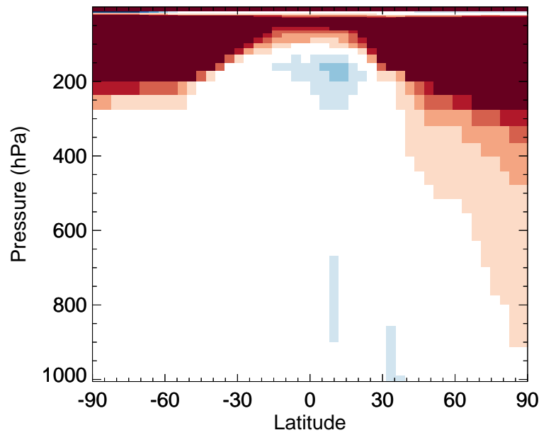
v11-02f-Run1 / v11-02e-Run1 MP - Zonal mean % diff for Apr
