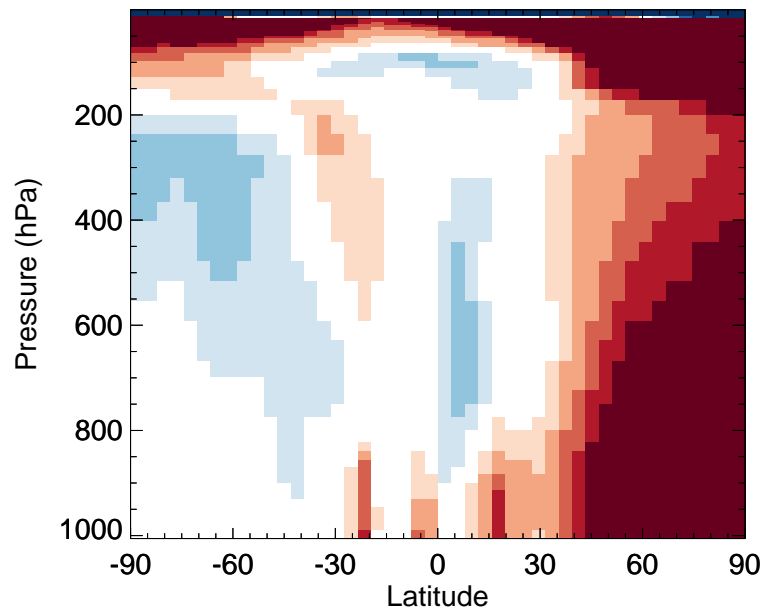
v11-02f-Run1 / v11-02e-Run1 C3H8 - Zonal mean % diff for Apr
