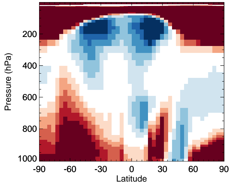
v11-02f-Run1 / v11-02e-Run1 MGLY - Zonal mean % diff for Apr
