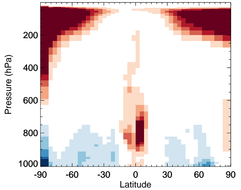
v11-02f-Run1 / v11-02e-Run1 BrO - Zonal mean % diff for Apr
