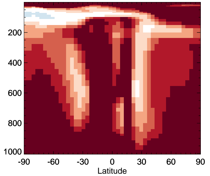
v11-02f-Run1 / v11-02e-Run1 RCHO - Zonal mean % diff for Apr
