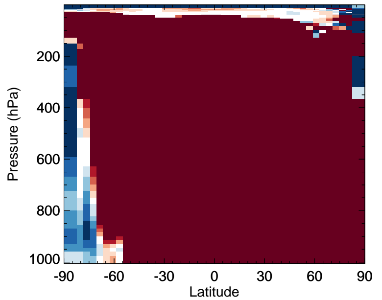
v11-02f-Run1 / v11-02e-Run0 RIPA - Zonal mean % diff for Apr
