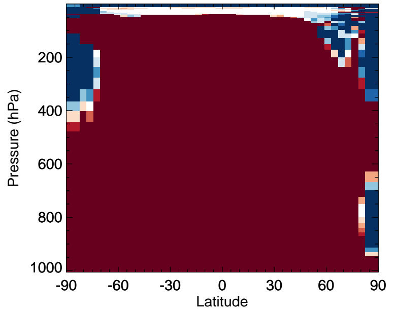
v11-02f-Run1 / v11-02e-Run0 ISN1 - Zonal mean % diff for Apr
