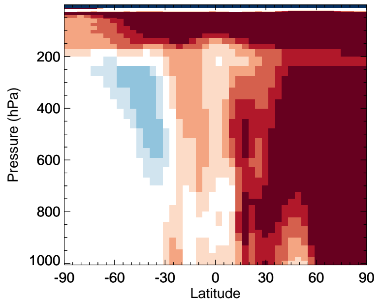
v11-02f-Run1 / v11-02e-Run1 ALD2 - Zonal mean % diff for Apr
