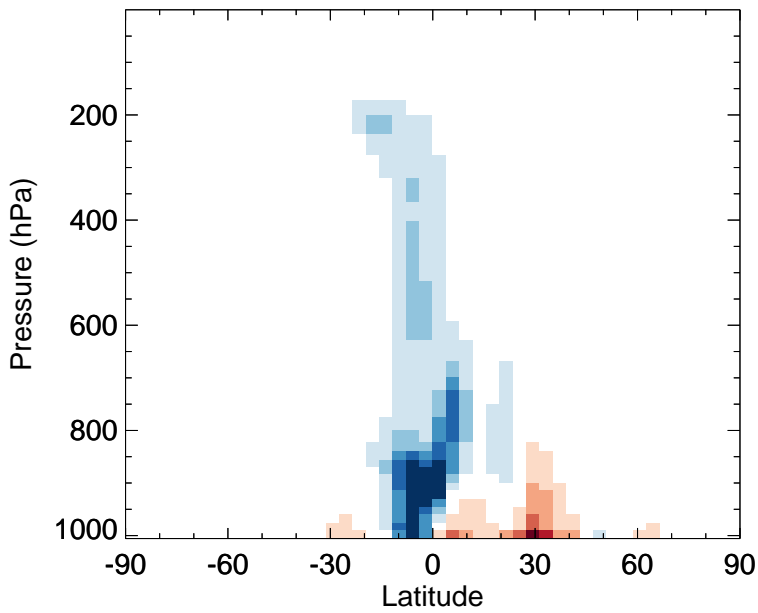
v11-02f-Run1 - v11-02e-Run0 EOH - Zonal mean abs diff for Apr
