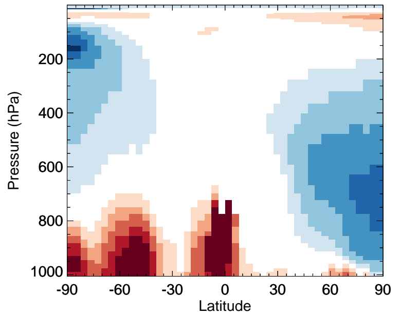
v11-02f-Run1 / v11-02e-Run1 MPN - Zonal mean % diff for Apr
