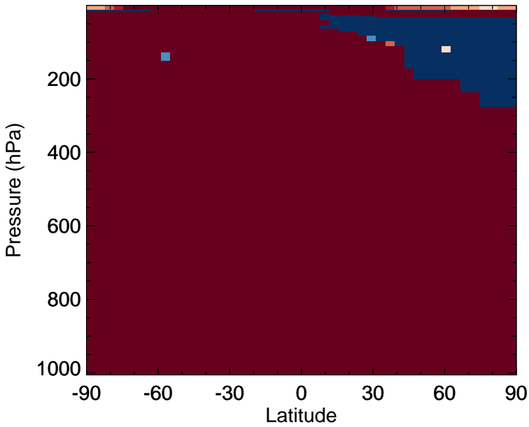
v11-02f-Run1 - v11-02e-Run0 N2O - Zonal mean abs diff for Apr
