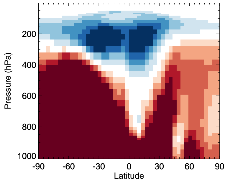
v11-02f-Run1 / v11-02e-Run1 TSOA2 - Zonal mean % diff for Apr
