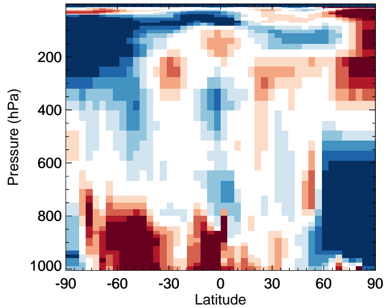
v11-02f-Run1 / v11-02e-Run0 HNO 4 - Zonal mean % diff for Apr
