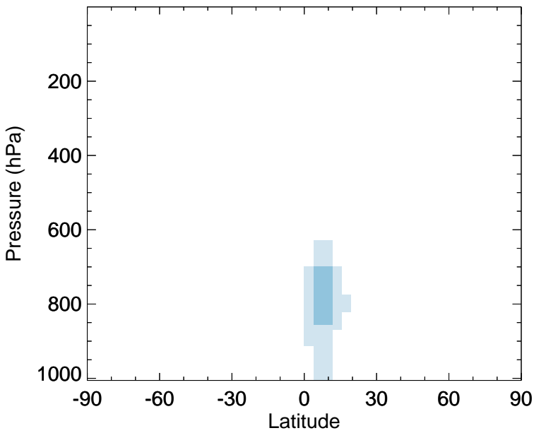
v11-02f-Run1 - v11-02e-Run0 ISO3 - Zonal mean abs diff for Apr
