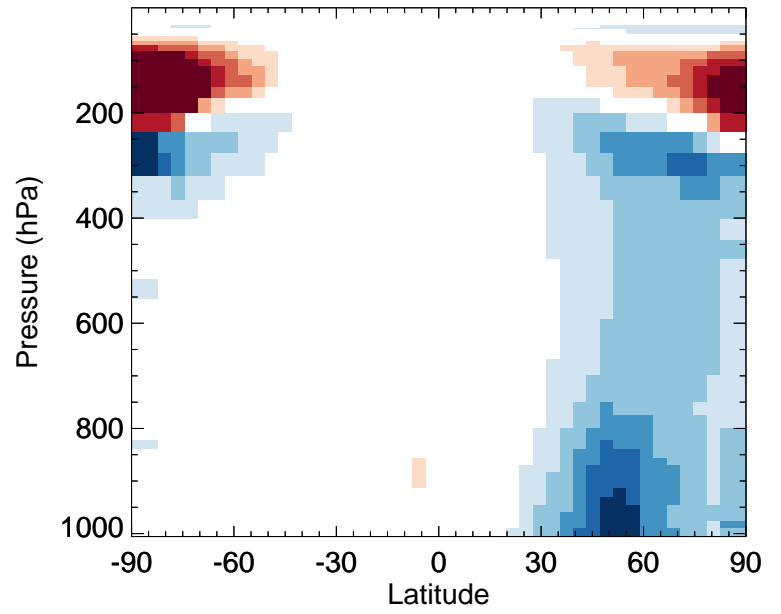
v11-02f-Run1 / v11-02e-Run1 HCl - Zonal mean % diff for Apr
