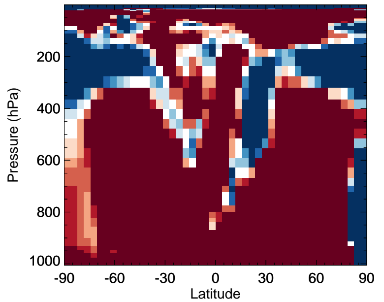
v11-02f-Run1 / v11-02e-Run0 IEPOXA - Zonal mean % diff for Apr
