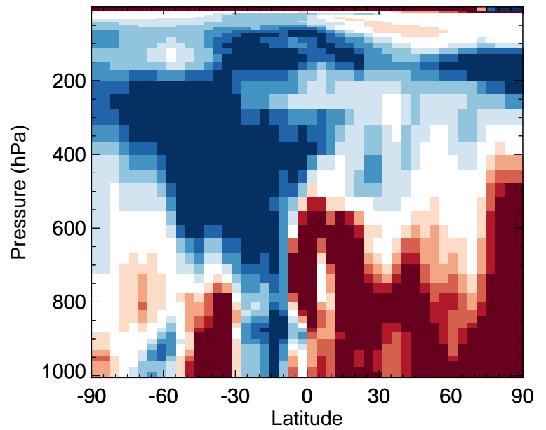
v11-02f-Run1 / v11-02e-Run0 BCPI - Zonal mean % diff for Apr
