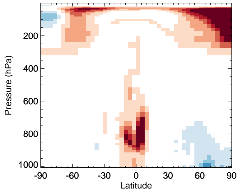
v11-02f-Run1 / v11-02e-Run1 HOBr - Zonal mean % diff for Apr
