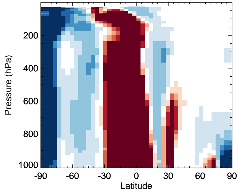
v11-02f-Run1 / v11-02e-Run1 SOAP - Zonal mean % diff for Apr
