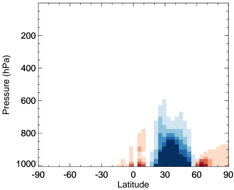
v11-02f-Run1 - v11-02e-Run1 TOLU - Zonal mean abs diff for Apr
