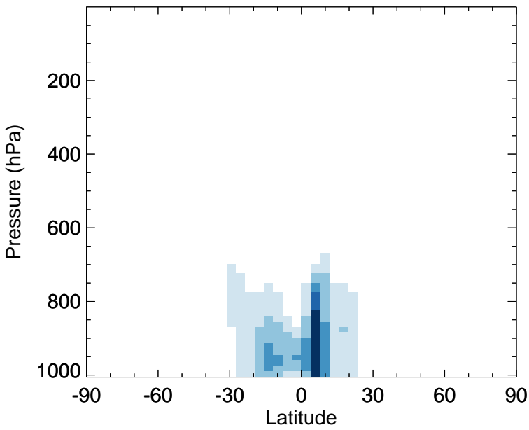
v11-02f-Run1 - v11-02e-Run1 MACR - Zonal mean abs diff for Apr
