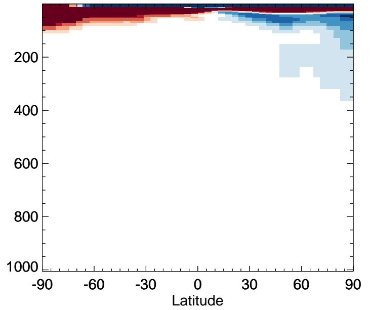
v11-02f-Run1 / v11-02e-Run0 CFC11 - Zonal mean % diff for Apr
