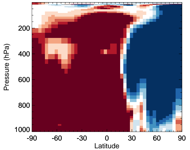
v11-02f-Run1 / v11-02e-Run0 ASOA1 - Zonal mean % diff for Apr
