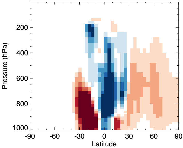
v11-02f-Run1 - v11-02e-Run0 MAP - Zonal mean abs diff for Apr
