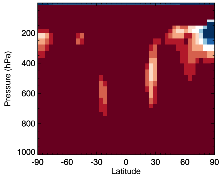
v11-02f-Run1 / v11-02e-Run0 ALK4 - Zonal mean % diff for Apr
