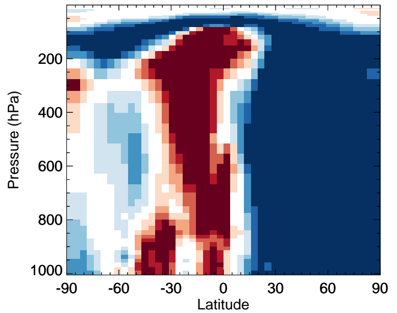
v11-02f-Run1 / v11-02e-Run0 ASOG2 - Zonal mean % diff for Apr
