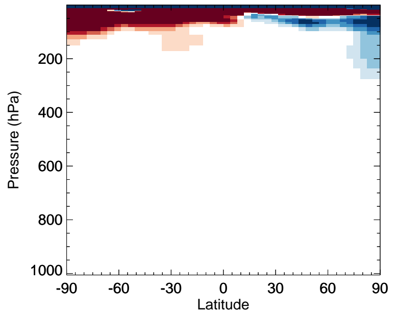
v11-02f-Run1 / v11-02e-Run0 CH2Br2 - Zonal mean % diff for Apr
