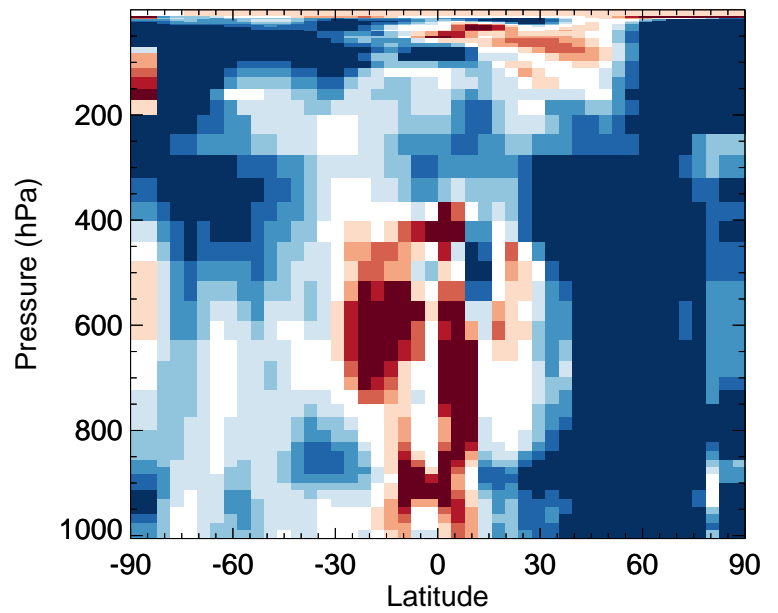
v11-02f-Run1 / v11-02e-Run0 ClOO - Zonal mean % diff for Apr
