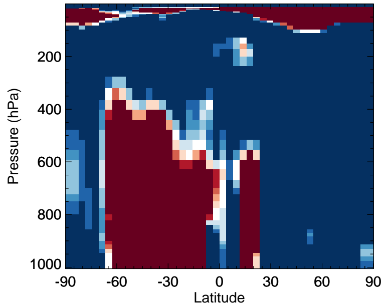
v11-02f-Run1 / v11-02e-Run0 DST2 - Zonal mean % diff for Apr
