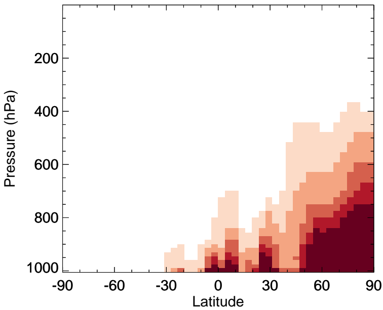
v11-02f-Run1 - v11-02e-Run0 ALK4 - Zonal mean abs diff for Apr
