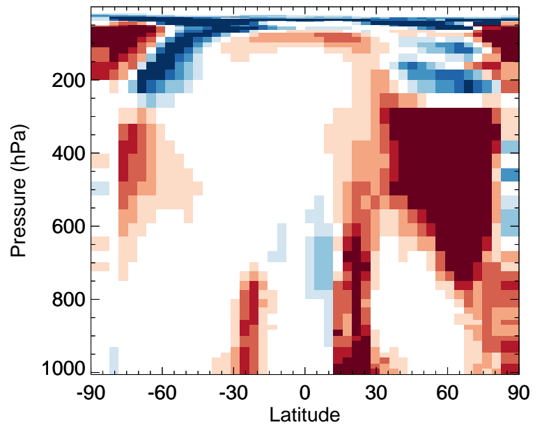
v11-02f-Run1 / v11-02e-Run1 HBr - Zonal mean % diff for Apr
