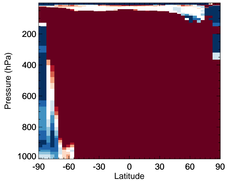
v11-02f-Run1 / v11-02e-Run0 RIPD - Zonal mean % diff for Apr
