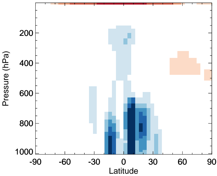
v11-02f-Run1 - v11-02e-Run1 MP - Zonal mean abs diff for Apr
