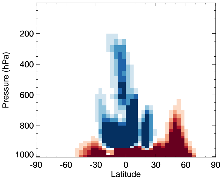
v11-02f-Run1 - v11-02e-Run0 PRPE - Zonal mean abs diff for Apr
