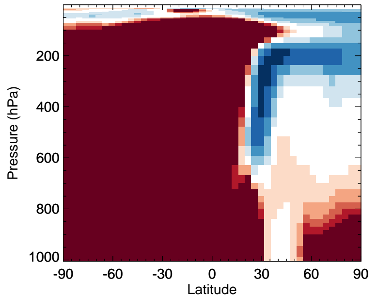
v11-02f-Run1 / v11-02e-Run1 BENZ - Zonal mean % diff for Apr
