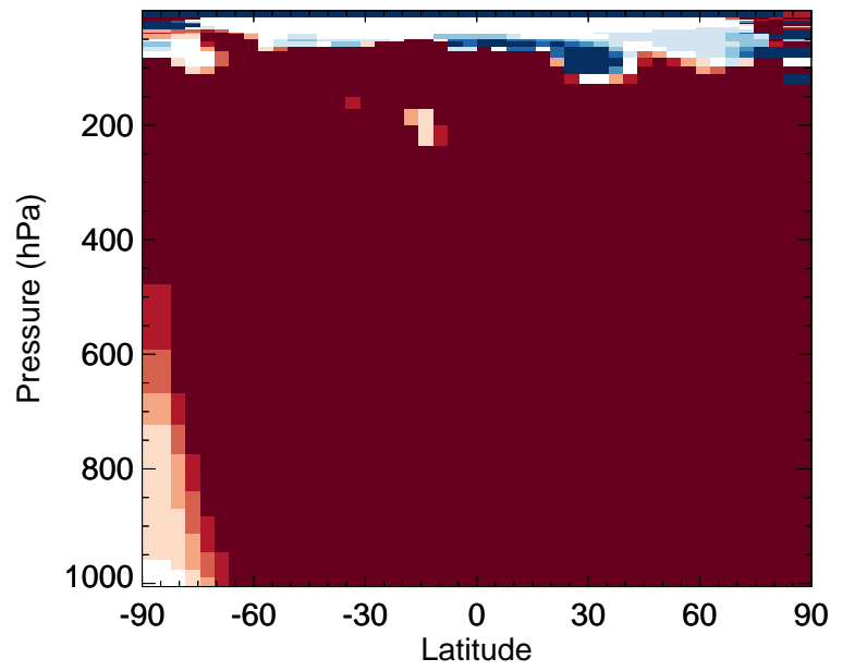
v11-02f-Run1 / v11-02e-Run1 RIPB - Zonal mean % diff for Apr
