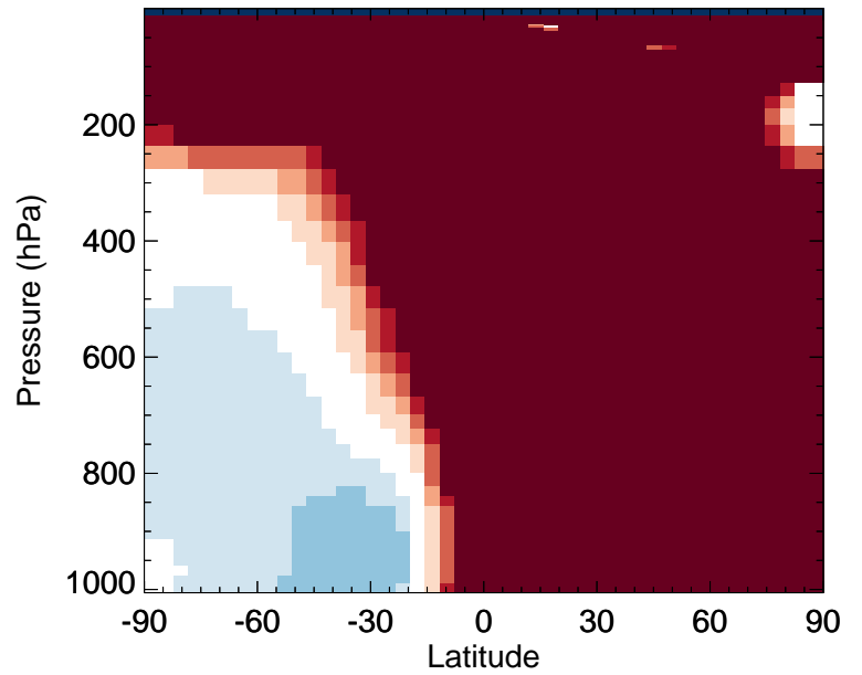
v11-02f-Run1 / v11-02e-Run0 C2H6 - Zonal mean % diff for Apr
