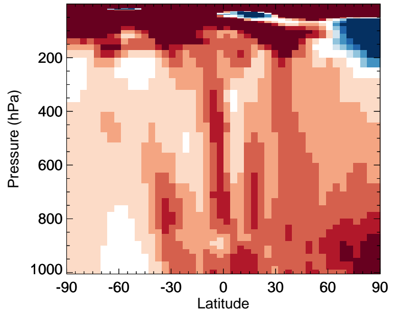
v11-02f-Run1 / v11-02e-Run0 ACET - Zonal mean % diff for Apr
