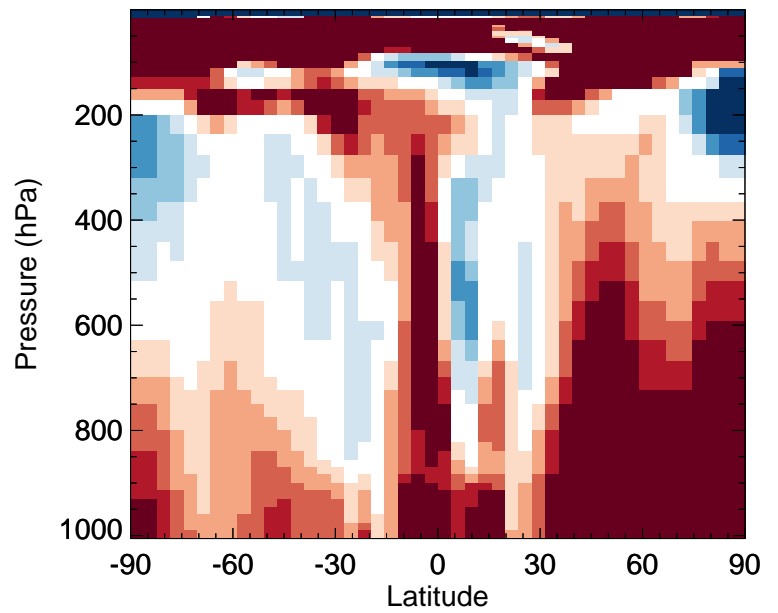
v11-02f-Run1 / v11-02e-Run0 C3H8 - Zonal mean % diff for Apr
