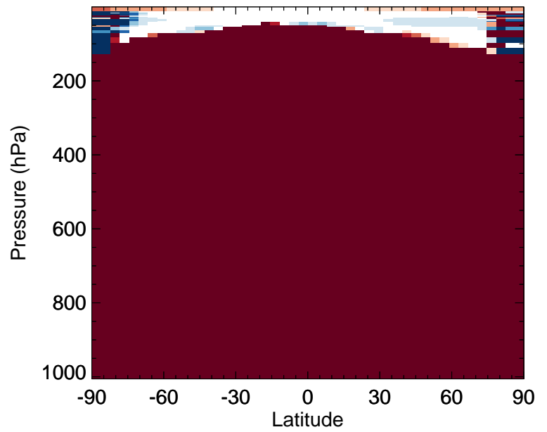
v11-02f-Run1 / v11-02e-Run1 MTPA - Zonal mean % diff for Apr
