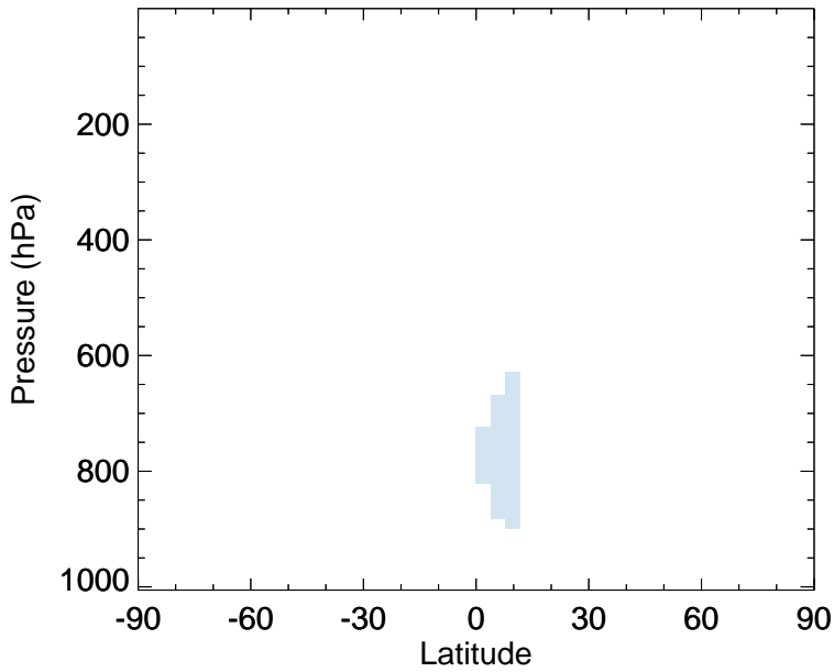
v11-02f-Run1 - v11-02e-Run0 IMAE - Zonal mean abs diff for Apr
