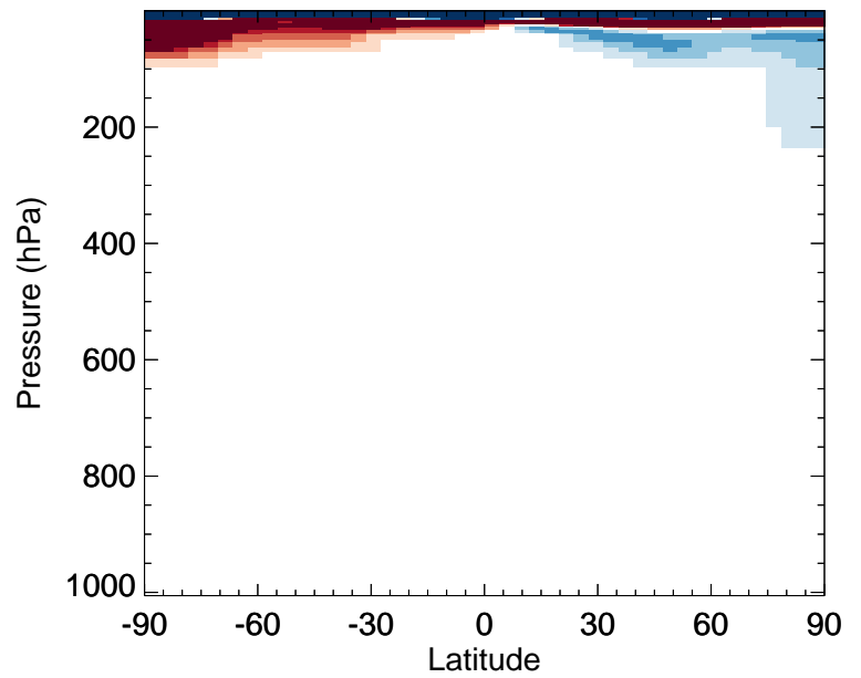
v11-02f-Run1 / v11-02e-Run0 CFC113 - Zonal mean % diff for Apr
