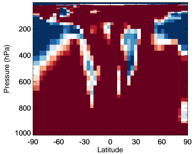
v11-02f-Run1 / v11-02e-Run0 GLYC - Zonal mean % diff for Apr
