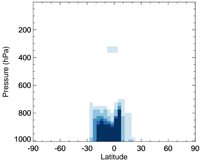
v11-02f-Run1 - v11-02e-Run1 ISOP - Zonal mean abs diff for Apr
