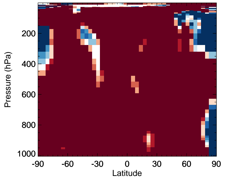
v11-02f-Run1 / v11-02e-Run0 OCPO - Zonal mean % diff for Apr
