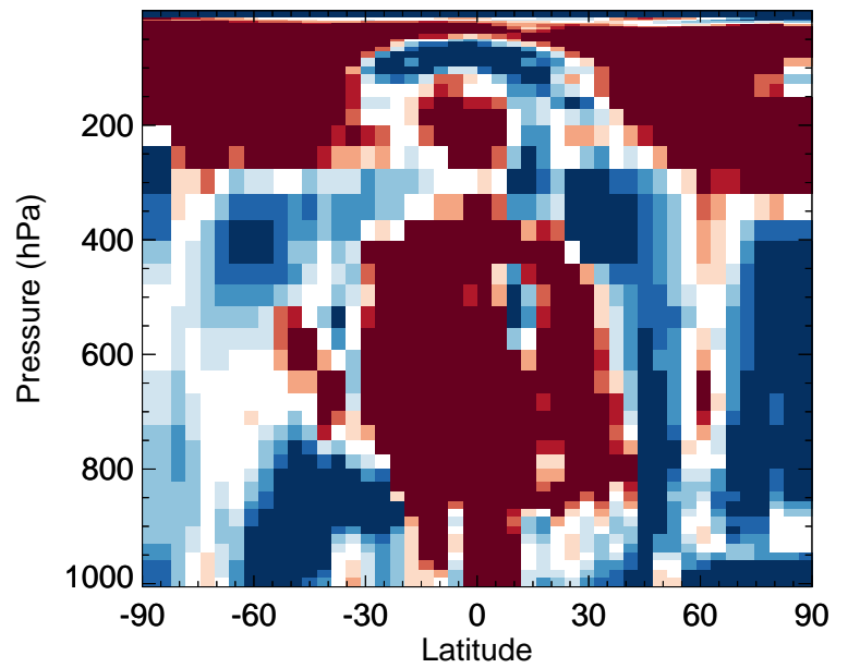
v11-02f-Run1 / v11-02e-Run0 OCIO - Zonal mean % diff for Apr
