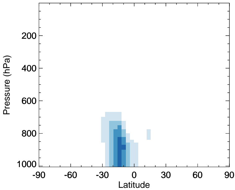
v11-02f-Run1 - v11-02e-Run0 SOAIE - Zonal mean abs diff for Apr
