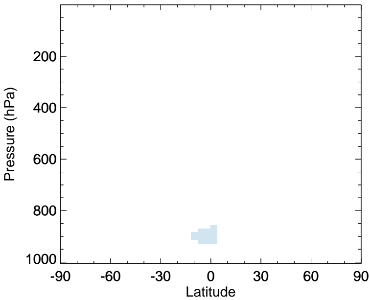
v11-02f-Run1 - v11-02e-Run0 HPALD - Zonal mean abs diff for Apr
