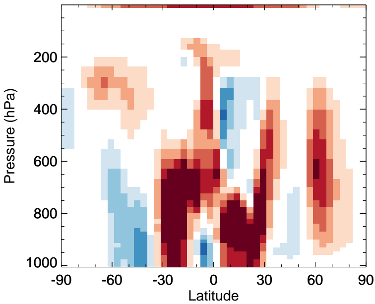
v11-02f-Run1 - v11-02e-Run0 MP - Zonal mean abs diff for Apr
