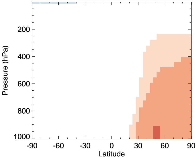
v11-02f-Run1 - v11-02e-Run1 CO - Zonal mean abs diff for Apr
