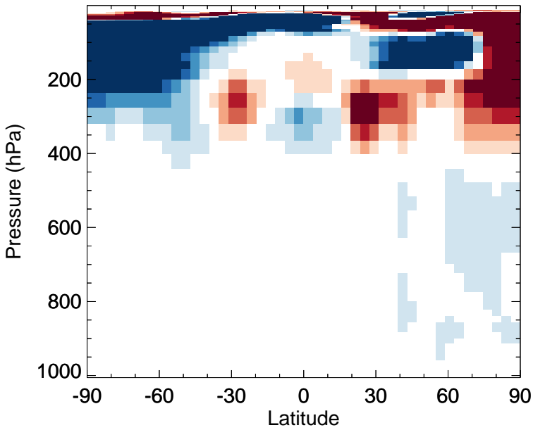
v11-02f-Run1 - v11-02e-Run0 HNO 4 - Zonal mean abs diff for Apr
