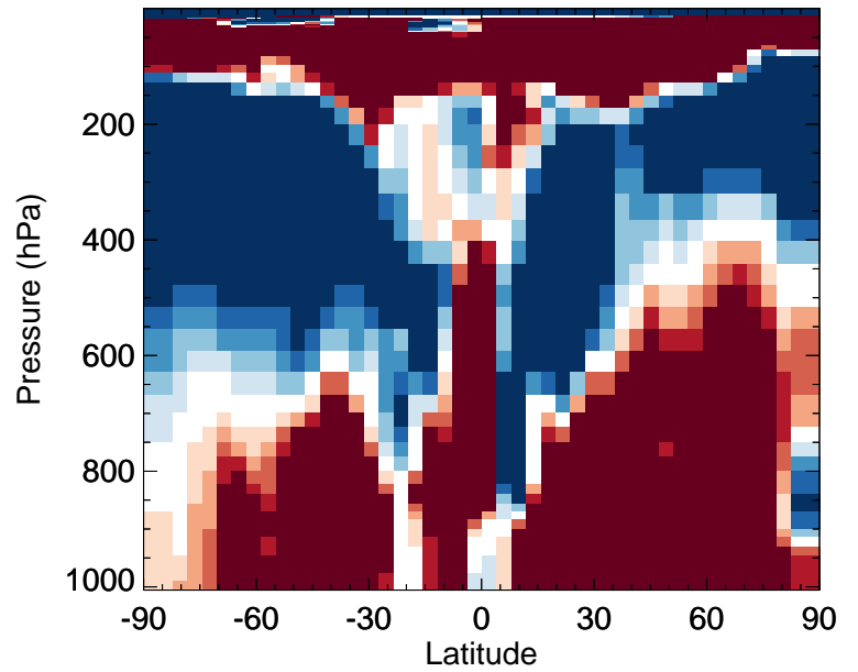
v11-02f-Run1 / v11-02e-Run0 IMAE - Zonal mean % diff for Apr
