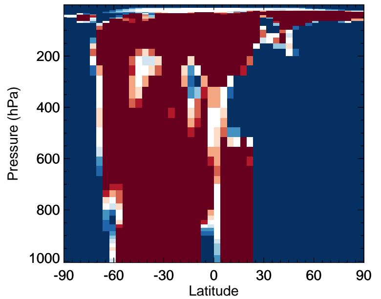
v11-02f-Run1 / v11-02e-Run0 DST4 - Zonal mean % diff for Apr
