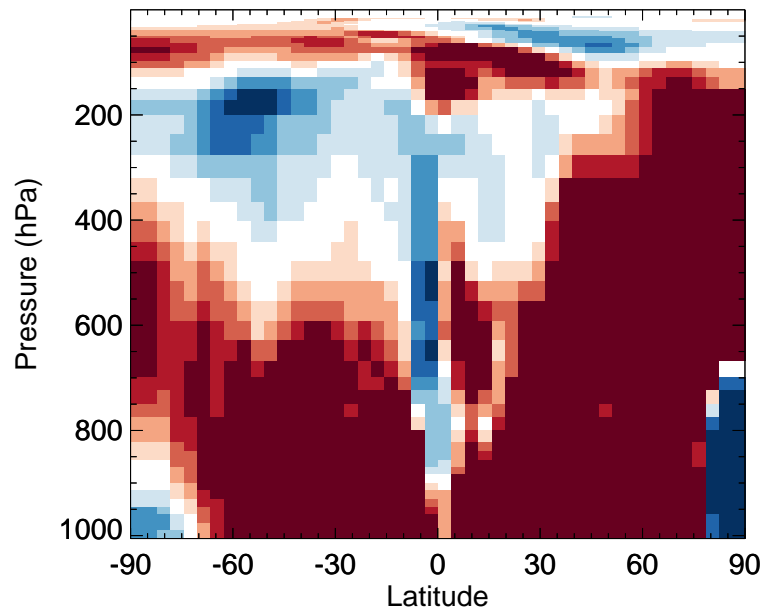
v11-02f-Run1 / v11-02e-Run0 DHDN - Zonal mean % diff for Apr
