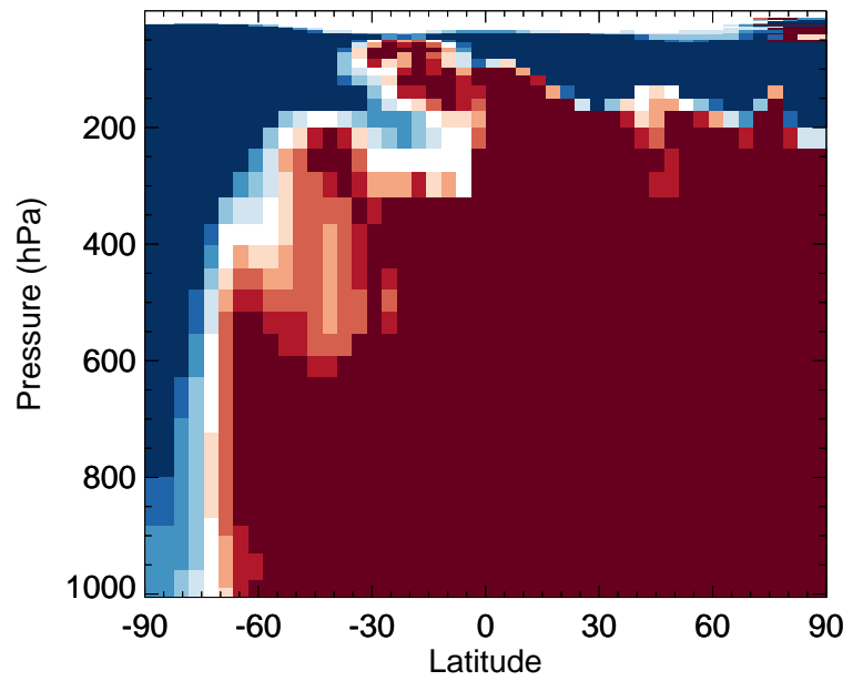
v11-02f-Run1 / v11-02e-Run1 HPALD - Zonal mean % diff for Apr
