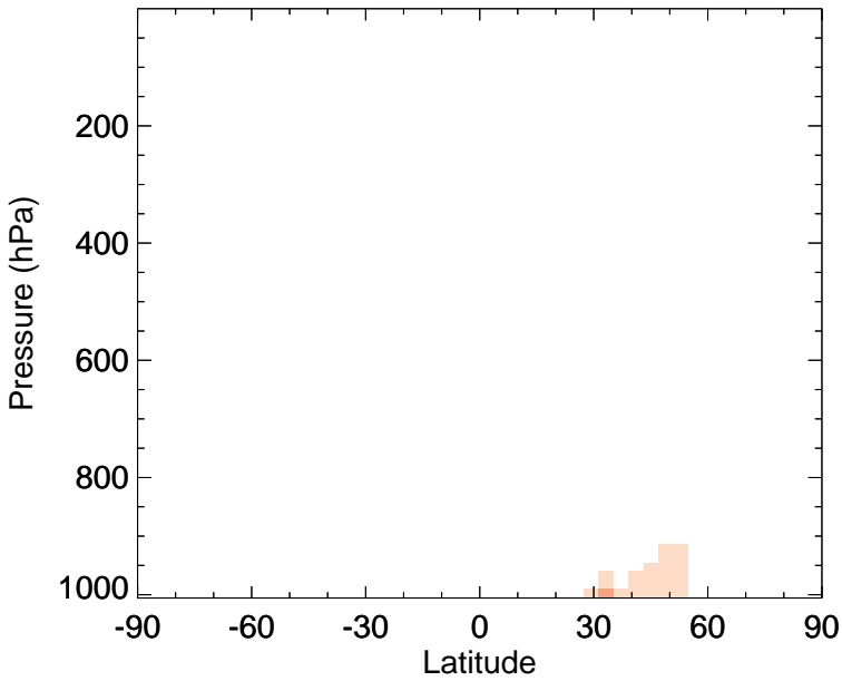
v11-02f-Run1 - v11-02e-Run0 NIT - Zonal mean abs diff for Apr
