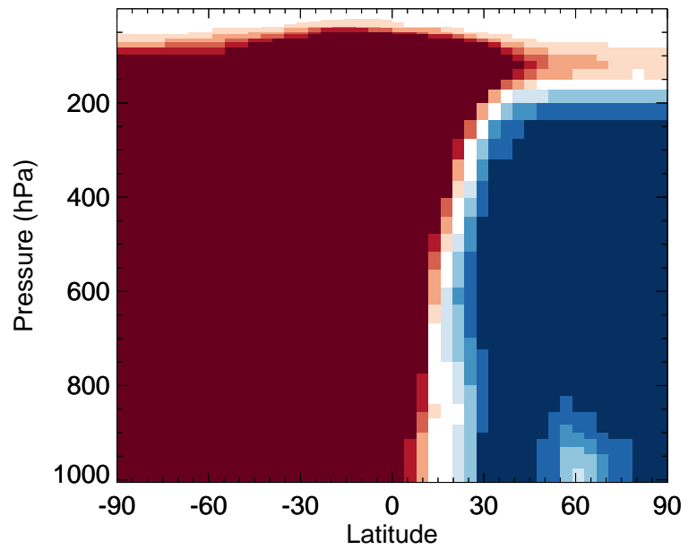
v11-02f-Run1 / v11-02e-Run1 ASOG1 - Zonal mean % diff for Apr
