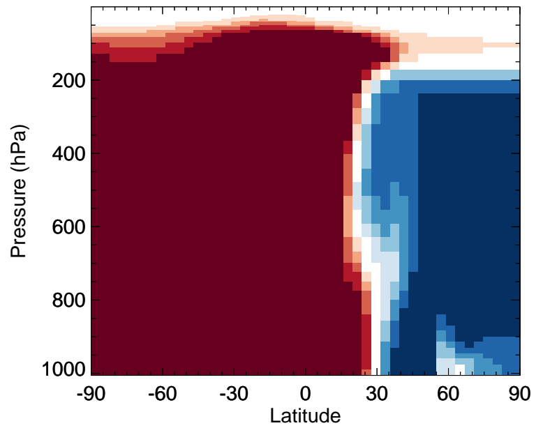
v11-02f-Run1 / v11-02e-Run1 ASOA1 - Zonal mean % diff for Apr
