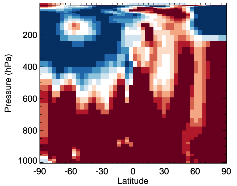
v11-02f-Run1 / v11-02e-Run0 ISOA2 - Zonal mean % diff for Apr
