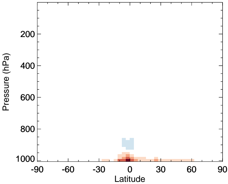
v11-02f-Run1 - v11-02e-Run0 RCHO - Zonal mean abs diff for Apr
