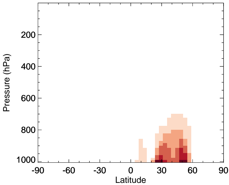
v11-02f-Run1 - v11-02e-Run0 OCPI - Zonal mean abs diff for Apr
