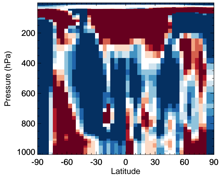
v11-02f-Run1 / v11-02e-Run0 NITs - Zonal mean % diff for Apr
