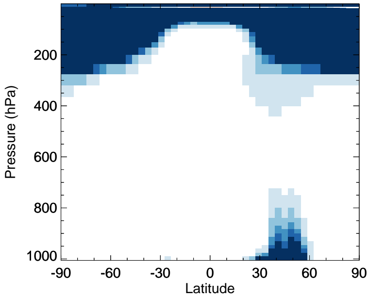
v11-02f-Run1 - v11-02e-Run1 N2O5 - Zonal mean abs diff for Apr
