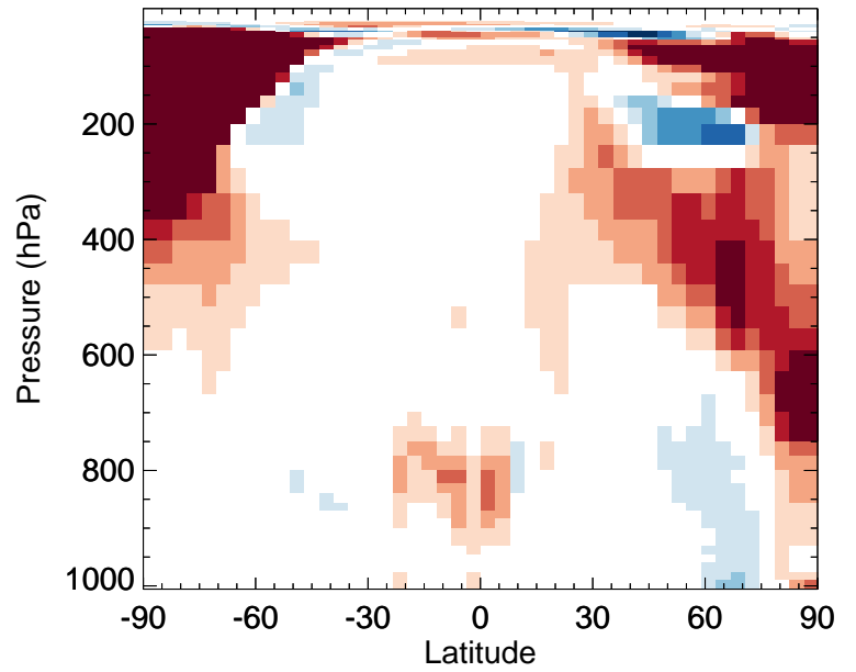
v11-02f-Run1 / v11-02e-Run1 Br2 - Zonal mean % diff for Apr
