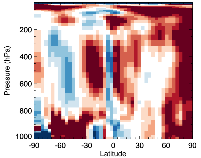
v11-02f-Run1 / v11-02e-Run0 HNO 3 - Zonal mean % diff for Apr
