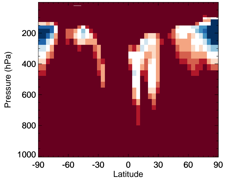
v11-02f-Run1 / v11-02e-Run0 MEK - Zonal mean % diff for Apr
