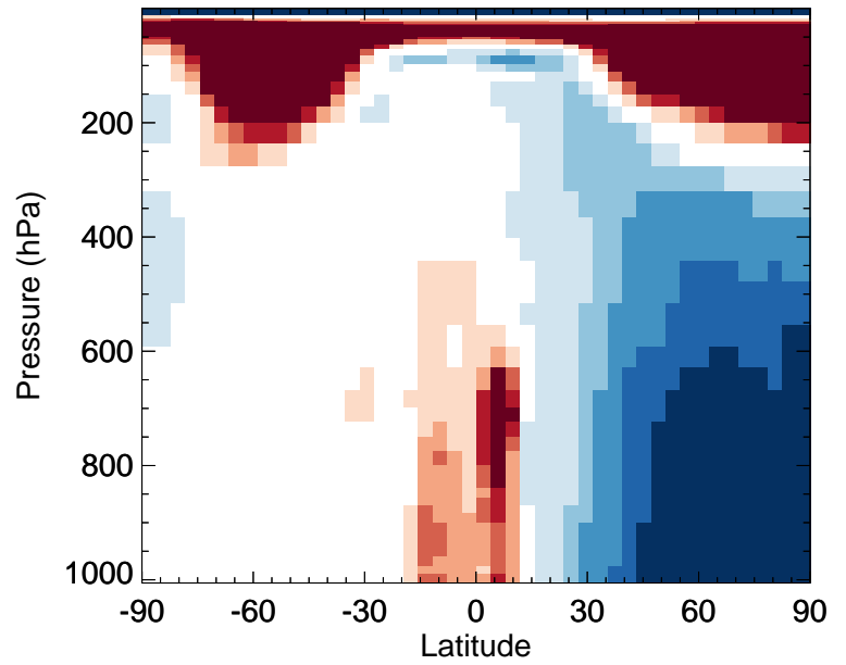
v11-02f-Run1 / v11-02e-Run1 HOCl - Zonal mean % diff for Apr
