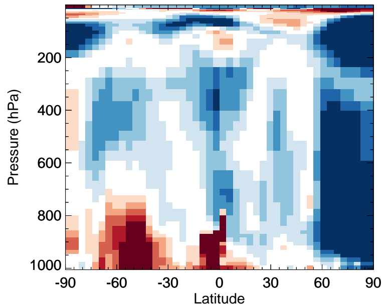
v11-02f-Run1 / v11-02e-Run0 MPN - Zonal mean % diff for Apr
