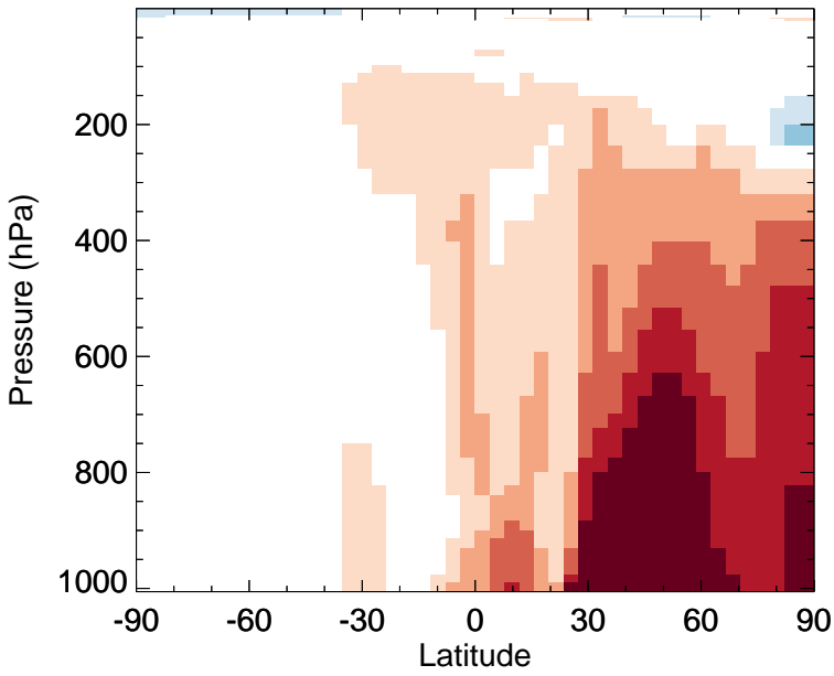
v11-02f-Run1 - v11-02e-Run0 CO - Zonal mean abs diff for Apr
