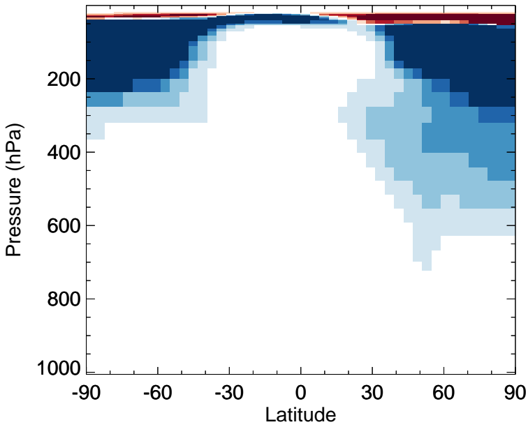
v11-02f-Run1 - v11-02e-Run1 HNO 4 - Zonal mean abs diff for Apr
