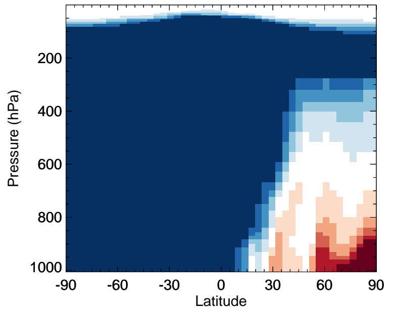
v11-02f-Run1 / v11-02e-Run1 SOAIE - Zonal mean % diff for Apr
