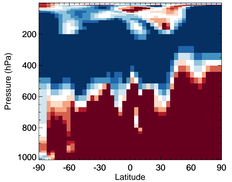
v11-02f-Run1 / v11-02e-Run0 TSOA3 - Zonal mean % diff for Apr
