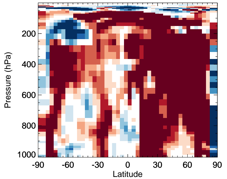
v11-02f-Run1 / v11-02e-Run0 HBr - Zonal mean % diff for Apr
