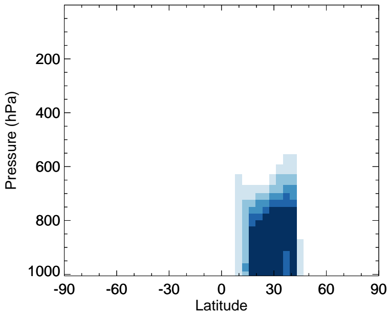
v11-02f-Run1 - v11-02e-Run0 DST4 - Zonal mean abs diff for Apr
