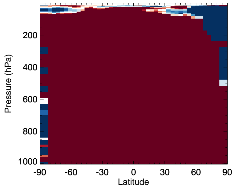
v11-02f-Run1 / v11-02e-Run0 MTPO - Zonal mean % diff for Apr
