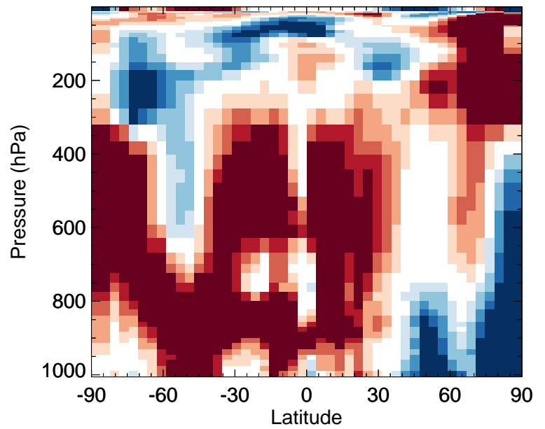
v11-02f-Run1 / v11-02e-Run0 NO3 - Zonal mean % diff for Apr
