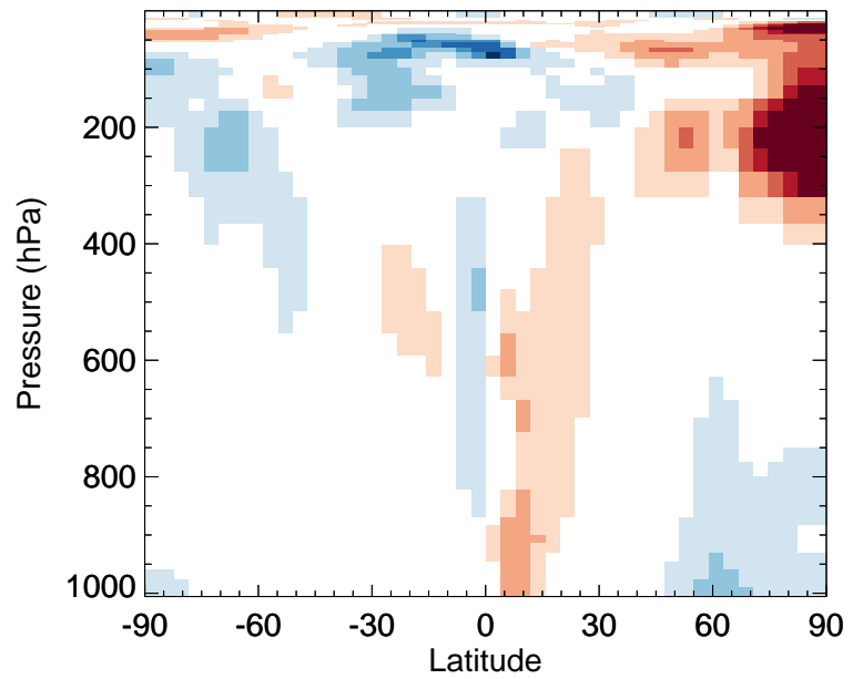
v11-02f-Run1 / v11-02e-Run0 O3 - Zonal mean % diff for Apr
