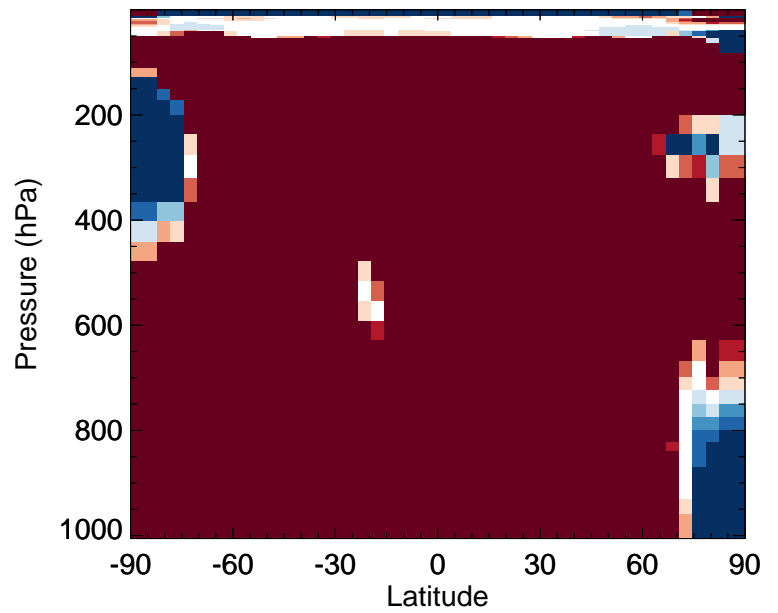
v11-02f-Run1 / v11-02e-Run0 NPMN - Zonal mean % diff for Apr
