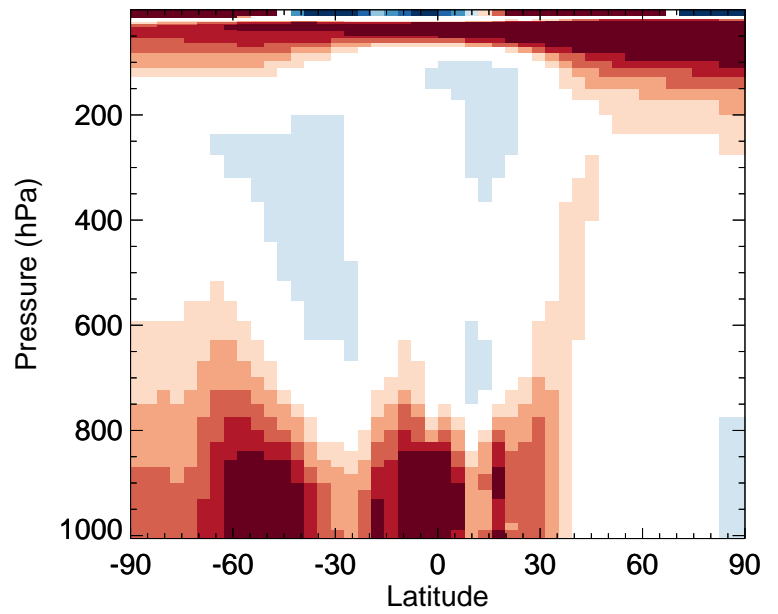
v11-02f-Run1 / v11-02e-Run1 PAN - Zonal mean % diff for Apr
