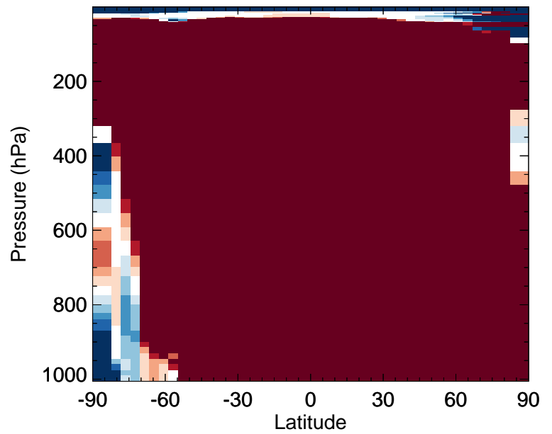
v11-02f-Run1 / v11-02e-Run0 LVOC - Zonal mean % diff for Apr
