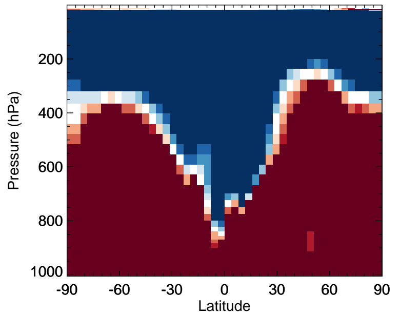
v11-02f-Run1 / v11-02e-Run1 IEPOXA - Zonal mean % diff for Apr
