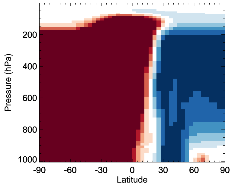
v11-02f-Run1 / v11-02e-Run1 ASOAN - Zonal mean % diff for Apr
