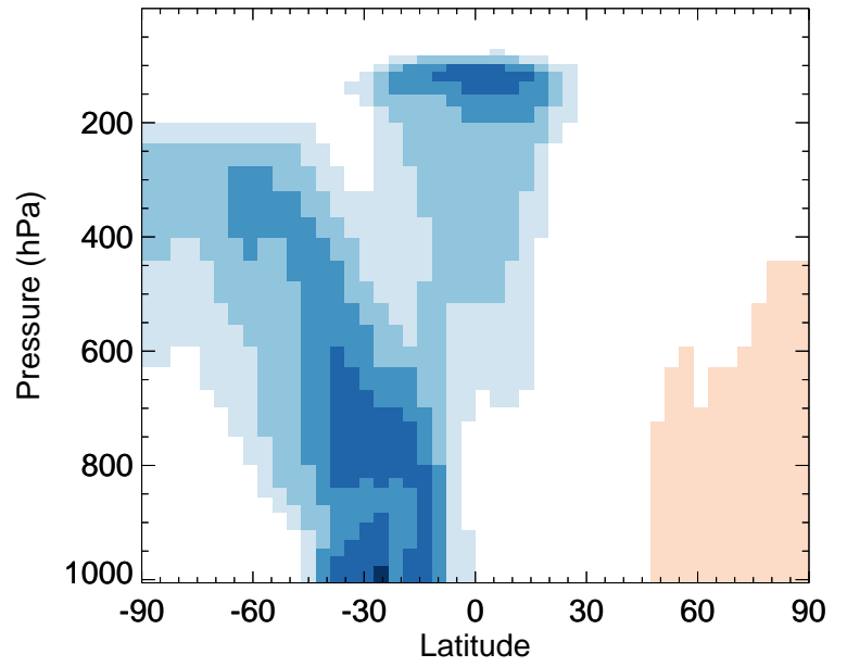
v11-02f-Run1 / v11-02e-Run1 NH4 - Zonal mean % diff for Apr
