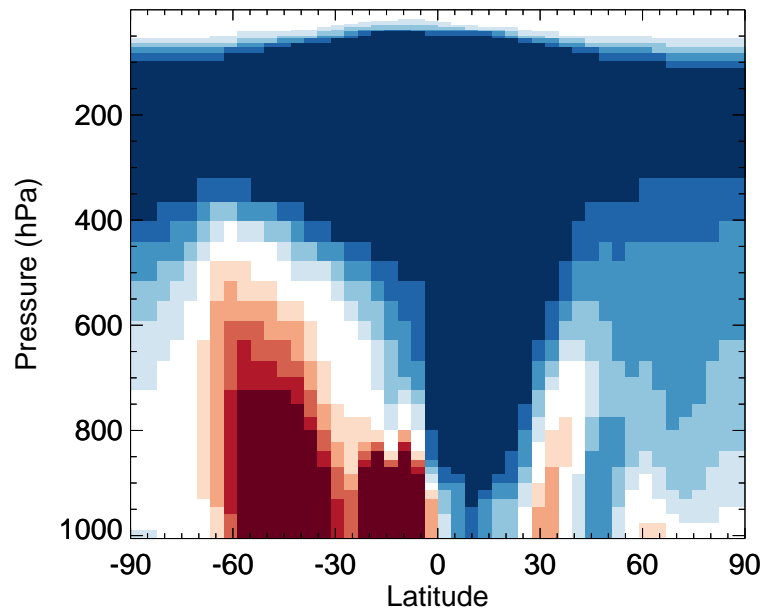
v11-02f-Run1 / v11-02e-Run1 ISOA1 - Zonal mean % diff for Apr
