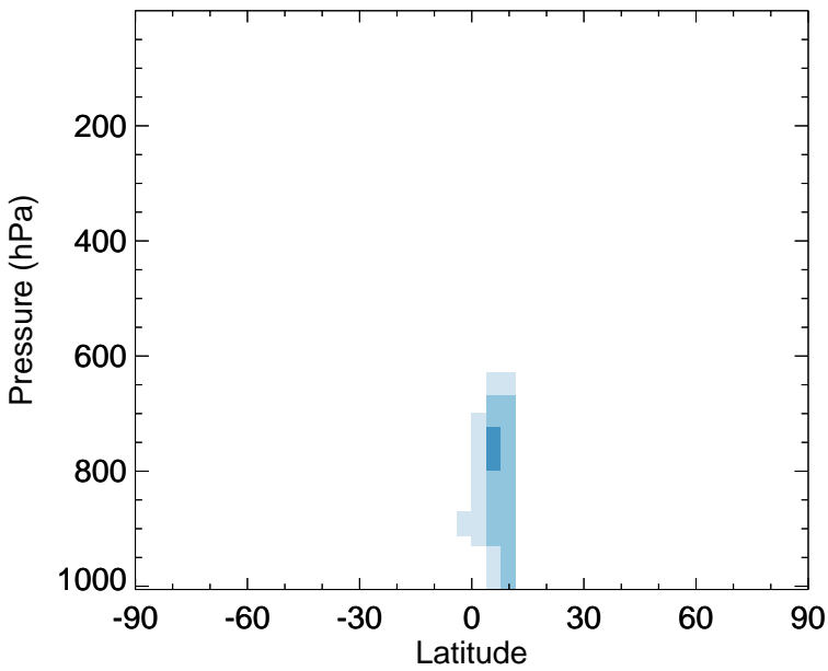
v11-02f-Run1 - v11-02e-Run0 IEPOXA - Zonal mean abs diff for Apr
