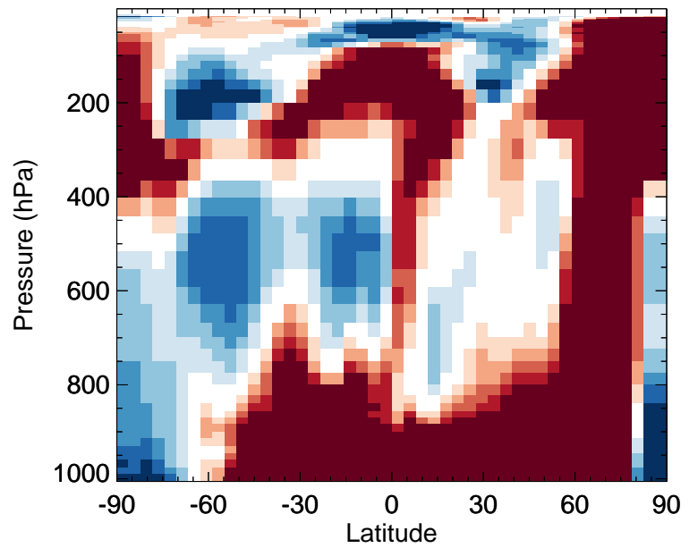
v11-02f-Run1 / v11-02e-Run0 TSOG0 - Zonal mean % diff for Apr
