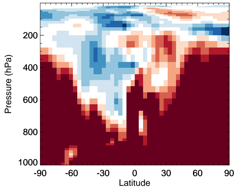
v11-02f-Run1 / v11-02e-Run0 OCPI - Zonal mean % diff for Apr
