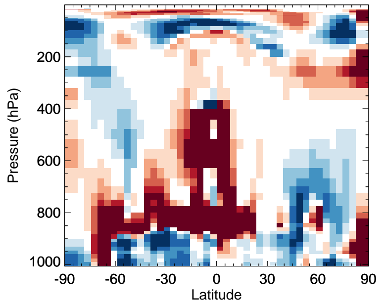
v11-02f-Run1 / v11-02e-Run0 HOBr - Zonal mean % diff for Apr
