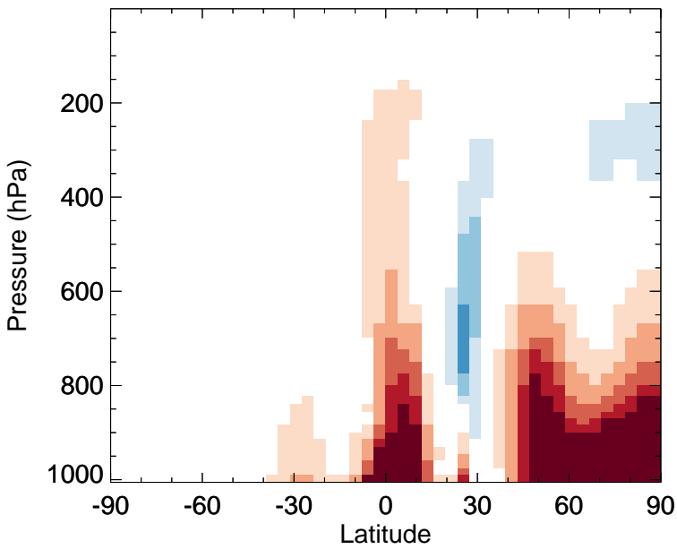
v11-02f-Run1 - v11-02e-Run0 BENZ - Zonal mean abs diff for Apr
