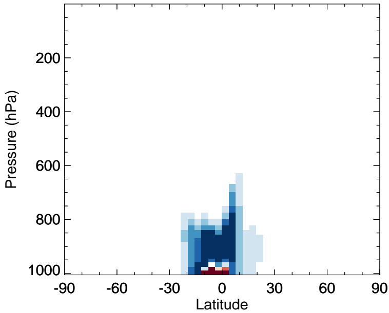
v11-02f-Run1 - v11-02e-Run0 ISOP - Zonal mean abs diff for Apr
