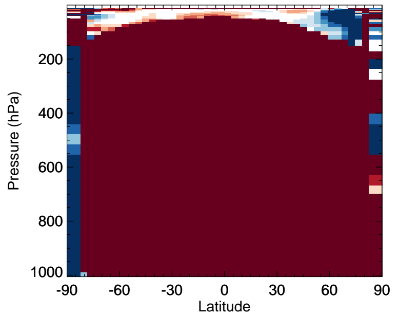
v11-02f-Run1 / v11-02e-Run0 LIMO - Zonal mean % diff for Apr
