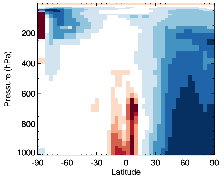
v11-02f-Run1 / v11-02e-Run1 ClOO - Zonal mean % diff for Apr
