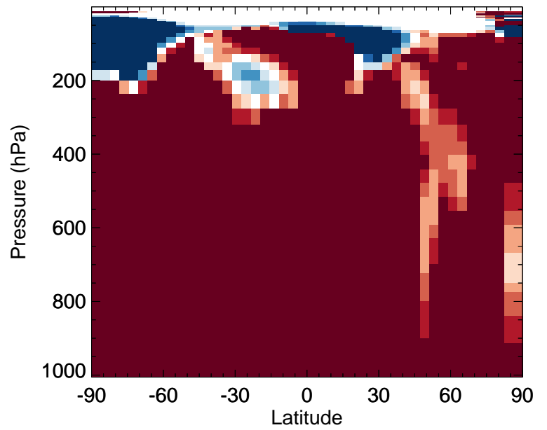
v11-02f-Run1 / v11-02e-Run1 ETHLN - Zonal mean % diff for Apr
