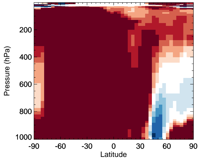
v11-02f-Run1 / v11-02e-Run1 OCPO - Zonal mean % diff for Apr
