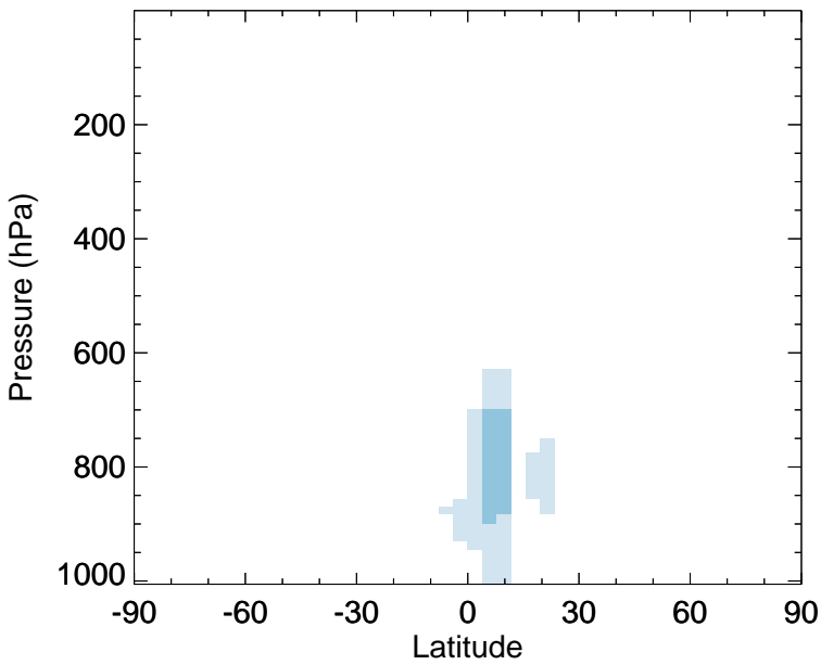
v11-02f-Run1 - v11-02e-Run0 GLYC - Zonal mean abs diff for Apr
