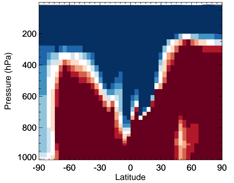
v11-02f-Run1 / v11-02e-Run1 HC187 - Zonal mean % diff for Apr
