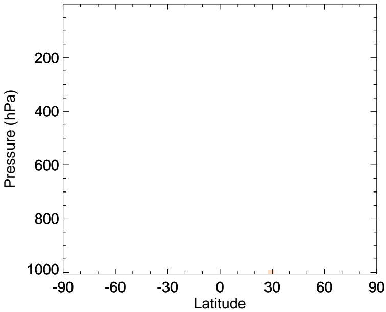
v11-02f-Run1 - v11-02e-Run0 SO 2 - Zonal mean abs diff for Apr
