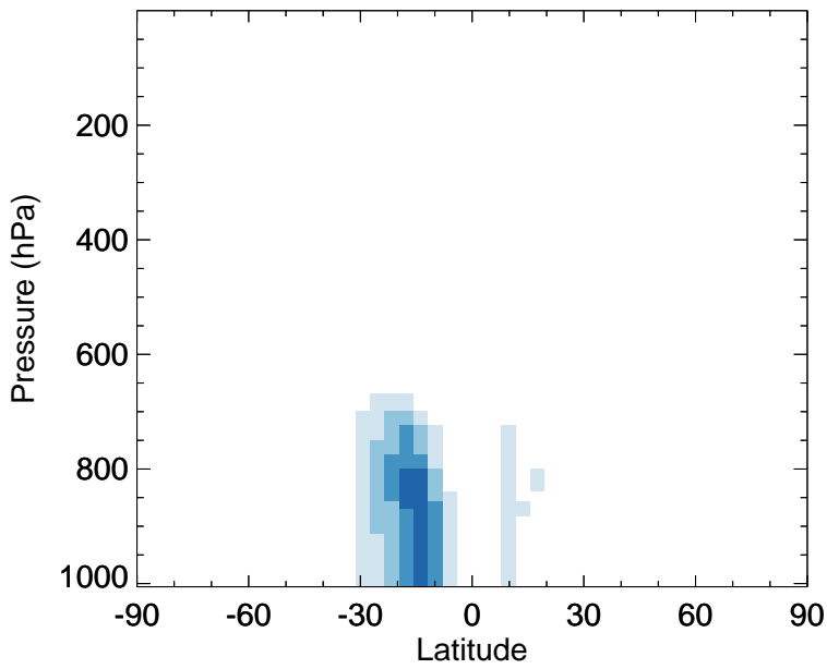
v11-02f-Run1 - v11-02e-Run1 SOAIE - Zonal mean abs diff for Apr
