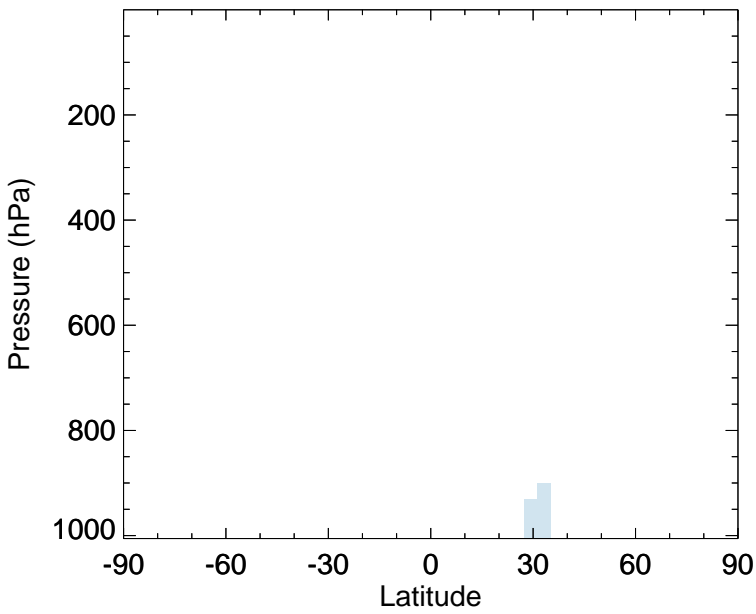
v11-02f-Run1 - v11-02e-Run1 SOAGX - Zonal mean abs diff for Apr
