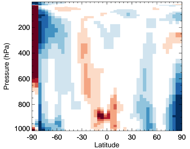
v11-02f-Run1 / v11-02e-Run0 OH - Zonal mean % diff for Apr
