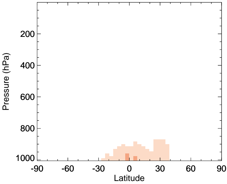
v11-02f-Run1 - v11-02e-Run1 INDIOL - Zonal mean abs diff for Apr
