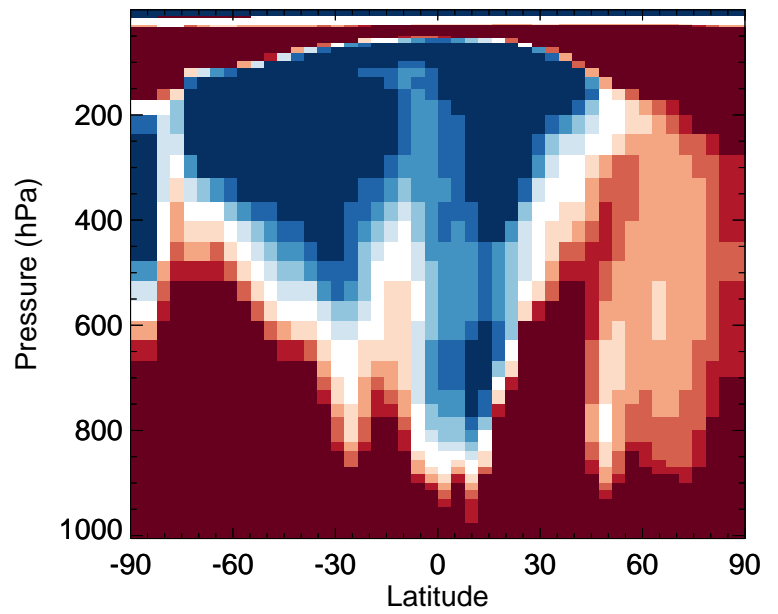
v11-02f-Run1 / v11-02e-Run1 HCOOH - Zonal mean % diff for Apr
