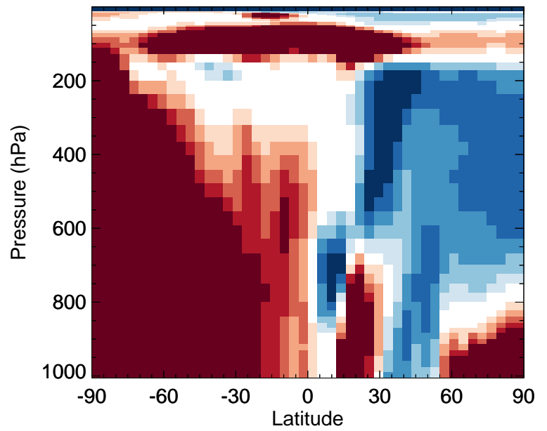
v11-02f-Run1 / v11-02e-Run1 GLYX - Zonal mean % diff for Apr
