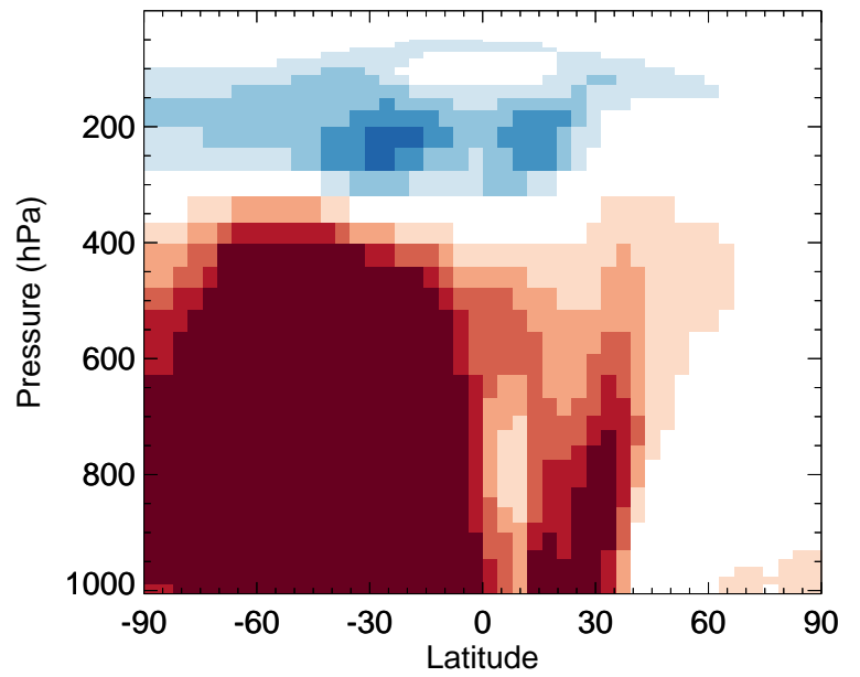
v11-02f-Run1 / v11-02e-Run1 ISOA2 - Zonal mean % diff for Apr
