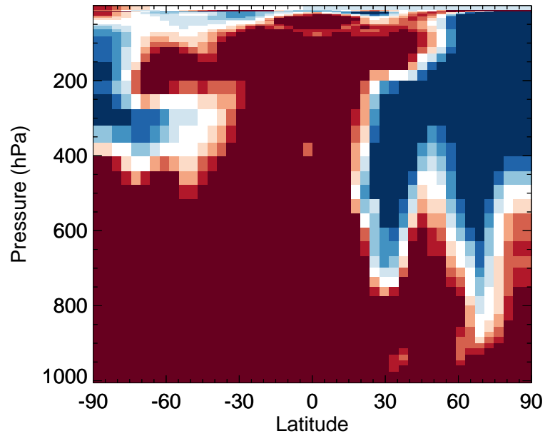
v11-02f-Run1 / v11-02e-Run0 ASOA3 - Zonal mean % diff for Apr
