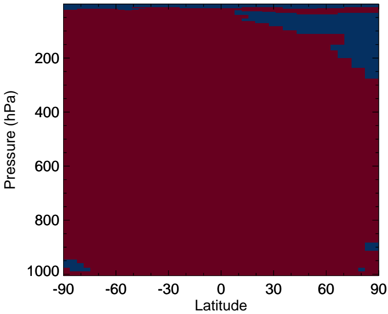
v11-02f-Run1 - v11-02e-Run0 CH4 - Zonal mean abs diff for Apr
