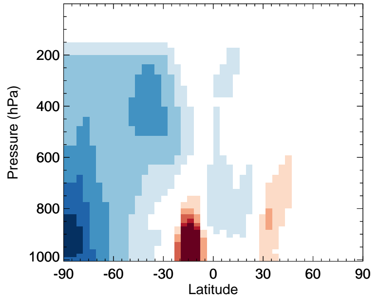
v11-02f-Run1 / v11-02e-Run1 SOAS - Zonal mean % diff for Apr
