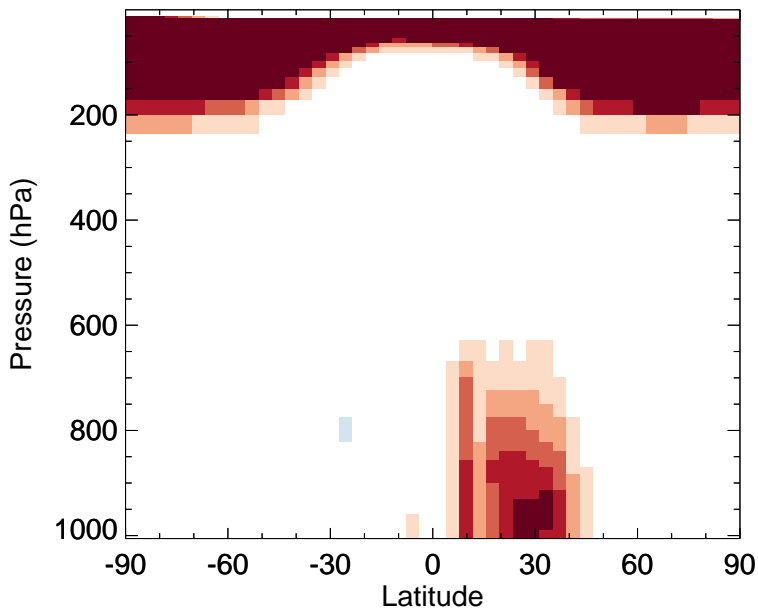
v11-02f-Run1 - v11-02e-Run1 HNO 3 - Zonal mean abs diff for Apr
