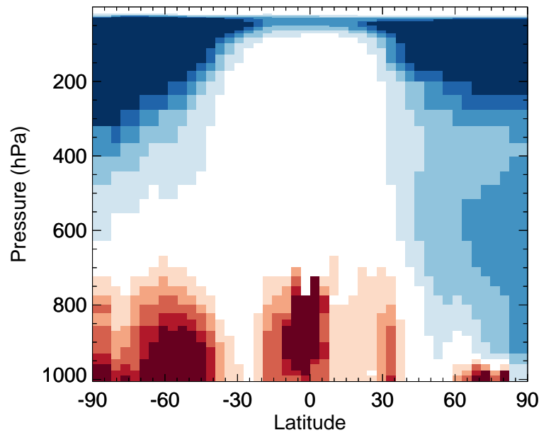
v11-02f-Run1 / v11-02e-Run1 NO - Zonal mean % diff for Apr
