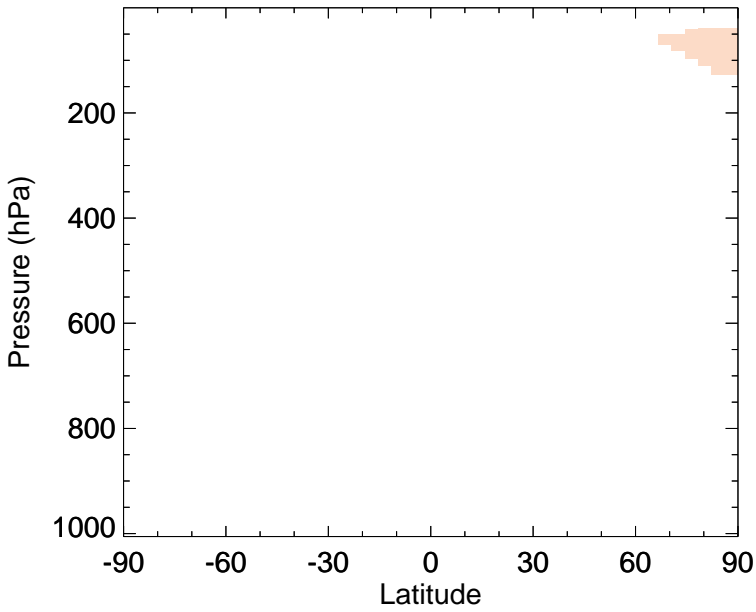
v11-02f-Run1 - v11-02e-Run1 BrO - Zonal mean abs diff for Apr
