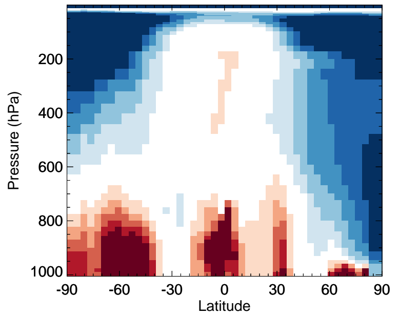
v11-02f-Run1 / v11-02e-Run1 HNO 2 - Zonal mean % diff for Apr
