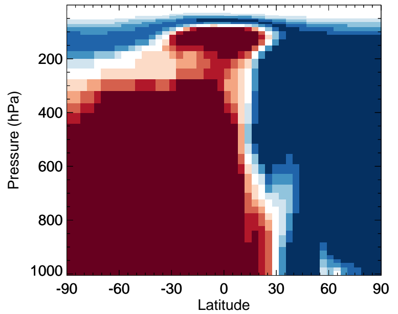
v11-02f-Run1 / v11-02e-Run1 ASOA2 - Zonal mean % diff for Apr
