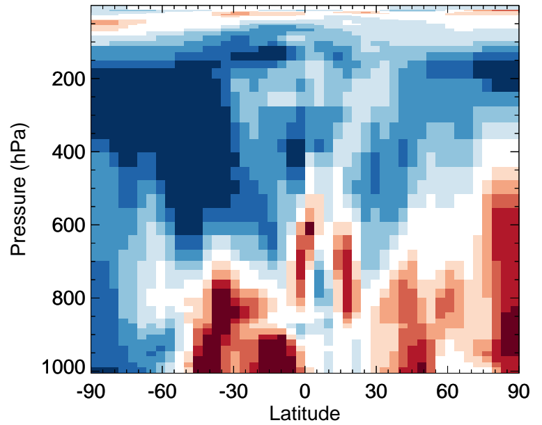
v11-02f-Run1 / v11-02e-Run0 SOAS - Zonal mean % diff for Apr
