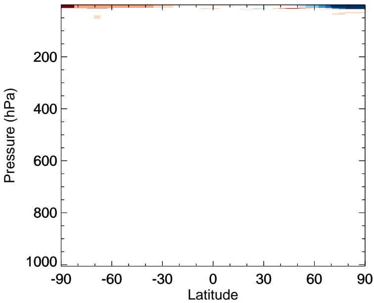
v11-02f-Run1 - v11-02e-Run0 ClO - Zonal mean abs diff for Apr
