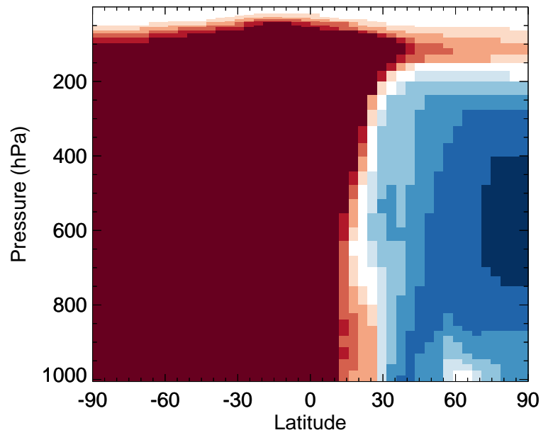
v11-02f-Run1 / v11-02e-Run1 ASOG3 - Zonal mean % diff for Apr
