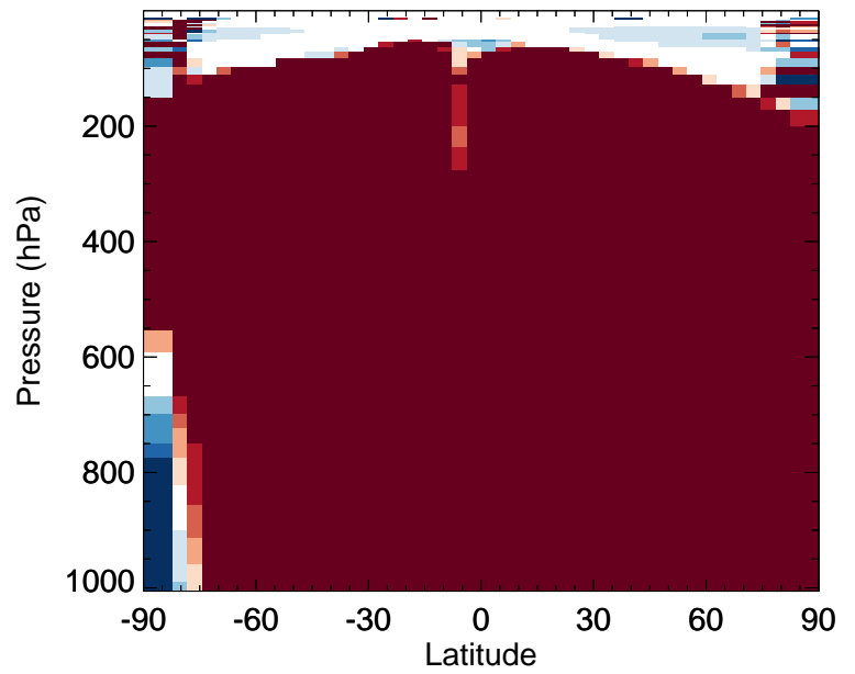
v11-02f-Run1 / v11-02e-Run1 LIMO - Zonal mean % diff for Apr
