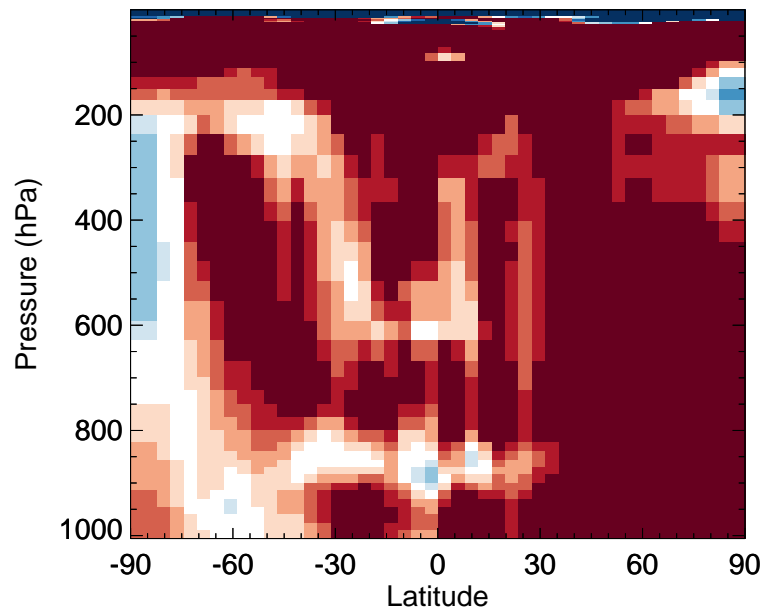
v11-02f-Run1 / v11-02e-Run0 ALD2 - Zonal mean % diff for Apr
