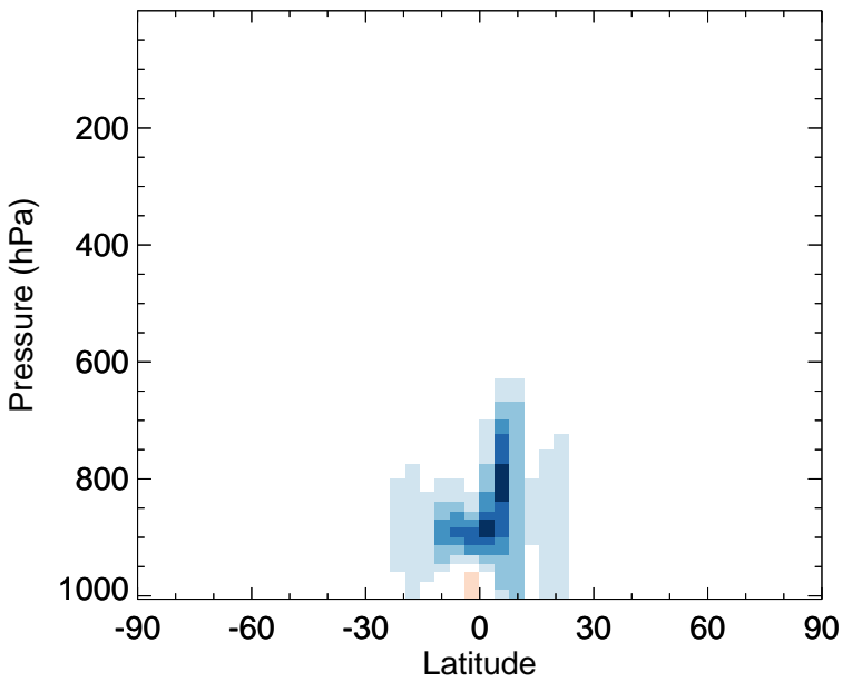
v11-02f-Run1 - v11-02e-Run0 MACR - Zonal mean abs diff for Apr
