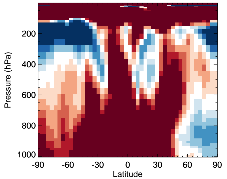
v11-02f-Run1 / v11-02e-Run0 EOH - Zonal mean % diff for Apr
