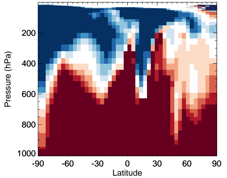
v11-02f-Run1 / v11-02e-Run1 MVKN - Zonal mean % diff for Apr
