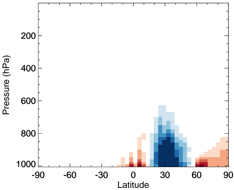
v11-02f-Run1 - v11-02e-Run0 TOLU - Zonal mean abs diff for Apr
