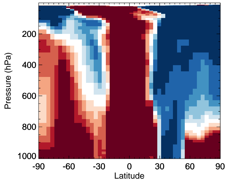
v11-02f-Run1 / v11-02e-Run1 TOLU - Zonal mean % diff for Apr
