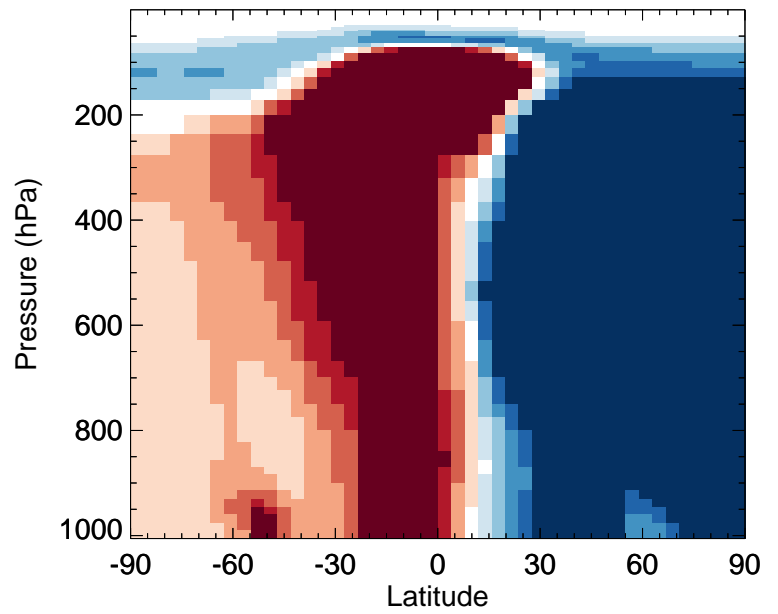
v11-02f-Run1 / v11-02e-Run1 ASOG2 - Zonal mean % diff for Apr
