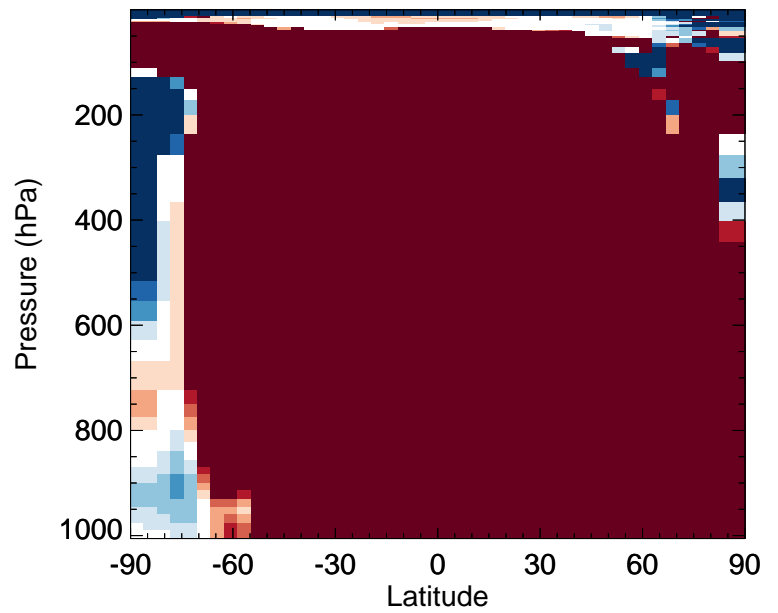
v11-02f-Run1 / v11-02e-Run0 HPALD - Zonal mean % diff for Apr
