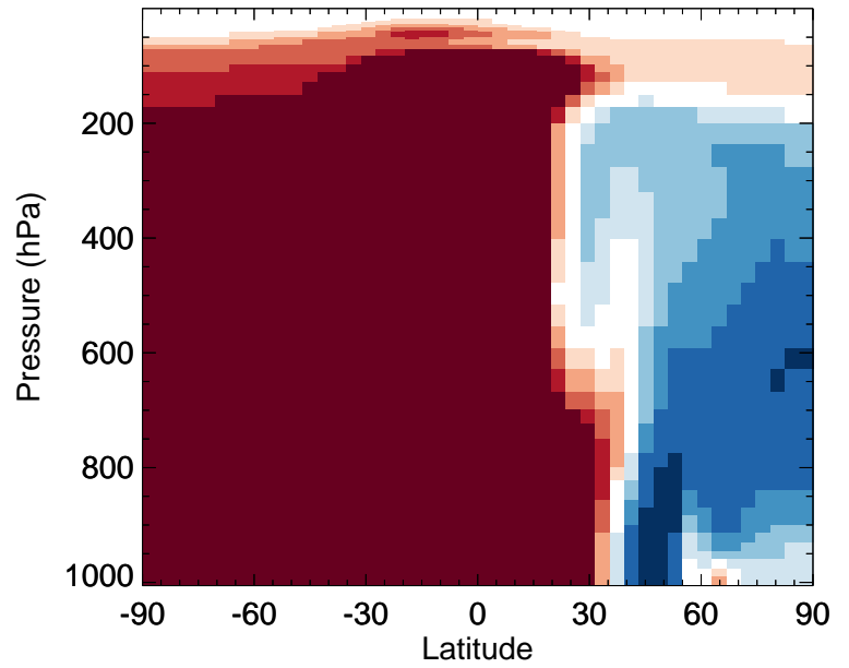
v11-02f-Run1 / v11-02e-Run1 ASOA3 - Zonal mean % diff for Apr
