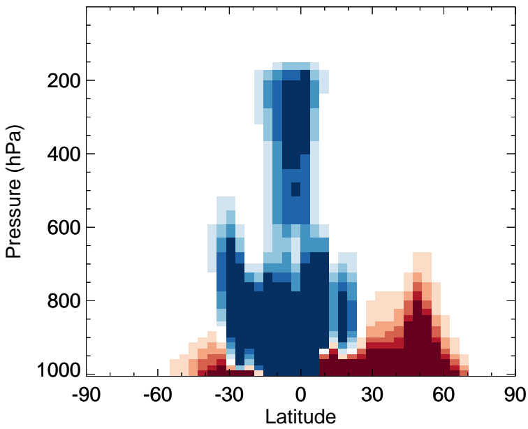
v11-02f-Run1 - v11-02e-Run1 PRPE - Zonal mean abs diff for Apr
