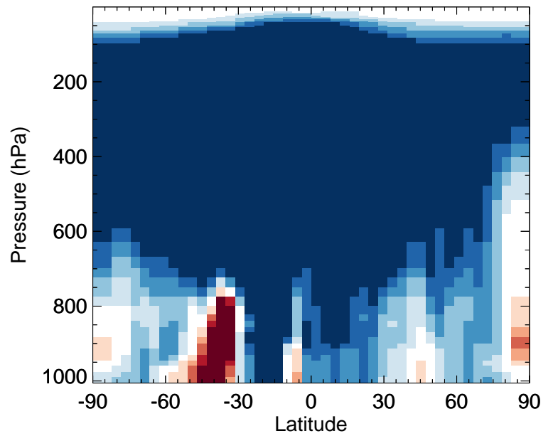
v11-02f-Run1 / v11-02e-Run0 SOAMG - Zonal mean % diff for Apr
