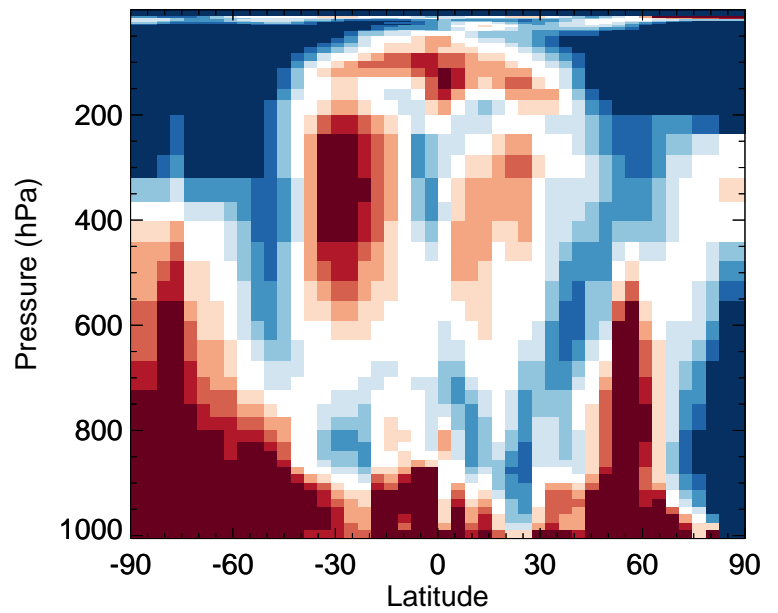
v11-02f-Run1 / v11-02e-Run0 HNO 2 - Zonal mean % diff for Apr
