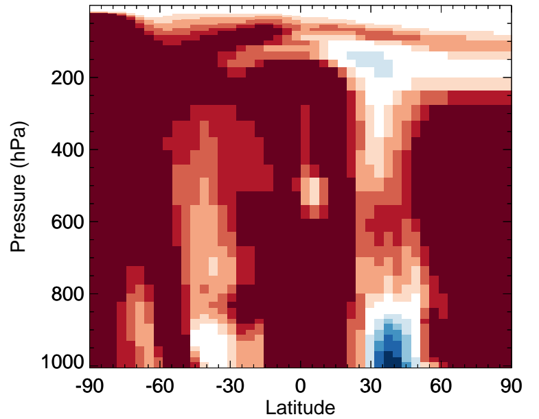
v11-02f-Run1 / v11-02e-Run0 ASOG3 - Zonal mean % diff for Jul
