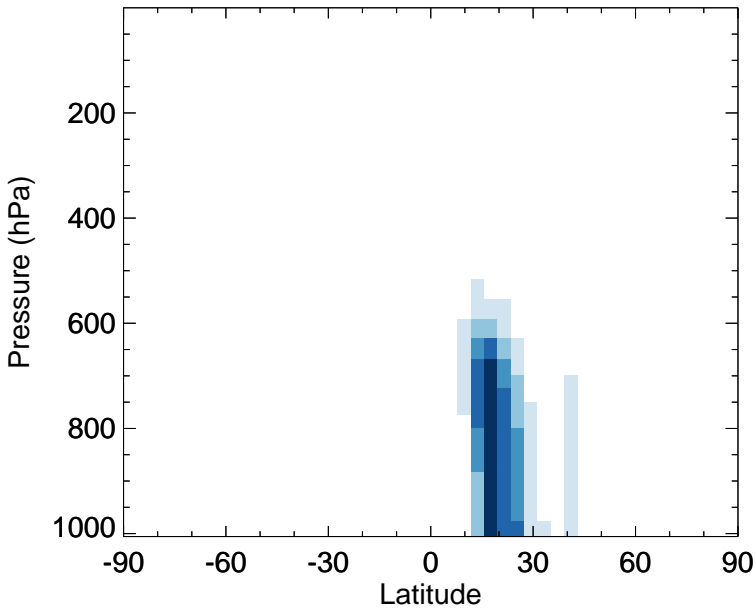
v11-02f-Run1 - v11-02e-Run0 DST2 - Zonal mean abs diff for Jul
