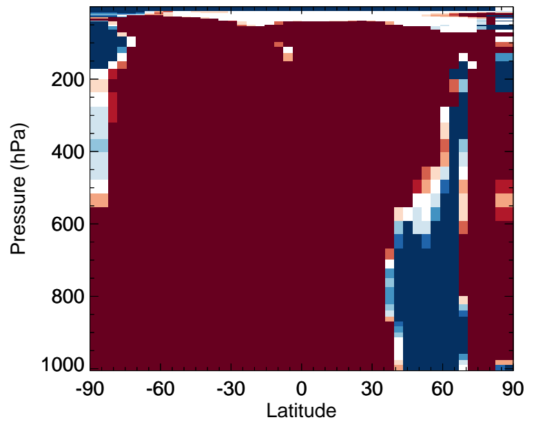
v11-02f-Run1 / v11-02e-Run0 ISN1 - Zonal mean % diff for Jul
