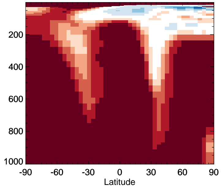
v11-02f-Run1 / v11-02e-Run1 MEK - Zonal mean % diff for Jul
