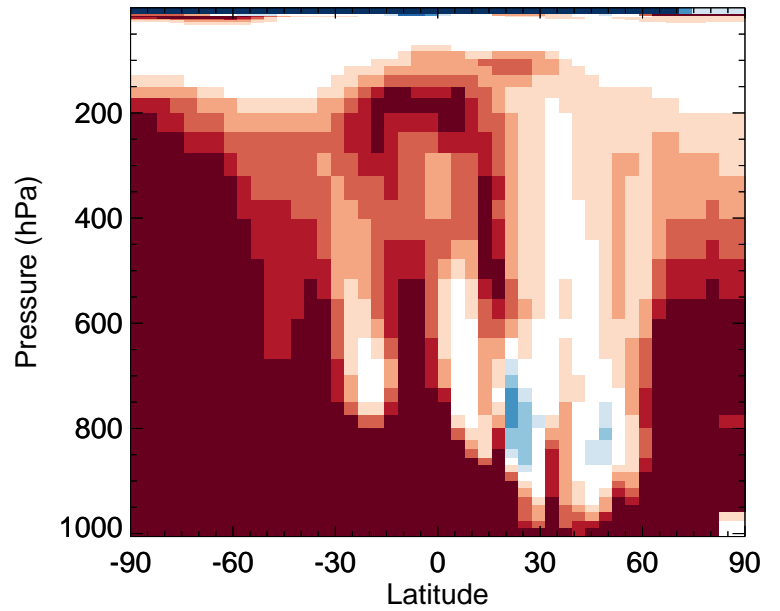
v11-02f-Run1 / v11-02e-Run0 PPN - Zonal mean % diff for Jul
