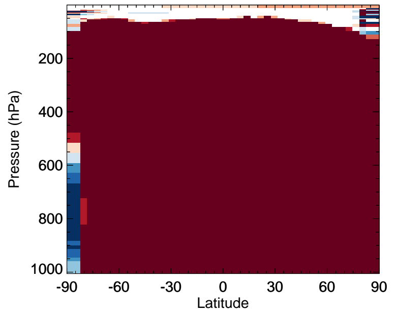
v11-02f-Run1 / v11-02e-Run1 MTPA - Zonal mean % diff for Jul
