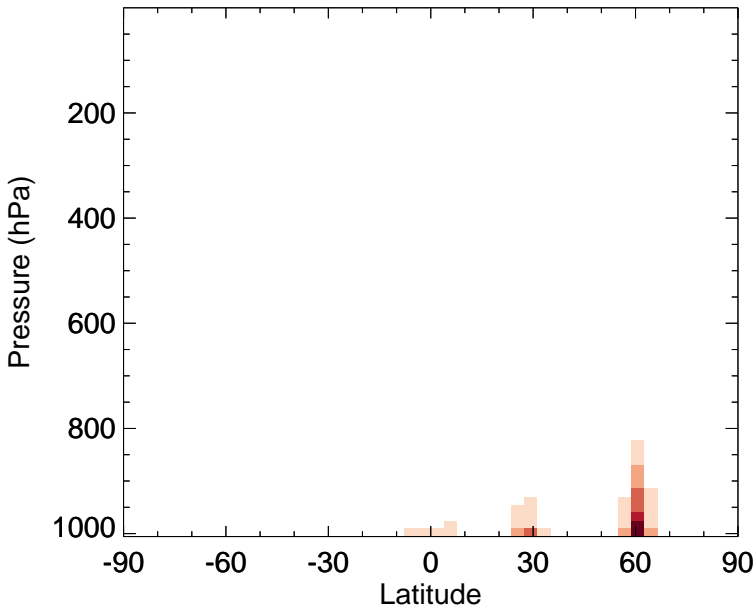
v11-02f-Run1 - v11-02e-Run0 SOAP - Zonal mean abs diff for Jul
