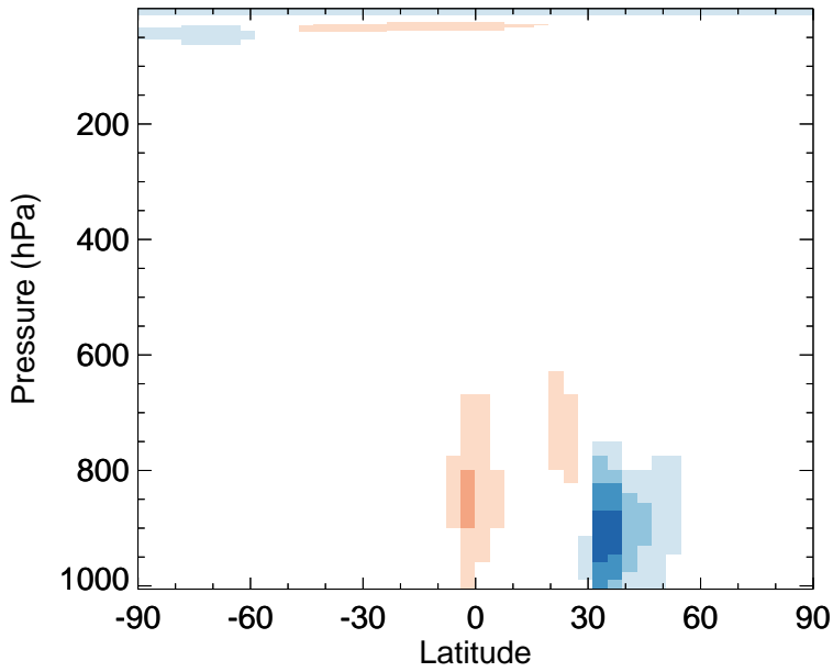
v11-02f-Run1 - v11-02e-Run1 H2O2 - Zonal mean abs diff for Jul
