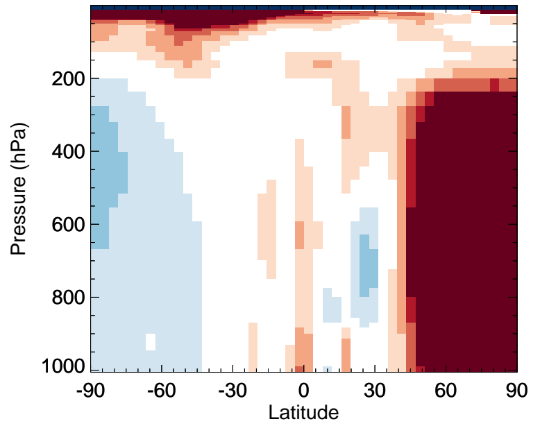
v11-02f-Run1 / v11-02e-Run1 C3H8 - Zonal mean % diff for Jul
