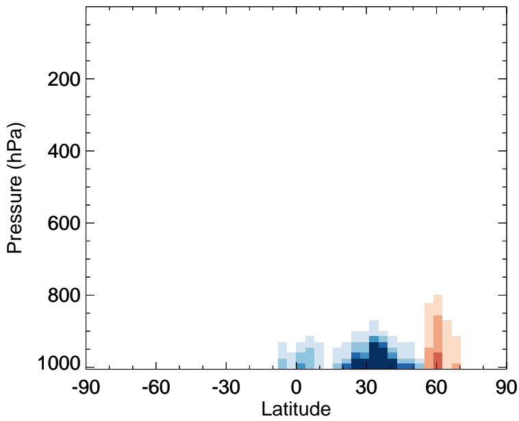
v11-02f-Run1 - v11-02e-Run1 XYLE - Zonal mean abs diff for Jul
