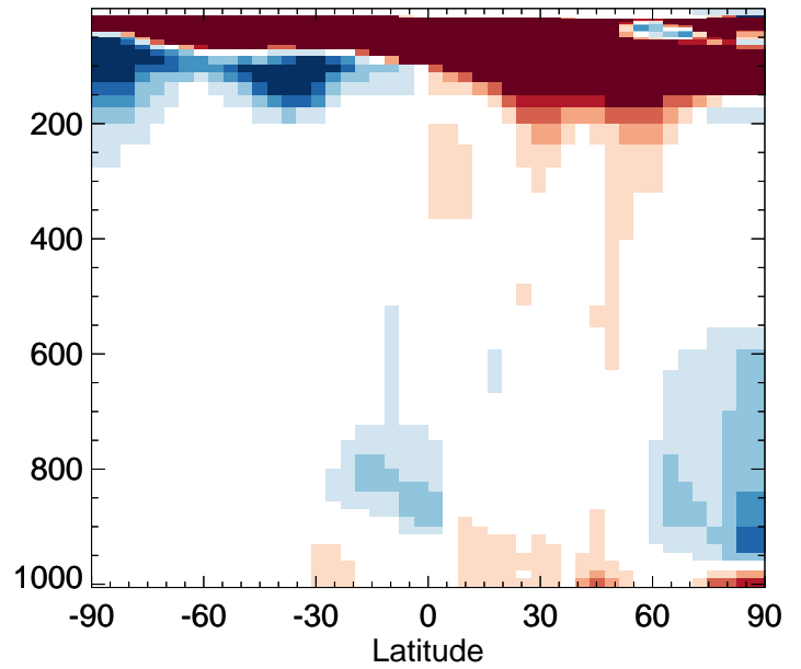
v11-02f-Run1 / v11-02e-Run0 CHBr3 - Zonal mean % diff for Jul
