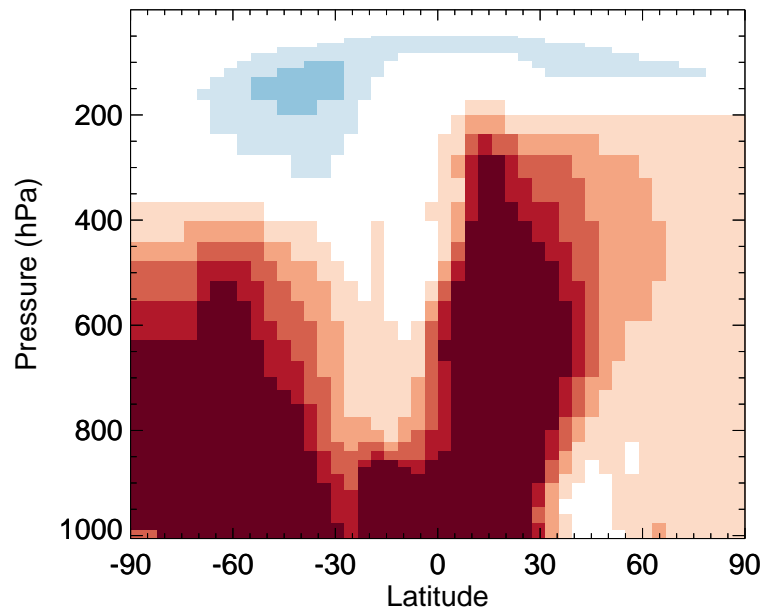
v11-02f-Run1 / v11-02e-Run1 ISOA2 - Zonal mean % diff for Jul
