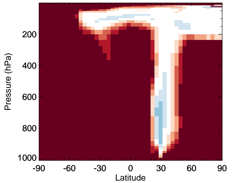
v11-02f-Run1 / v11-02e-Run1 RCHO - Zonal mean % diff for Jul
