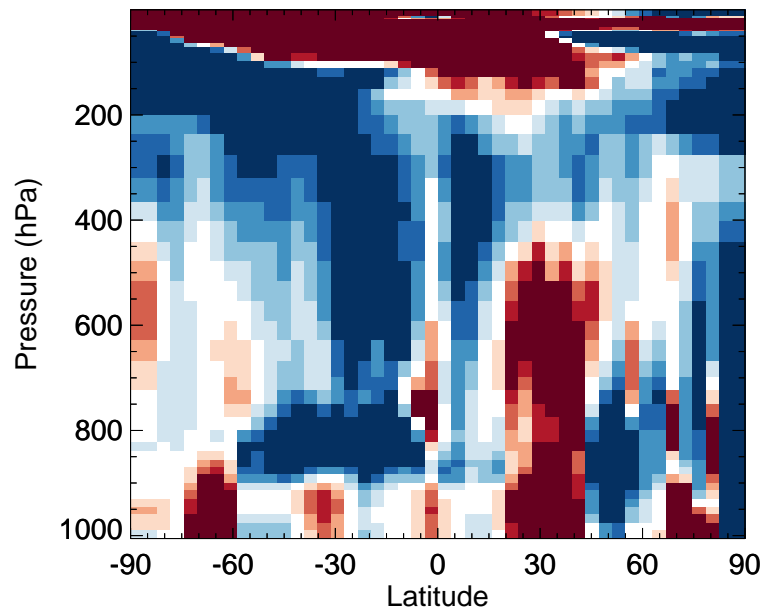
v11-02f-Run1 / v11-02e-Run0 SALC - Zonal mean % diff for Jul
