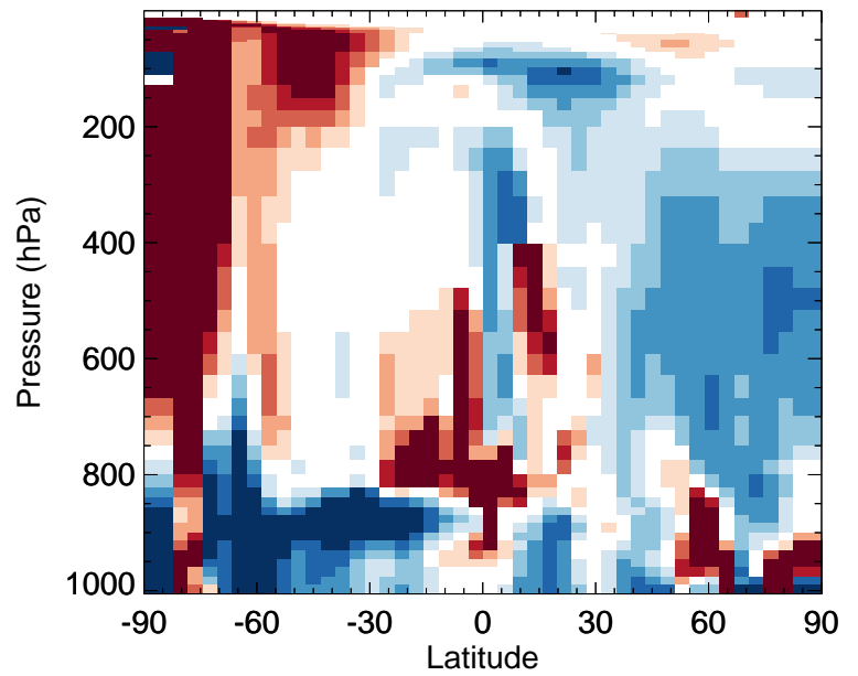
v11-02f-Run1 / v11-02e-Run0 BrO - Zonal mean % diff for Jul
