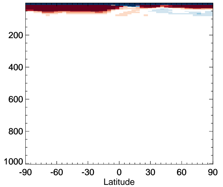
v11-02f-Run1 / v11-02e-Run0 CH3Br - Zonal mean % diff for Jul
