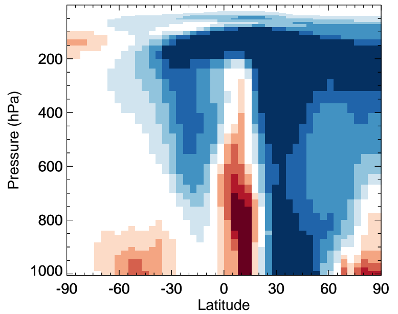
v11-02f-Run1 / v11-02e-Run1 ASOG2 - Zonal mean % diff for Jul
