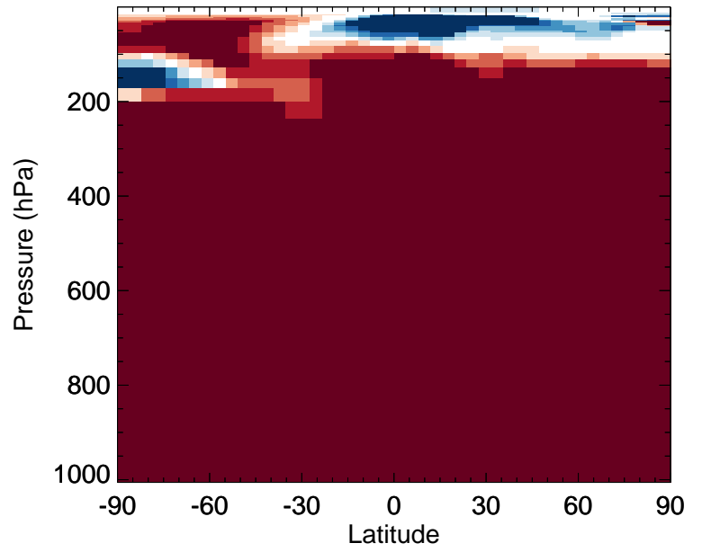
v11-02f-Run1 / v11-02e-Run1 HONIT - Zonal mean % diff for Jul
