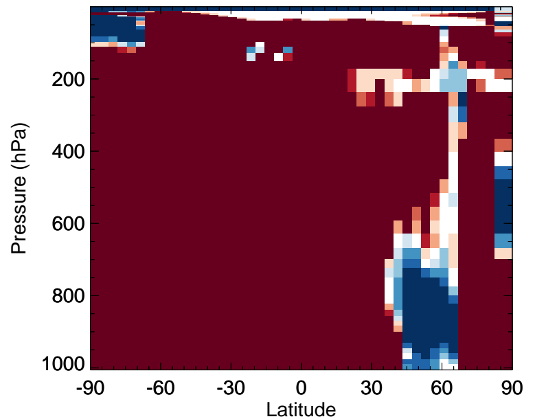
v11-02f-Run1 / v11-02e-Run0 MACR - Zonal mean % diff for Jul
