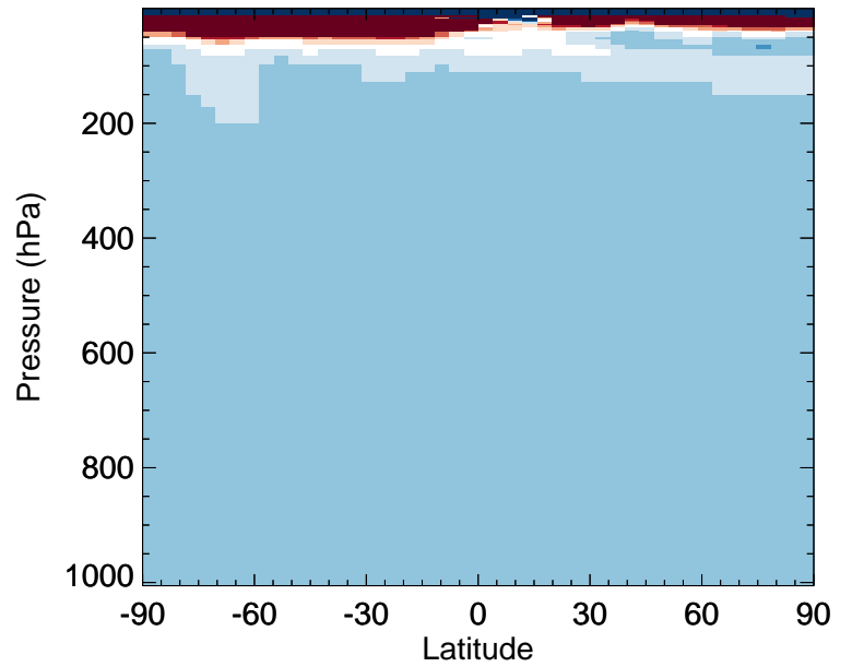
v11-02f-Run1 / v11-02e-Run0 H2402 - Zonal mean % diff for Jul
