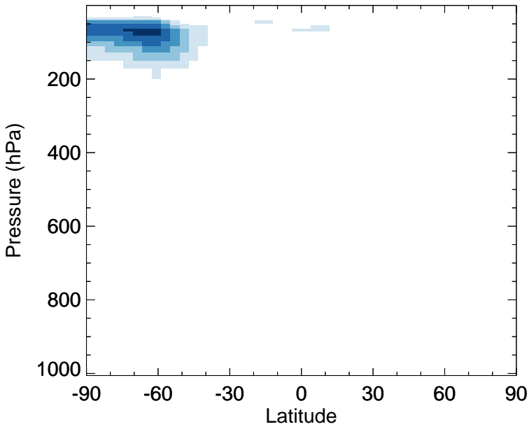
v11-02f-Run1 - v11-02e-Run0 MPN - Zonal mean abs diff for Jul
