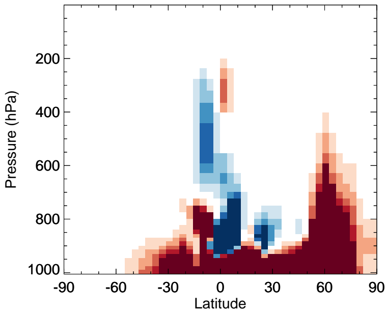
v11-02f-Run1 - v11-02e-Run0 PRPE - Zonal mean abs diff for Jul
