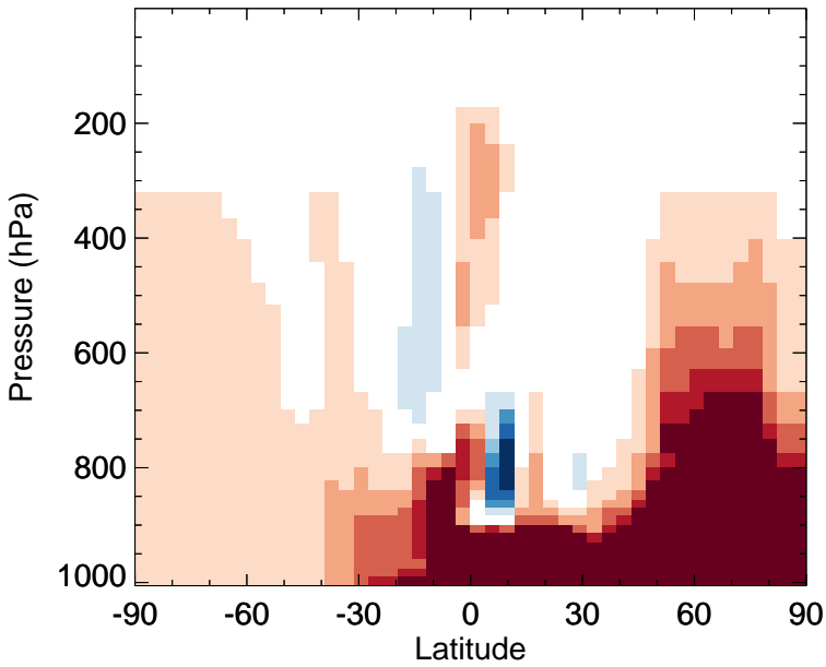
v11-02f-Run1 - v11-02e-Run0 MEK - Zonal mean abs diff for Jul
