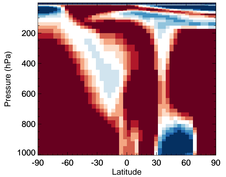
v11-02f-Run1 / v11-02e-Run1 GLYX - Zonal mean % diff for Jul
