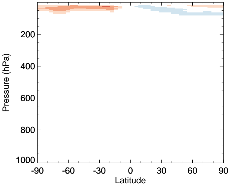
v11-02f-Run1 - v11-02e-Run0 CFC12 - Zonal mean abs diff for Jul
