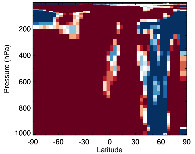
v11-02f-Run1 / v11-02e-Run0 IEPOXB - Zonal mean % diff for Jul
