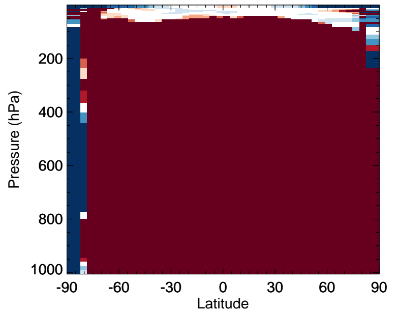
v11-02f-Run1 / v11-02e-Run0 MTPA - Zonal mean % diff for Jul
