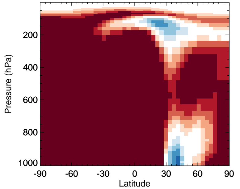
v11-02f-Run1 / v11-02e-Run1 ASOA1 - Zonal mean % diff for Jul
