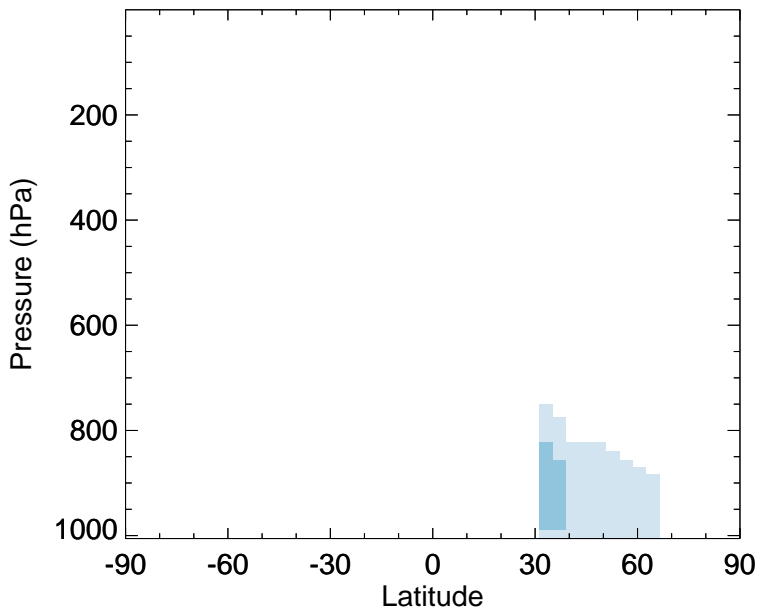
v11-02f-Run1 - v11-02e-Run1 ISO3 - Zonal mean abs diff for Jul
