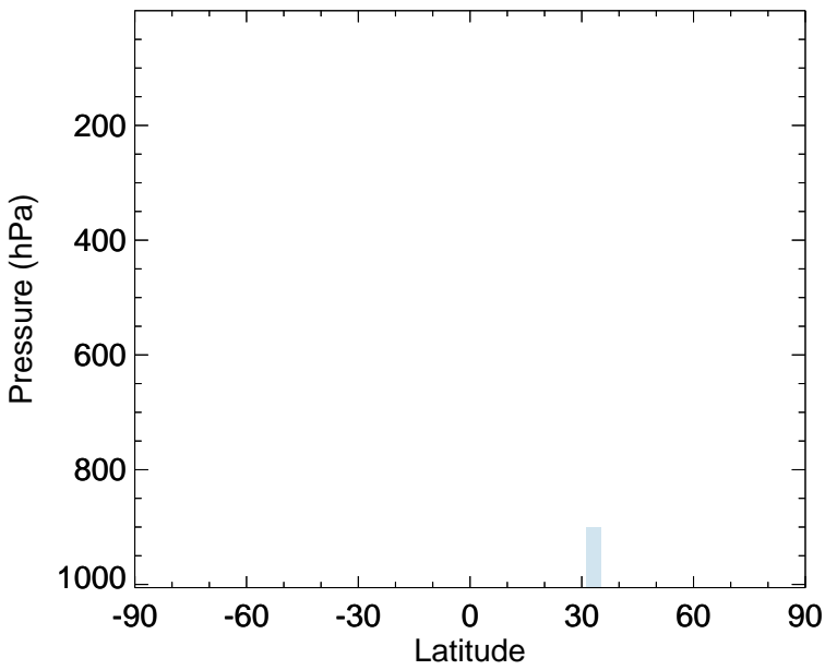
v11-02f-Run1 - v11-02e-Run1 IPMN - Zonal mean abs diff for Jul
