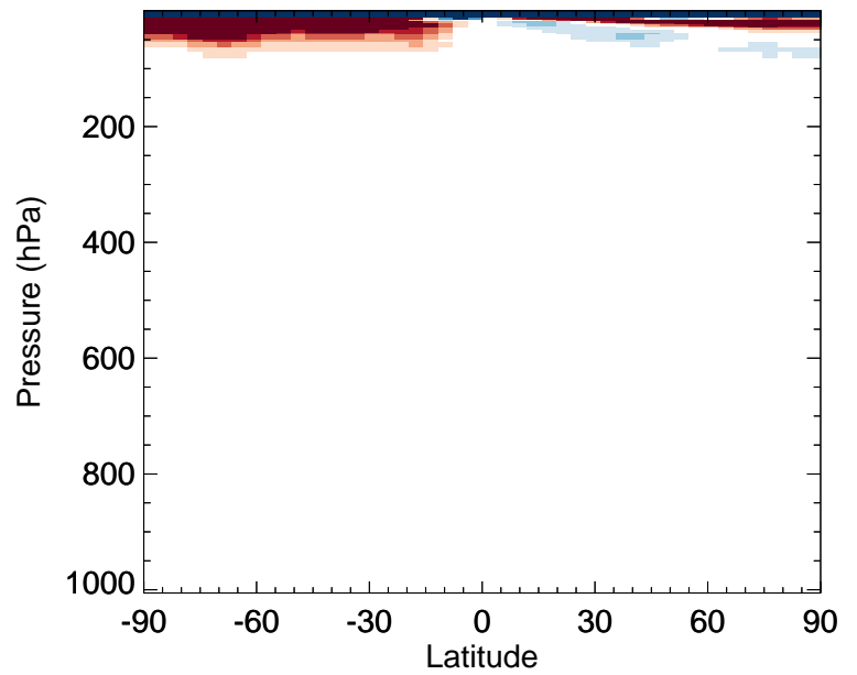
v11-02f-Run1 / v11-02e-Run0 CH3Cl - Zonal mean % diff for Jul
