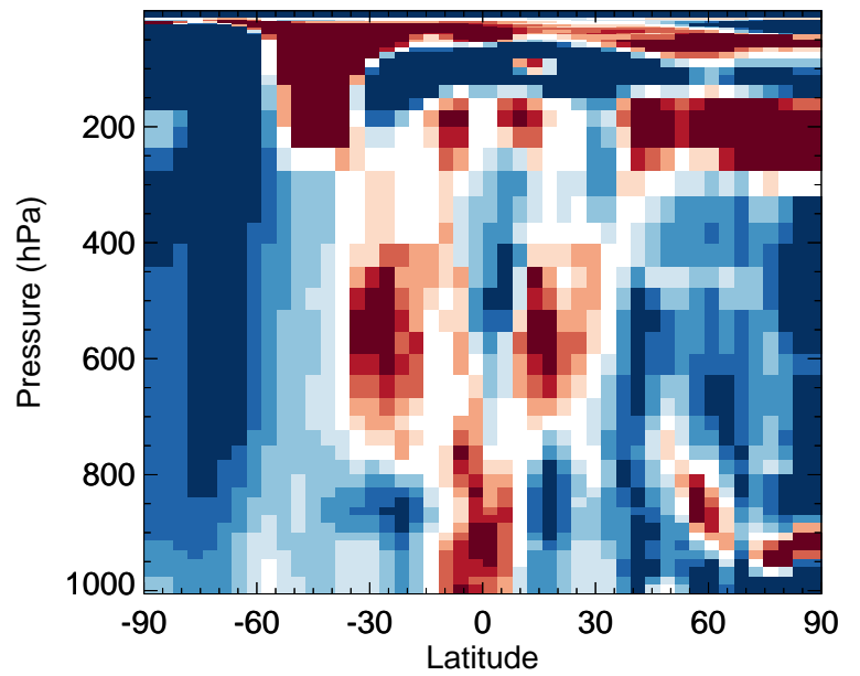
v11-02f-Run1 / v11-02e-Run0 HOCl - Zonal mean % diff for Jul
