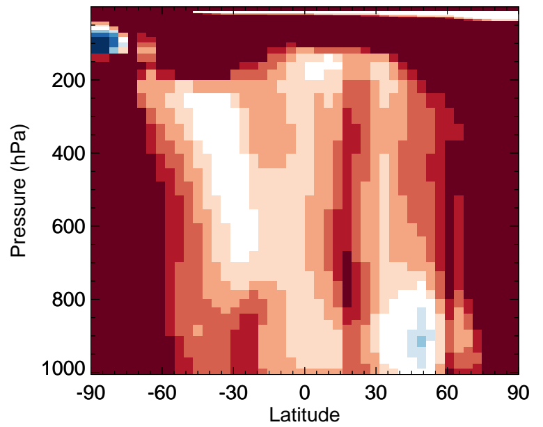
v11-02f-Run1 / v11-02e-Run1 ACTA - Zonal mean % diff for Jul
