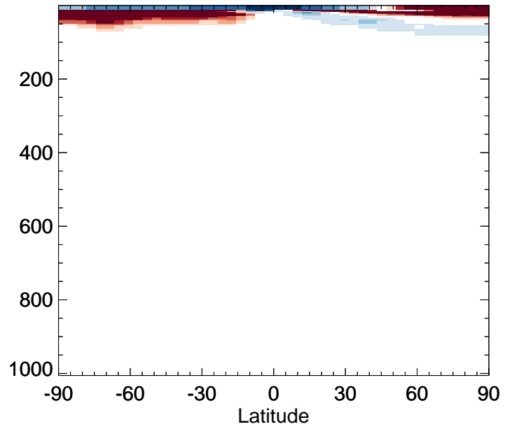
v11-02f-Run1 / v11-02e-Run0 CFC12 - Zonal mean % diff for Jul
