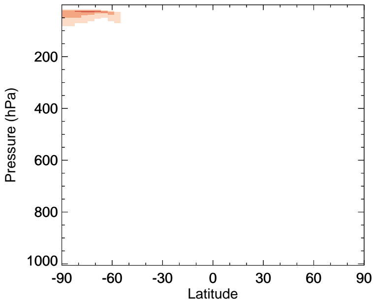
v11-02f-Run1 - v11-02e-Run0 OCIO - Zonal mean abs diff for Jul
