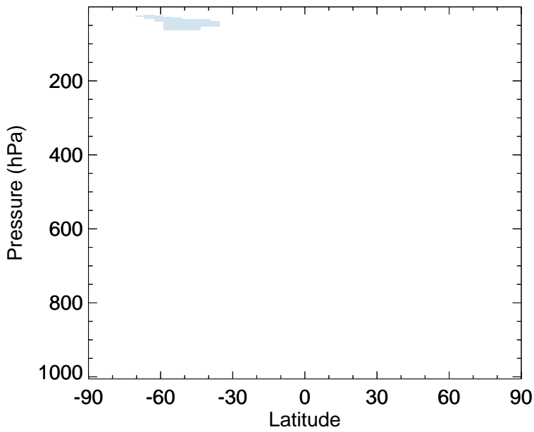
v11-02f-Run1 - v11-02e-Run1 BrNO3 - Zonal mean abs diff for Jul
