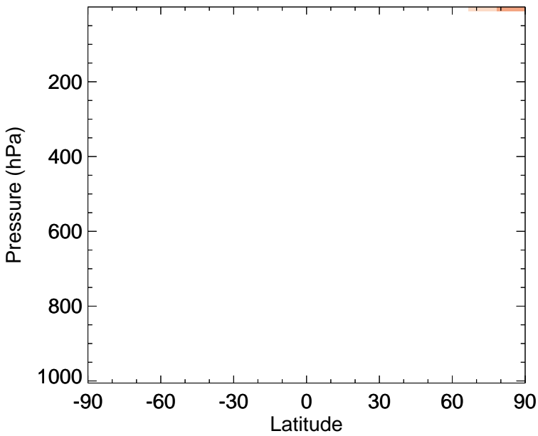
v11-02f-Run1 - v11-02e-Run0 ACTA - Zonal mean abs diff for Jul
