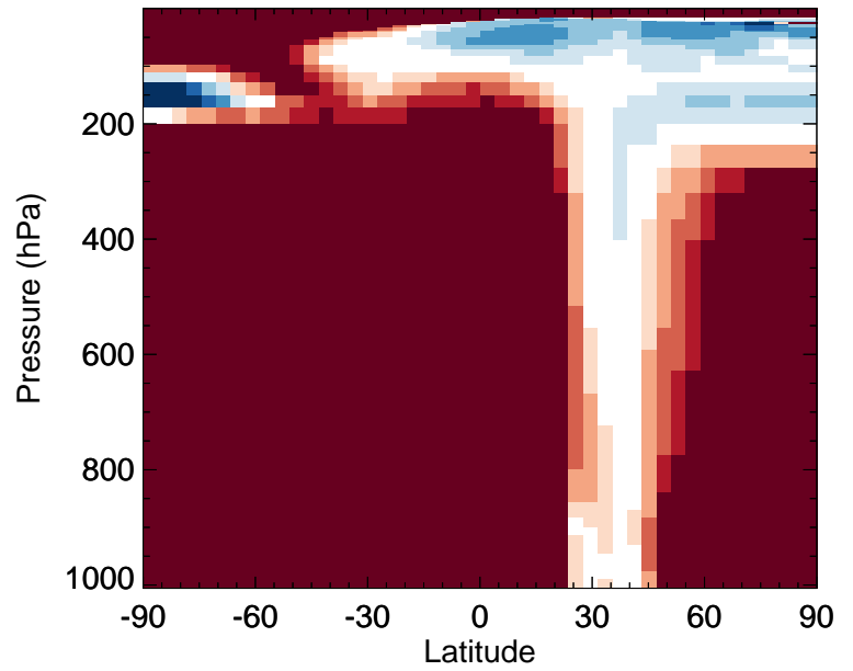
v11-02f-Run1 / v11-02e-Run1 R4N2 - Zonal mean % diff for Jul
