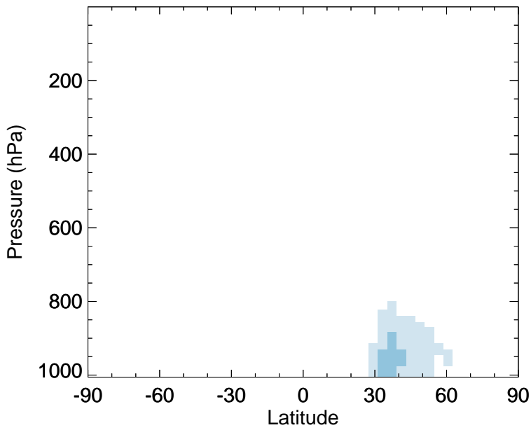
v11-02f-Run1 - v11-02e-Run1 SOAGX - Zonal mean abs diff for Jul
