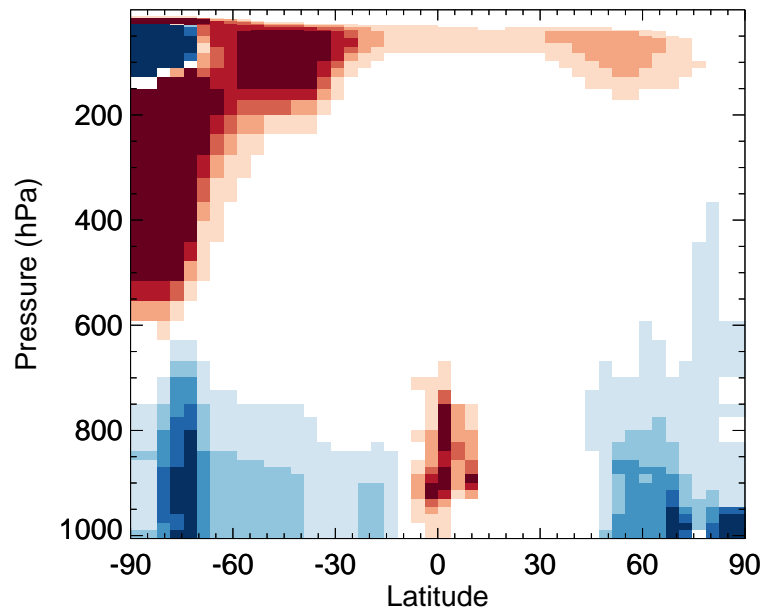
v11-02f-Run1 / v11-02e-Run1 BrO - Zonal mean % diff for Jul
