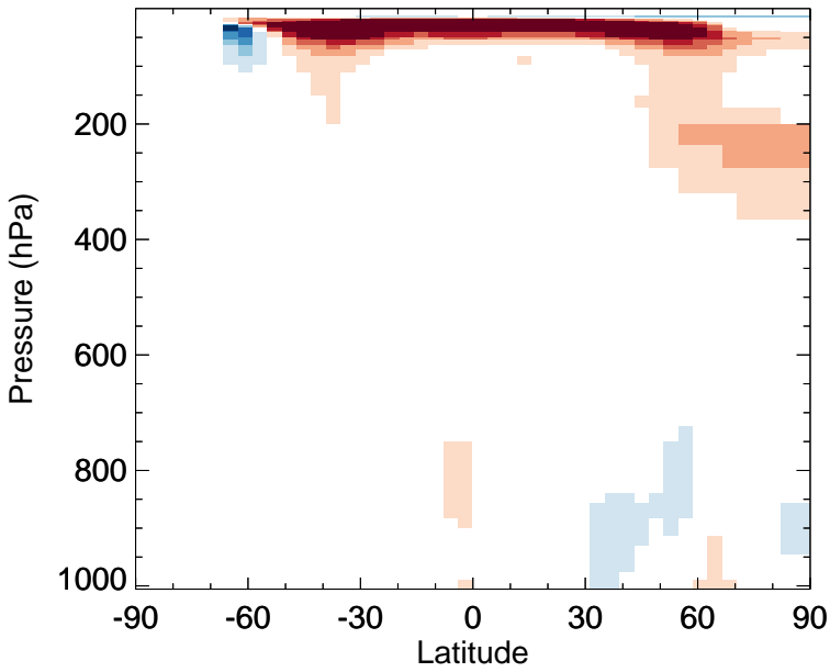
v11-02f-Run1 - v11-02e-Run1 HO2 - Zonal mean abs diff for Jul
