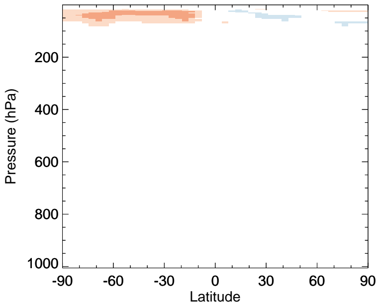
v11-02f-Run1 - v11-02e-Run0 CH3Cl - Zonal mean abs diff for Jul
