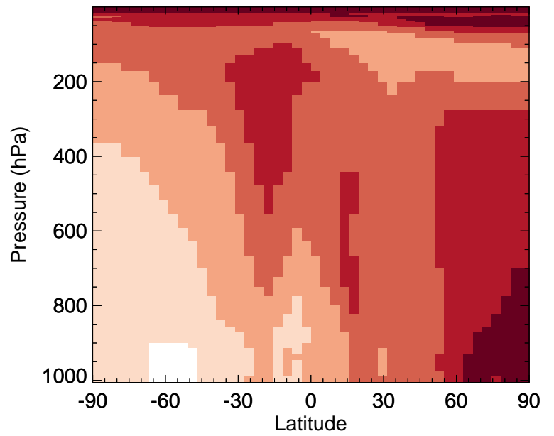
v11-02f-Run1 / v11-02e-Run1 ACET - Zonal mean % diff for Jul
