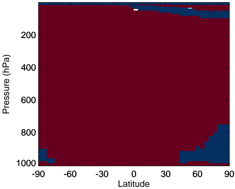
v11-02f-Run1 - v11-02e-Run0 CH4 - Zonal mean abs diff for Jul
