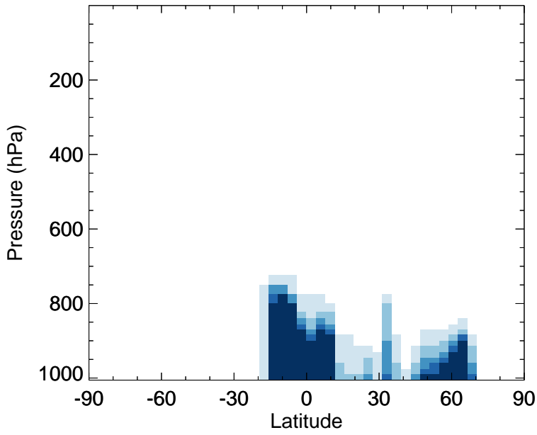
v11-02f-Run1 - v11-02e-Run1 ISOP - Zonal mean abs diff for Jul
