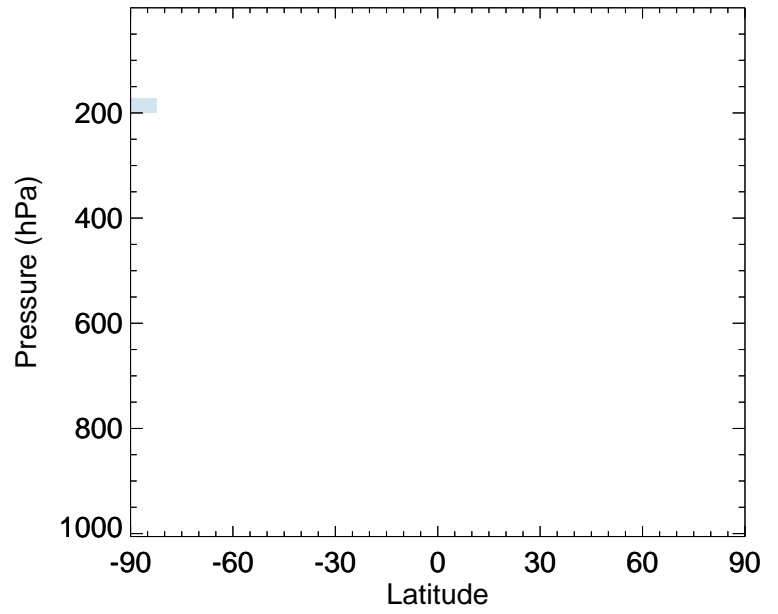
v11-02f-Run1 / v11-02e-Run1 SALA - Zonal mean % diff for Jul
