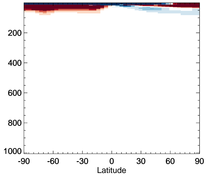
v11-02f-Run1 / v11-02e-Run0 H1301 - Zonal mean % diff for Jul
