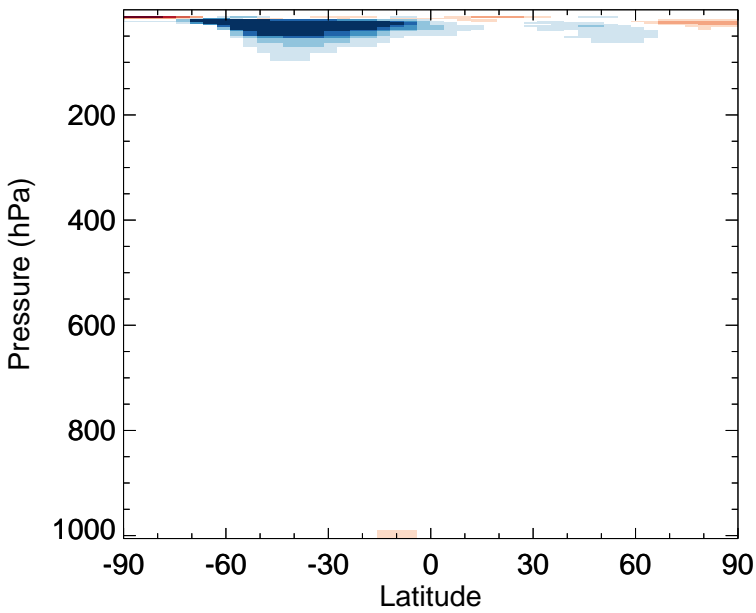
v11-02f-Run1 - v11-02e-Run0 NO2 - Zonal mean abs diff for Jul
