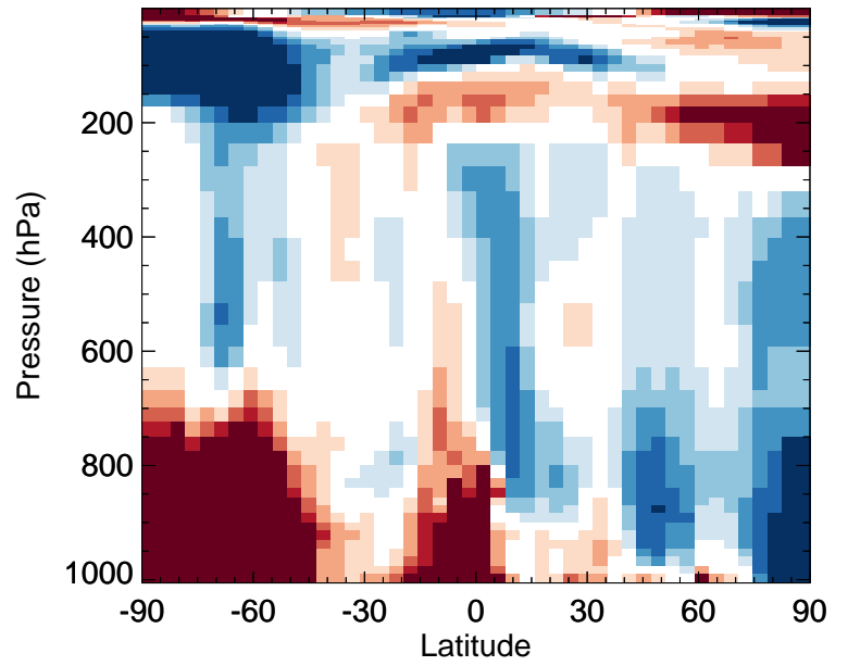
v11-02f-Run1 / v11-02e-Run0 MPN - Zonal mean % diff for Jul
