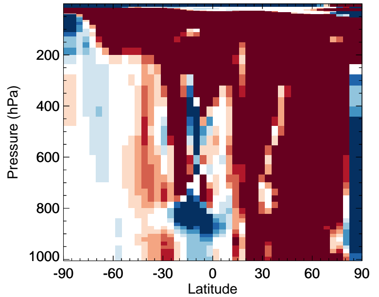
v11-02f-Run1 / v11-02e-Run0 DMS - Zonal mean % diff for Jul
