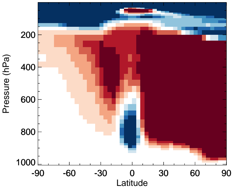
v11-02f-Run1 - v11-02e-Run1 CH4 - Zonal mean abs diff for Jul
