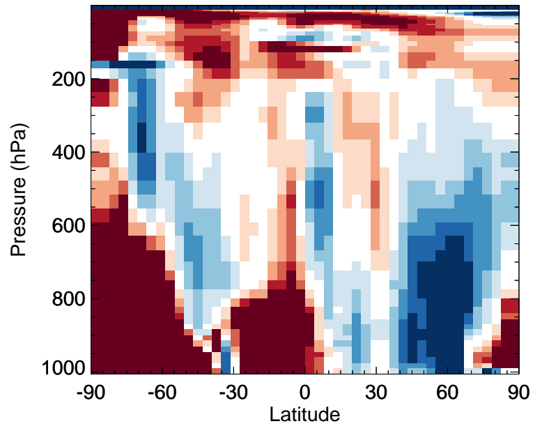
v11-02f-Run1 / v11-02e-Run0 HNO 3 - Zonal mean % diff for Jul
