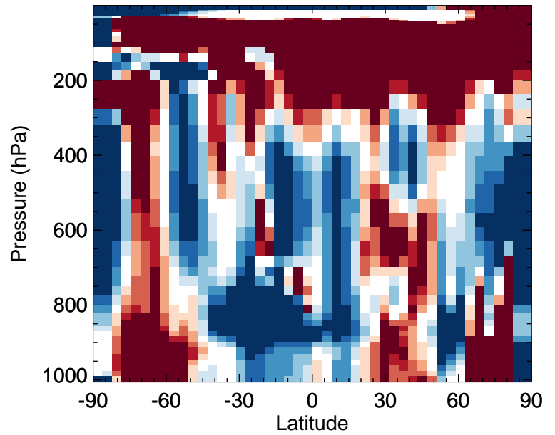
v11-02f-Run1 / v11-02e-Run0 NITs - Zonal mean % diff for Jul
