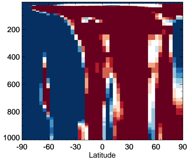
v11-02f-Run1 / v11-02e-Run0 DST4 - Zonal mean % diff for Jul
