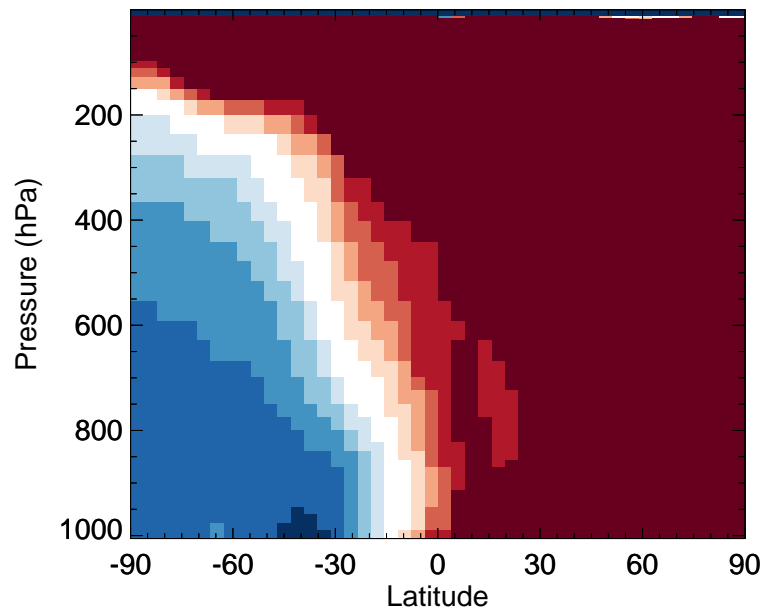
v11-02f-Run1 / v11-02e-Run0 C2H6 - Zonal mean % diff for Jul
