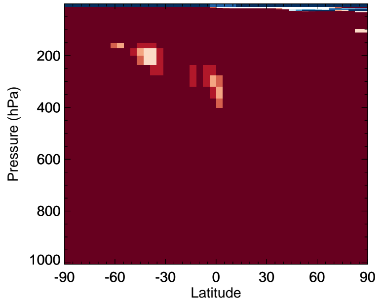
v11-02f-Run1 / v11-02e-Run0 HONIT - Zonal mean % diff for Jul
