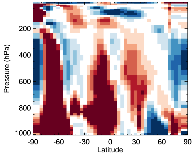
v11-02f-Run1 / v11-02e-Run0 NO3 - Zonal mean % diff for Jul
