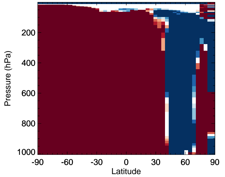
v11-02f-Run1 / v11-02e-Run1 ISOP - Zonal mean % diff for Jul
