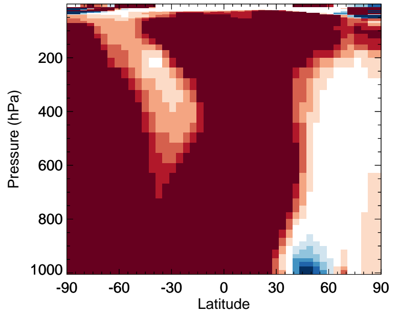
v11-02f-Run1 / v11-02e-Run1 OCPO - Zonal mean % diff for Jul
