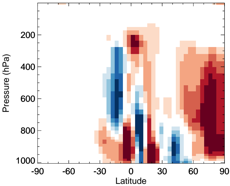
v11-02f-Run1 - v11-02e-Run0 MAP - Zonal mean abs diff for Jul
