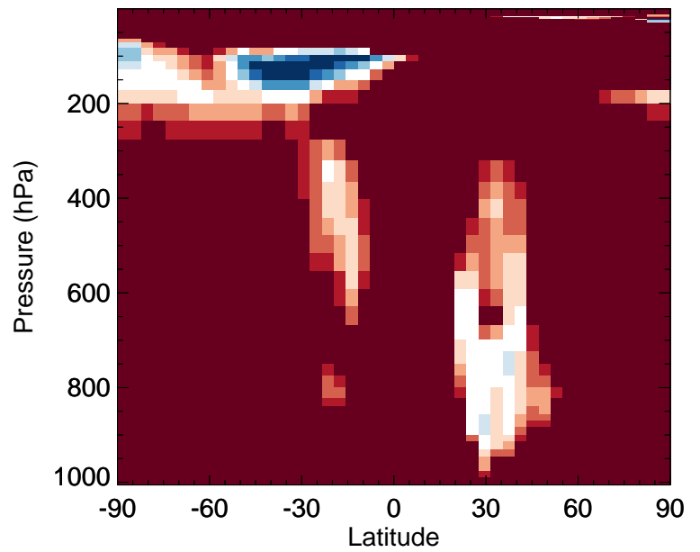
v11-02f-Run1 / v11-02e-Run0 RCHO - Zonal mean % diff for Jul
