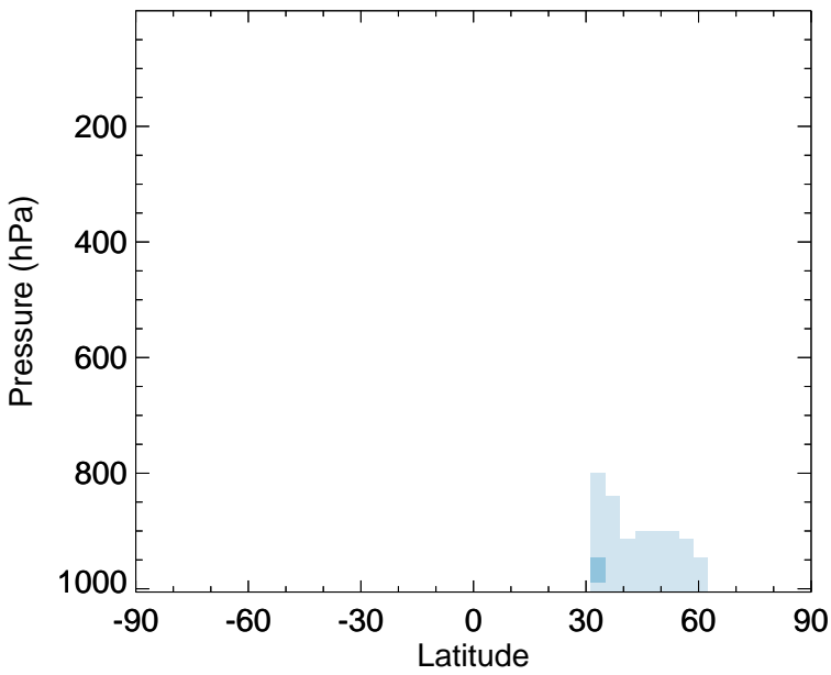
v11-02f-Run1 - v11-02e-Run1 CH 2 O - Zonal mean abs diff for Jul
