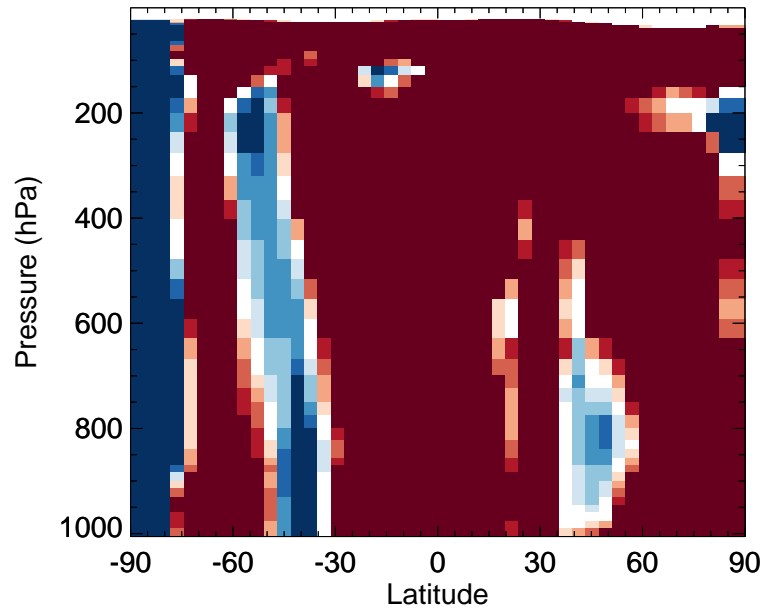
v11-02f-Run1 / v11-02e-Run0 SOAP - Zonal mean % diff for Jul
