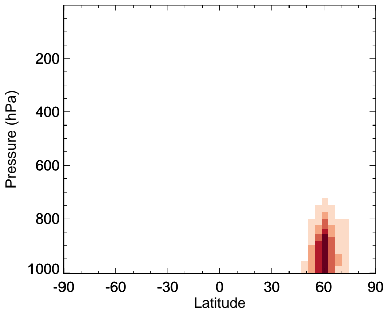
v11-02f-Run1 - v11-02e-Run1 ALD2 - Zonal mean abs diff for Jul
