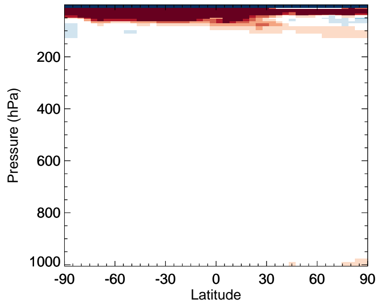
v11-02f-Run1 / v11-02e-Run0 CH2Br2 - Zonal mean % diff for Jul
