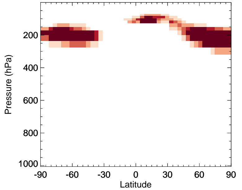
v11-02f-Run1 / v11-02e-Run1 H2O - Zonal mean % diff for Jul
