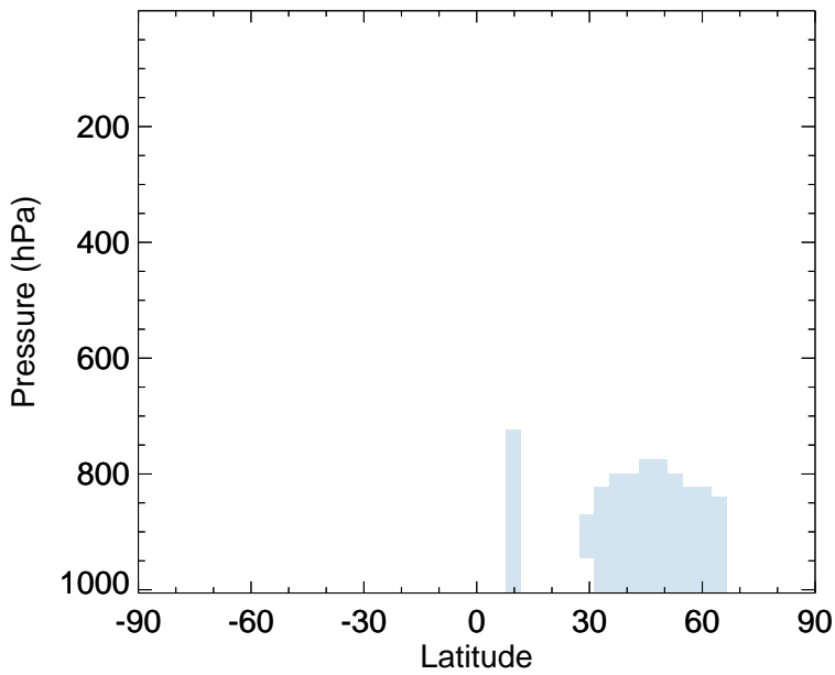
v11-02f-Run1 - v11-02e-Run0 ISO3 - Zonal mean abs diff for Jul
