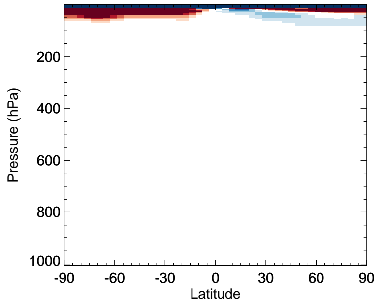
v11-02f-Run1 / v11-02e-Run0 CFC113 - Zonal mean % diff for Jul
