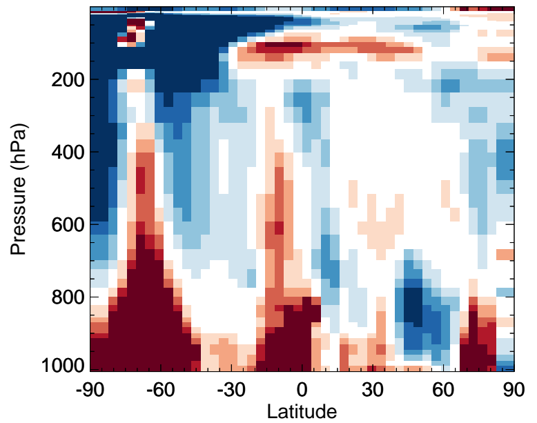
v11-02f-Run1 / v11-02e-Run0 NO2 - Zonal mean % diff for Jul
