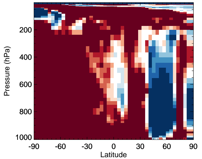
v11-02f-Run1 / v11-02e-Run0 HCOOH - Zonal mean % diff for Jul
