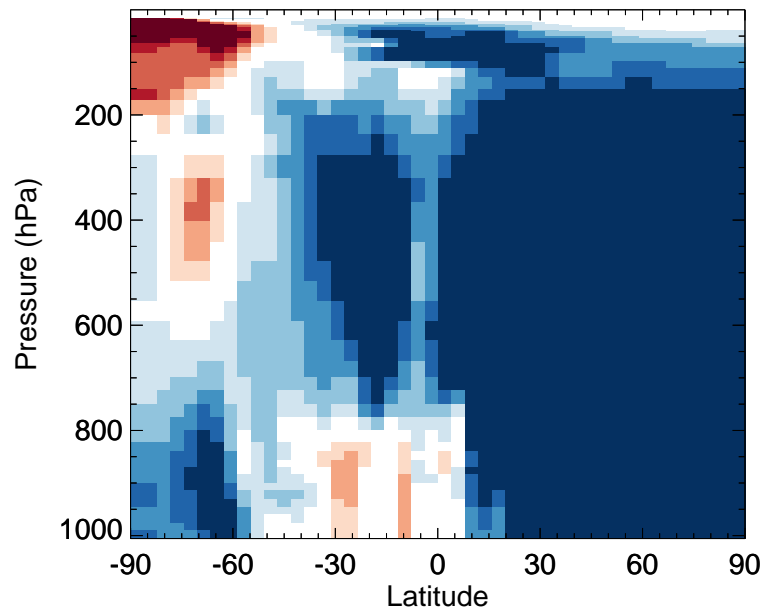
v11-02f-Run1 / v11-02e-Run0 ISOG1 - Zonal mean % diff for Jul
