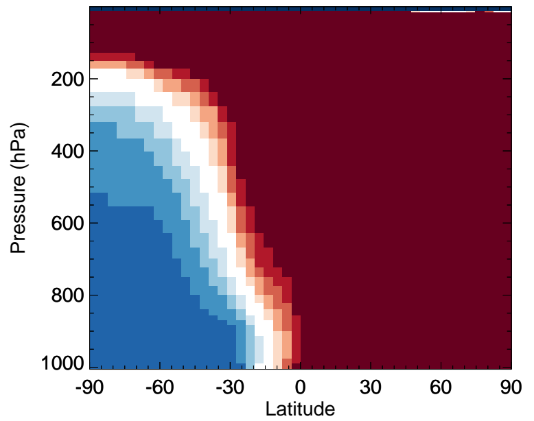
v11-02f-Run1 / v11-02e-Run1 C2H6 - Zonal mean % diff for Jul
