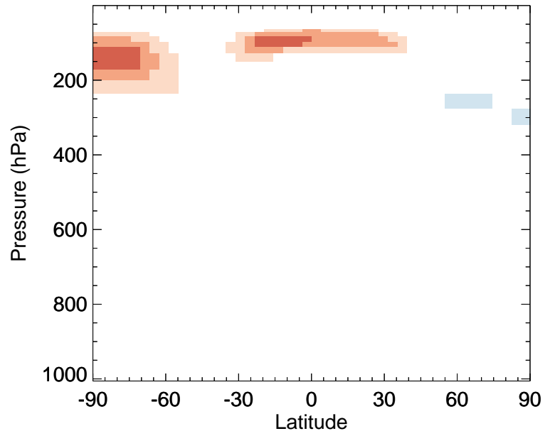
v11-02f-Run1 / v11-02e-Run1 ISOG2 - Zonal mean % diff for Jul
