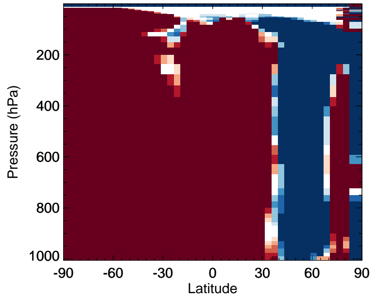
v11-02f-Run1 / v11-02e-Run1 RIPA - Zonal mean % diff for Jul
