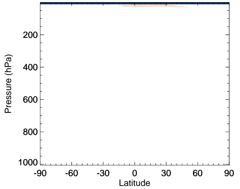
v11-02f-Run1 / v11-02e-Run1 CCI4 - Zonal mean % diff for Jul
