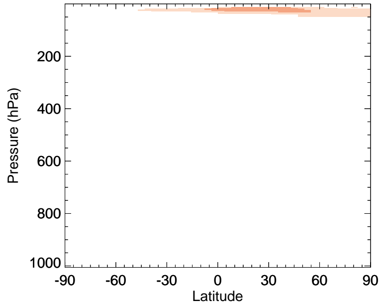
v11-02f-Run1 / v11-02e-Run1 H1211 - Zonal mean % diff for Jul
