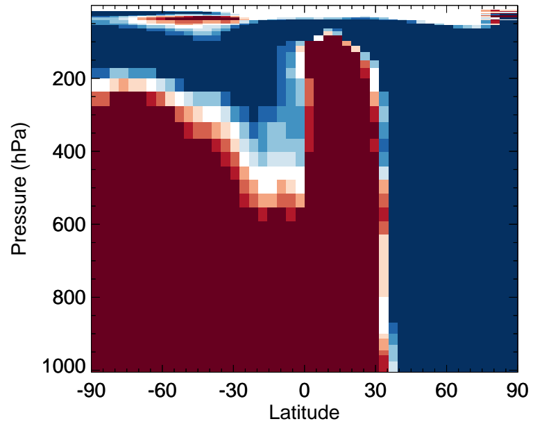
v11-02f-Run1 / v11-02e-Run1 MVKN - Zonal mean % diff for Jul
