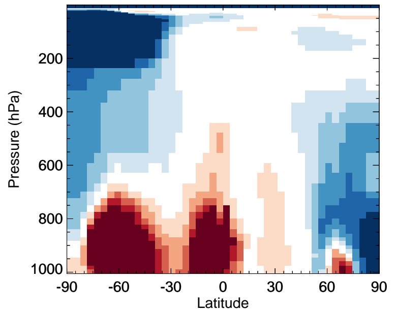
v11-02f-Run1 / v11-02e-Run1 HNO 4 - Zonal mean % diff for Jul
