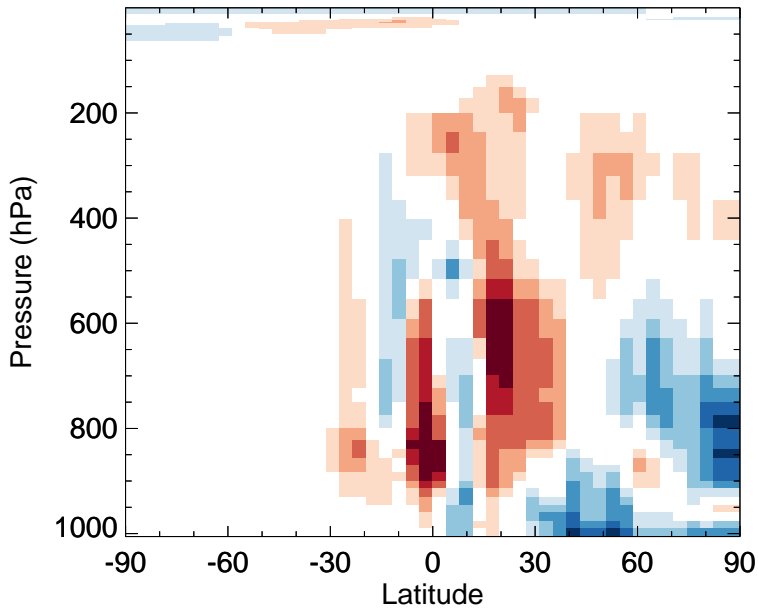
v11-02f-Run1 - v11-02e-Run0 H2O2 - Zonal mean abs diff for Jul
