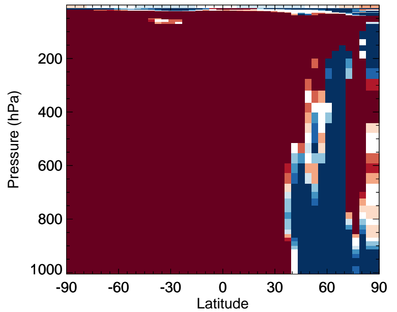
v11-02f-Run1 / v11-02e-Run0 ISN1OG - Zonal mean % diff for Jul
