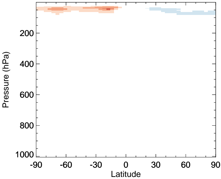
v11-02f-Run1 - v11-02e-Run0 OCS - Zonal mean abs diff for Jul
