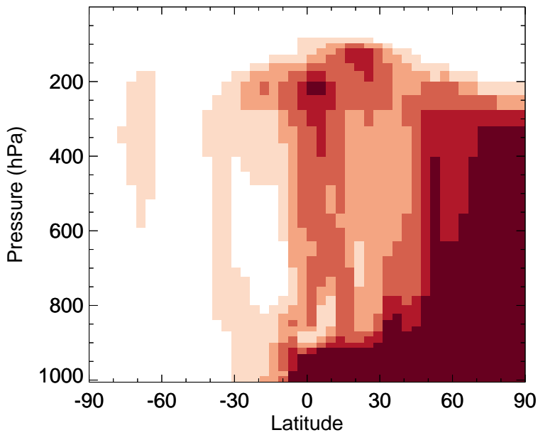
v11-02f-Run1 - v11-02e-Run0 ACET - Zonal mean abs diff for Jul
