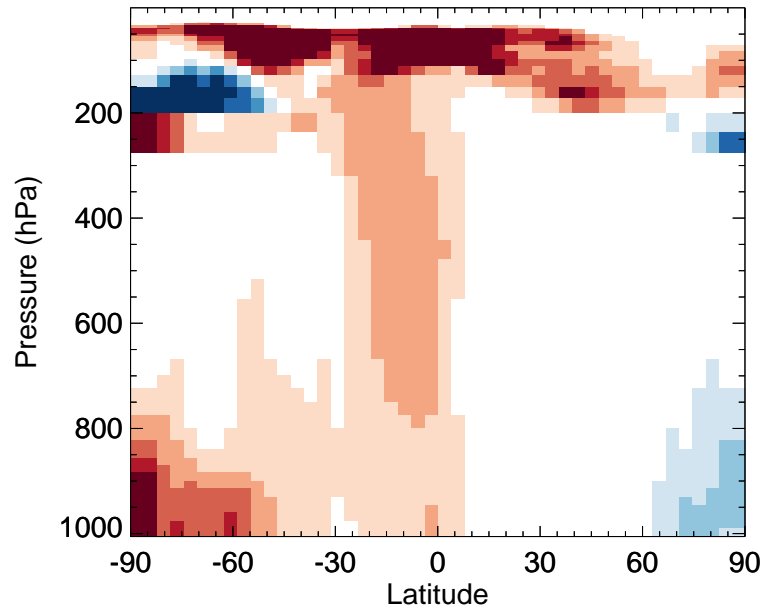
v11-02f-Run1 / v11-02e-Run1 NITs - Zonal mean % diff for Jul
