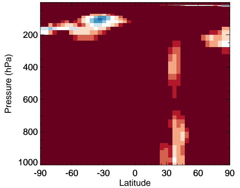
v11-02f-Run1 / v11-02e-Run0 R4N2 - Zonal mean % diff for Jul
