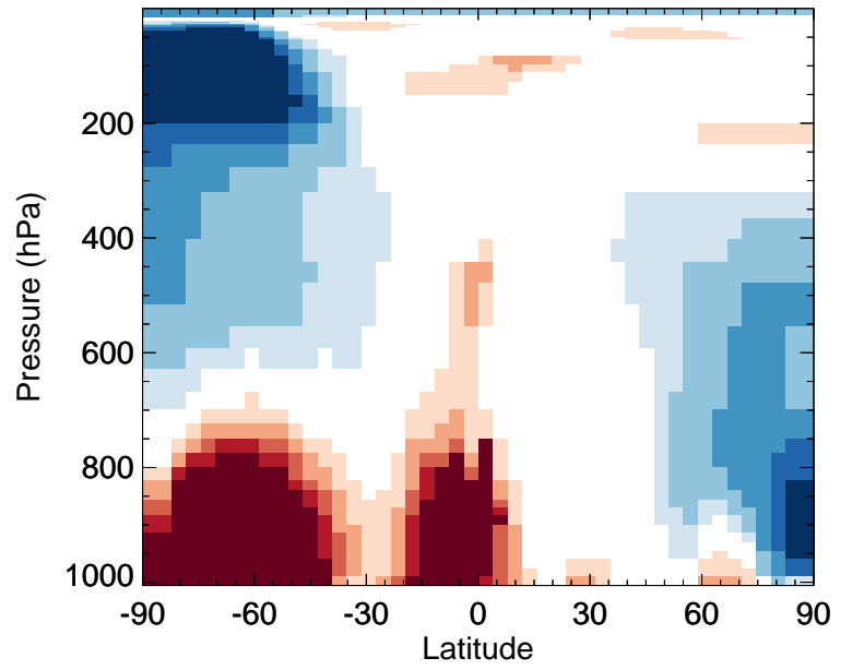
v11-02f-Run1 / v11-02e-Run1 MPN - Zonal mean % diff for Jul
