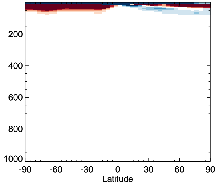
v11-02f-Run1 / v11-02e-Run0 OCS - Zonal mean % diff for Jul
