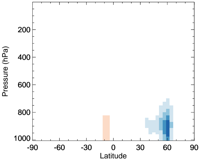
v11-02f-Run1 - v11-02e-Run1 PAN - Zonal mean abs diff for Jul
