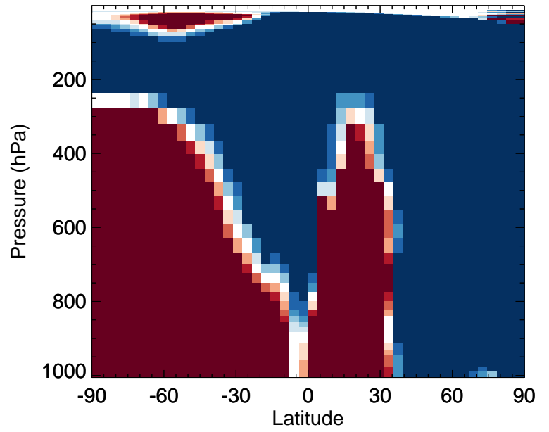
v11-02f-Run1 / v11-02e-Run1 IEPOXA - Zonal mean % diff for Jul
