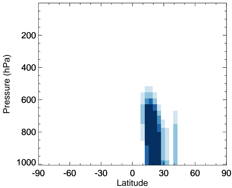
v11-02f-Run1 - v11-02e-Run0 DST3 - Zonal mean abs diff for Jul
