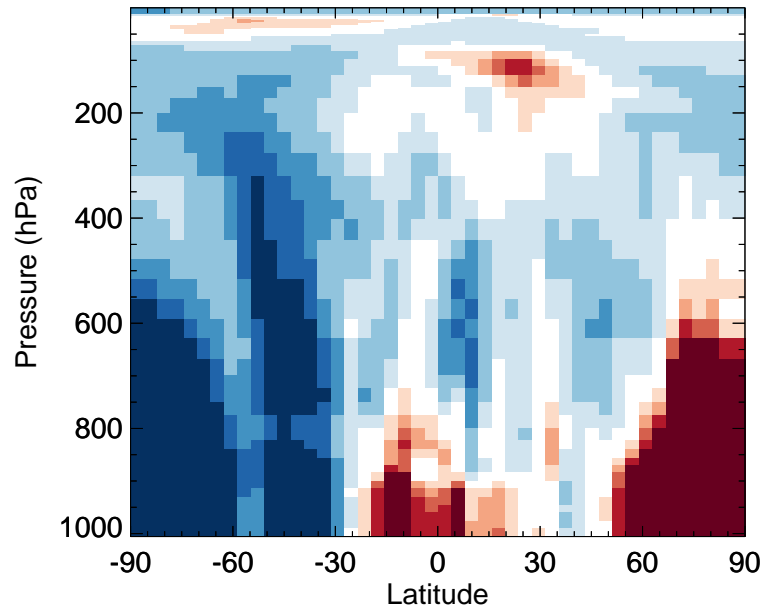
v11-02f-Run1 / v11-02e-Run0 SOAS - Zonal mean % diff for Jul
