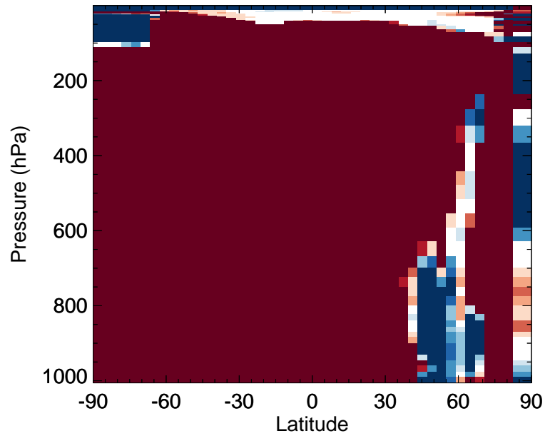
v11-02f-Run1 / v11-02e-Run0 RIPA - Zonal mean % diff for Jul
