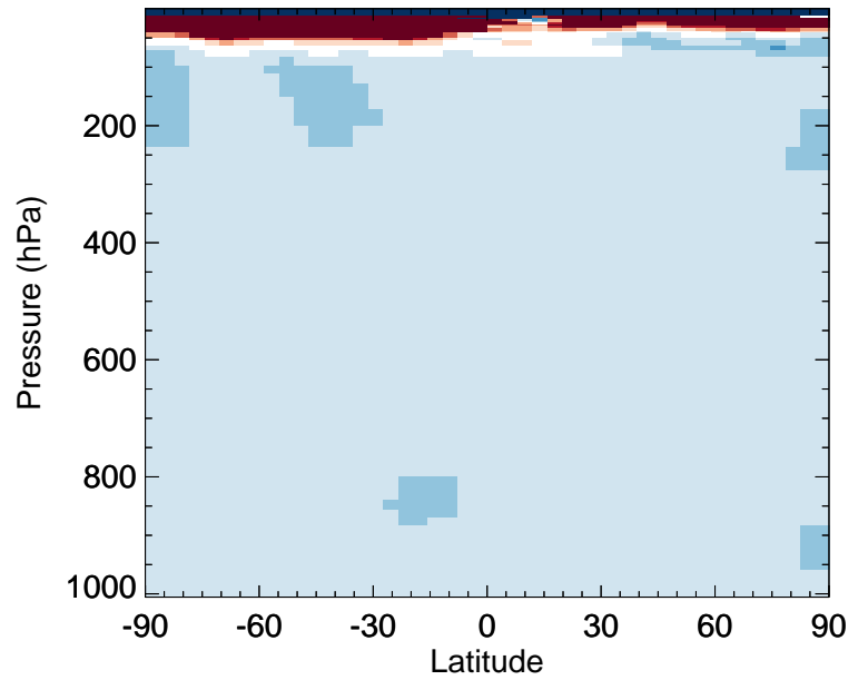
v11-02f-Run1 / v11-02e-Run0 H1211 - Zonal mean % diff for Jul
