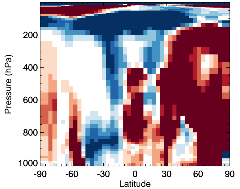
v11-02f-Run1 / v11-02e-Run0 SO 2 - Zonal mean % diff for Jul
