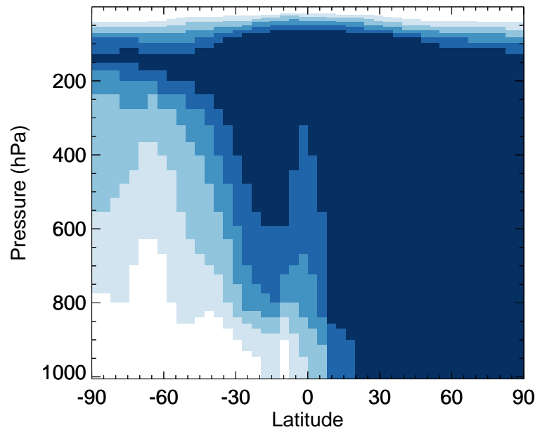
v11-02f-Run1 / v11-02e-Run1 SOAGX - Zonal mean % diff for Jul
