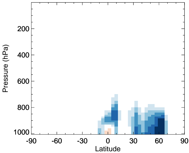
v11-02f-Run1 - v11-02e-Run0 MVK - Zonal mean abs diff for Jul
