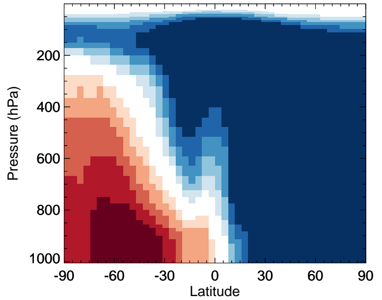
v11-02f-Run1 / v11-02e-Run1 ISN1OA - Zonal mean % diff for Jul
