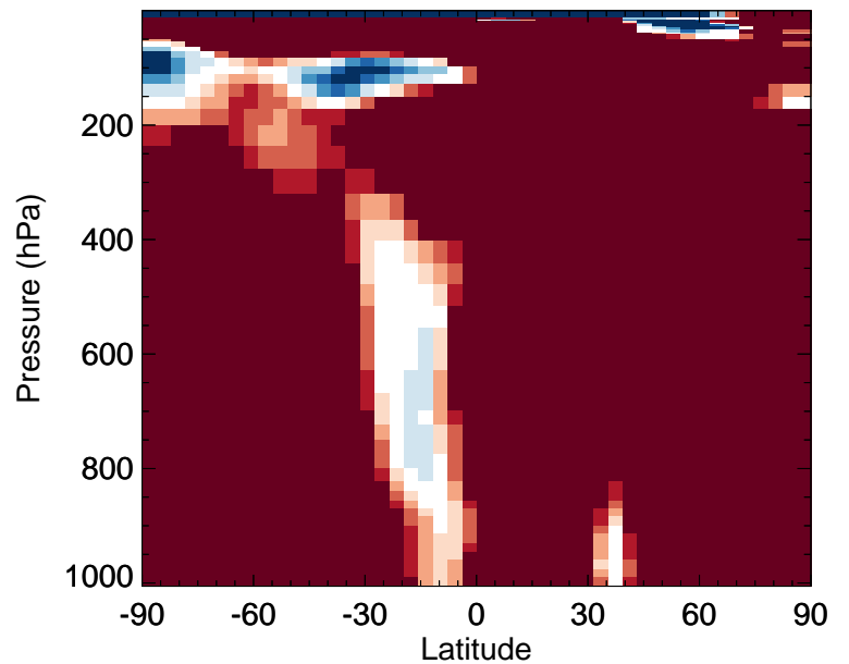
v11-02f-Run1 / v11-02e-Run0 BENZ - Zonal mean % diff for Jul
