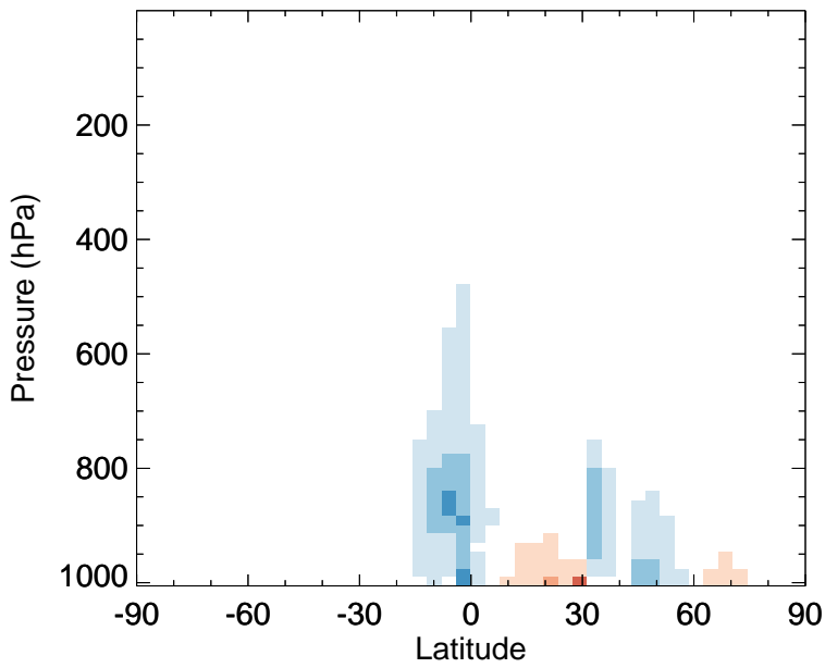
v11-02f-Run1 - v11-02e-Run1 EOH - Zonal mean abs diff for Jul
