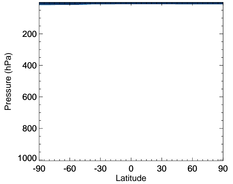
v11-02f-Run1 / v11-02e-Run1 CFC114 - Zonal mean % diff for Jul
