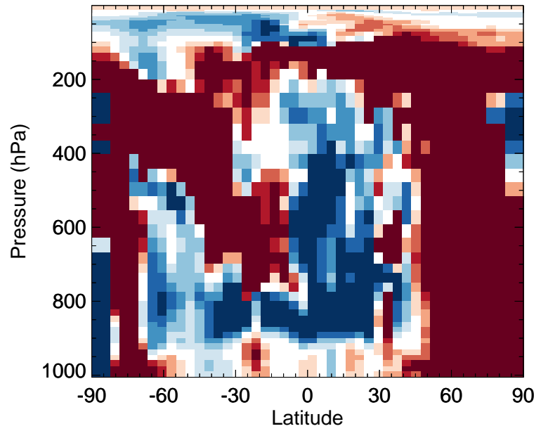
v11-02f-Run1 / v11-02e-Run0 NH3 - Zonal mean % diff for Jul
