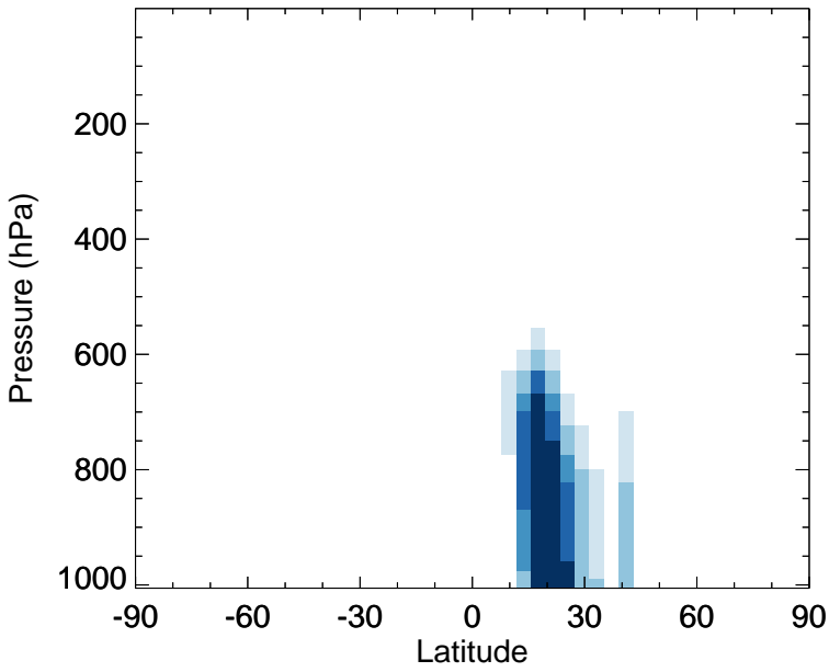
v11-02f-Run1 - v11-02e-Run0 DST4 - Zonal mean abs diff for Jul
