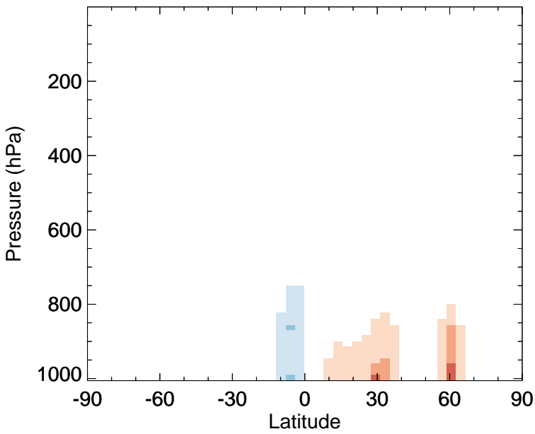
v11-02f-Run1 - v11-02e-Run1 OCPI - Zonal mean abs diff for Jul
