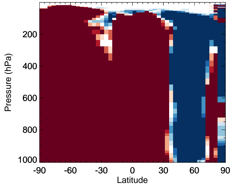
v11-02f-Run1 / v11-02e-Run1 MOBA - Zonal mean % diff for Jul
