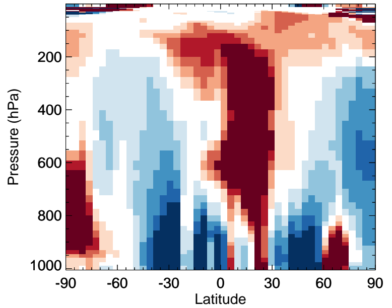
v11-02f-Run1 / v11-02e-Run1 BCPO - Zonal mean % diff for Jul
