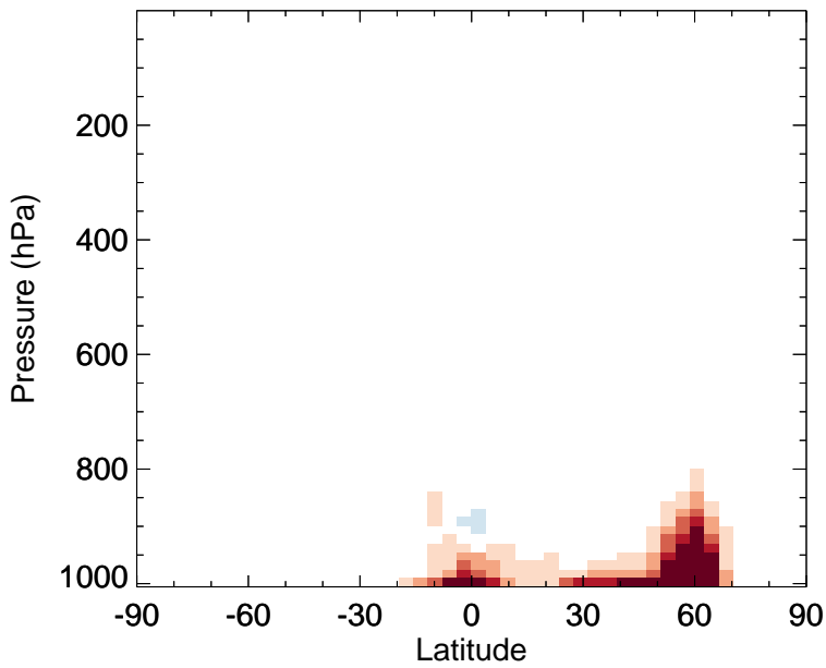
v11-02f-Run1 - v11-02e-Run0 RCHO - Zonal mean abs diff for Jul
