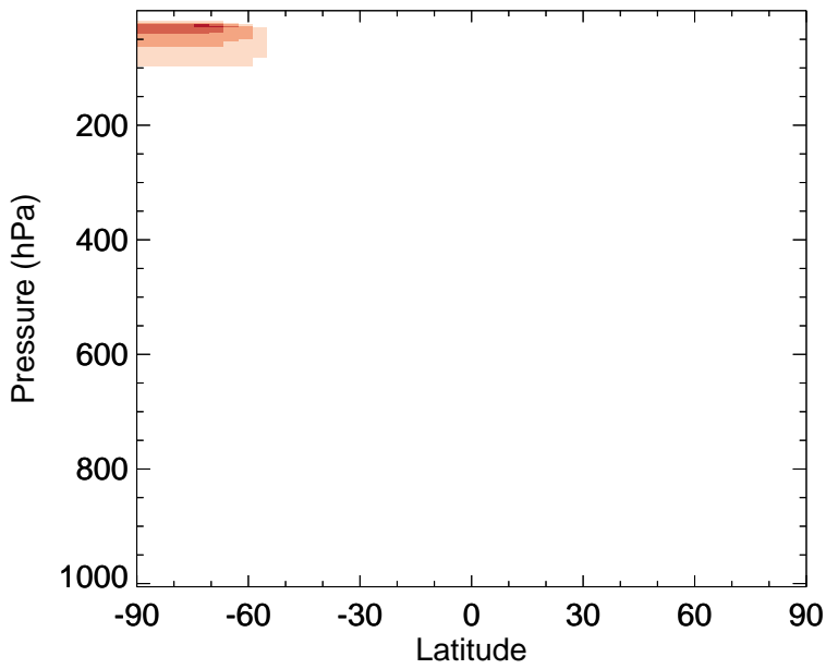
v11-02f-Run1 - v11-02e-Run1 OCIO - Zonal mean abs diff for Jul
