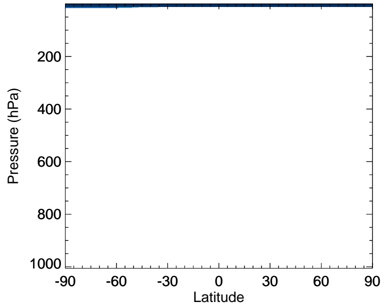
v11-02f-Run1 / v11-02e-Run1 CH4 - Zonal mean % diff for Jul
