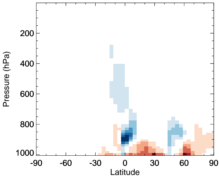
v11-02f-Run1 - v11-02e-Run0 EOH - Zonal mean abs diff for Jul
