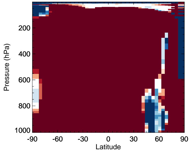
v11-02f-Run1 / v11-02e-Run0 ISOP - Zonal mean % diff for Jul
