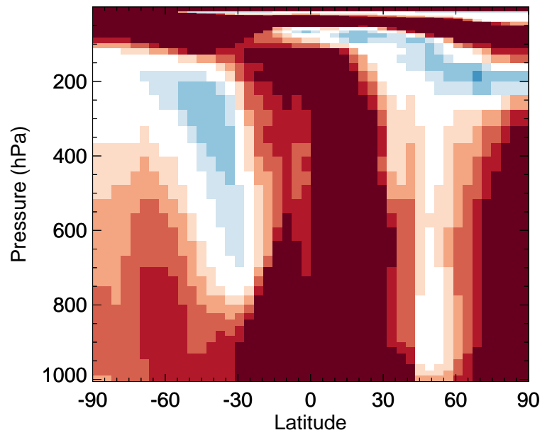
v11-02f-Run1 / v11-02e-Run1 EOH - Zonal mean % diff for Jul
