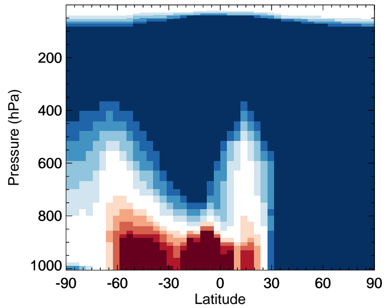
v11-02f-Run1 / v11-02e-Run1 ISOA1 - Zonal mean % diff for Jul
