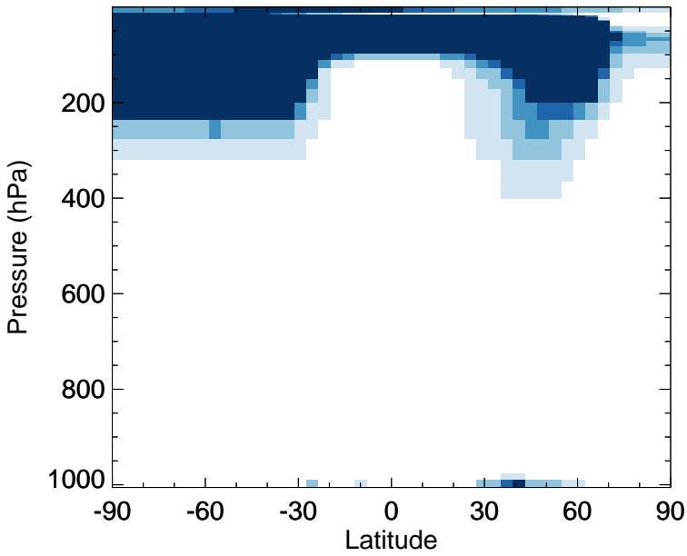
v11-02f-Run1 - v11-02e-Run1 N2O5 - Zonal mean abs diff for Jul
