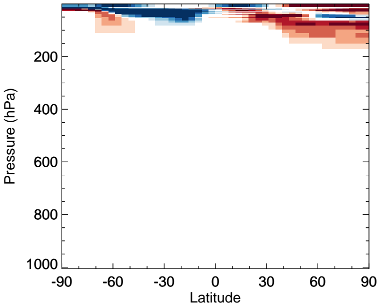
v11-02f-Run1 - v11-02e-Run0 HCl - Zonal mean abs diff for Jul
