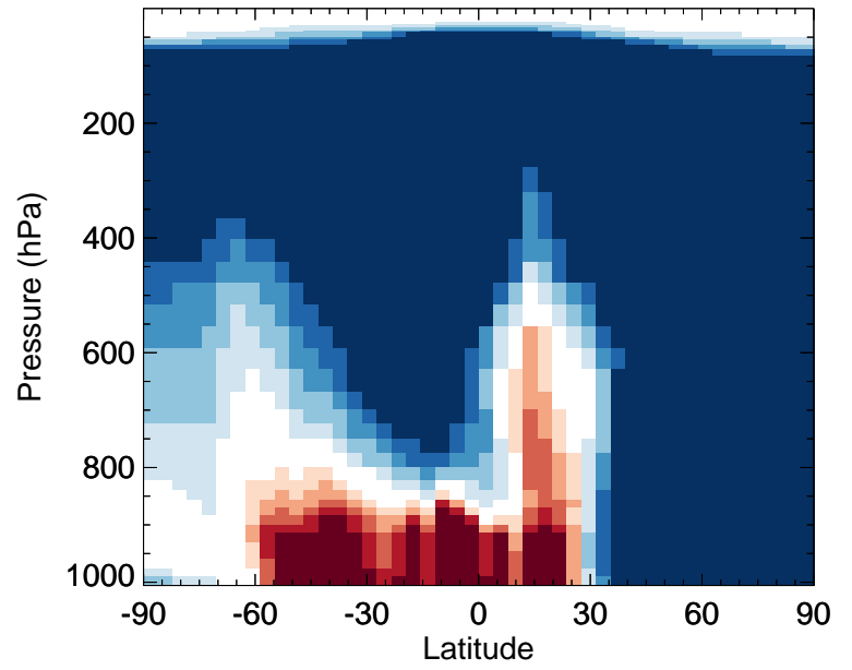
v11-02f-Run1 / v11-02e-Run1 ISOA3 - Zonal mean % diff for Jul
