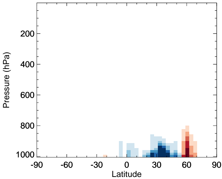
v11-02f-Run1 - v11-02e-Run0 XYLE - Zonal mean abs diff for Jul
