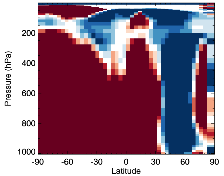
v11-02f-Run1 / v11-02e-Run1 MACR - Zonal mean % diff for Jul
