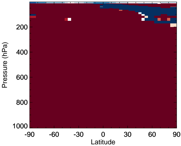
v11-02f-Run1 - v11-02e-Run0 N2O - Zonal mean abs diff for Jul
