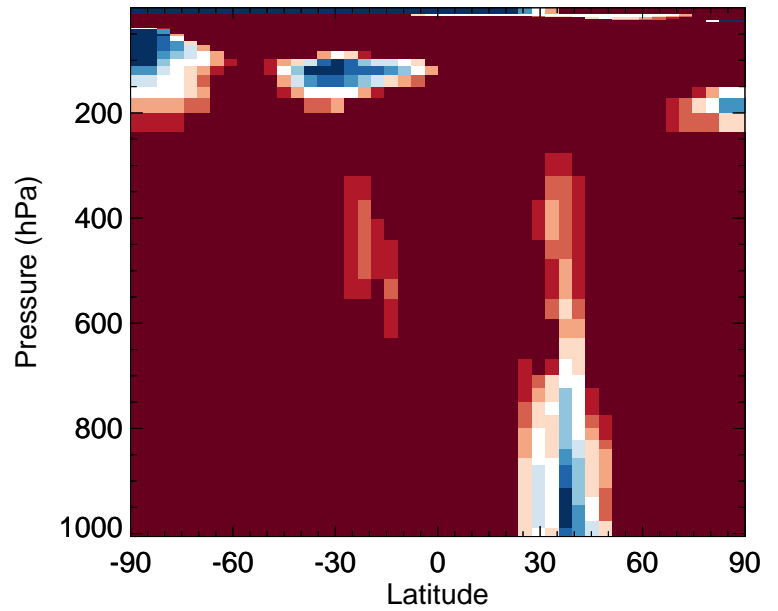
v11-02f-Run1 / v11-02e-Run0 ALK4 - Zonal mean % diff for Jul
