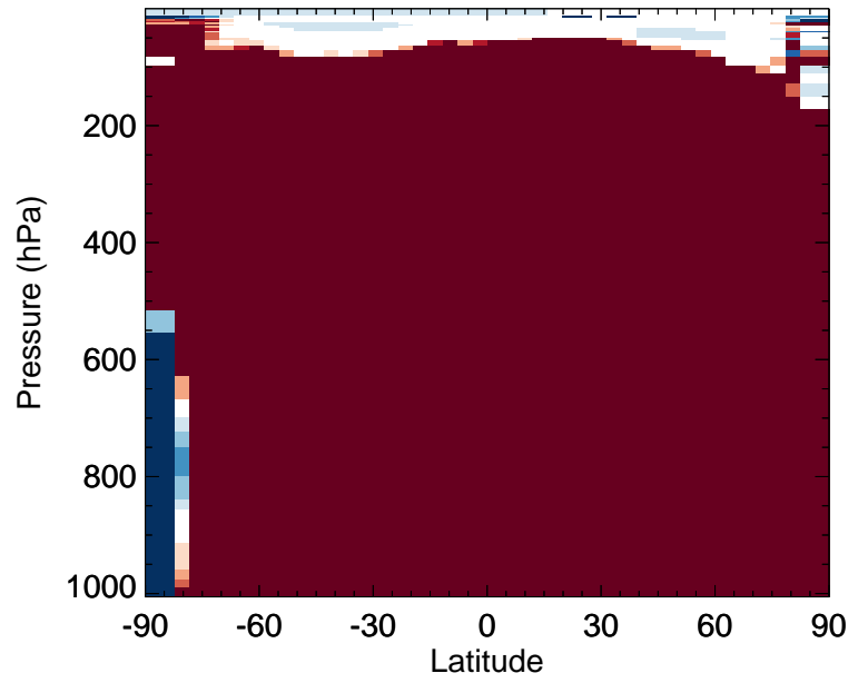
v11-02f-Run1 / v11-02e-Run1 LIMO - Zonal mean % diff for Jul
