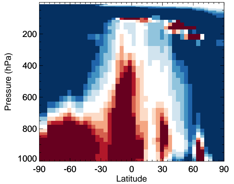
v11-02f-Run1 / v11-02e-Run1 ClNO 2 - Zonal mean % diff for Jul
