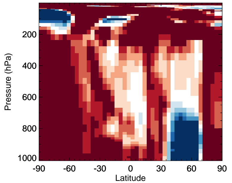
v11-02f-Run1 / v11-02e-Run0 MGLY - Zonal mean % diff for Jul
