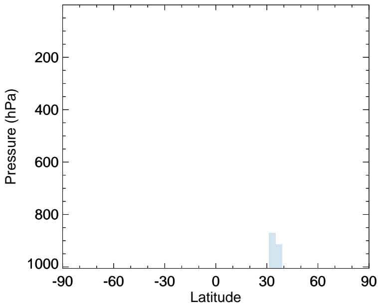
v11-02f-Run1 - v11-02e-Run1 MGLY - Zonal mean abs diff for Jul
