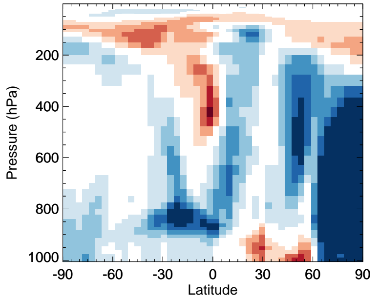
v11-02f-Run1 / v11-02e-Run0 MSA - Zonal mean % diff for Jul
