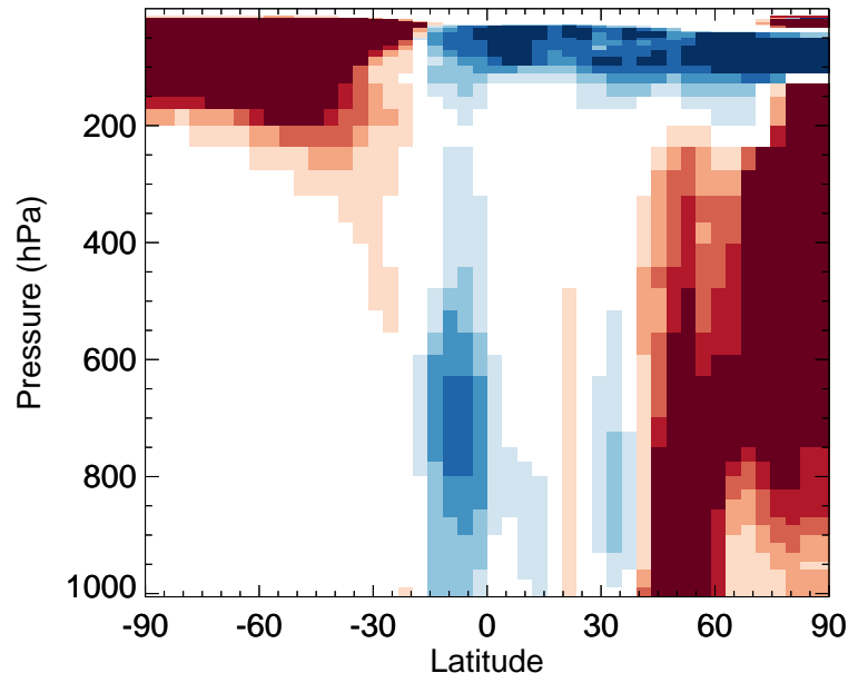
v11-02f-Run1 / v11-02e-Run1 DMS - Zonal mean % diff for Jul
