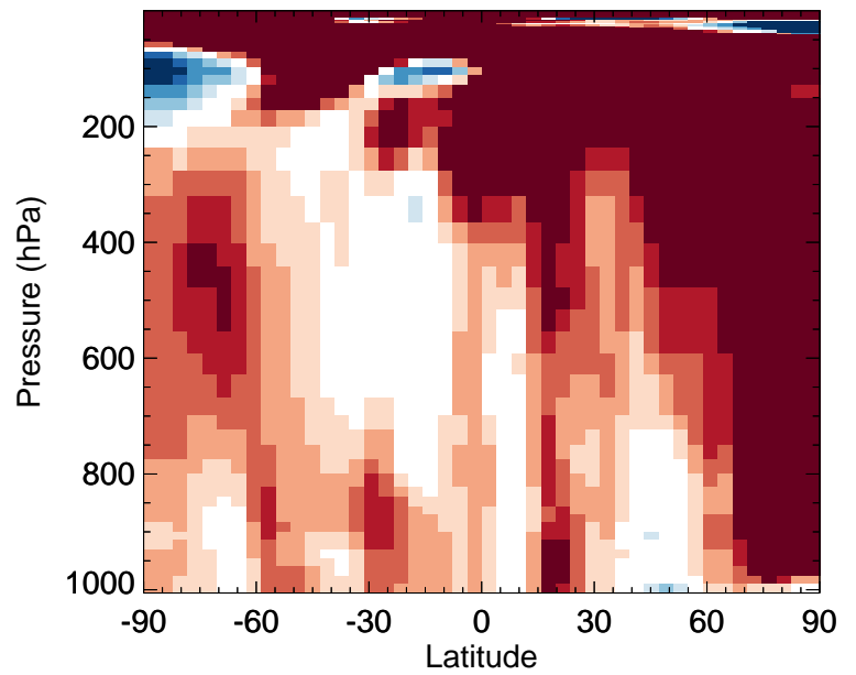
v11-02f-Run1 / v11-02e-Run0 MAP - Zonal mean % diff for Jul
