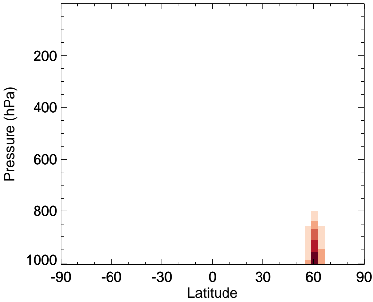
v11-02f-Run1 - v11-02e-Run0 NH3 - Zonal mean abs diff for Jul
