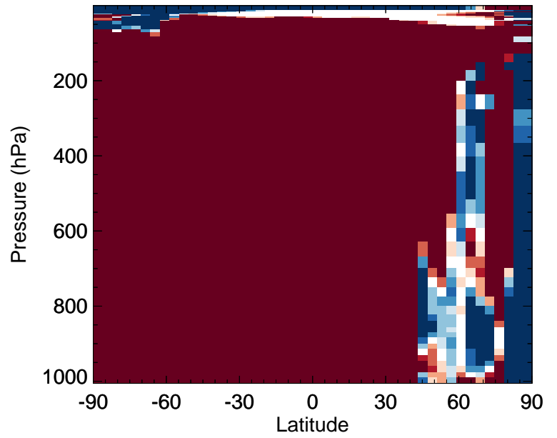
v11-02f-Run1 / v11-02e-Run0 LVOC - Zonal mean % diff for Jul
