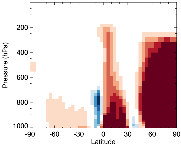
v11-02f-Run1 - v11-02e-Run0 BENZ - Zonal mean abs diff for Jul
