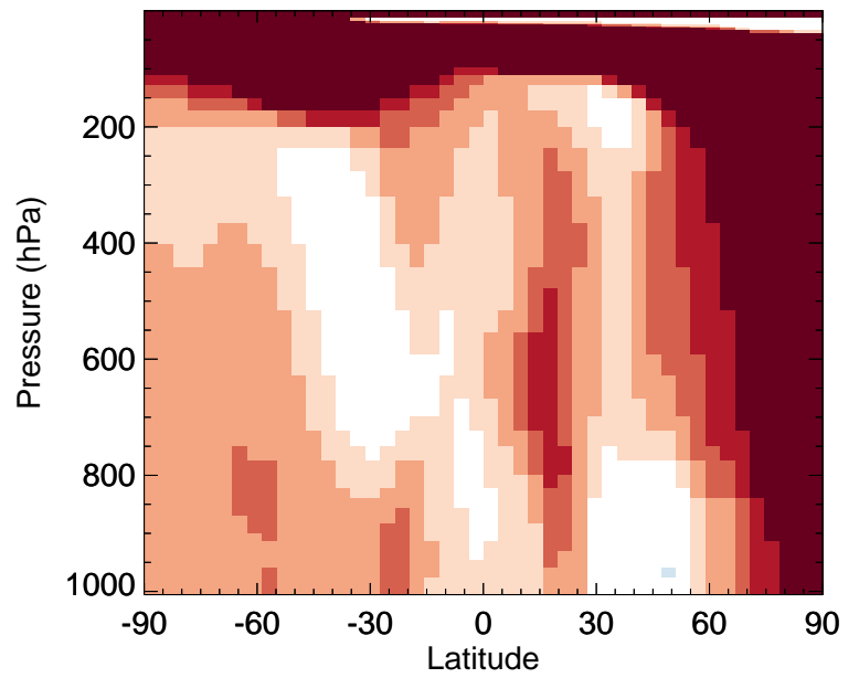
v11-02f-Run1 / v11-02e-Run1 MAP - Zonal mean % diff for Jul
