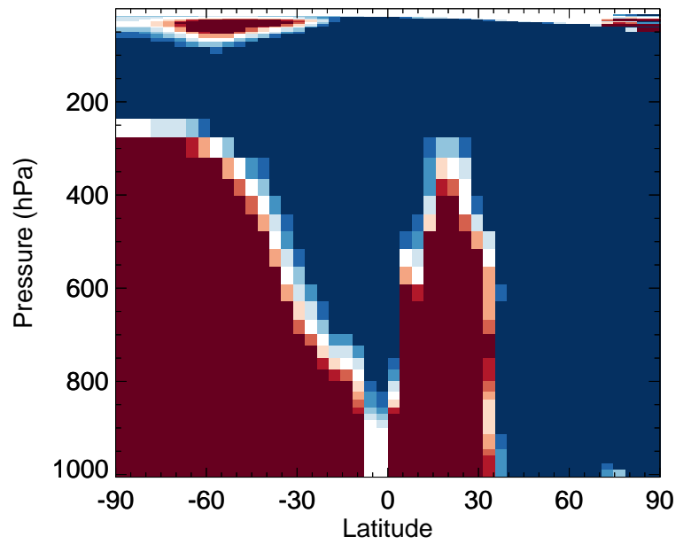
v11-02f-Run1 / v11-02e-Run1 IEPOXD - Zonal mean % diff for Jul
