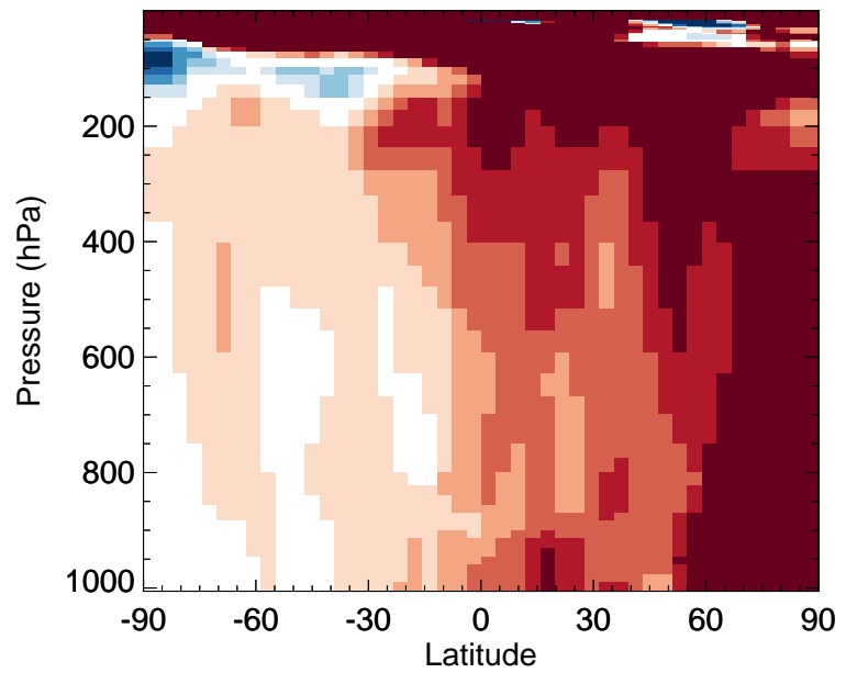
v11-02f-Run1 / v11-02e-Run0 ACET - Zonal mean % diff for Jul
