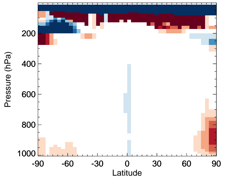
v11-02f-Run1 / v11-02e-Run1 SO 4 s - Zonal mean % diff for Jul
