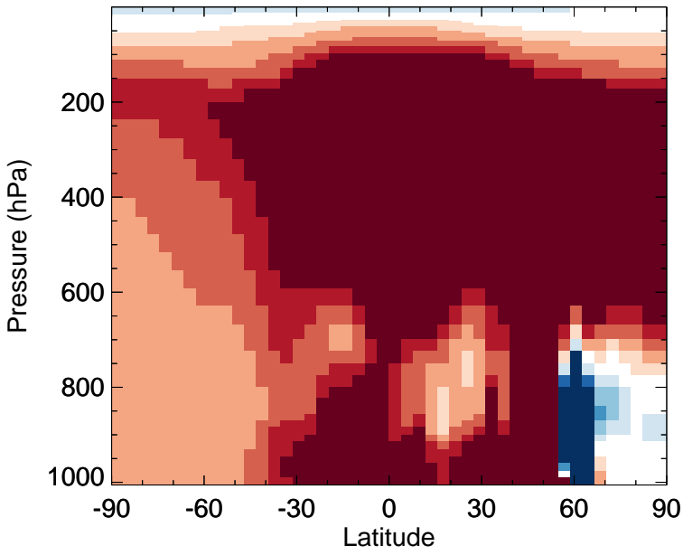
v11-02f-Run1 - v11-02e-Run1 PPN - Zonal mean abs diff for Jul
