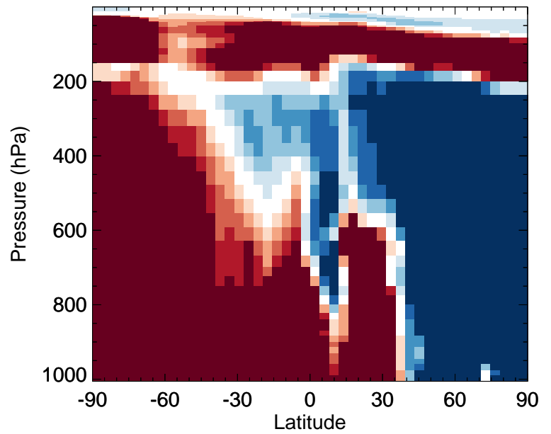
v11-02f-Run1 / v11-02e-Run0 DHDN - Zonal mean % diff for Jul
