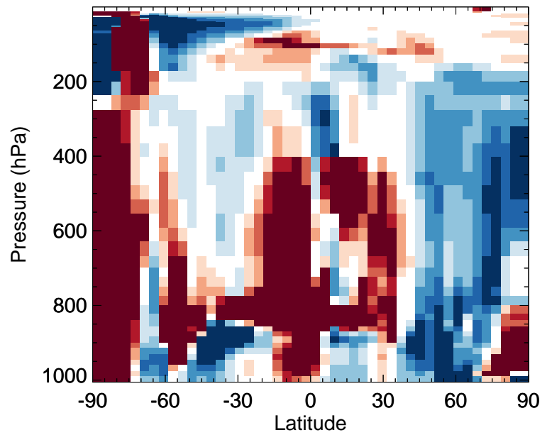
v11-02f-Run1 / v11-02e-Run0 BrNO3 - Zonal mean % diff for Jul
