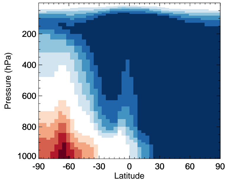
v11-02f-Run1 / v11-02e-Run1 SOAMG - Zonal mean % diff for Jul
