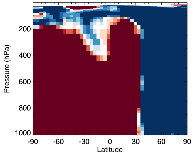
v11-02f-Run1 / v11-02e-Run1 ISN1OG - Zonal mean % diff for Jul
