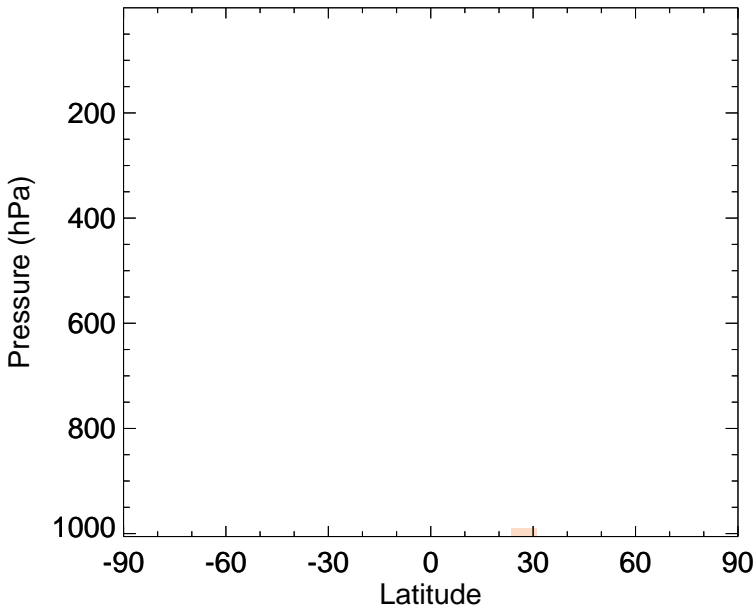
v11-02f-Run1 - v11-02e-Run0 SO 2 - Zonal mean abs diff for Jul
