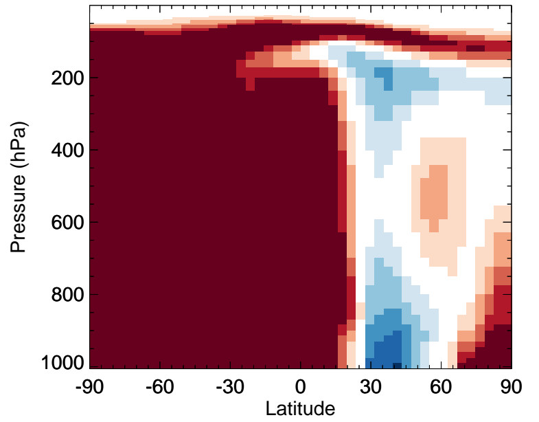
v11-02f-Run1 / v11-02e-Run1 ASOG1 - Zonal mean % diff for Jul
