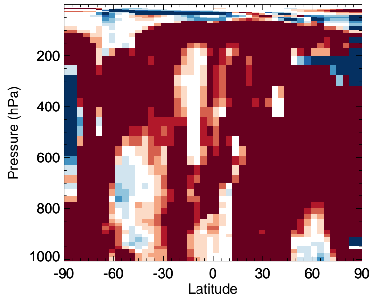
v11-02f-Run1 / v11-02e-Run0 HBr - Zonal mean % diff for Jul
