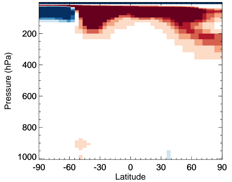
v11-02f-Run1 / v11-02e-Run1 H2O2 - Zonal mean % diff for Jul
