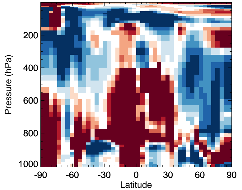
v11-02f-Run1 / v11-02e-Run0 ClNO 3 - Zonal mean % diff for Jul
