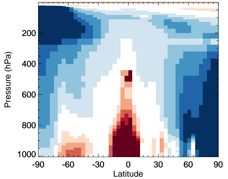
v11-02f-Run1 / v11-02e-Run1 ClNO 3 - Zonal mean % diff for Jul
