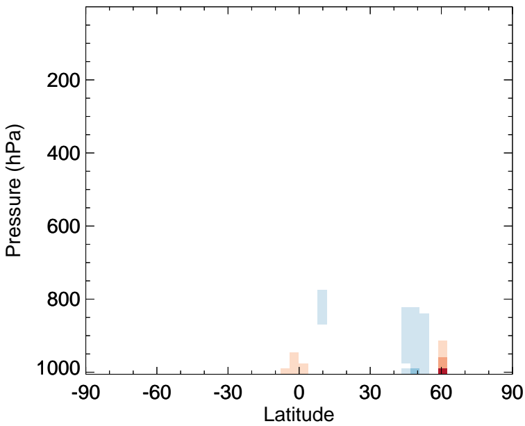
v11-02f-Run1 - v11-02e-Run0 CH 2 O - Zonal mean abs diff for Jul
