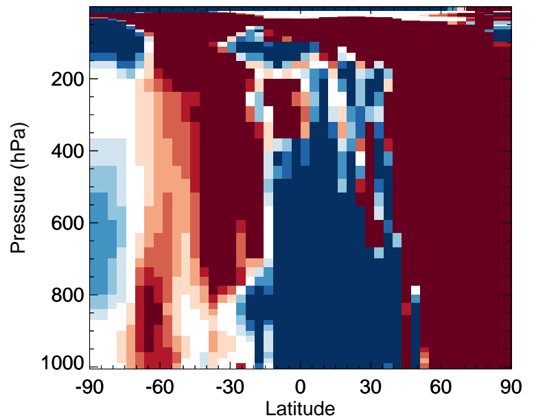
v11-02f-Run1 / v11-02e-Run0 XYLE - Zonal mean % diff for Jul
