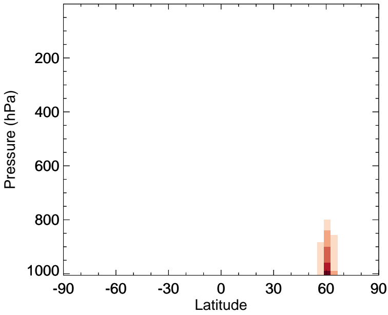
v11-02f-Run1 - v11-02e-Run1 NH3 - Zonal mean abs diff for Jul
