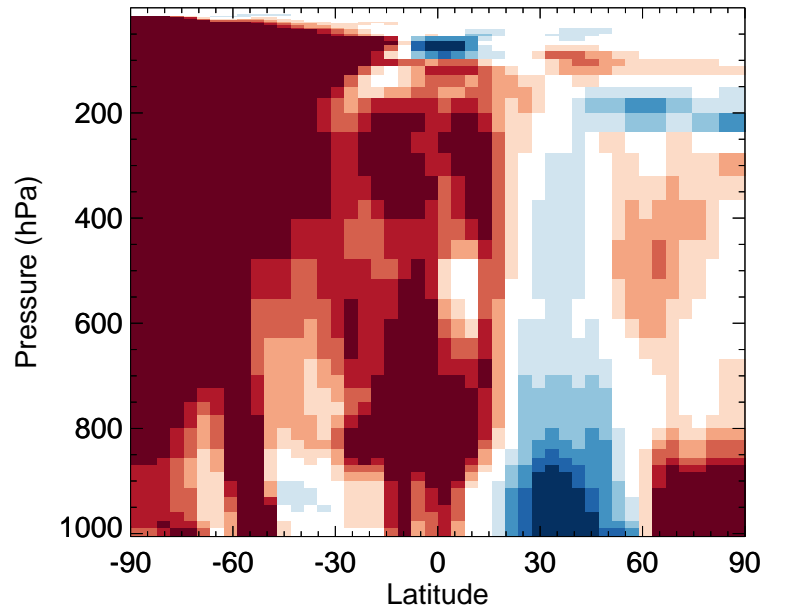
v11-02f-Run1 / v11-02e-Run0 ASOG1 - Zonal mean % diff for Jul
