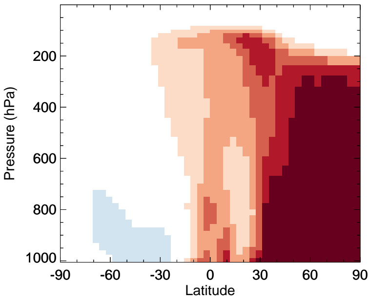
v11-02f-Run1 - v11-02e-Run1 C2H6 - Zonal mean abs diff for Jul
