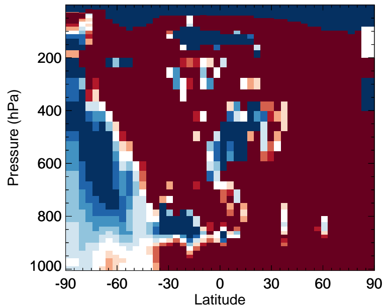
v11-02f-Run1 / v11-02e-Run0 NIT - Zonal mean % diff for Jul
