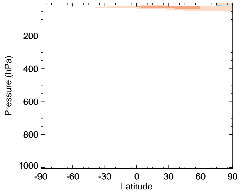
v11-02f-Run1 / v11-02e-Run1 CH2Br2 - Zonal mean % diff for Jul
