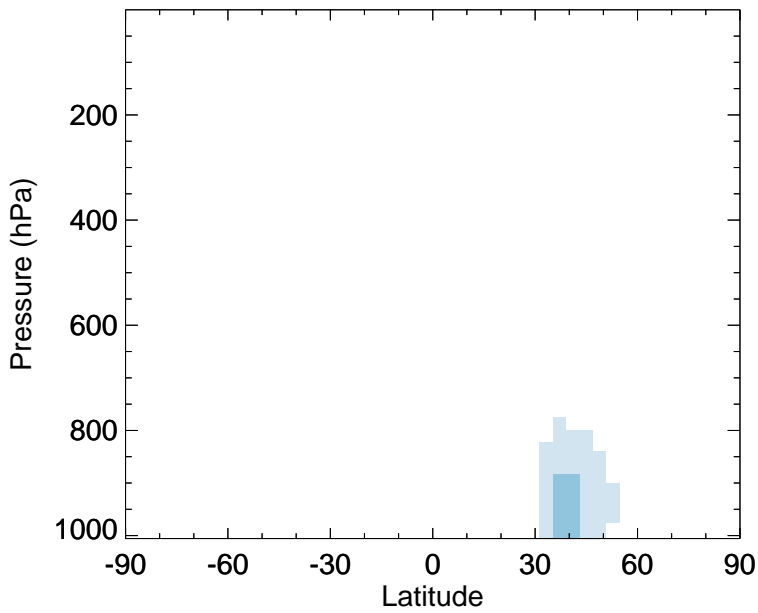
v11-02f-Run1 - v11-02e-Run0 SOAGX - Zonal mean abs diff for Jul
