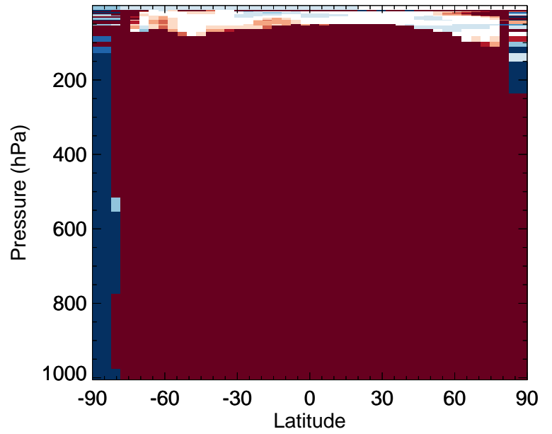
v11-02f-Run1 / v11-02e-Run0 LIMO - Zonal mean % diff for Jul
