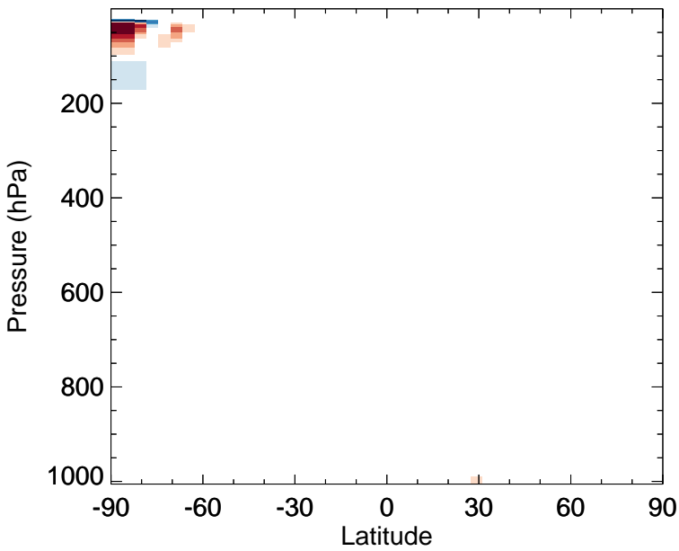
v11-02f-Run1 - v11-02e-Run0 NIT - Zonal mean abs diff for Jul
