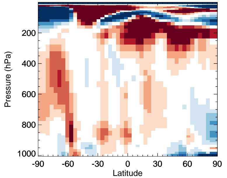
v11-02f-Run1 / v11-02e-Run0 H2O2 - Zonal mean % diff for Jul
