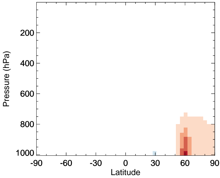
v11-02f-Run1 - v11-02e-Run1 C3H8 - Zonal mean abs diff for Jul
