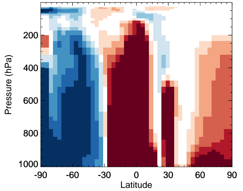
v11-02f-Run1 / v11-02e-Run1 SOAP - Zonal mean % diff for Jul
