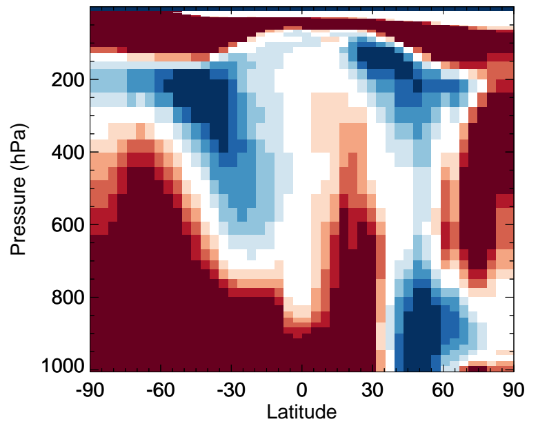
v11-02f-Run1 / v11-02e-Run1 HAC - Zonal mean % diff for Jul
