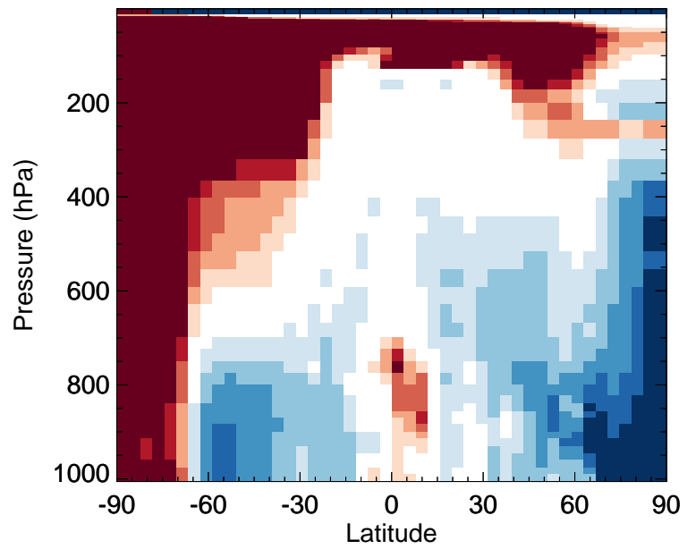
v11-02f-Run1 / v11-02e-Run1 OCIO - Zonal mean % diff for Jul
