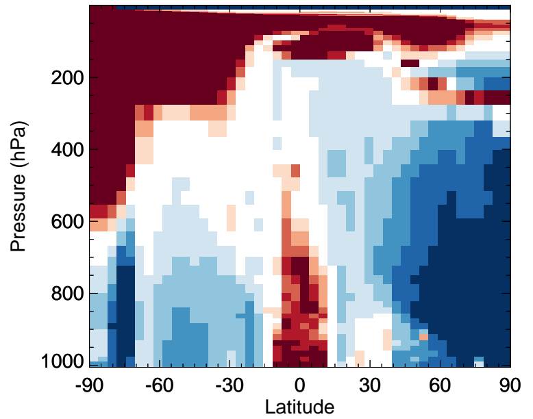
v11-02f-Run1 / v11-02e-Run1 Cl2O2 - Zonal mean % diff for Jul
