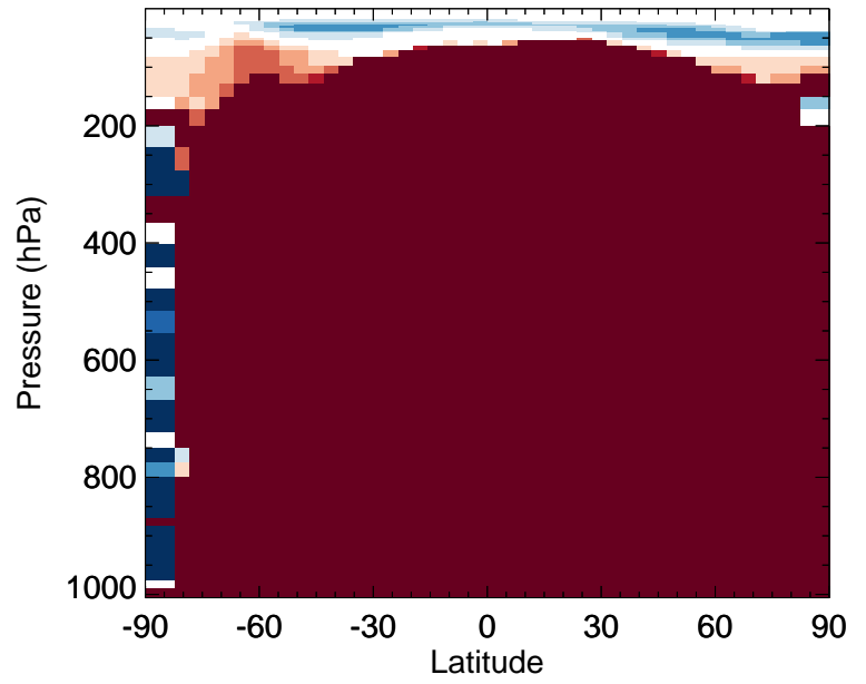
v11-02f-Run1 / v11-02e-Run1 MTPO - Zonal mean % diff for Jul
