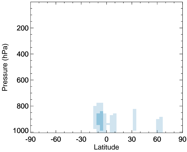
v11-02f-Run1 - v11-02e-Run1 RIPA - Zonal mean abs diff for Jul
