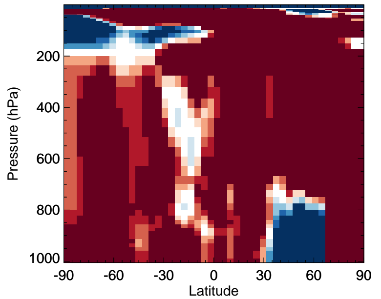
v11-02f-Run1 / v11-02e-Run0 GLYX - Zonal mean % diff for Jul
