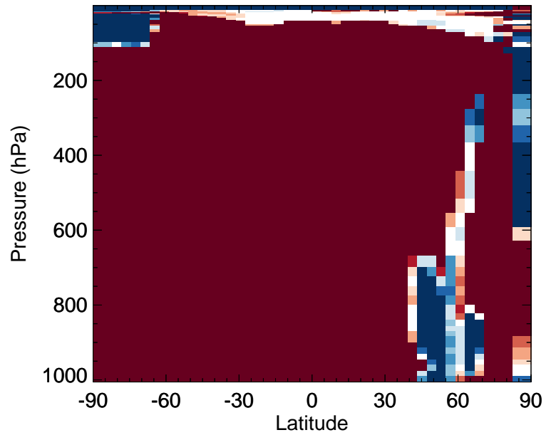
v11-02f-Run1 / v11-02e-Run0 RIPB - Zonal mean % diff for Jul
