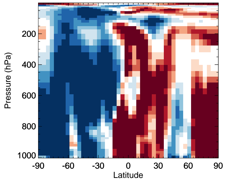
v11-02f-Run1 / v11-02e-Run0 ISOA2 - Zonal mean % diff for Jul
