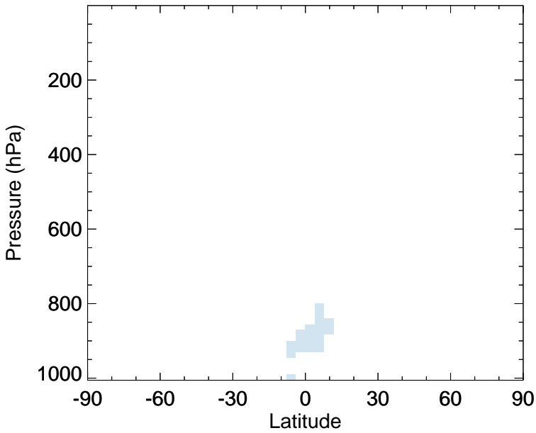
v11-02f-Run1 - v11-02e-Run0 RIPA - Zonal mean abs diff for Jul
