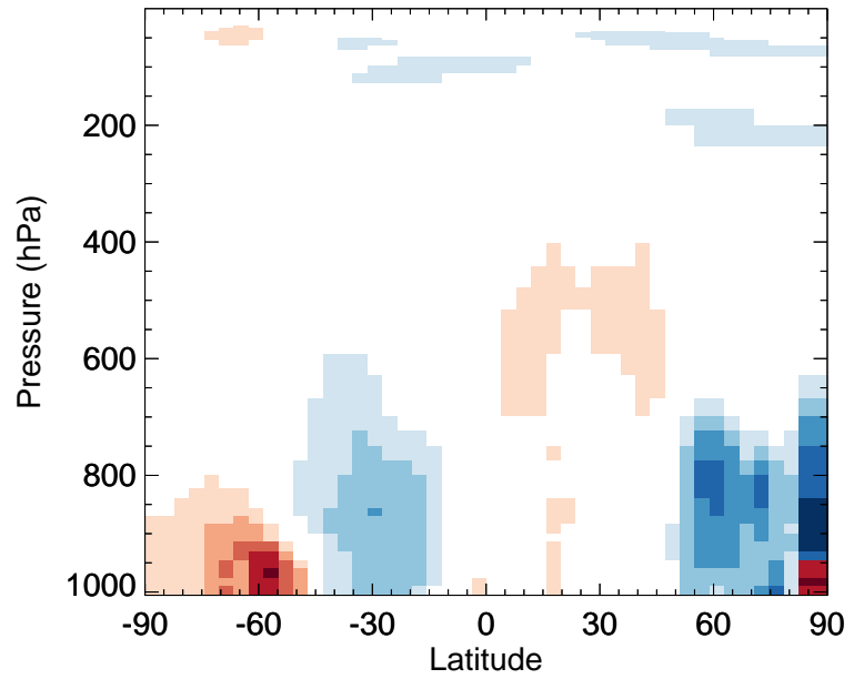
v11-02f-Run1 / v11-02e-Run1 SO 2 - Zonal mean % diff for Jul
