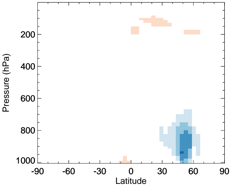
v11-02f-Run1 - v11-02e-Run0 PAN - Zonal mean abs diff for Jul
