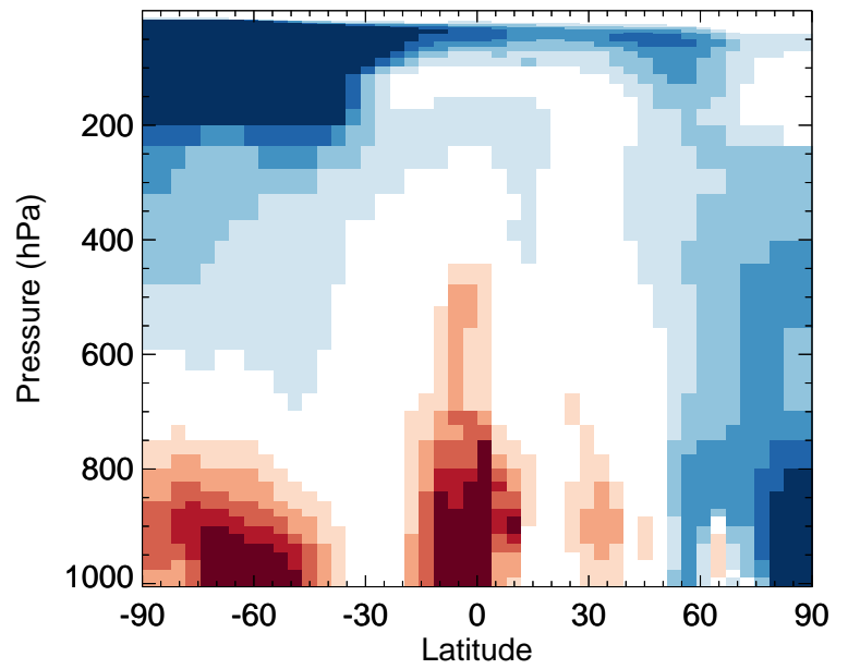
v11-02f-Run1 / v11-02e-Run1 BrNO2 - Zonal mean % diff for Jul
