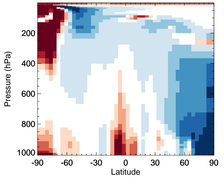
v11-02f-Run1 / v11-02e-Run1 CIOO - Zonal mean % diff for Jul
