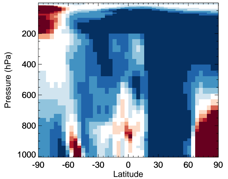
v11-02f-Run1 / v11-02e-Run0 ASOG2 - Zonal mean % diff for Jul
