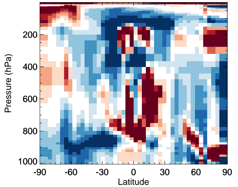
v11-02f-Run1 / v11-02e-Run0 BrCl - Zonal mean % diff for Jul
