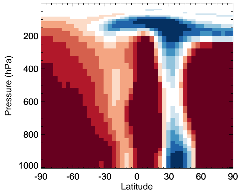
v11-02f-Run1 / v11-02e-Run1 ASOAN - Zonal mean % diff for Jul
