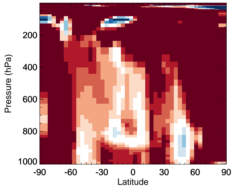
v11-02f-Run1 / v11-02e-Run0 ACTA - Zonal mean % diff for Jul
