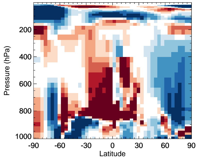
v11-02f-Run1 / v11-02e-Run0 HOBr - Zonal mean % diff for Jul
