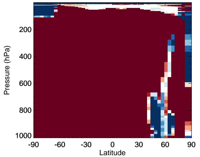
v11-02f-Run1 / v11-02e-Run0 RIPD - Zonal mean % diff for Jul
