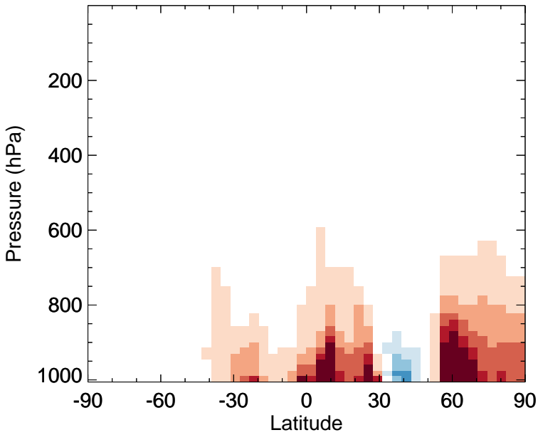
v11-02f-Run1 - v11-02e-Run0 ALK4 - Zonal mean abs diff for Jul
