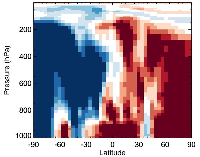
v11-02f-Run1 / v11-02e-Run0 OCPI - Zonal mean % diff for Jul
