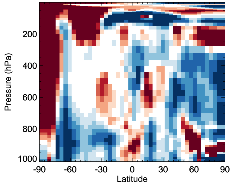
v11-02f-Run1 / v11-02e-Run0 ClO - Zonal mean % diff for Jul
