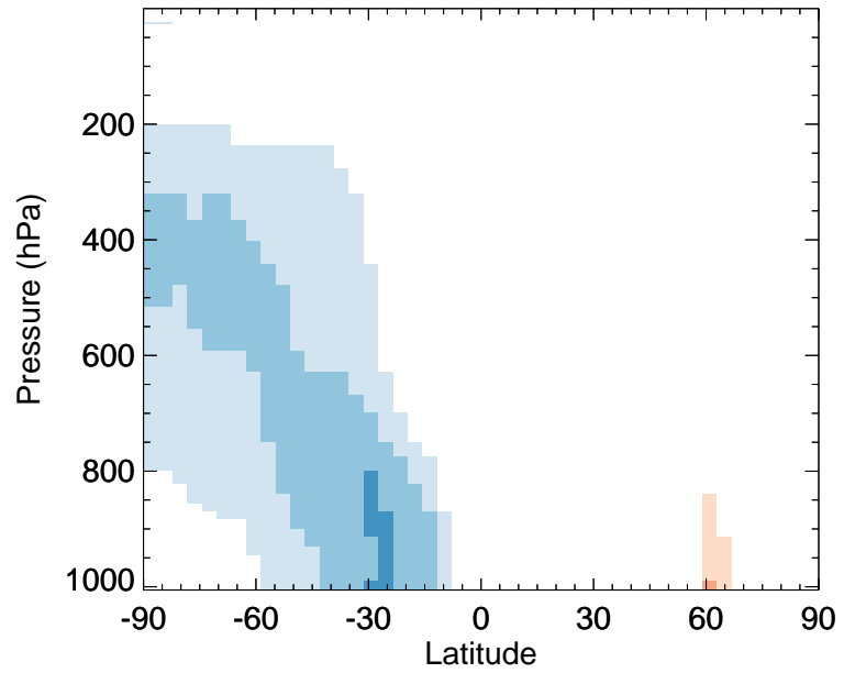
v11-02f-Run1 / v11-02e-Run1 SO4 - Zonal mean % diff for Jul
