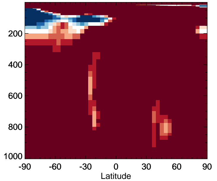
v11-02f-Run1 / v11-02e-Run0 MEK - Zonal mean % diff for Jul
