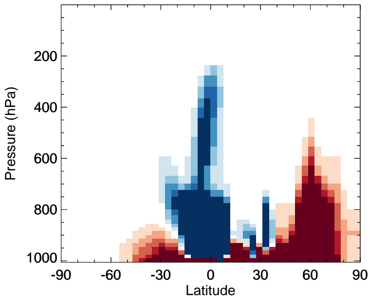
v11-02f-Run1 - v11-02e-Run1 PRPE - Zonal mean abs diff for Jul
