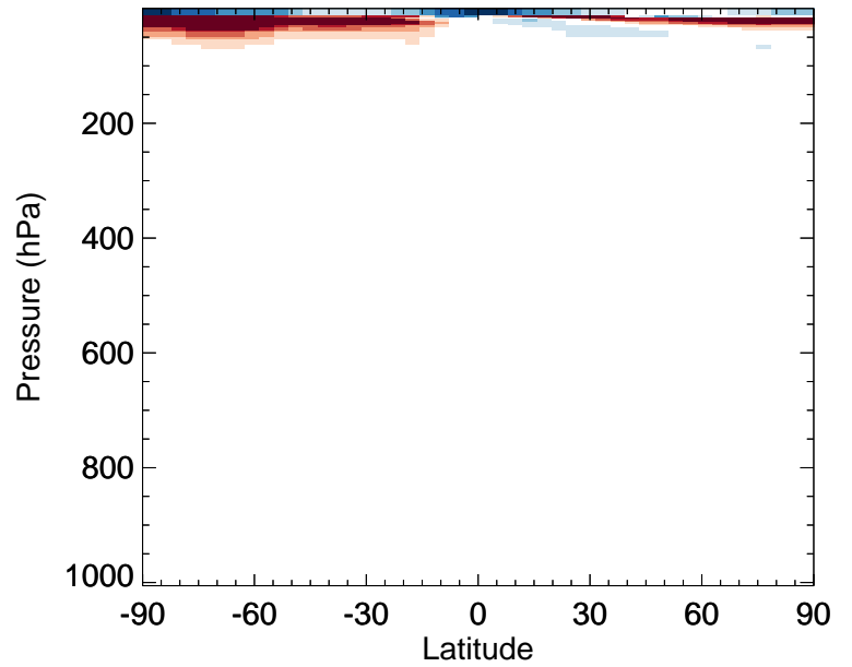
v11-02f-Run1 / v11-02e-Run0 N2O - Zonal mean % diff for Jul
