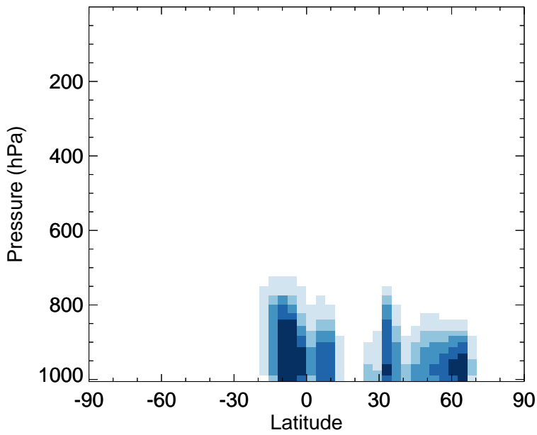
v11-02f-Run1 - v11-02e-Run1 MACR - Zonal mean abs diff for Jul
