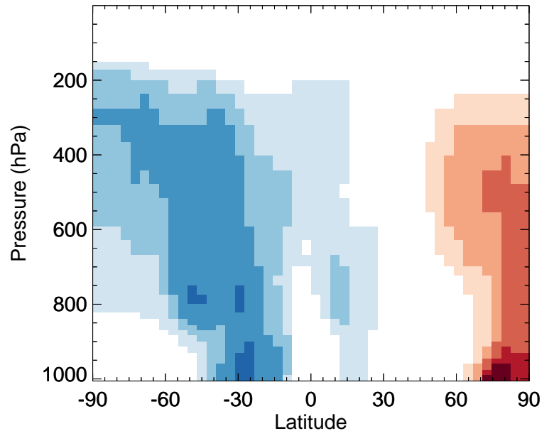
v11-02f-Run1 / v11-02e-Run1 NH4 - Zonal mean % diff for Jul
