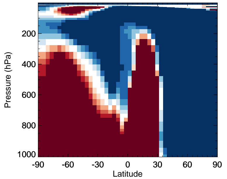
v11-02f-Run1 / v11-02e-Run1 GLYC - Zonal mean % diff for Jul
