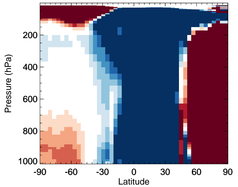
v11-02f-Run1 / v11-02e-Run1 XYLE - Zonal mean % diff for Jul
