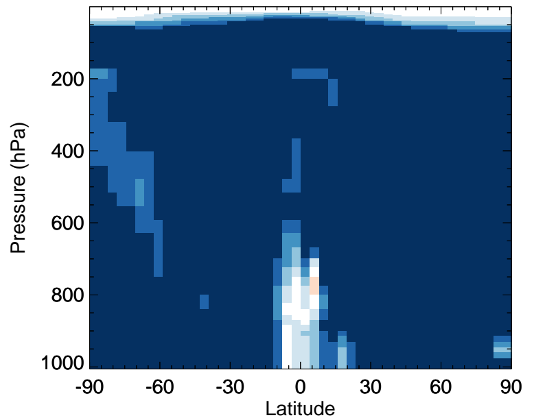
v11-02f-Run1 / v11-02e-Run0 SOAME - Zonal mean % diff for Jul
