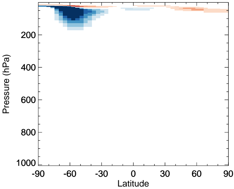
v11-02f-Run1 - v11-02e-Run1 ClNO 3 - Zonal mean abs diff for Jul
