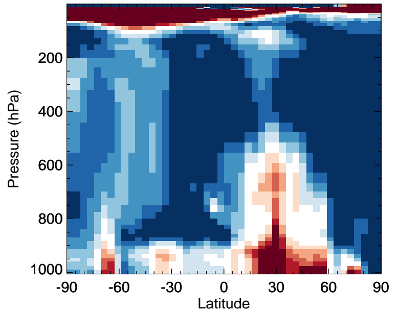
v11-02f-Run1 / v11-02e-Run0 SALA - Zonal mean % diff for Jul
