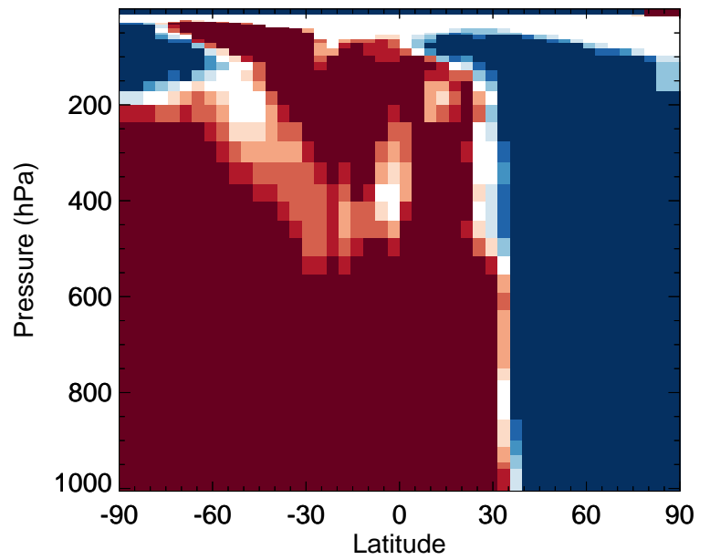
v11-02f-Run1 / v11-02e-Run1 NPMN - Zonal mean % diff for Jul
