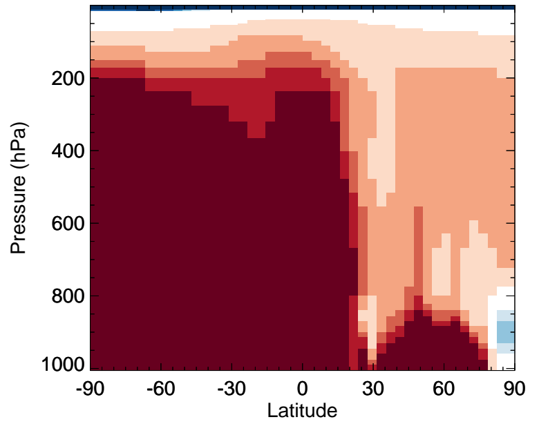
v11-02f-Run1 / v11-02e-Run1 PPN - Zonal mean % diff for Jul
