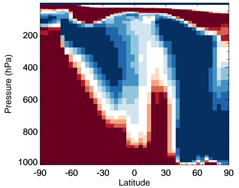
v11-02f-Run1 / v11-02e-Run1 HCOOH - Zonal mean % diff for Jul
