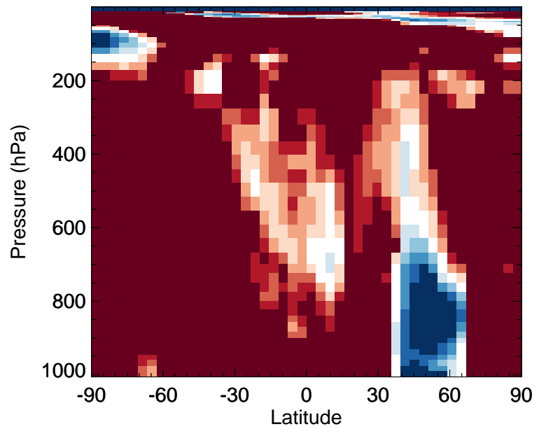
v11-02f-Run1 / v11-02e-Run0 HAC - Zonal mean % diff for Jul
