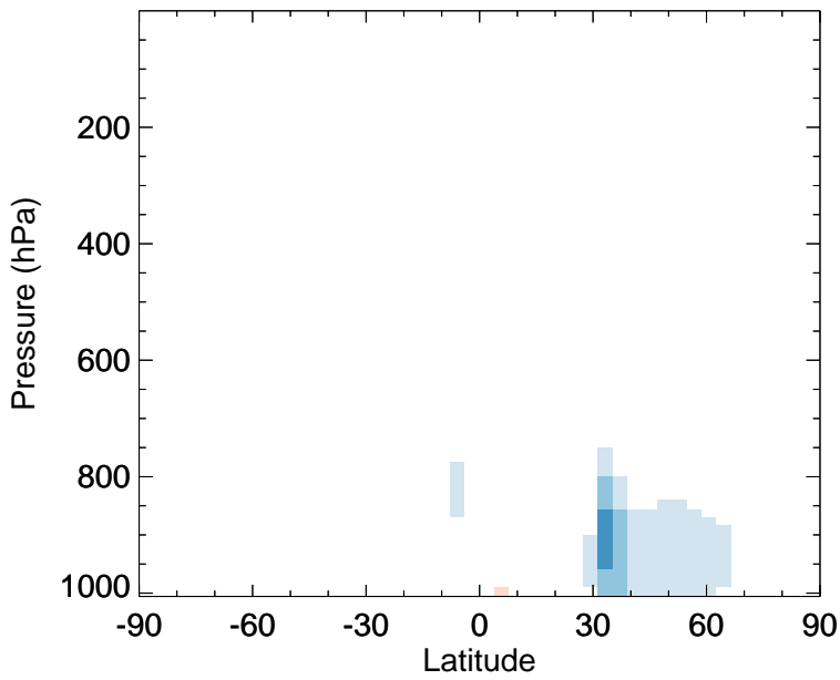
v11-02f-Run1 - v11-02e-Run1 HAC - Zonal mean abs diff for Jul
