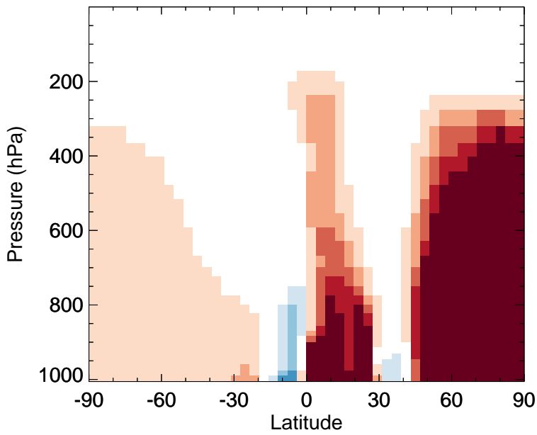
v11-02f-Run1 - v11-02e-Run1 BENZ - Zonal mean abs diff for Jul
