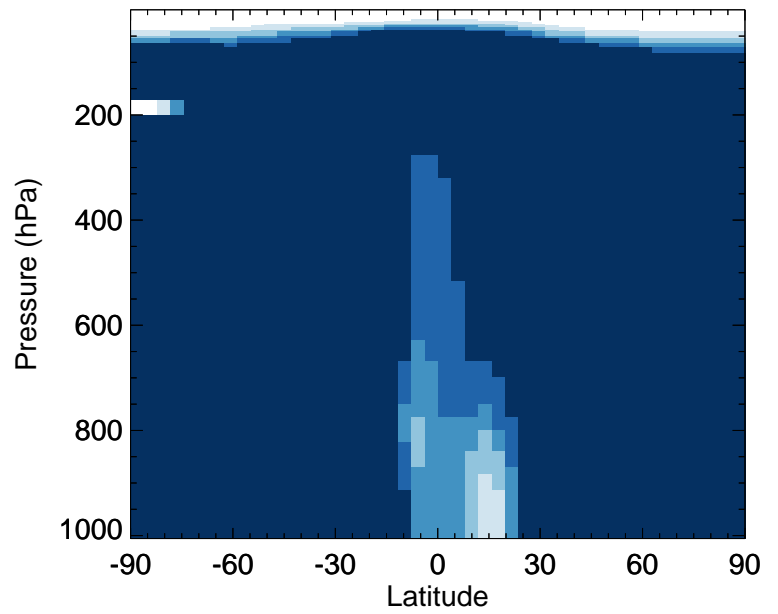
v11-02f-Run1 / v11-02e-Run1 SOAME - Zonal mean % diff for Jul
