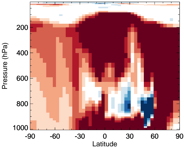
v11-02f-Run1 - v11-02e-Run0 PPN - Zonal mean abs diff for Jul
