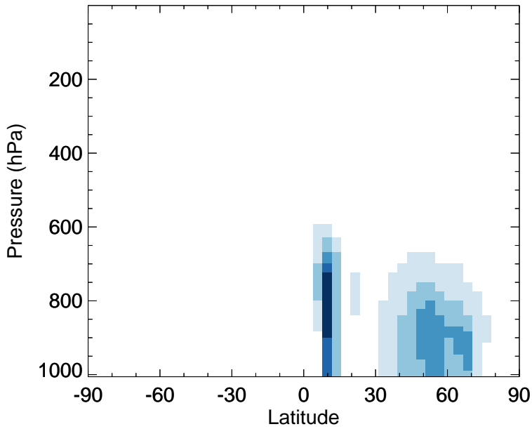
v11-02f-Run1 - v11-02e-Run0 SOAIE - Zonal mean abs diff for Jul
