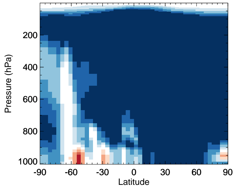
v11-02f-Run1 / v11-02e-Run0 SOAMG - Zonal mean % diff for Jul
