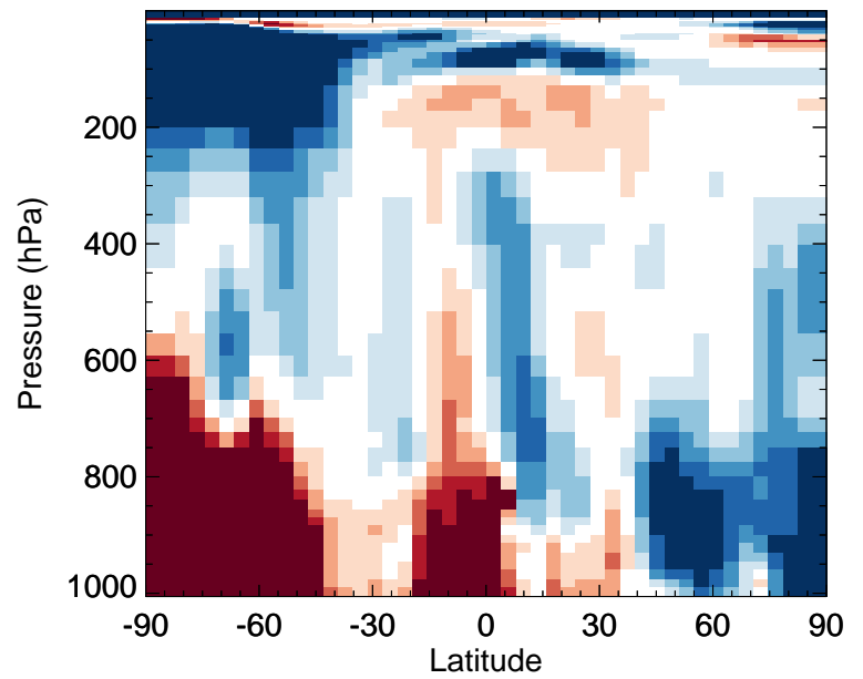
v11-02f-Run1 / v11-02e-Run0 HNO 4 - Zonal mean % diff for Jul
