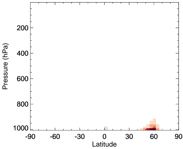
v11-02f-Run1 - v11-02e-Run1 MTPA - Zonal mean abs diff for Jul
