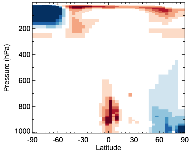
v11-02f-Run1 / v11-02e-Run1 HOBr - Zonal mean % diff for Jul
