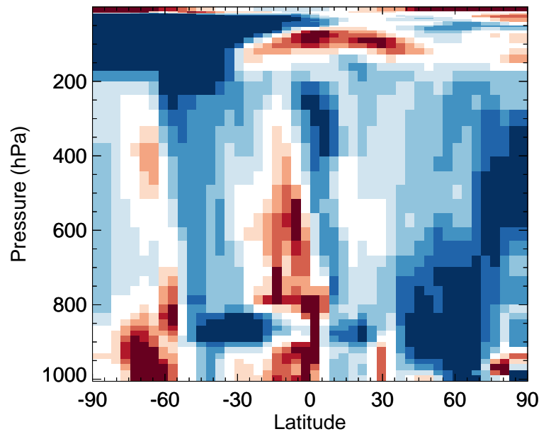
v11-02f-Run1 / v11-02e-Run0 BrNO2 - Zonal mean % diff for Jul
