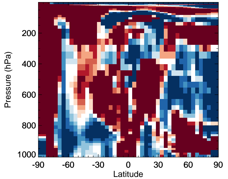
v11-02f-Run1 / v11-02e-Run0 Cl2O2 - Zonal mean % diff for Jul
