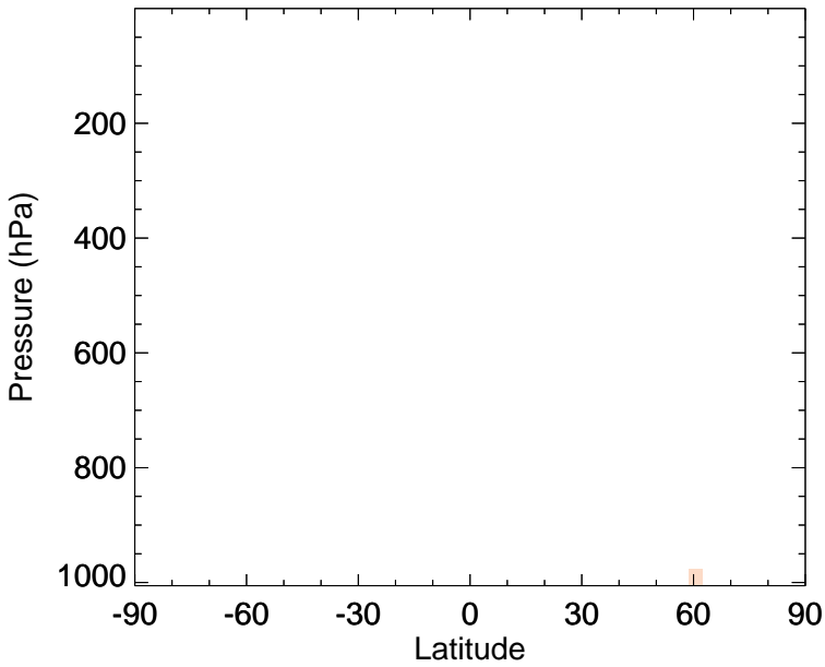
v11-02f-Run1 - v11-02e-Run0 BCPO - Zonal mean abs diff for Jul
