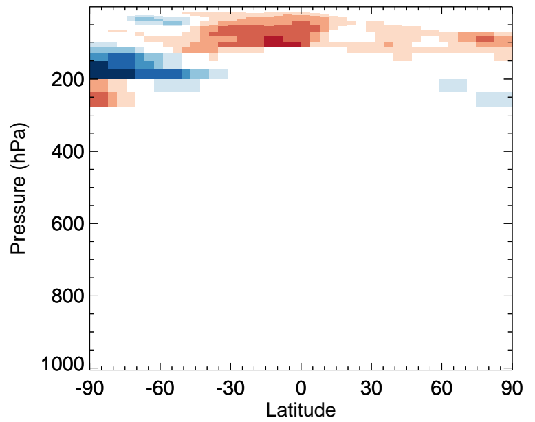
v11-02f-Run1 / v11-02e-Run1 SALC - Zonal mean % diff for Jul
