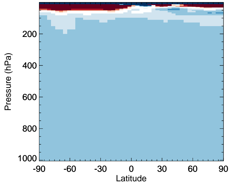
v11-02f-Run1 / v11-02e-Run0 CCI4 - Zonal mean % diff for Jul
