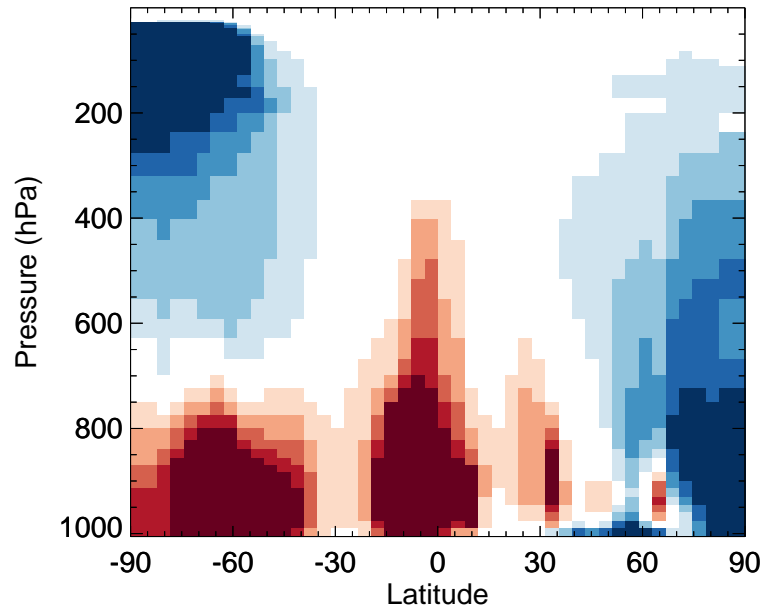
v11-02f-Run1 / v11-02e-Run1 NO3 - Zonal mean % diff for Jul
