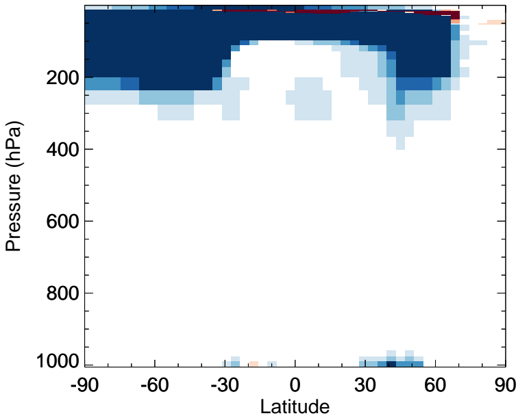
v11-02f-Run1 - v11-02e-Run0 N2O5 - Zonal mean abs diff for Jul
