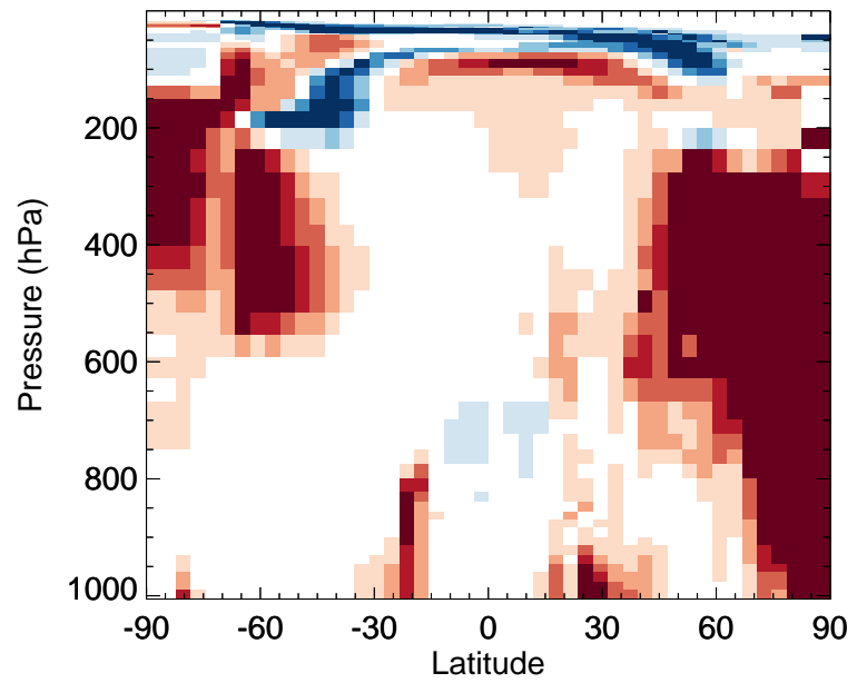
v11-02f-Run1 / v11-02e-Run1 HBr - Zonal mean % diff for Jul
