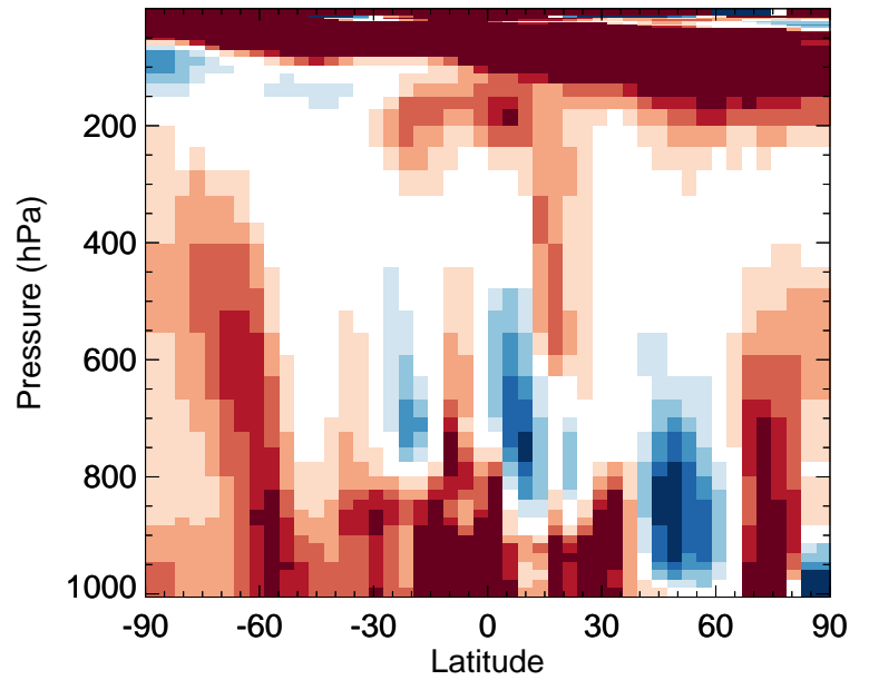
v11-02f-Run1 / v11-02e-Run0 PAN - Zonal mean % diff for Jul
