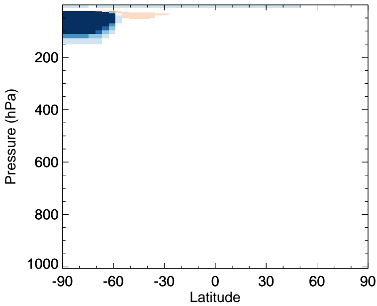
v11-02f-Run1 - v11-02e-Run1 HOCl - Zonal mean abs diff for Jul
