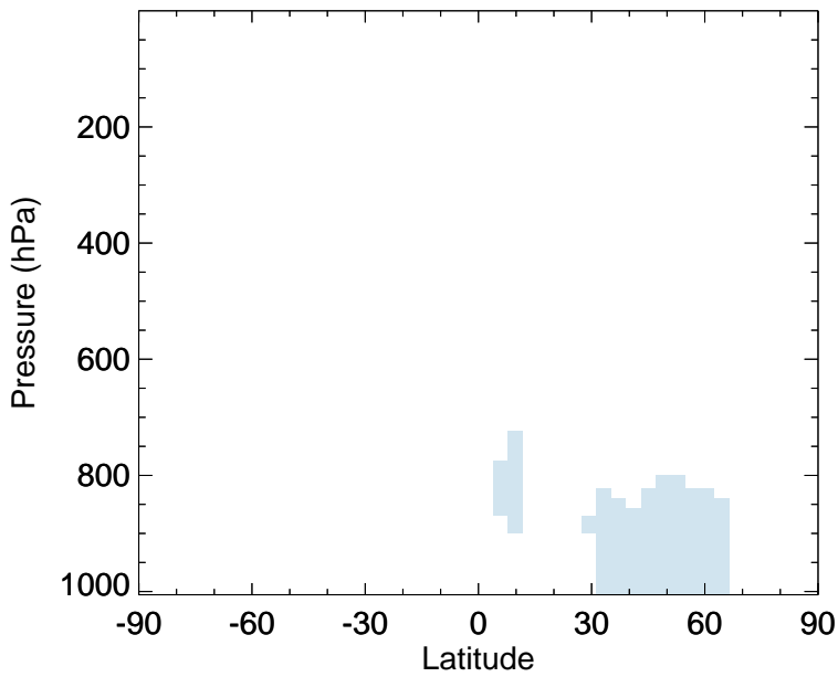
v11-02f-Run1 - v11-02e-Run0 HAC - Zonal mean abs diff for Jul
