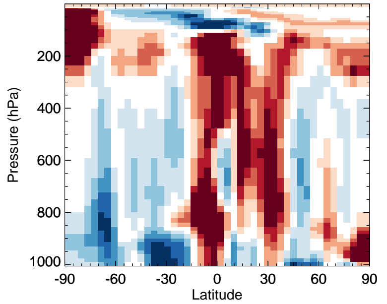
v11-02f-Run1 / v11-02e-Run0 ISOG2 - Zonal mean % diff for Jul
