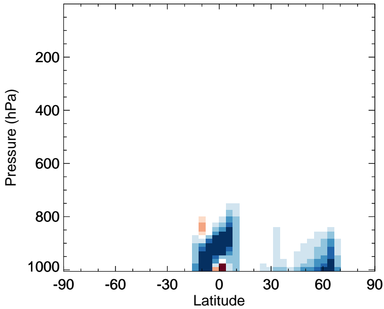
v11-02f-Run1 - v11-02e-Run0 ISOP - Zonal mean abs diff for Jul
