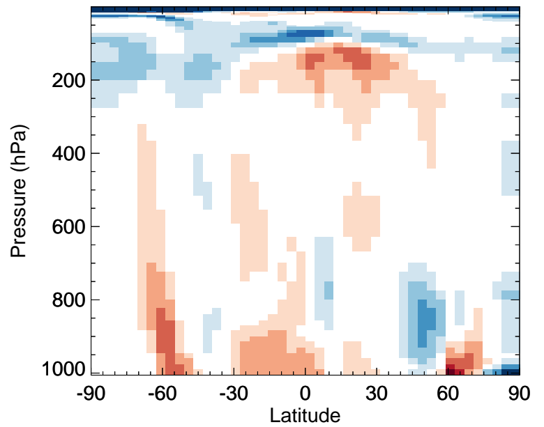
v11-02f-Run1 / v11-02e-Run0 CH 2 O - Zonal mean % diff for Jul
