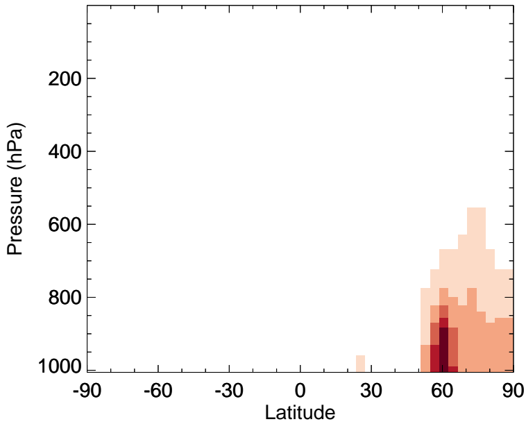
v11-02f-Run1 - v11-02e-Run0 C3H8 - Zonal mean abs diff for Jul
