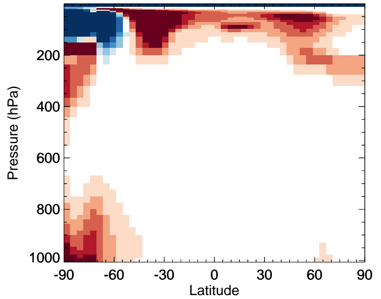
v11-02f-Run1 / v11-02e-Run1 HO2 - Zonal mean % diff for Jul
