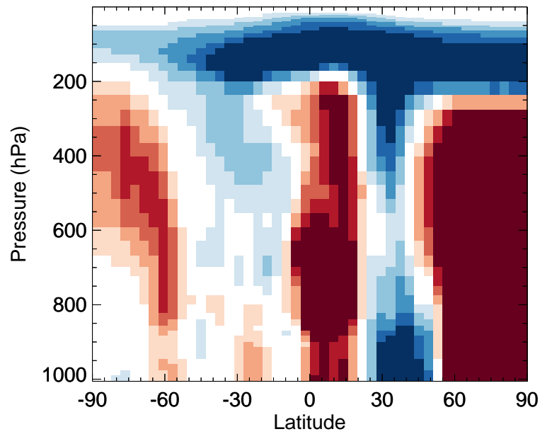
v11-02f-Run1 / v11-02e-Run0 ASOAN - Zonal mean % diff for Jul
