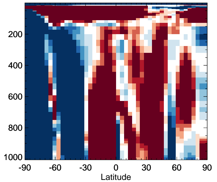
v11-02f-Run1 / v11-02e-Run0 DST3 - Zonal mean % diff for Jul
