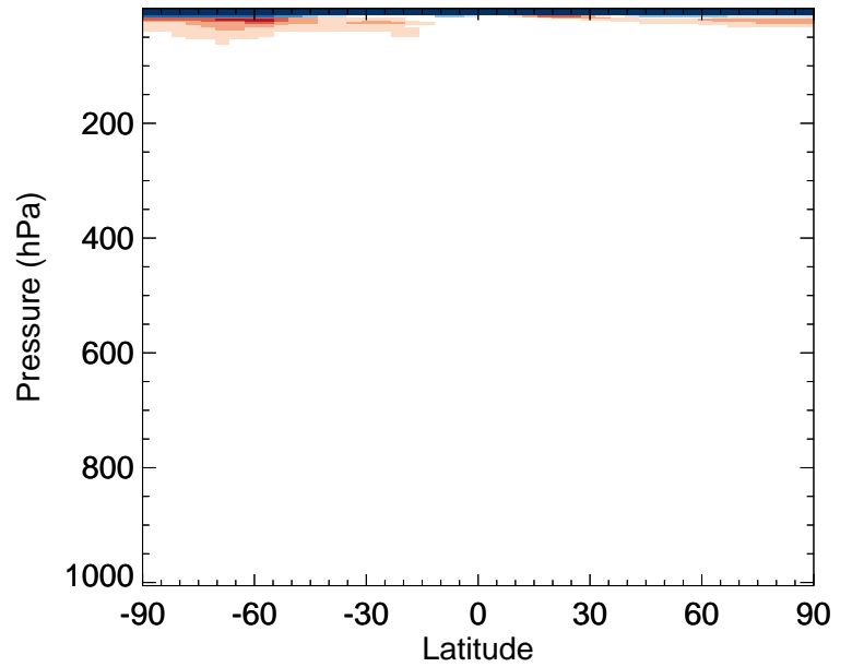
v11-02f-Run1 / v11-02e-Run0 CH4 - Zonal mean % diff for Jul
