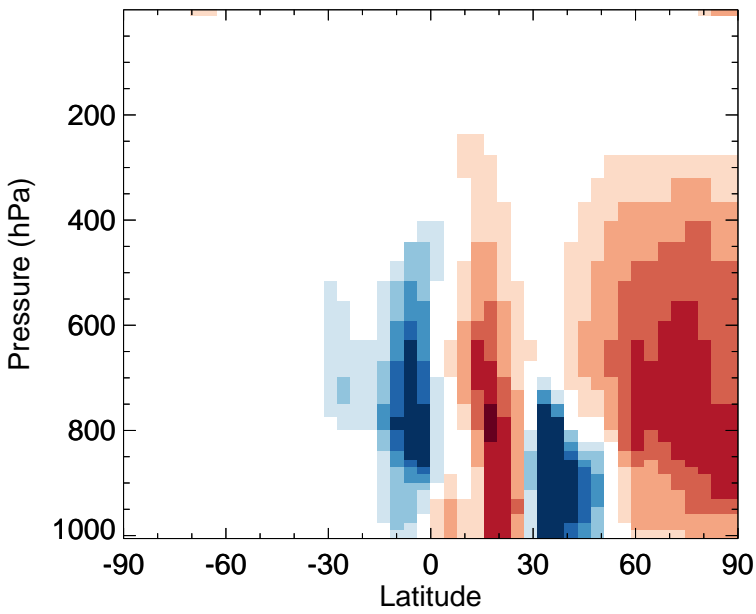
v11-02f-Run1 - v11-02e-Run1 MAP - Zonal mean abs diff for Jul
