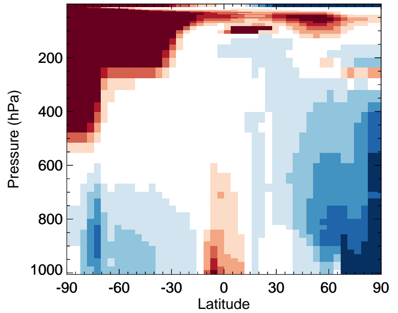
v11-02f-Run1 / v11-02e-Run1 ClO - Zonal mean % diff for Jul
