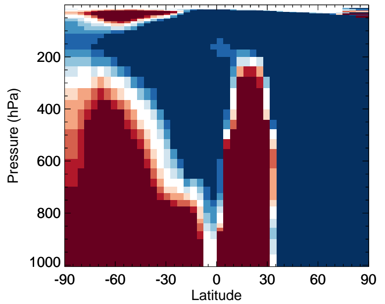
v11-02f-Run1 / v11-02e-Run1 HC187 - Zonal mean % diff for Jul
