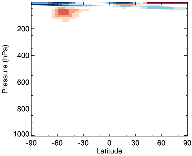
v11-02f-Run1 - v11-02e-Run1 HCl - Zonal mean abs diff for Jul
