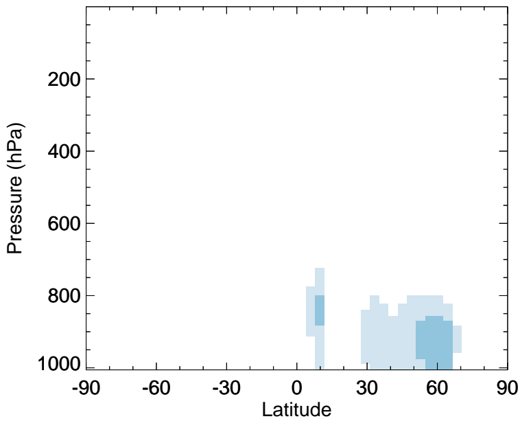
v11-02f-Run1 - v11-02e-Run0 GLYC - Zonal mean abs diff for Jul
