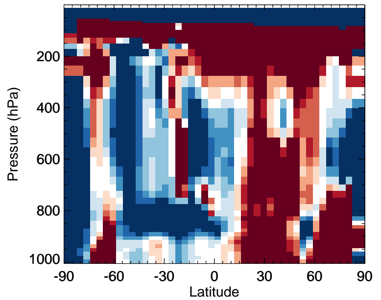
v11-02f-Run1 / v11-02e-Run0 SO 4 s - Zonal mean % diff for Jul
