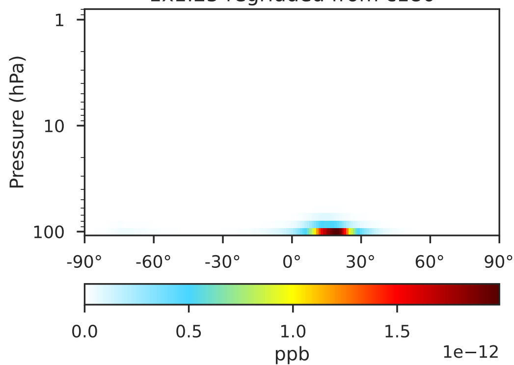
GCHP 14.2.2 using mass flux (Dev) 1x1.25 regridged from c180
