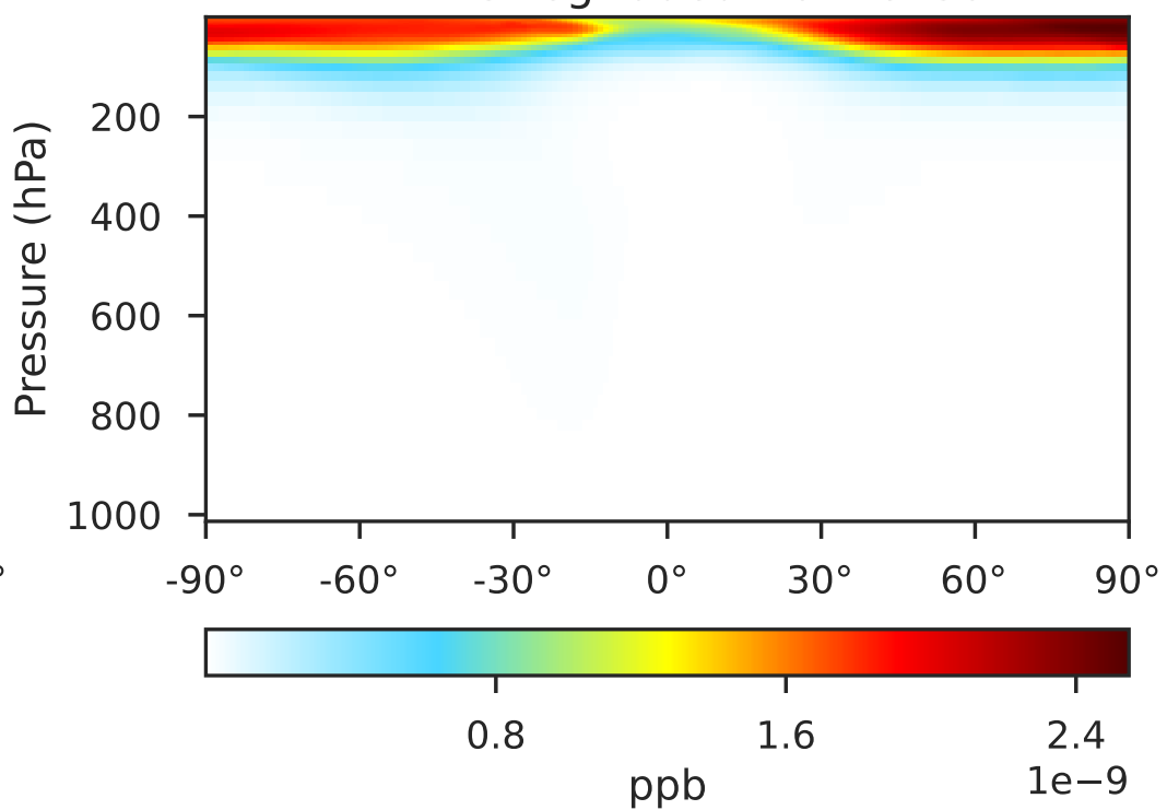
GCHP 14.2.2 using mass flux (Dev) 1x1.25 regridded from c180
