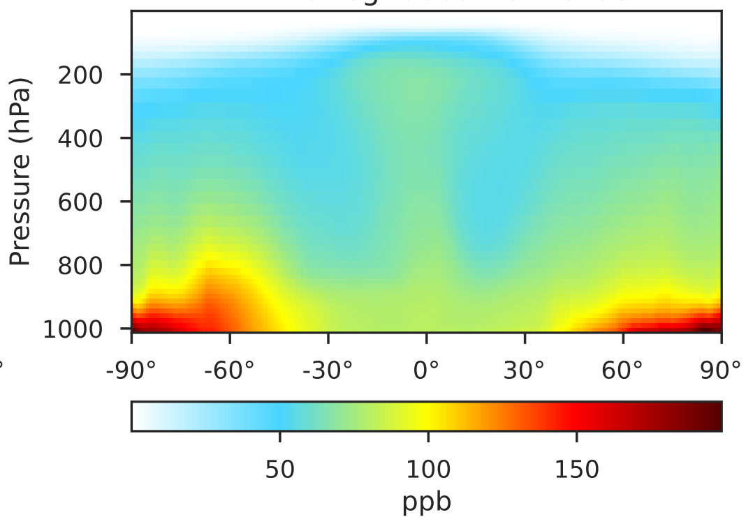
GCHP 14.2.2 using mass flux (Dev) 1x1.25 regrided from c180
