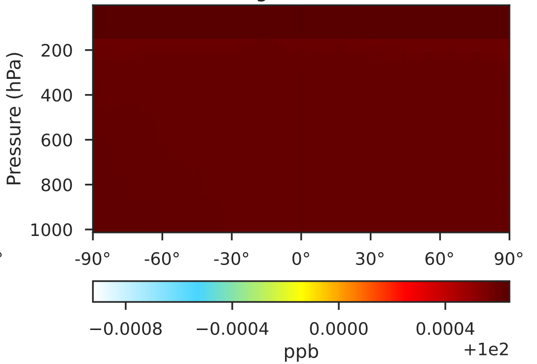
GCHP 14.2.2 using mass flux (Dev) 1x1.25 regridged from c180
