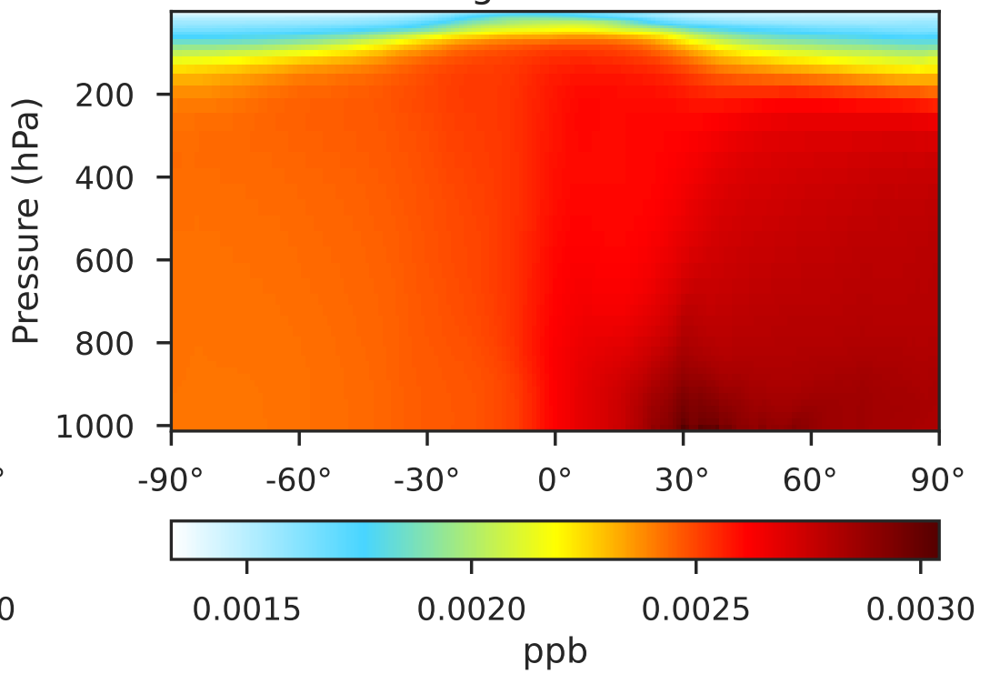
GCHP 14.2.2 using mass flux (Dev) 1x1.25 regrided from c180
