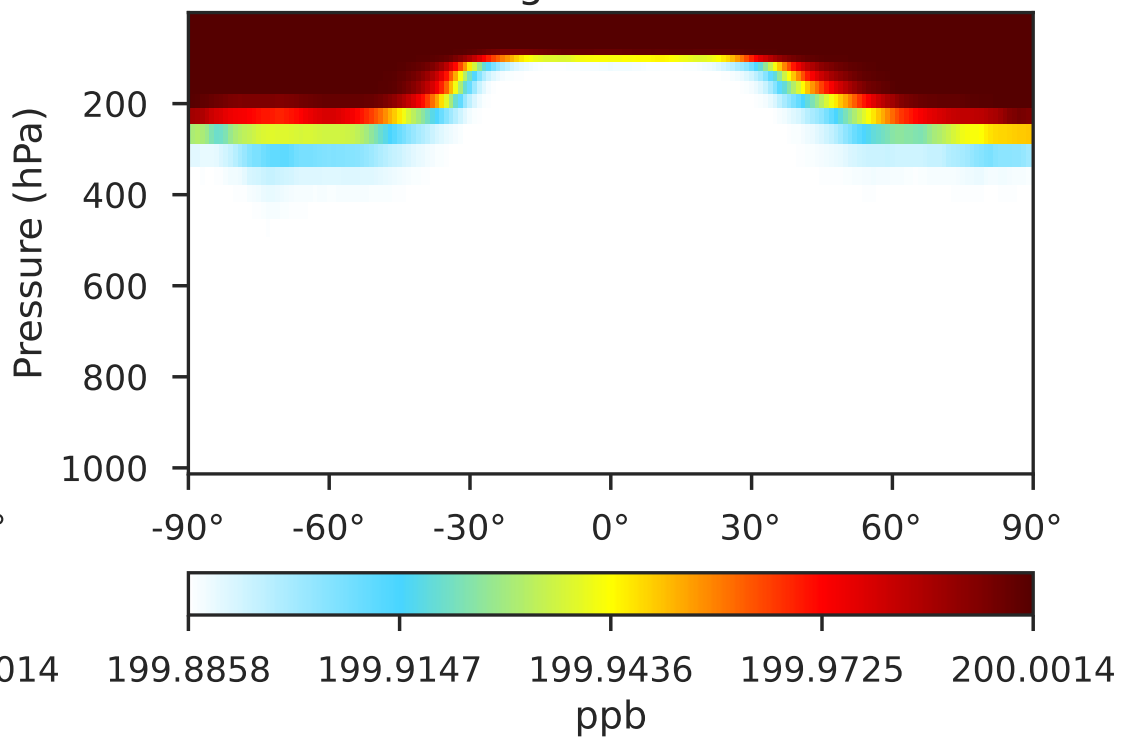
GCHP 14.2.2 using mass flux (Dev) 1x1.25 regrided from c180
