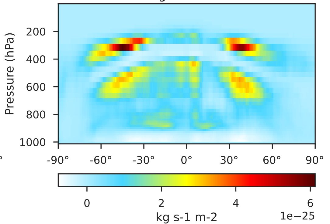
GCHP 14.2.2 using mass flux (Dev), Normalized by Area 1x1.25 regridged from c180
