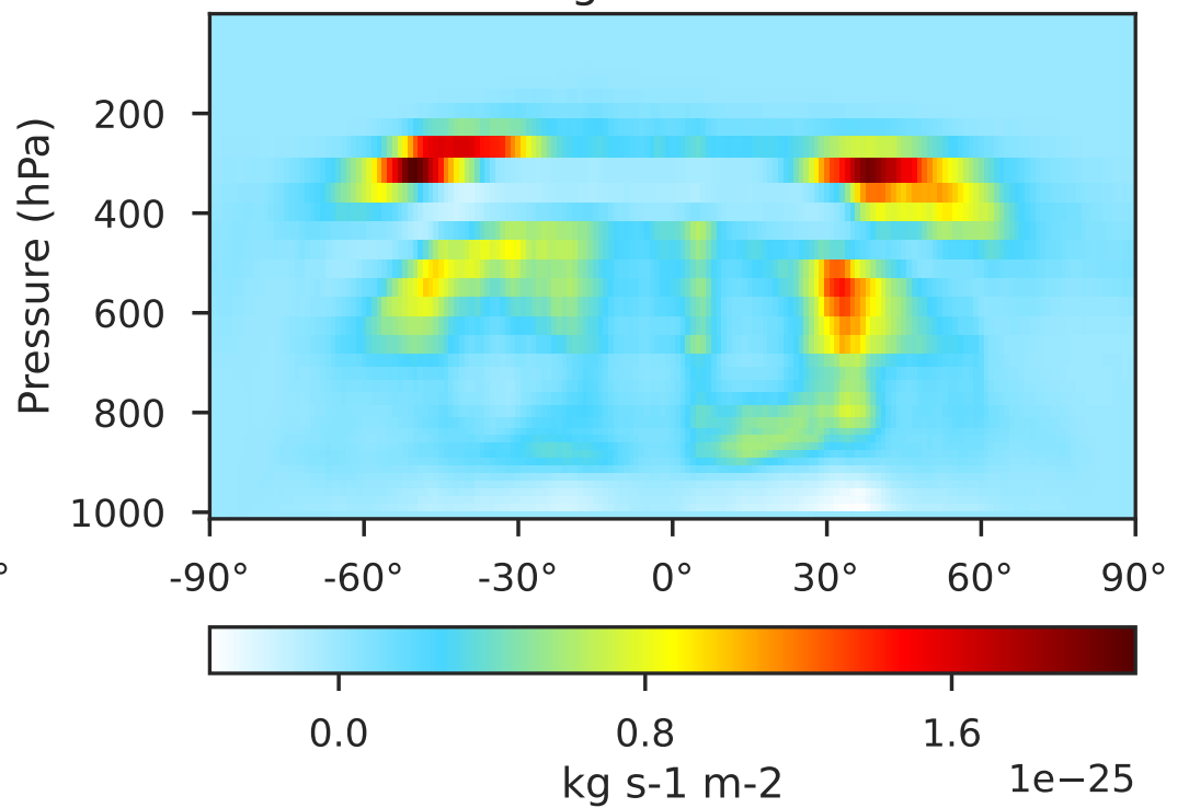
GCHP 14.2.2 using mass flux (Dev), Normalized by Area 1x1.25 regrided from c180
