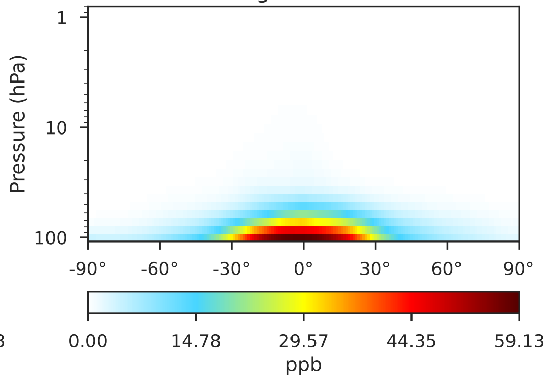
GCHP 14.2.2 using wind (Dev) 1x1.25 regrided from c180
