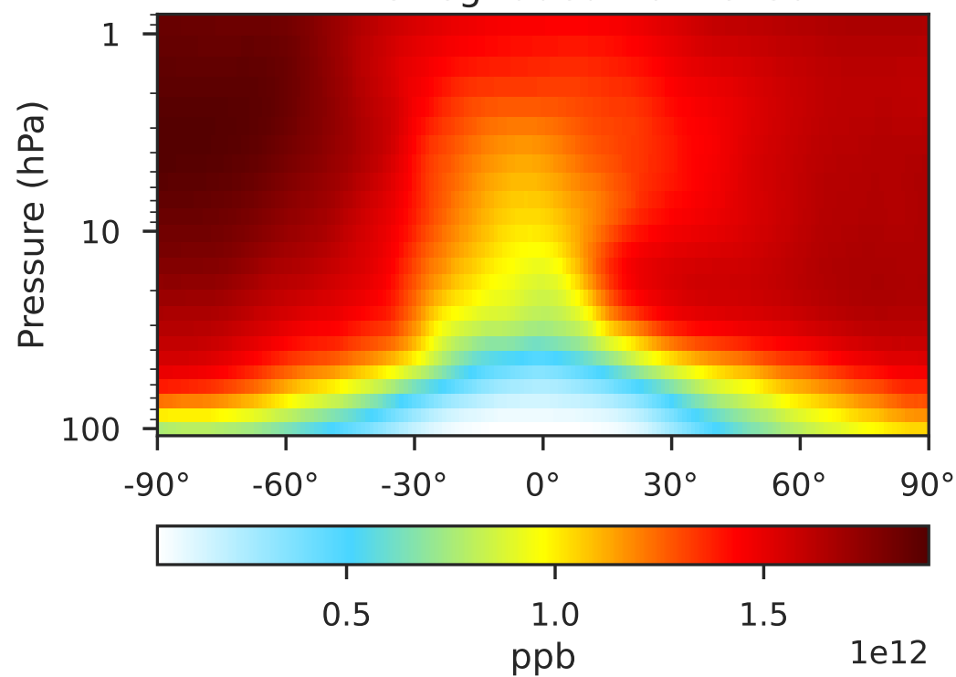
GCHP 14.2.2 using wind (Dev) 1x1.25 regrided from c180
