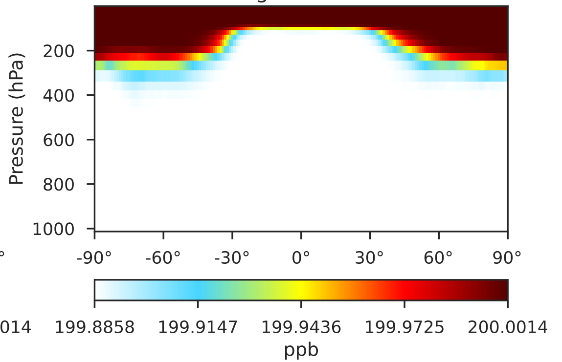
GCHP 14.2.2 using wind (Dev) 1x1.25 regrided from c180
