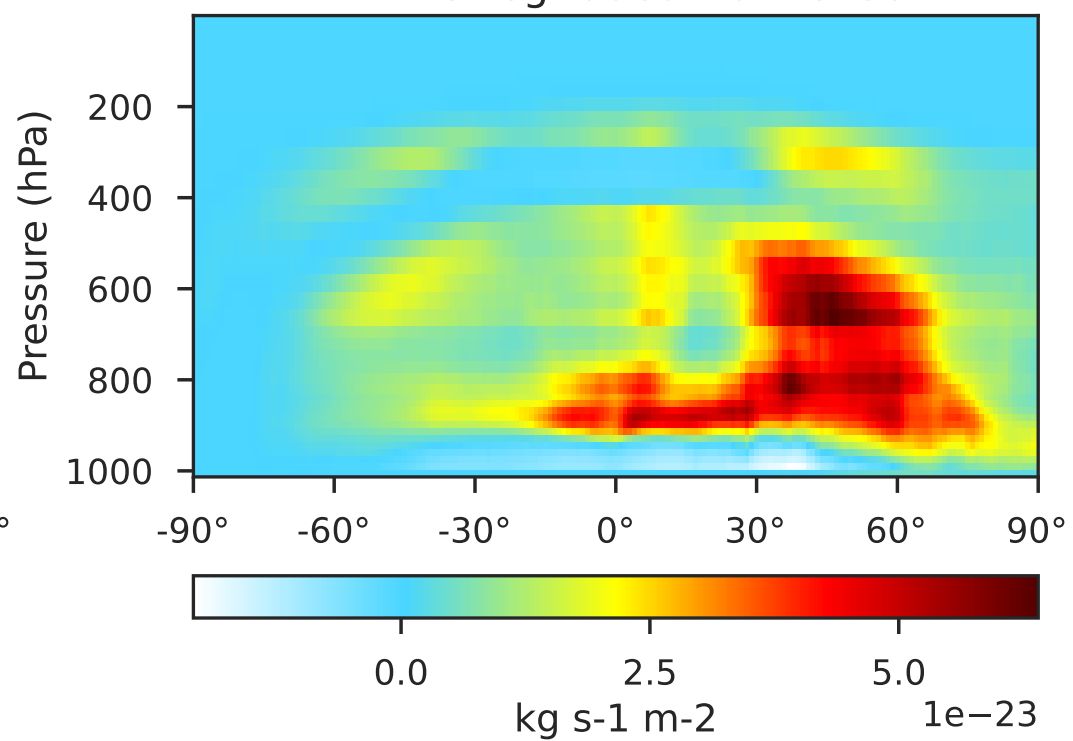
GCHP 14.2.2 using wind (Dev), Normalized by Area 1x1.25 regrided from c180
