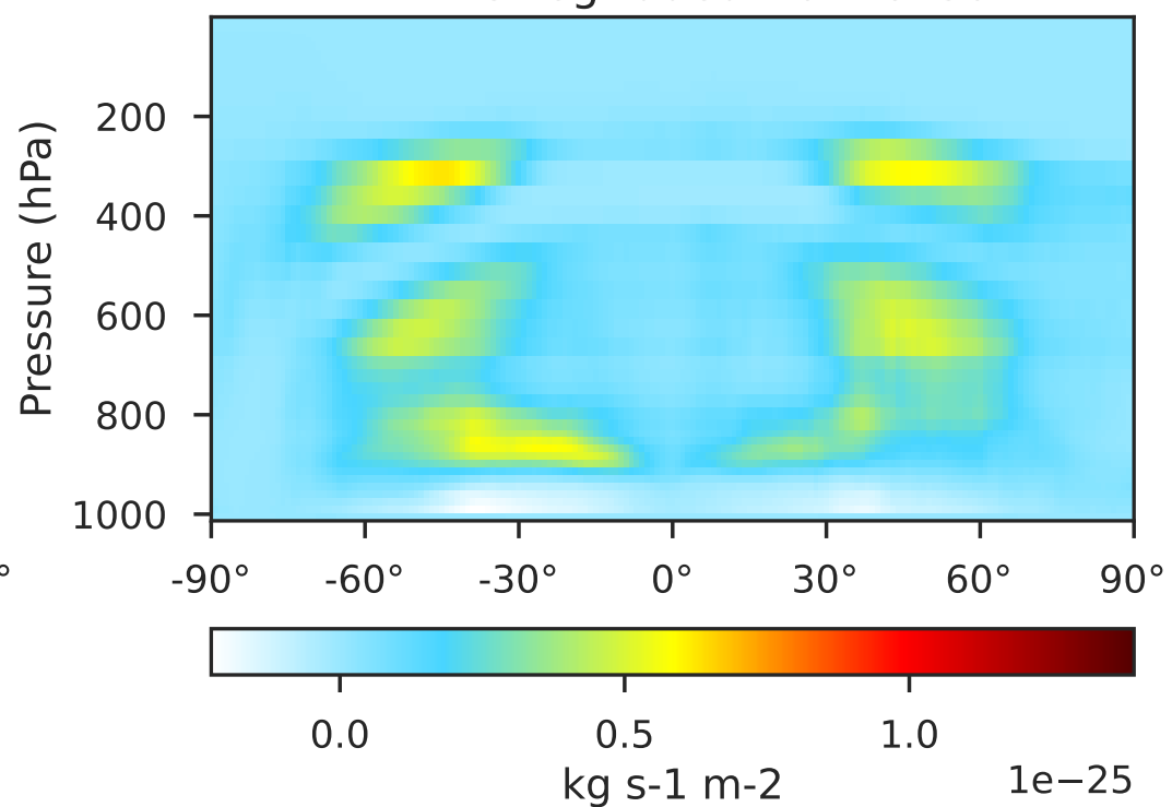
GCHP 14.2.2 using wind (Dev), Normalized by Area 1x1.25 regridged from c180
