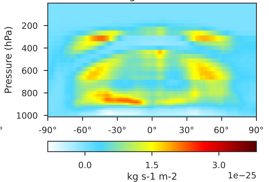
GCHP 14.2.2 using wind (Dev), Normalized by Area 1x1.25 regrided from c180
