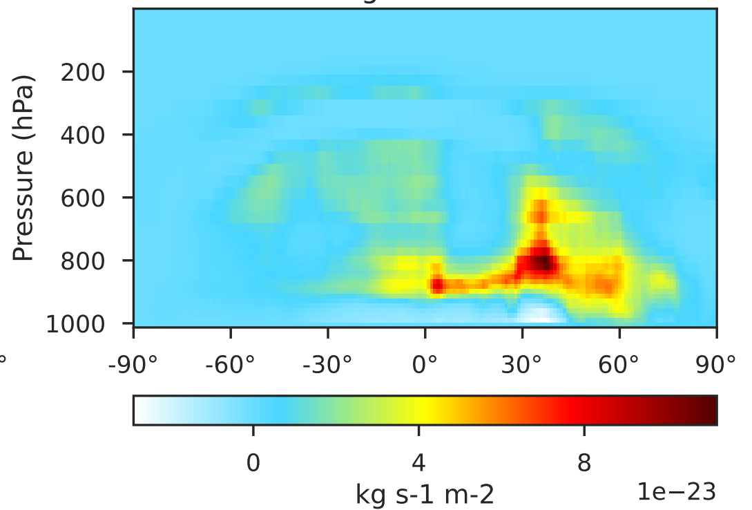
GCHP 14.2.2 using wind (Dev), Normalized by Area 1x1.25 regridged from c180
