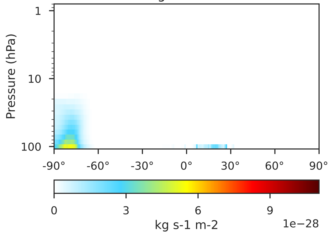
GCHP 14.2.2 using wind (Dev), Normalized by Area 1x1.25 regridded from c180
