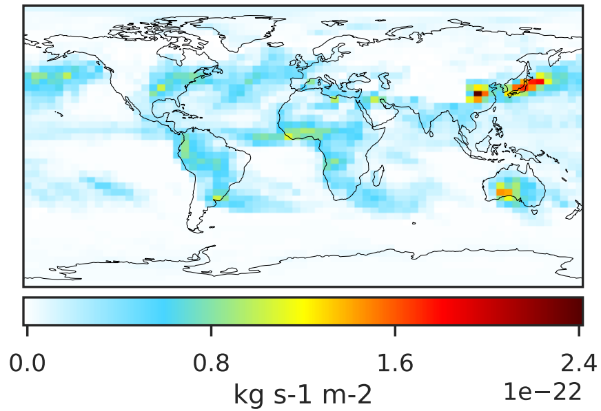
GCC 14.2.2 (Ref), Normalized by Area 4.0x5.0
