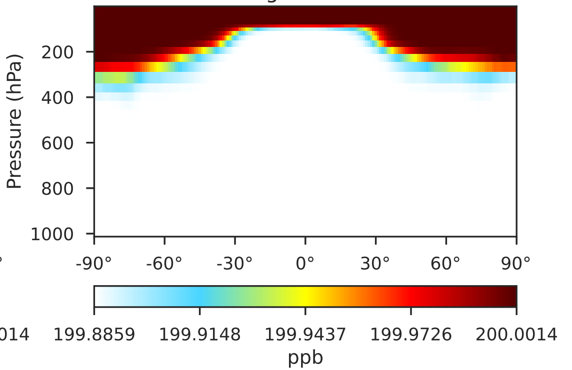
GCHP 14.2.2 using mass flux (Dev) 1x1.25 regrided from c30
