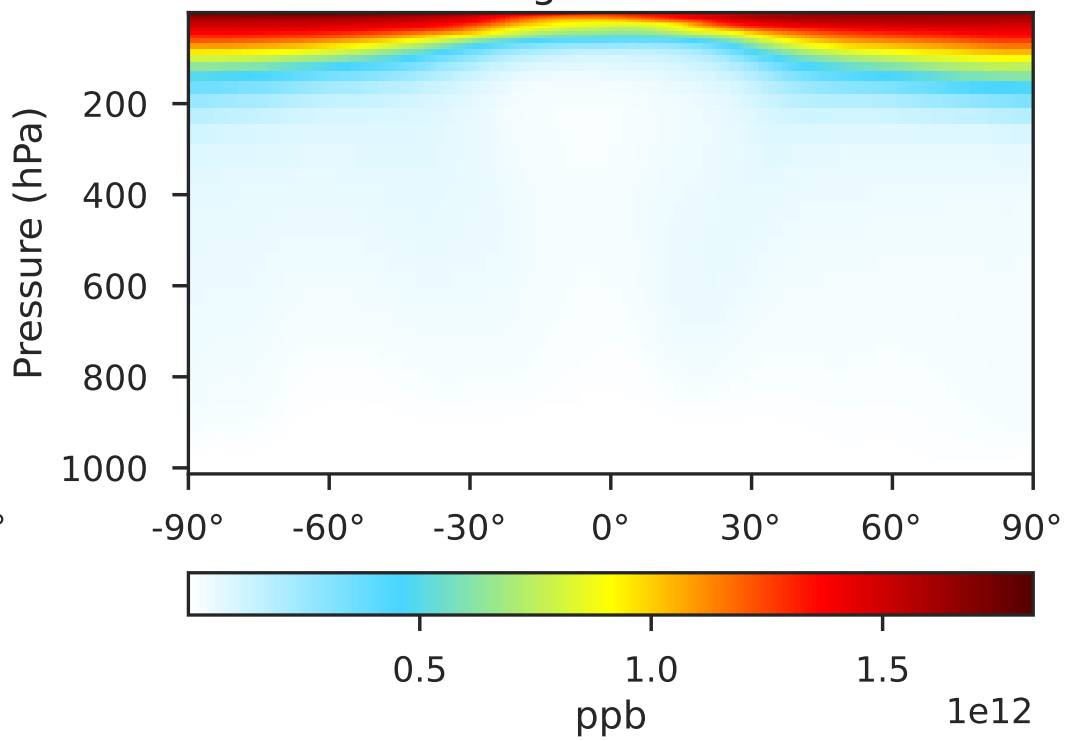
GCHP 14.2.2 using mass flux (Dev) 1x1.25 regridged from c30
