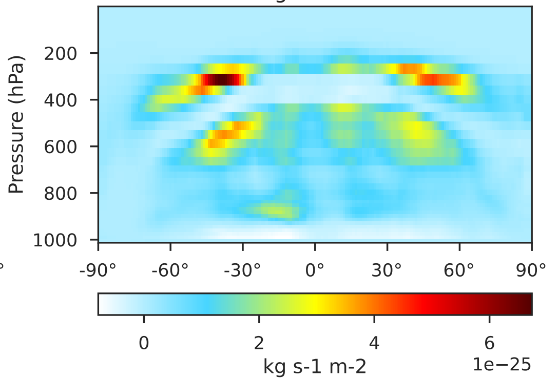
GCHP 14.2.2 using mass flux (Dev), Normalized by Area 1x1.25 regridged from c30
