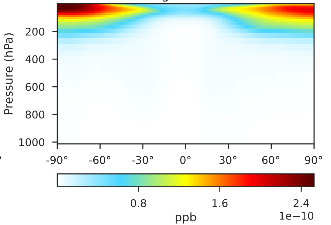
GCHP 14.2.2 using wind (Dev) 1x1.25 regridded from c30
