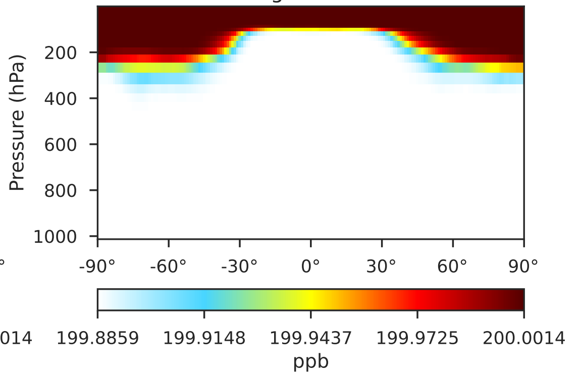
GCHP 14.2.2 using wind (Dev) 1x1.25 regrided from c30
