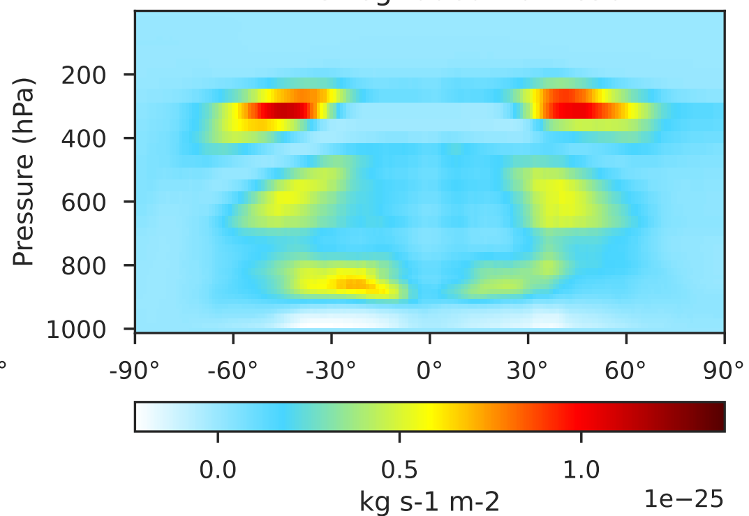
GCHP 14.2.2 using wind (Dev), Normalized by Area 1x1.25 regridged from c30
