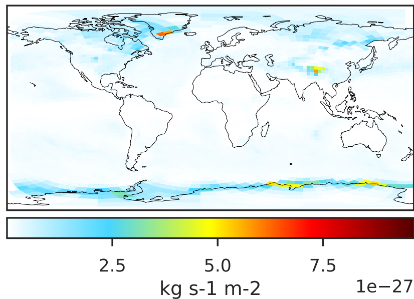
GCHP 14.2.2 using wind (Dev), Normalized by Area c30
