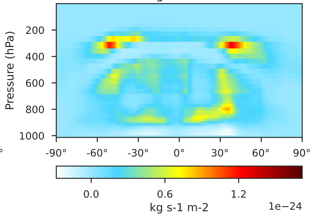
GCHP 14.2.2 using wind (Dev), Normalized by Area 1x1.25 regridged from c30
