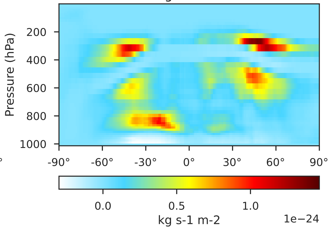
GCHP 14.2.2 using wind (Dev), Normalized by Area 1x1.25 regrided from c30
