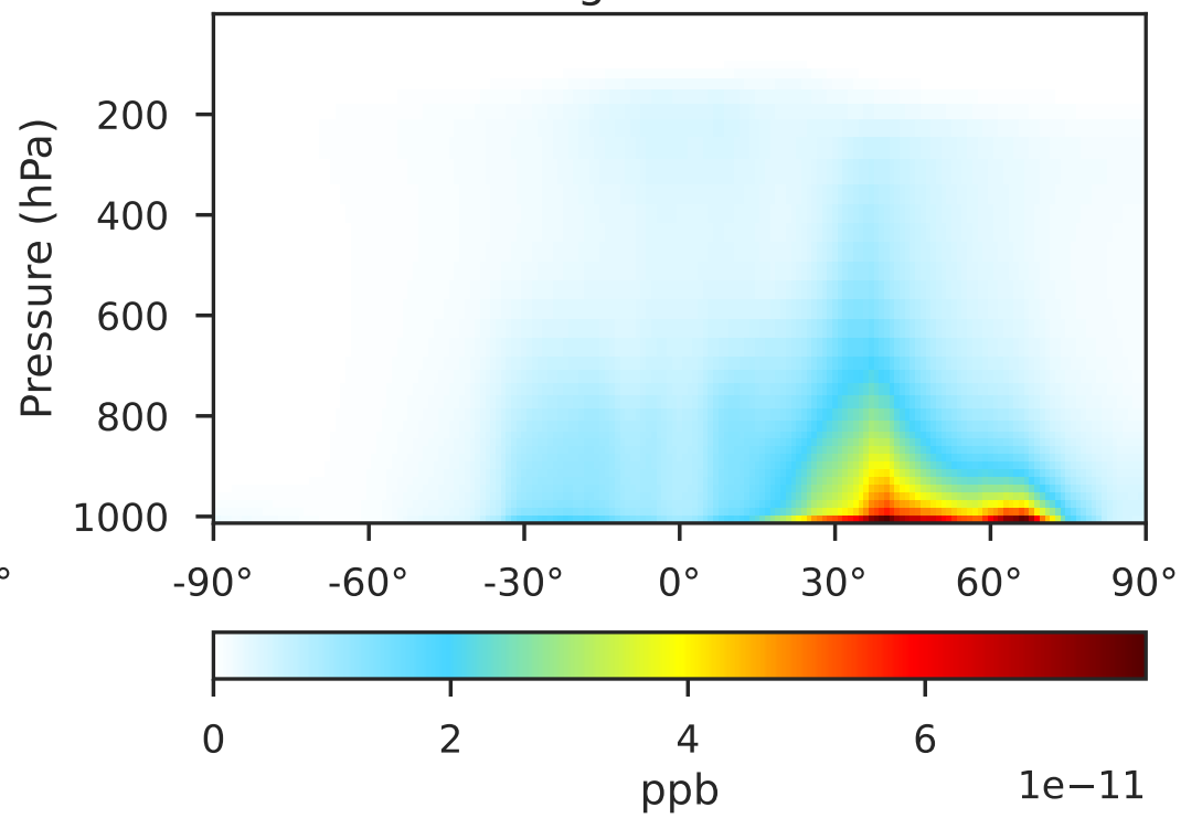
GCHP 14.2.2 using mass flux (Dev) 1x1.25 regridded from c180
