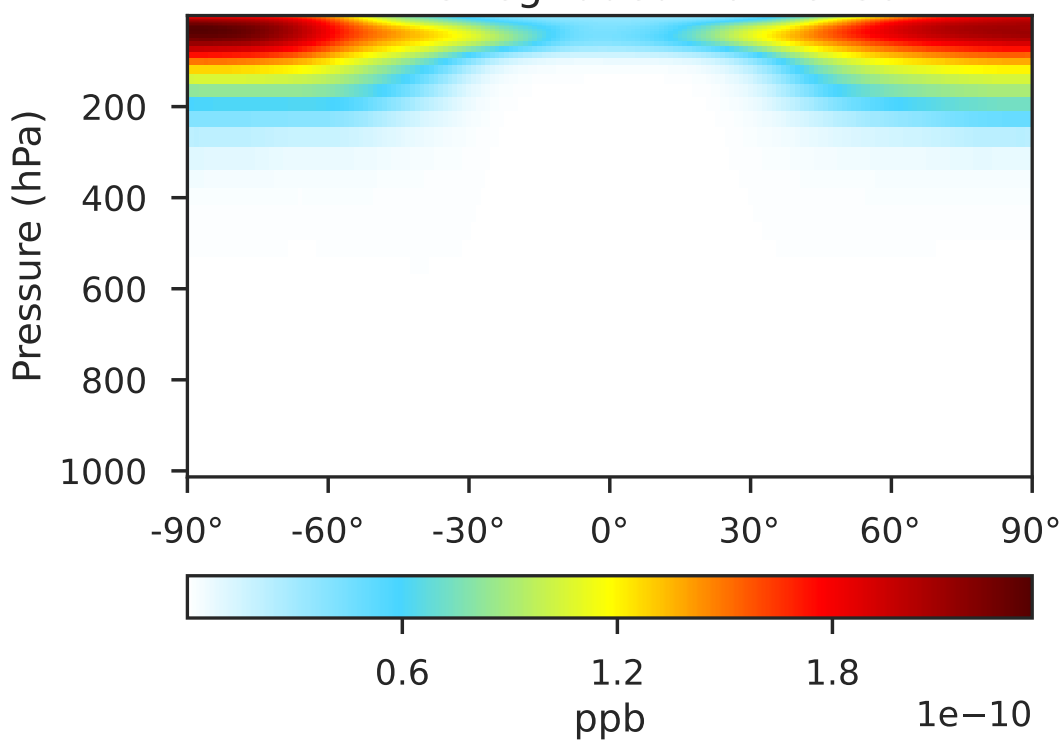
GCHP 14.2.2 using wind (Ref) 1x1.25 regridded from c180
