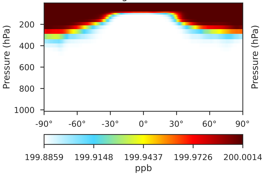
GCHP 14.2.2 using wind (Ref) 1x1.25 regridded from c180
