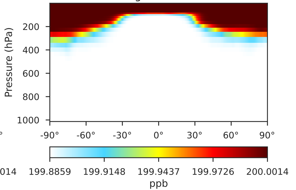
GCHP 14.2.2 using mass flux (Dev) 1x1.25 regridded from c180
