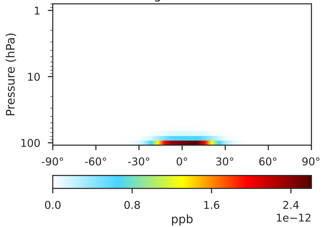
GCHP 14.2.2 using wind (c180) (Dev) 1x1.25 regrided from c180
