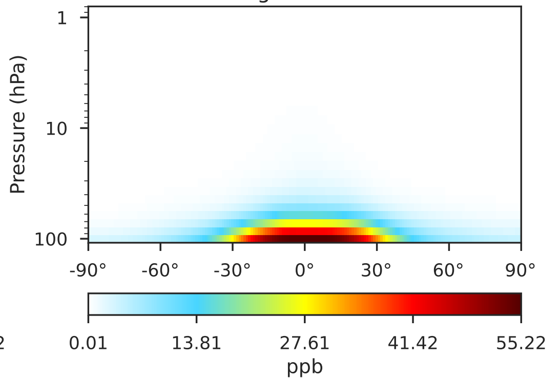
GCHP 14.2.2 using wind (c180) (Dev) 1x1.25 regridded from c180
