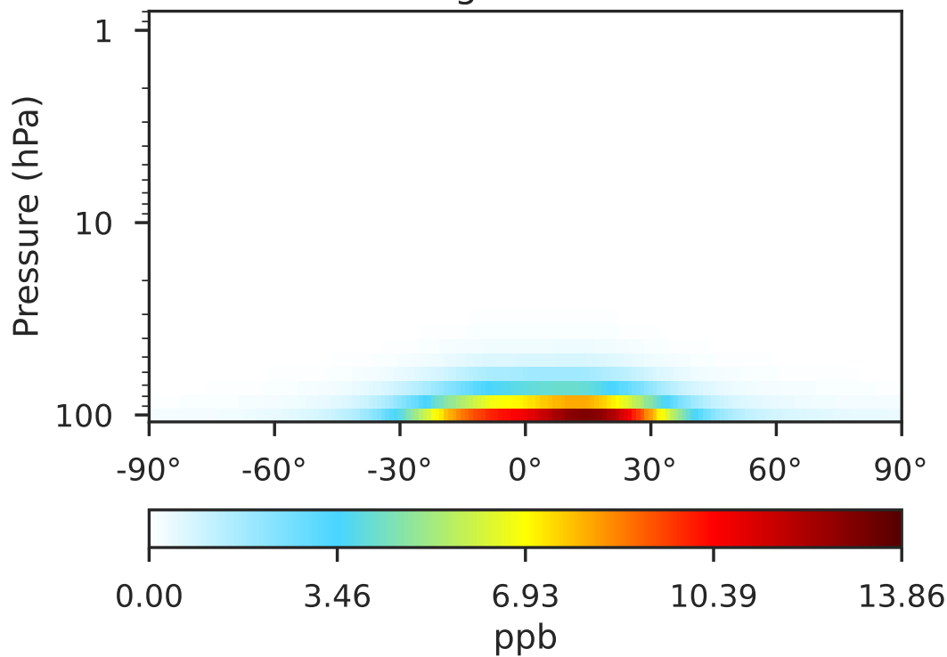
GCHP 14.2.2 using wind (c30) (Ref) 1x1.25 regrided from c30
