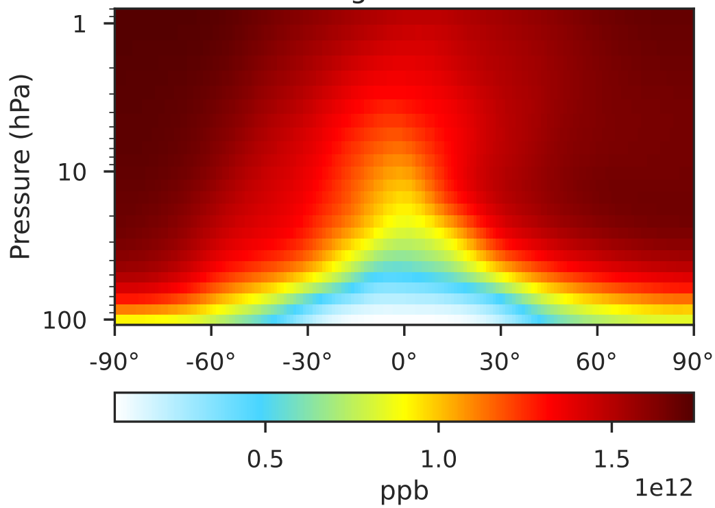
GCHP 14.2.2 using wind (c30) (Ref) 1x1.25 regridded from c30
