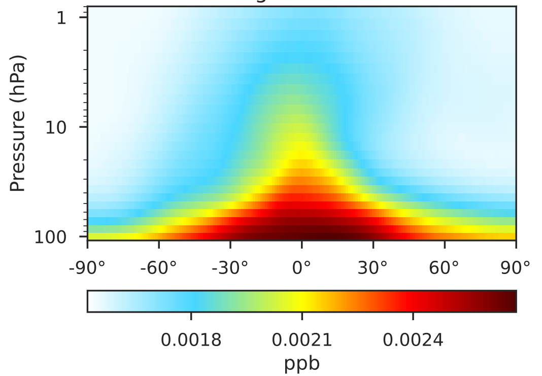
GCHP 14.2.2 using wind (c180) (Dev) 1x1.25 regridded from c180
