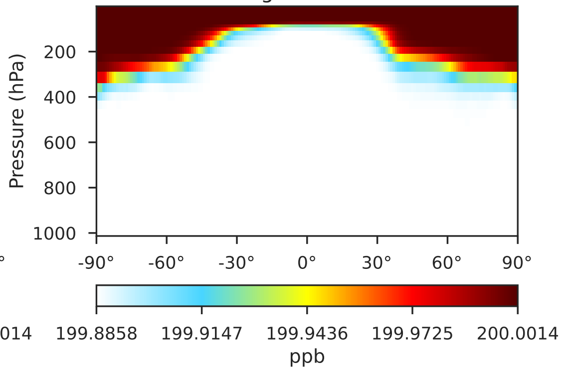
GCHP 14.2.2 using wind (c180) (Dev) 1x1.25 regridded from c180
