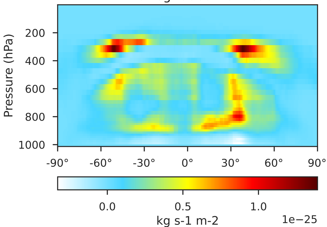
GCHP 14.2.2 using wind (c30) (Ref), Normalized by Area 1x1.25 regridted from c30
