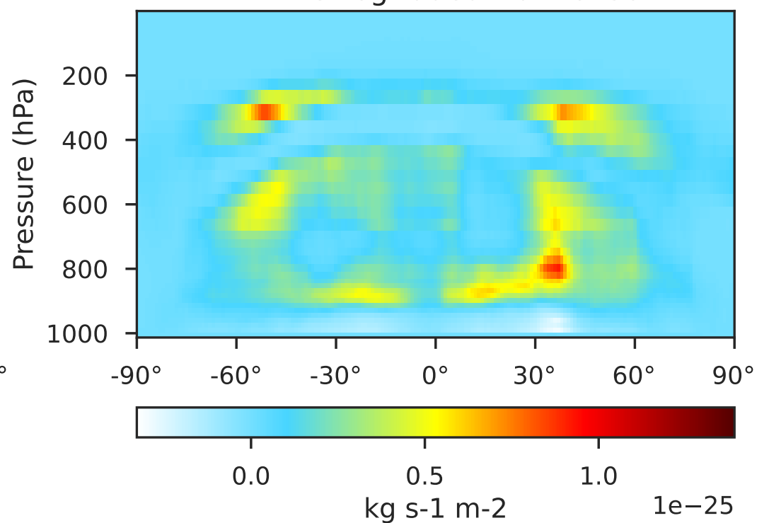
GCHP 14.2.2 using wind (c180) (Dev), Normalized by Area 1x1.25 regridted from c180
