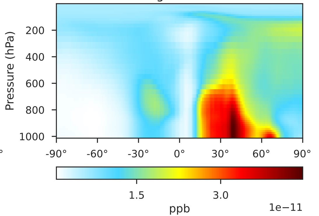
GCHP 14.2.2 using mass flux (Dev) 1x1.25 regridded from c30
