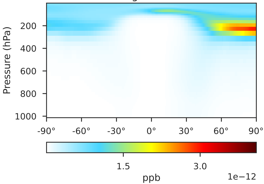
GCHP 14.2.2 using wind (Ref) 1x1.25 regridded from c30
