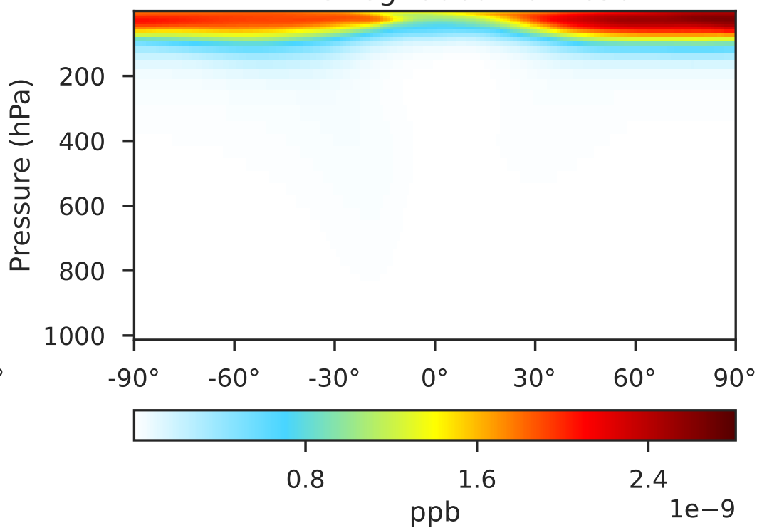
GCHP 14.2.2 using mass flux (Dev) 1x1.25 regridded from c30
