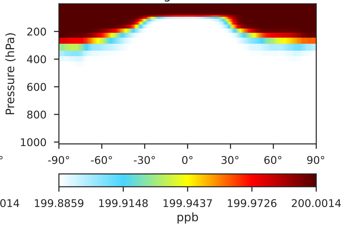
GCHP 14.2.2 using mass flux (Dev) 1x1.25 regridded from c30
