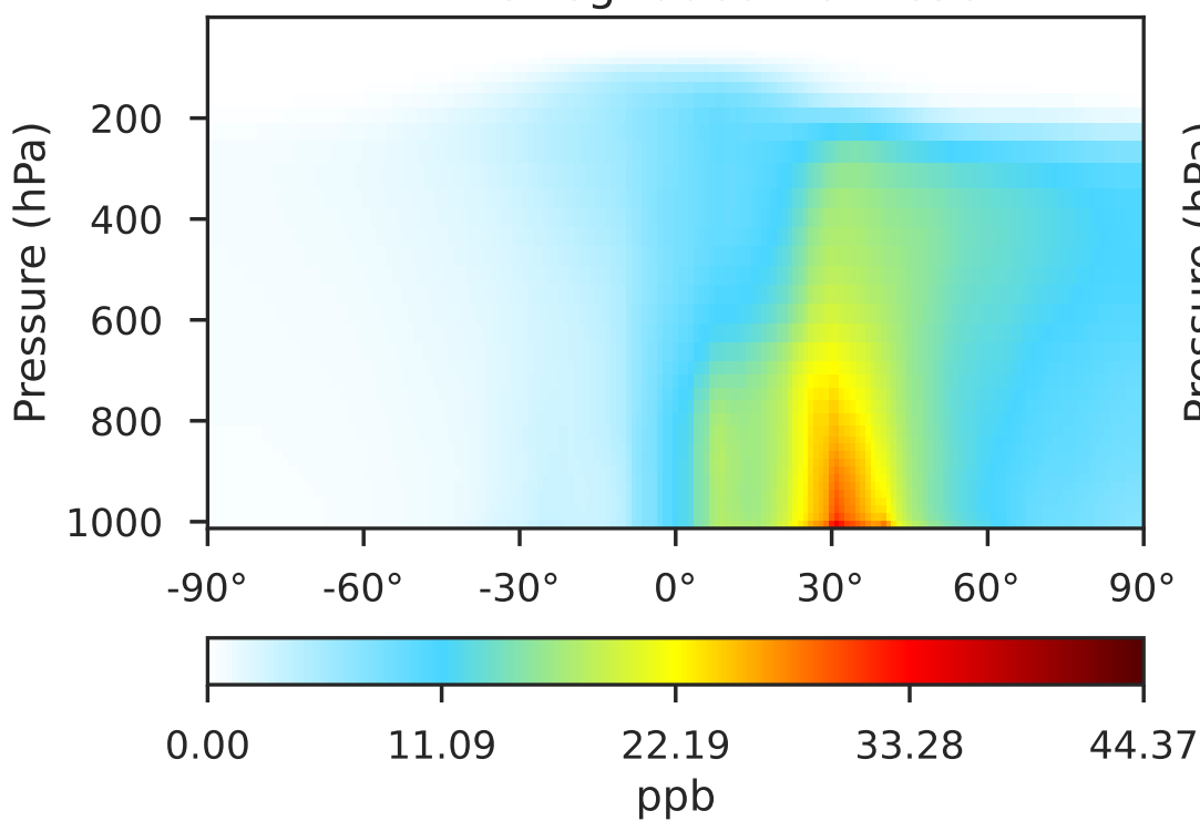
GCHP 14.2.2 using wind (Ref) 1x1.25 regrided from c30
