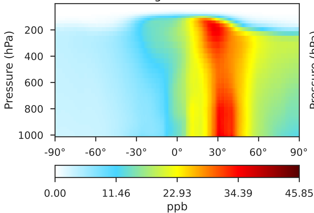
GCHP 14.2.2 using wind (Ref) 1x1.25 regridded from c30
