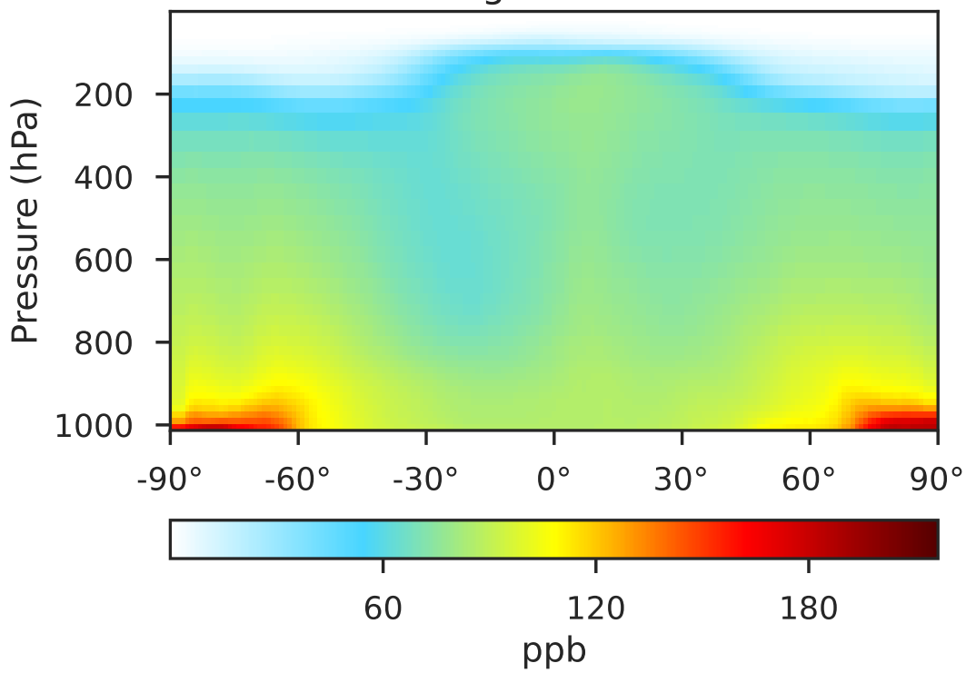
GCHP 14.2.2 using wind (Ref) 1x1.25 regrided from c30
