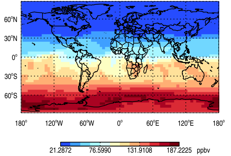
Tracer Map @ 500 hPa - SHEmis90dayTracer
