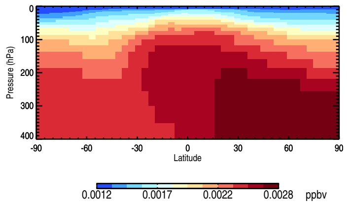
Tracer Curtain @ -180.000 - SF6Tracer
