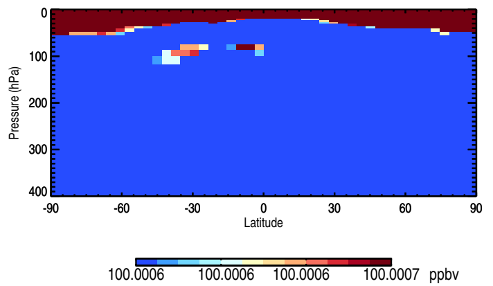
Tracer Curtain @ -180.000 - PassiveTracer
