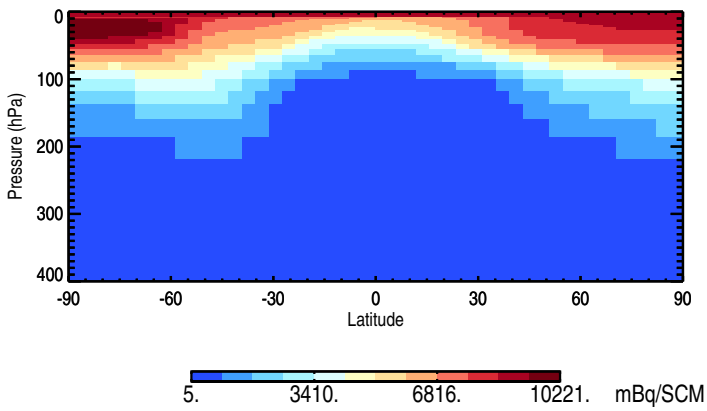
Tracer Curtain Zonal mean - Be10Strat
