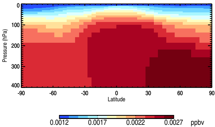
Tracer Curtain Zonal mean - SF6Tracer
