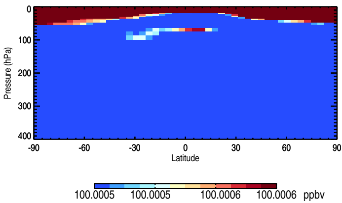
Tracer Curtain Zonal mean - PassiveTracer
