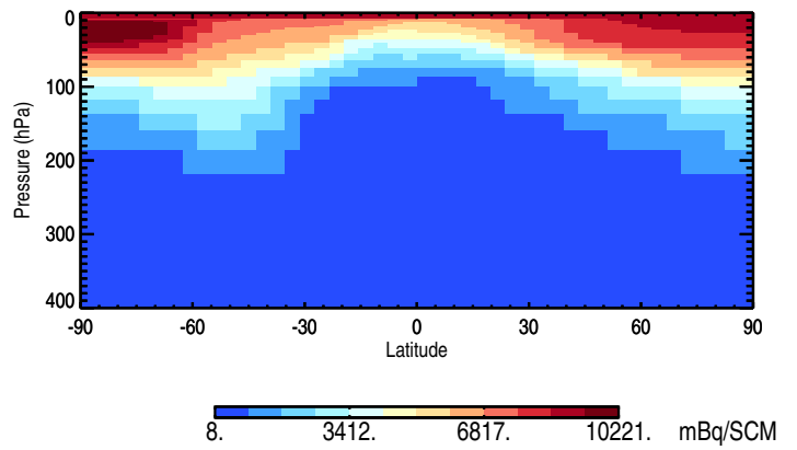
Tracer Curtain @ -180.000 - Be10Strat
