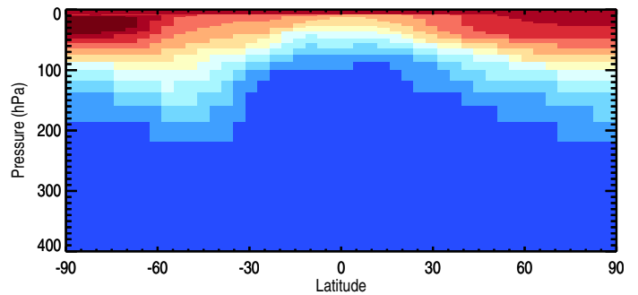
Tracer Curtain @ -180.000 - Be10
