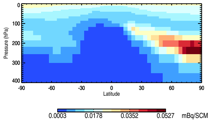
Tracer Curtain @ -180.000 - Pb210Strat
