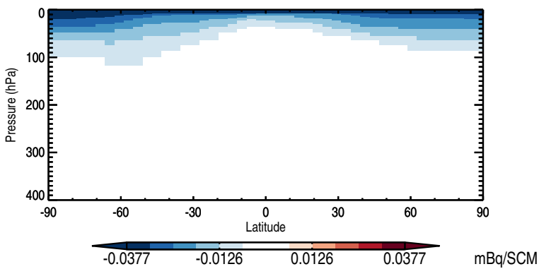
Zonal mean abs diff: Pb210
