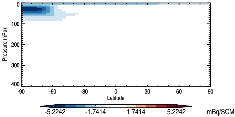
Zonal mean abs diff: Be7
