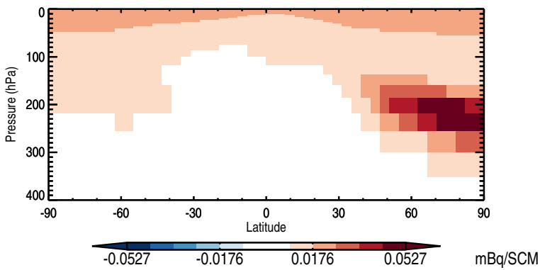
Zonal mean abs diff: Pb210Strat
