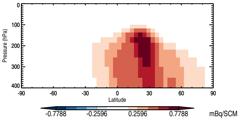
Zonal mean abs diff: Rn222
