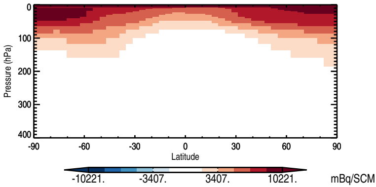
Zonal mean abs diff: Be10Strat
