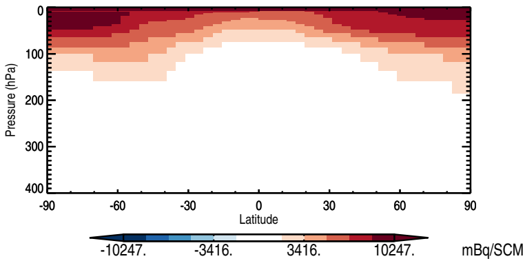
Zonal mean abs diff: Be10
