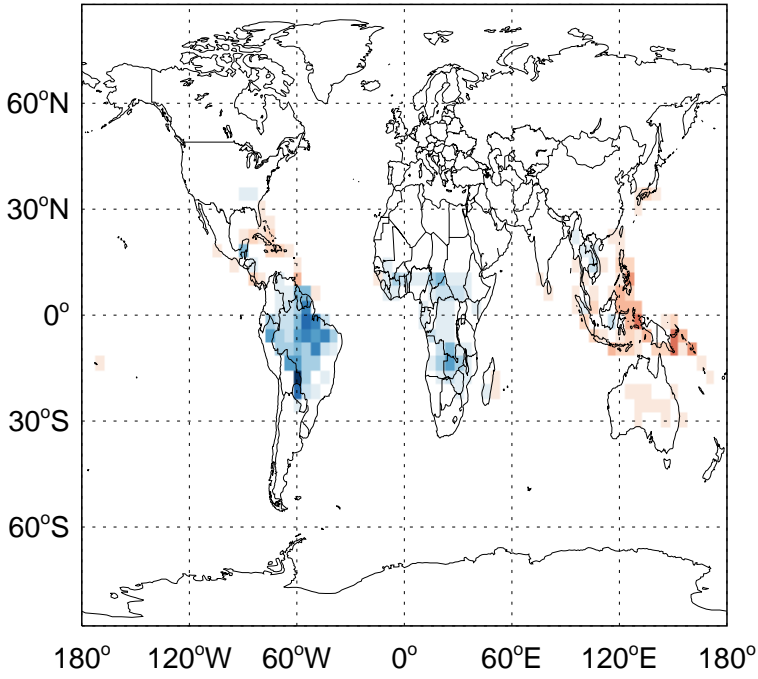
ALD2 biogenic emissions for Oct
