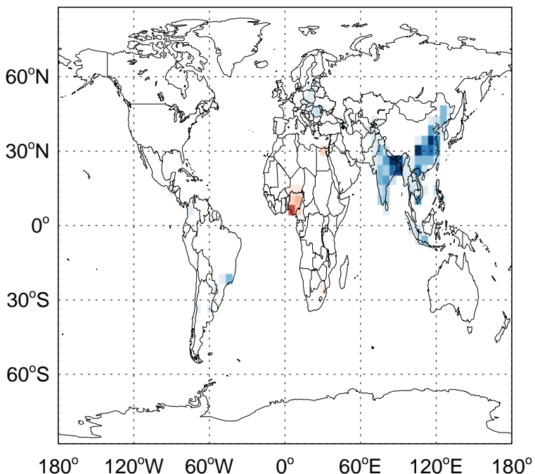
BC biofuel emissions for Apr
