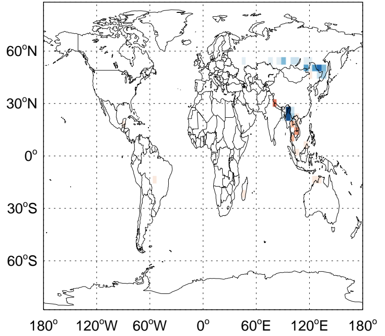
BC biomass emissions for Apr
