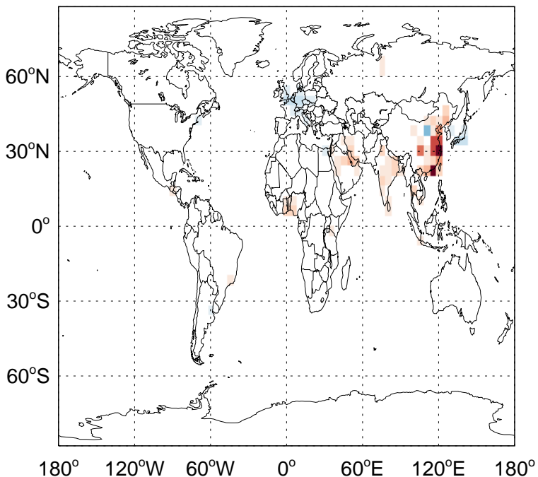
BC column anthro emissions for Apr
