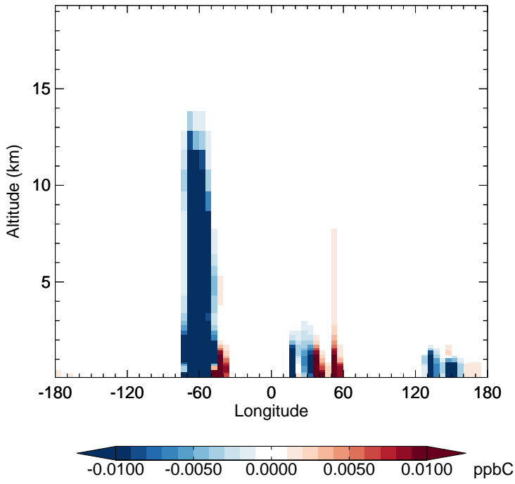
GC_12.0.0 - v11-02f-Run1 PRPE - Diff along 15S for Jan
