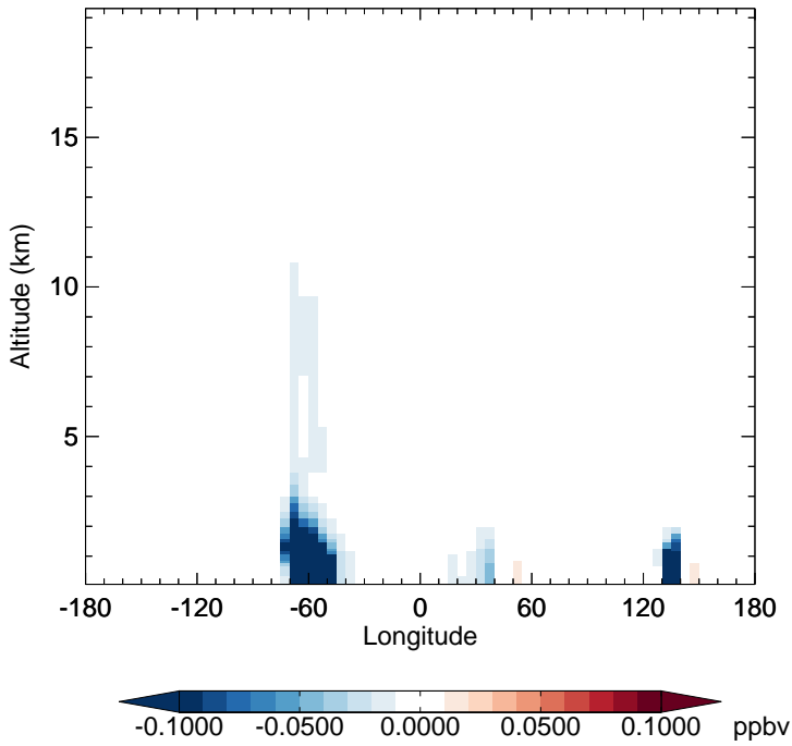
GC_12.0.0 - v11-02e-Run1 HPALD - Diff along 15S for Jan
