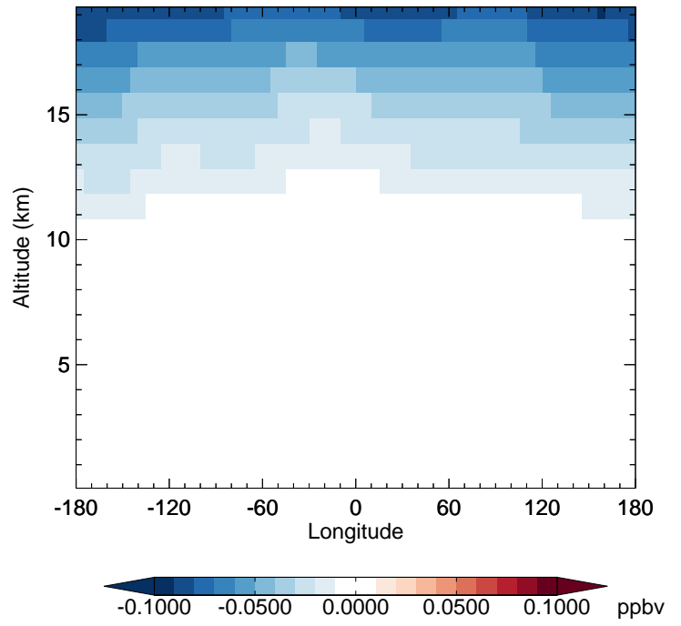
GC_12.0.0 - v11-02f-Run1 HCl - Diff along 42N for Jan
