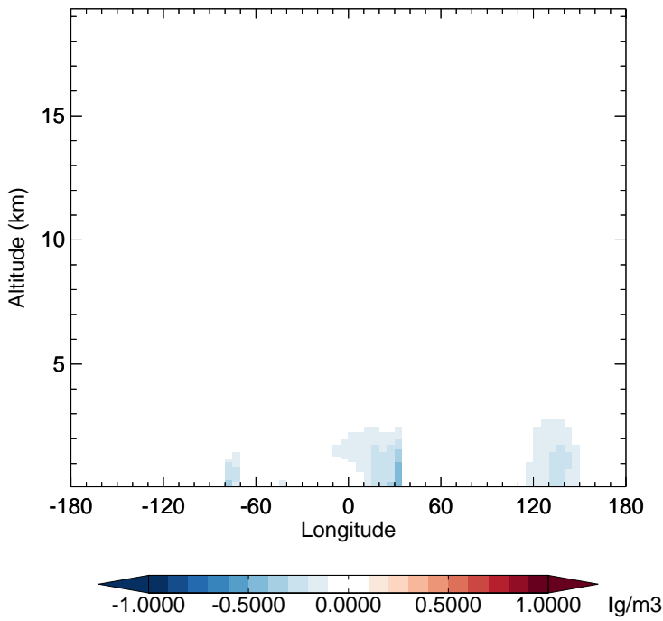
GC_12.0.0 - v11-02e-Run1 SO4 - Diff along 15S for Jan
