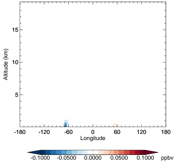
GC_12.0.0 - v11-02e-Run1 SOAP - Diff along 42N for Jan
