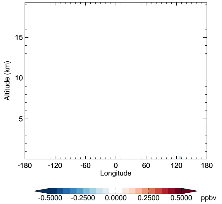
GC_12.0.0 - v11-02f-Run1 CH 2 O - Diff along 42N for Jan
