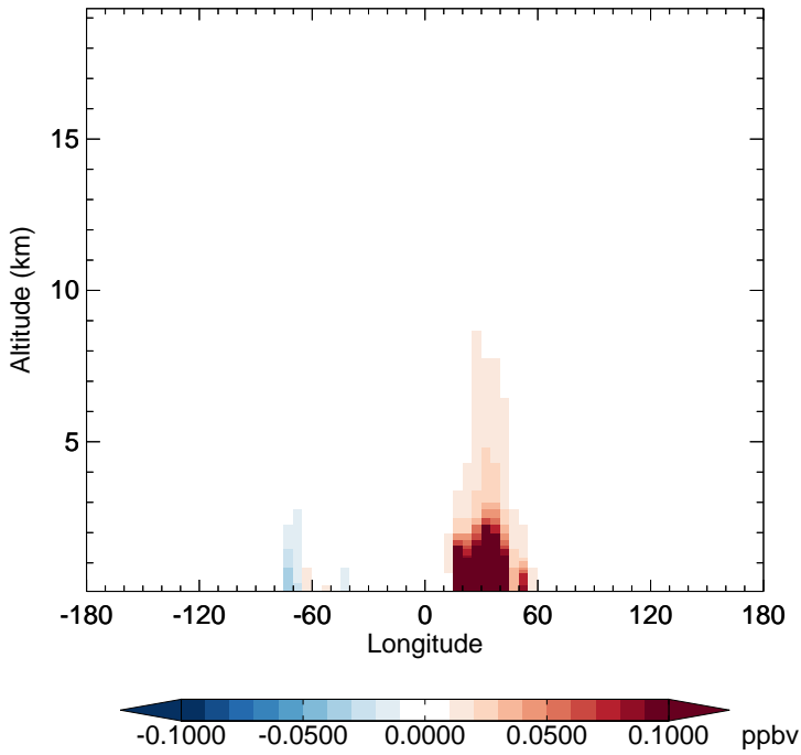
GC_12.0.0 - v11-02e-Run1 TOLU - Diff along 15S for Jan
