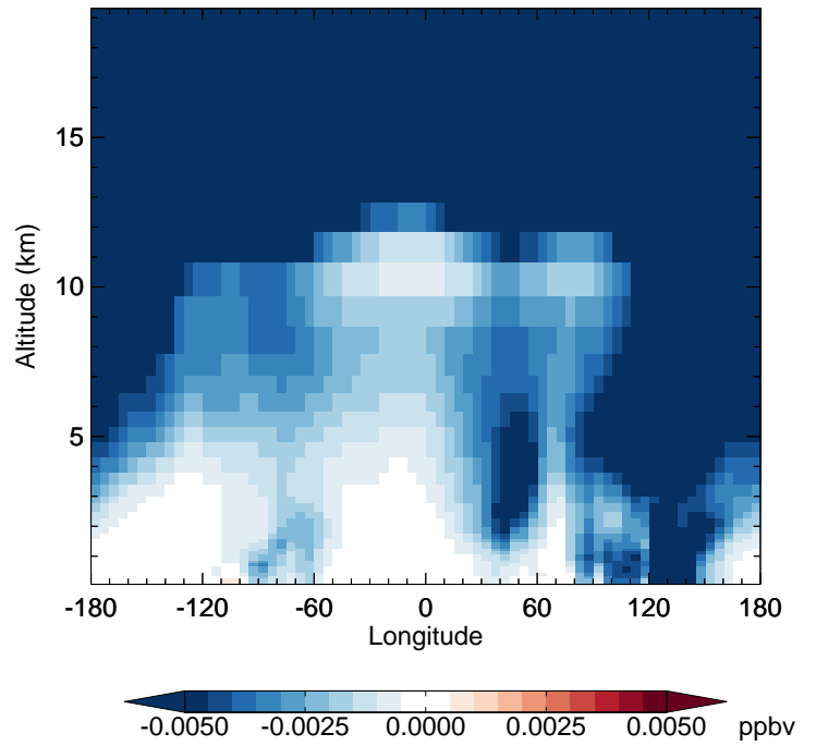
GC_12.0.0 - v11-02e-Run1 HNO 4 - Diff along 42N for Jan
