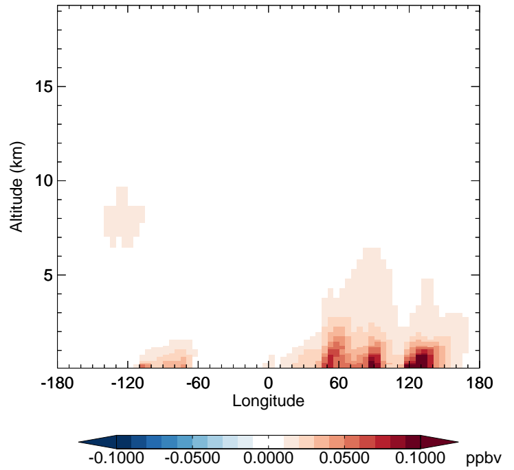
GC_12.0.0 - v11-02e-Run1 HCOOH - Diff along 42N for Jan
