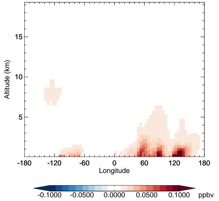
GC_12.0.0 - v11-02f-Run1 HCOOH - Diff along 42N for Jan
