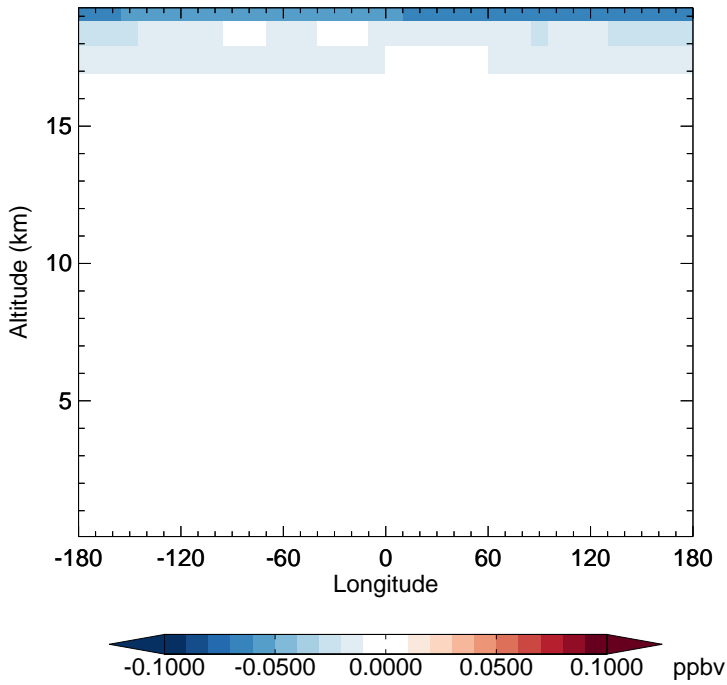
GC_12.0.0 - v11-02e-Run1 HCl - Diff along 15S for Jan
