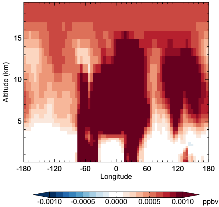
GC_12.0.0 - v11-02e-Run1 PPN - Diff along 15S for Jan
