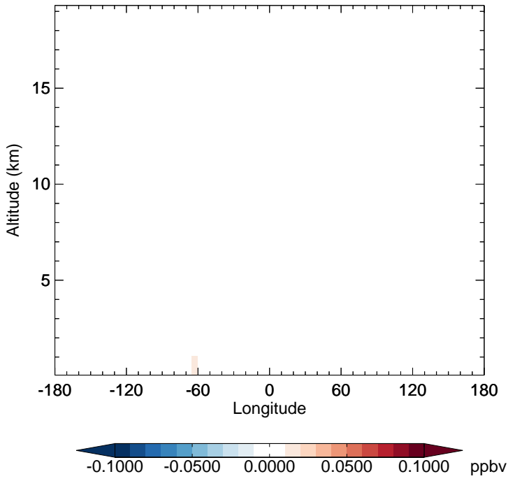
GC_12.0.0 - v11-02f-Run1 TSOG3 - Diff along 15S for Jan
