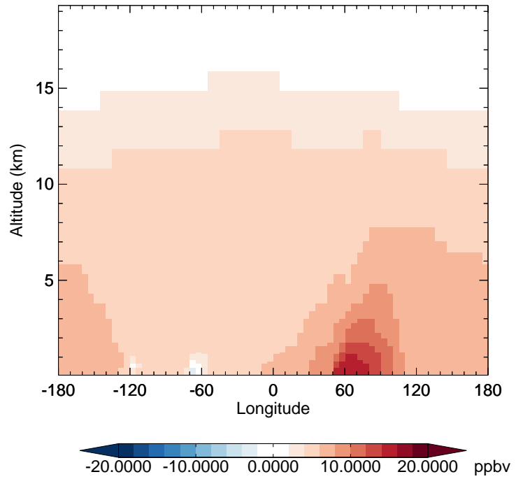
GC_12.0.0 - v11-02e-Run1 CO - Diff along 42N for Jan
