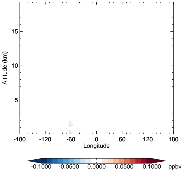
GC_12.0.0 - v11-02e-Run1 TSOA2 - Diff along 15S for Jan
