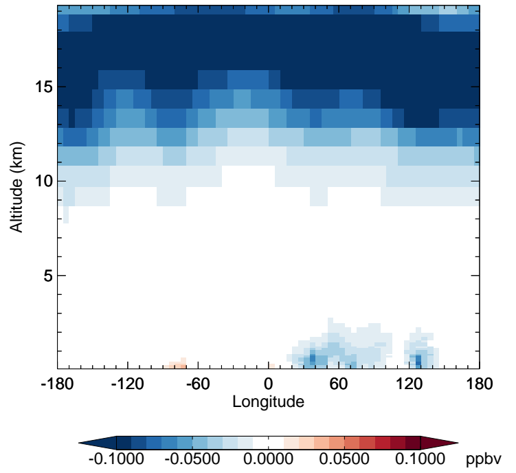
GC_12.0.0 - v11-02f-Run1 HNO 3 - Diff along 42N for Jan
