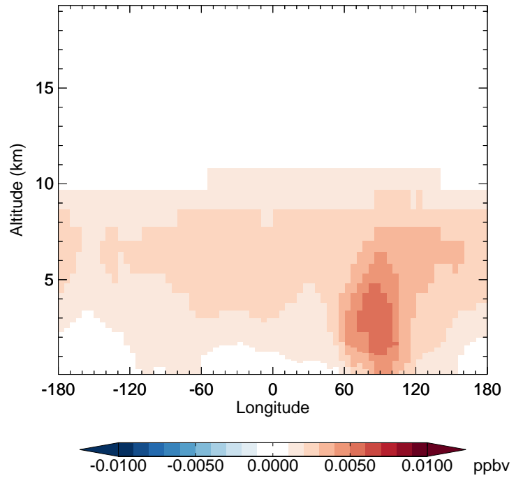
GC_12.0.0 - v11-02e-Run1 MAP - Diff along 42N for Jan
