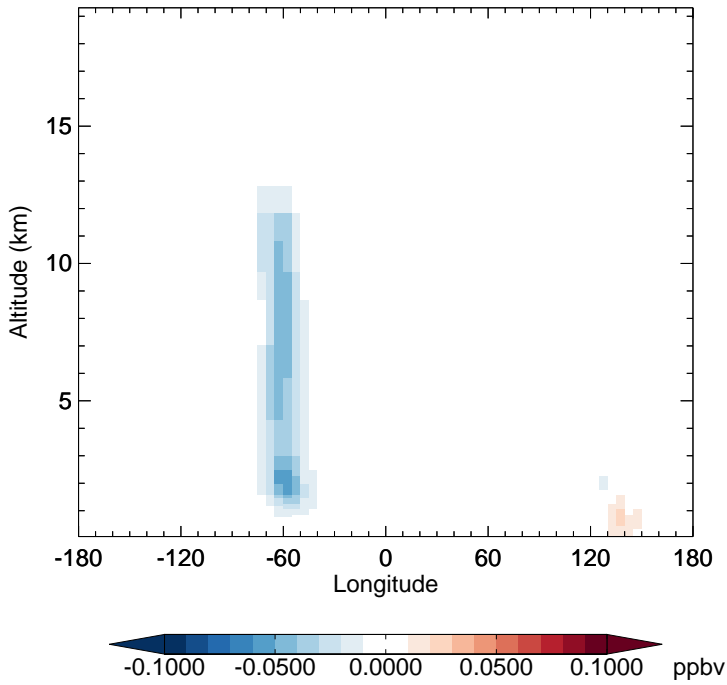
GC_12.0.0 - v11-02e-Run1 HC187 - Diff along 15S for Jan
