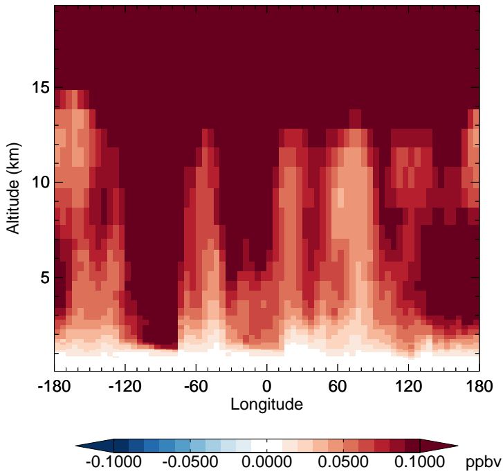
GC_12.0.0 - v11-02e-Run1 N2O - Diff along 15S for Jan
