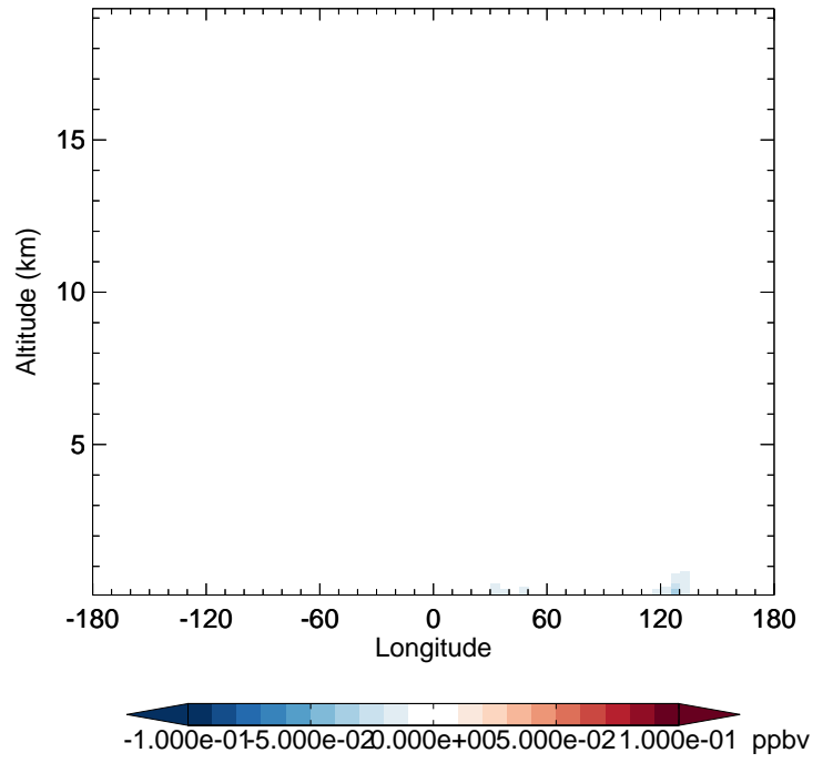
GC_12.0.0 - v11-02f-Run1 GLYC - Diff along 42N for Jan
