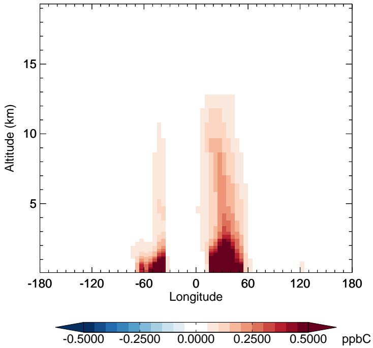
GC_12.0.0 - v11-02e-Run1 ALK4 - Diff along 15S for Jan
