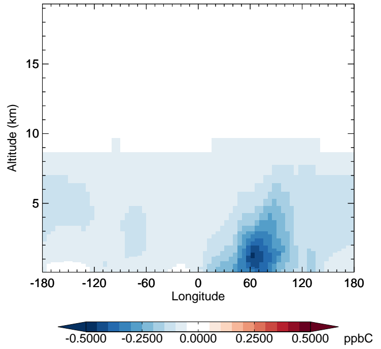
GC_12.0.0 - v11-02f-Run1 ACET - Diff along 42N for Jan
