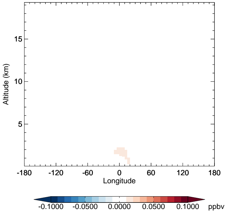
GC_12.0.0 - v11-02f-Run1 SOAME - Diff along 15S for Jan
