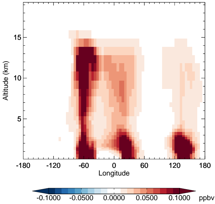
GC_12.0.0 - v11-02f-Run1 HCOOH - Diff along 15S for Jan
