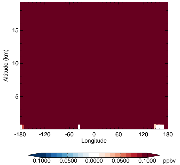
GC_12.0.0 - v11-02e-Run1 CH4 - Diff along 42N for Jan
