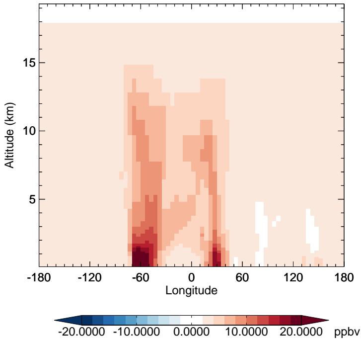
GC_12.0.0 - v11-02f-Run1 CO - Diff along 15S for Jan
