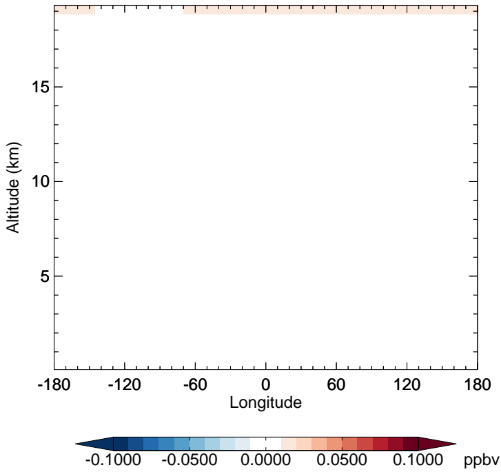
GC_12.0.0 - v11-02f-Run1 CFC12 - Diff along 15S for Jan
