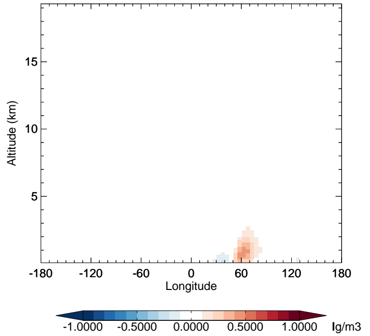
GC_12.0.0 - v11-02f-Run1 SOAS - Diff along 42N for Jan
