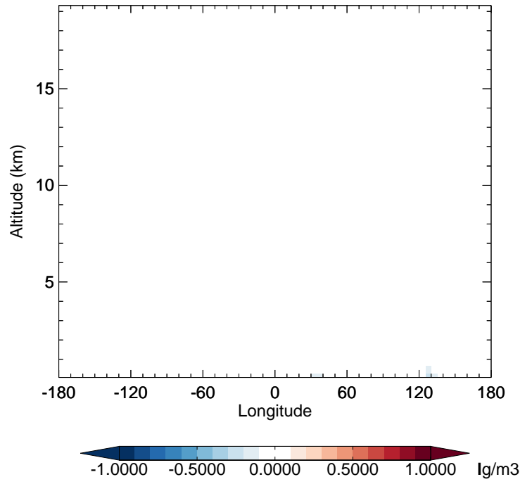
GC_12.0.0 - v11-02f-Run1 NH4 - Diff along 42N for Jan
