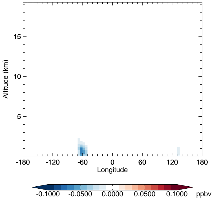
GC_12.0.0 - v11-02f-Run1 HPALD - Diff along 15S for Jan
