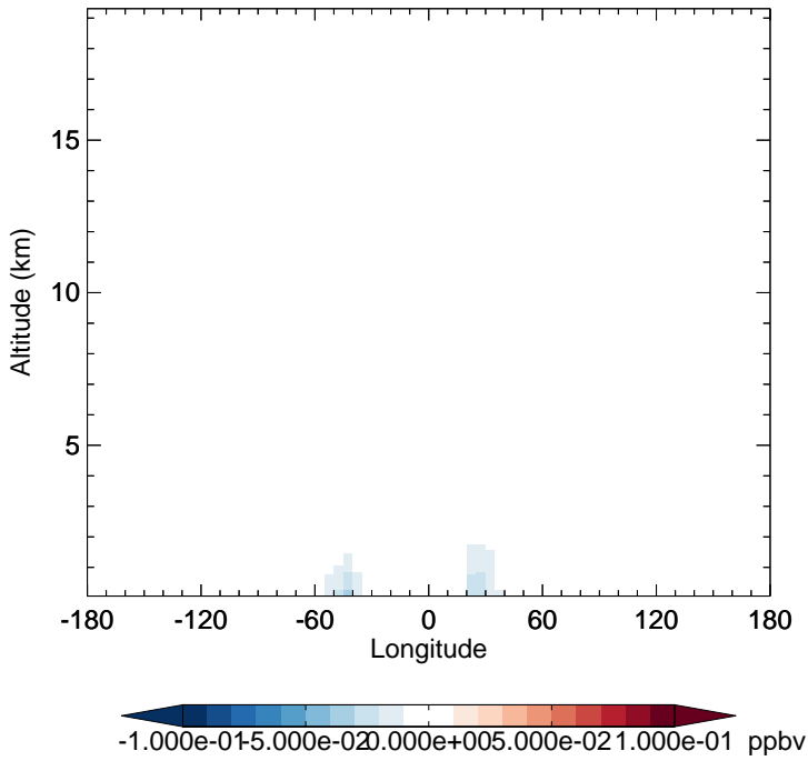
GC_12.0.0 - v11-02e-Run1 MONITA - Diff along 15S for Jan
