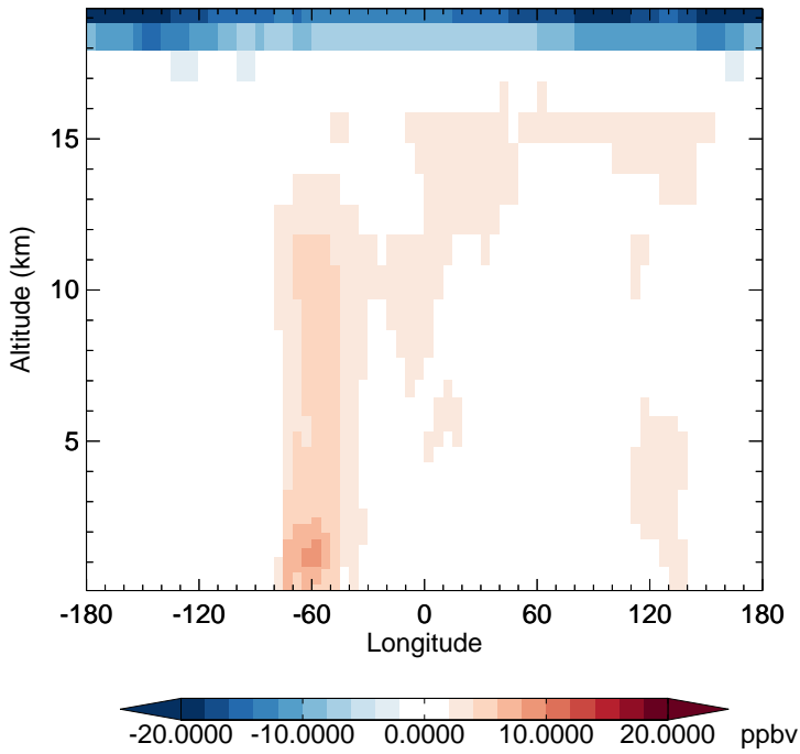
GC_12.0.0 - v11-02e-Run1 O3 - Diff along 15S for Jan
