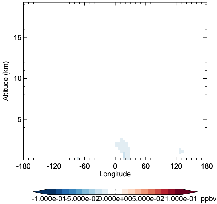
GC_12.0.0 - v11-02e-Run1 SOAME - Diff along 15S for Jan
