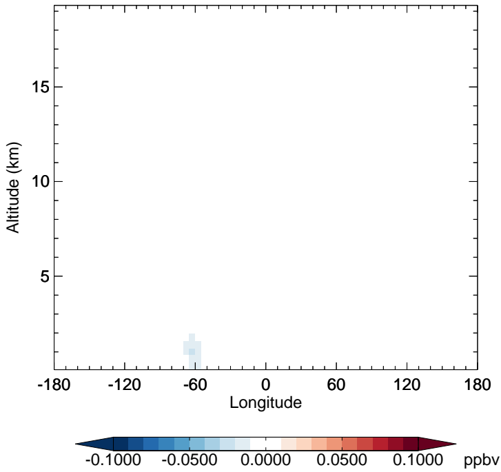
GC_12.0.0 - v11-02e-Run1 RIPD - Diff along 15S for Jan
