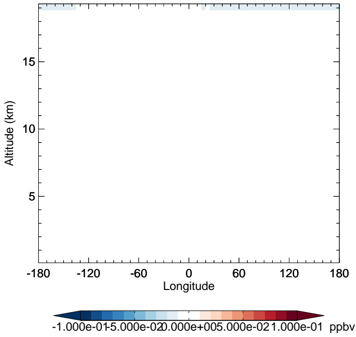
GC_12.0.0 - v11-02f-Run1 CINO3 - Diff along 15S for Jan
