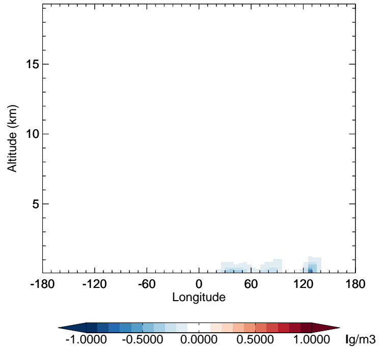
GC_12.0.0 - v11-02f-Run1 NIT - Diff along 42N for Jan
