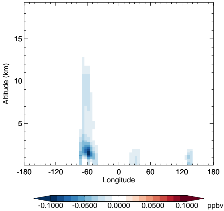
GC_12.0.0 - v11-02e-Run1 IPMN - Diff along 15S for Jan
