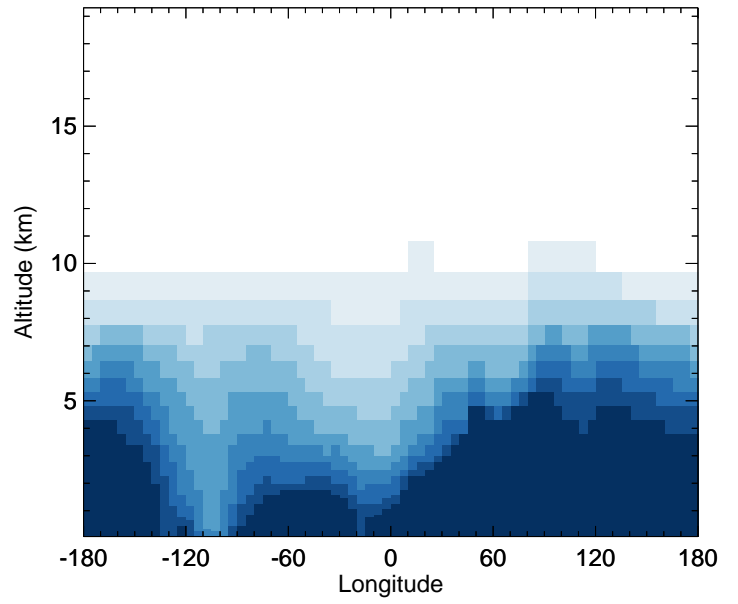
GC_12.0.0 - v11-02f-Run1 C3H8 - Diff along 42N for Jan
