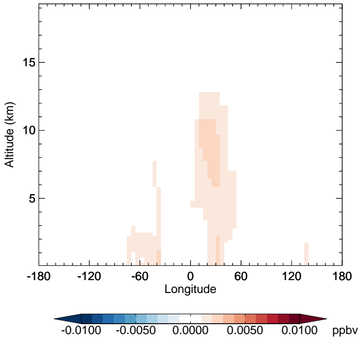
GC_12.0.0 - v11-02e-Run1 R4N2 - Diff along 15S for Jan
