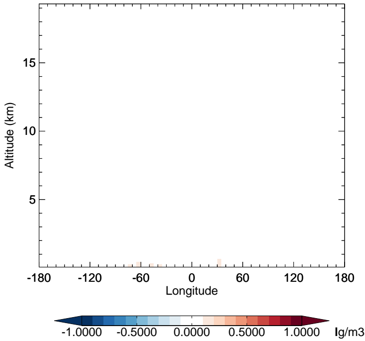
GC_12.0.0 - v11-02e-Run1 NH3 - Diff along 15S for Jan
