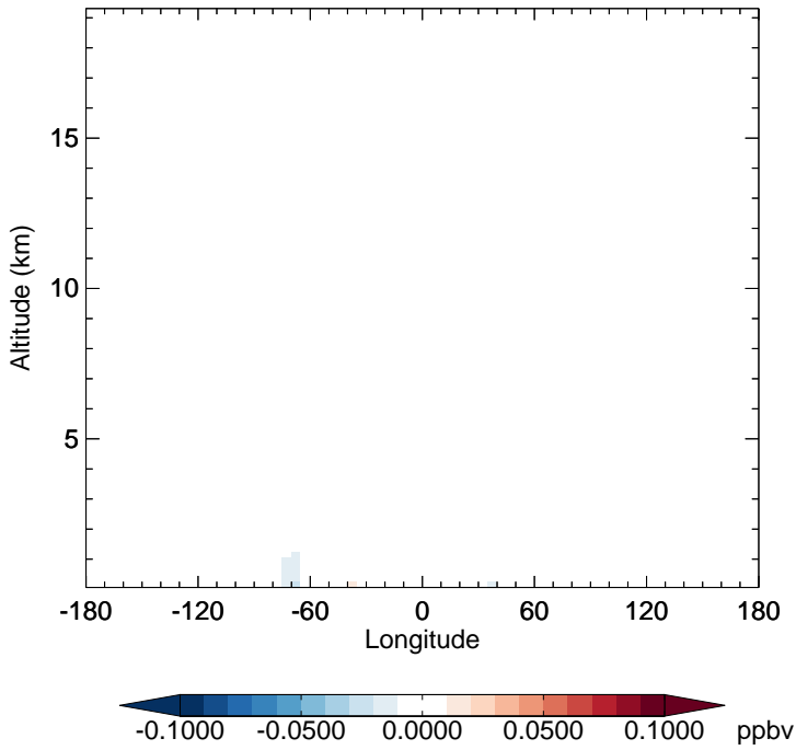
GC_12.0.0 - v11-02e-Run1 XYLE - Diff along 15S for Jan
