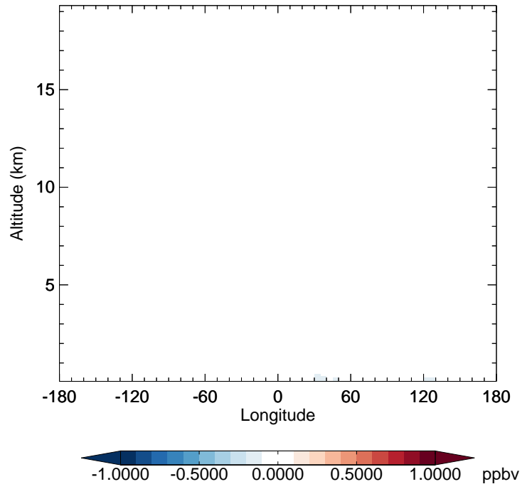
GC_12.0.0 - v11-02f-Run1 NO2 - Diff along 42N for Jan
