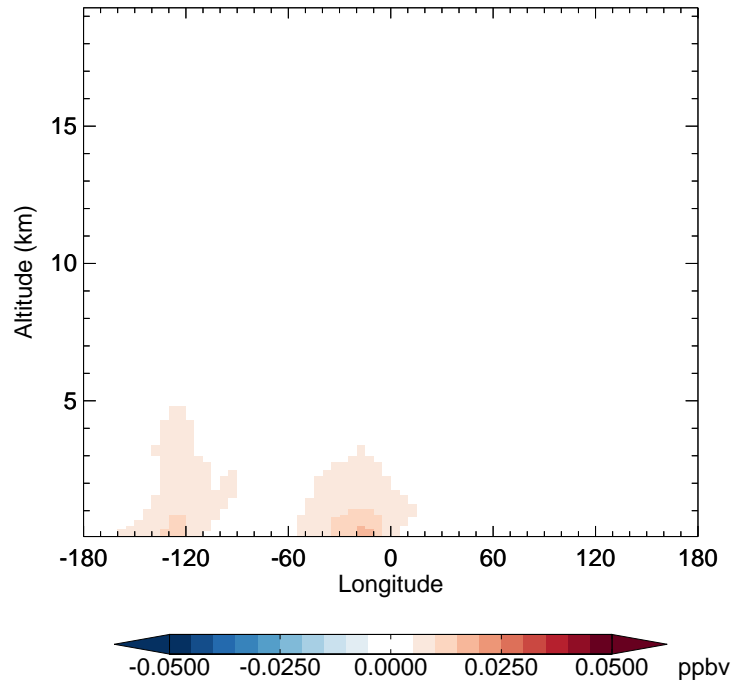
GC_12.0.0 - v11-02f-Run1 MP - Diff along 42N for Jan
