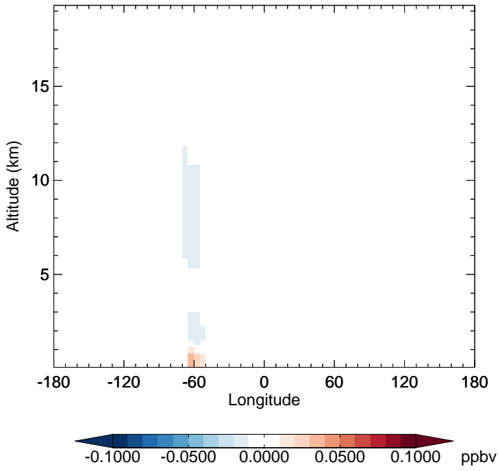
GC_12.0.0 - v11-02f-Run1 HAC - Diff along 15S for Jan
