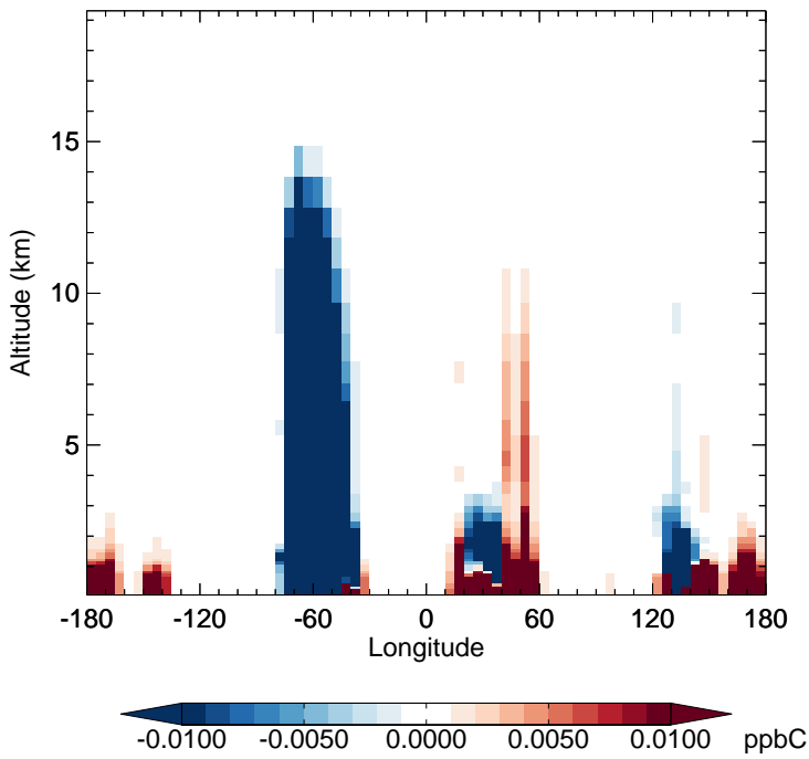
GC_12.0.0 - v11-02e-Run1 PRPE - Diff along 15S for Jan
