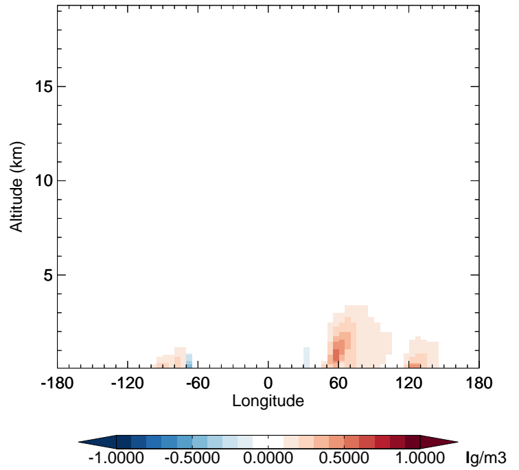
GC_12.0.0 - v11-02e-Run1 SO 2 - Diff along 42N for Jan
