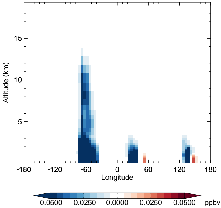
GC_12.0.0 - v11-02e-Run1 MVK - Diff along 15S for Jan
