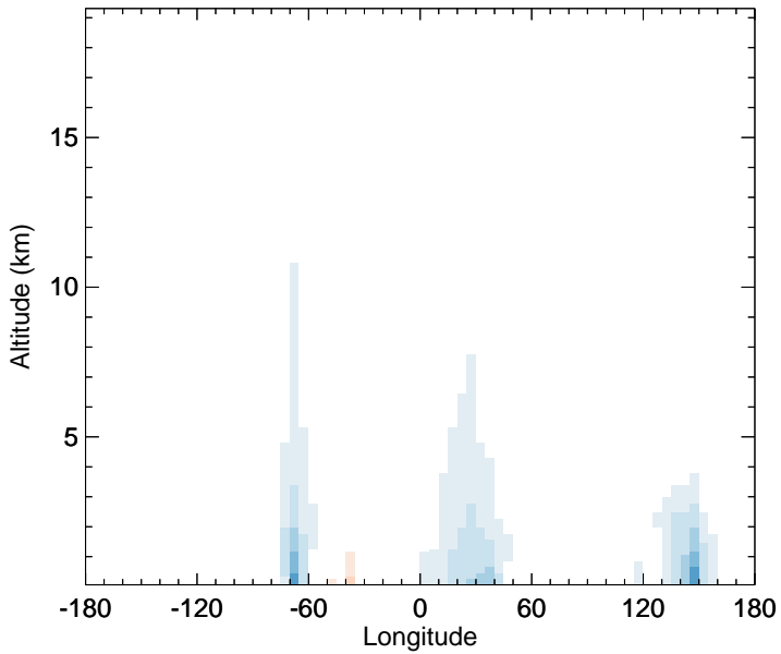
GC_12.0.0 - v11-02e-Run1 C3H8 - Diff along 15S for Jan
