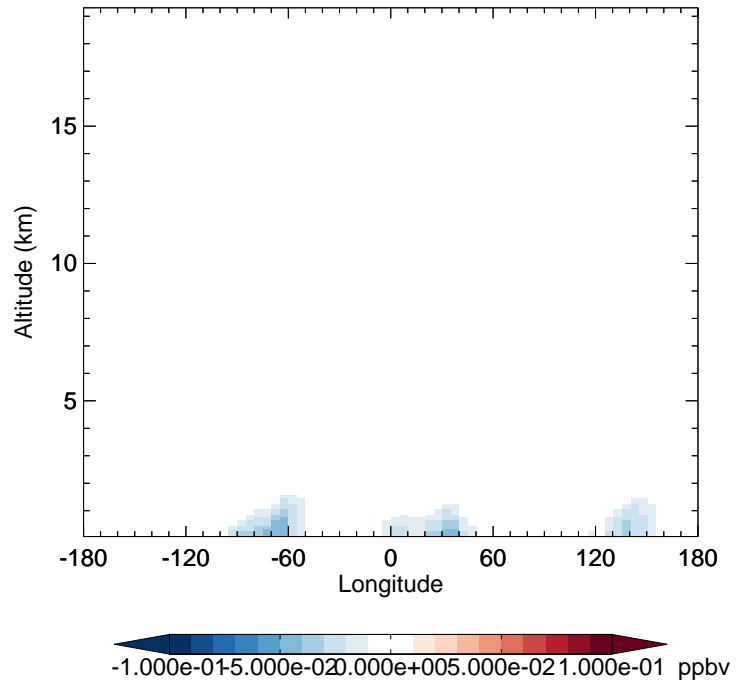
GC_12.0.0 - v11-02e-Run1 CINO2 - Diff along 42N for Jan
