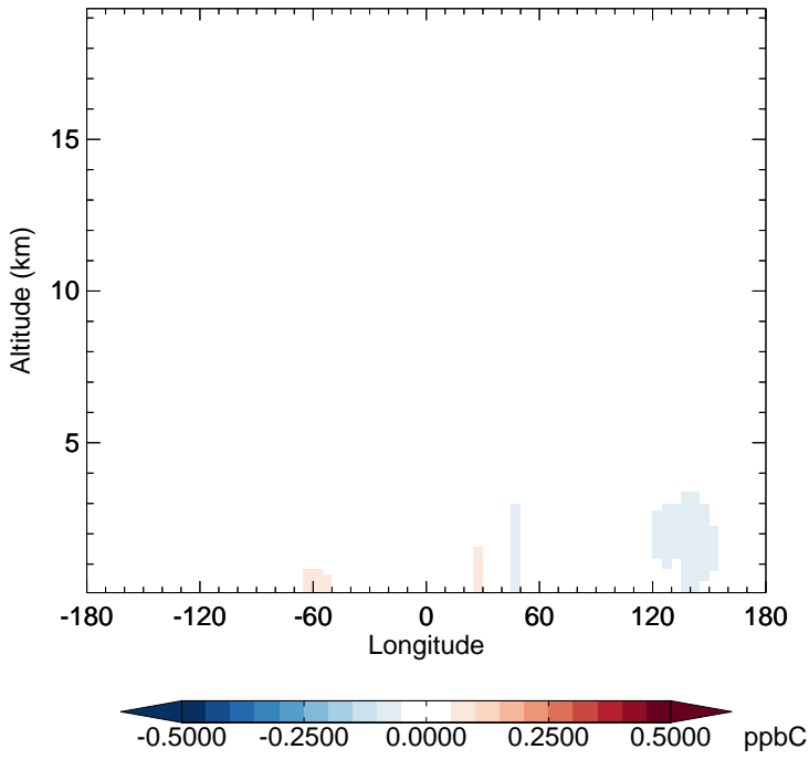
GC_12.0.0 - v11-02f-Run1 ACET - Diff along 15S for Jan
