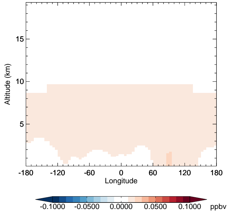
GC_12.0.0 - v11-02f-Run1 ACTA - Diff along 42N for Jan
