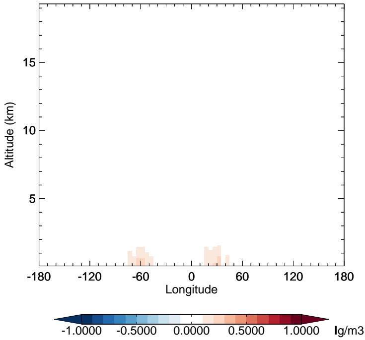
GC_12.0.0 - v11-02f-Run1 SOAS - Diff along 15S for Jan
