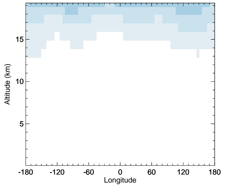
GC_12.0.0 - v11-02e-Run1 BrNO3 - Diff along 42N for Jan
