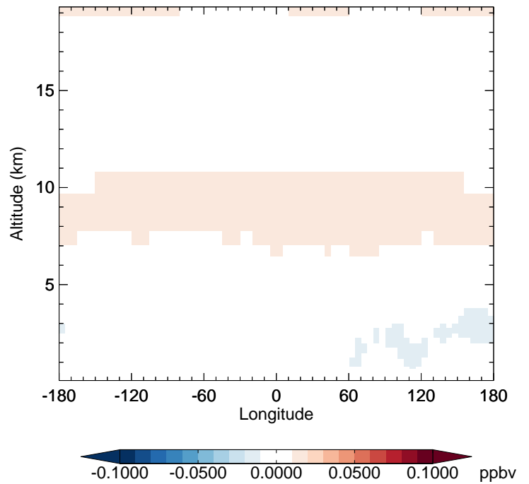
GC_12.0.0 - v11-02e-Run1 H2O2 - Diff along 42N for Jan
