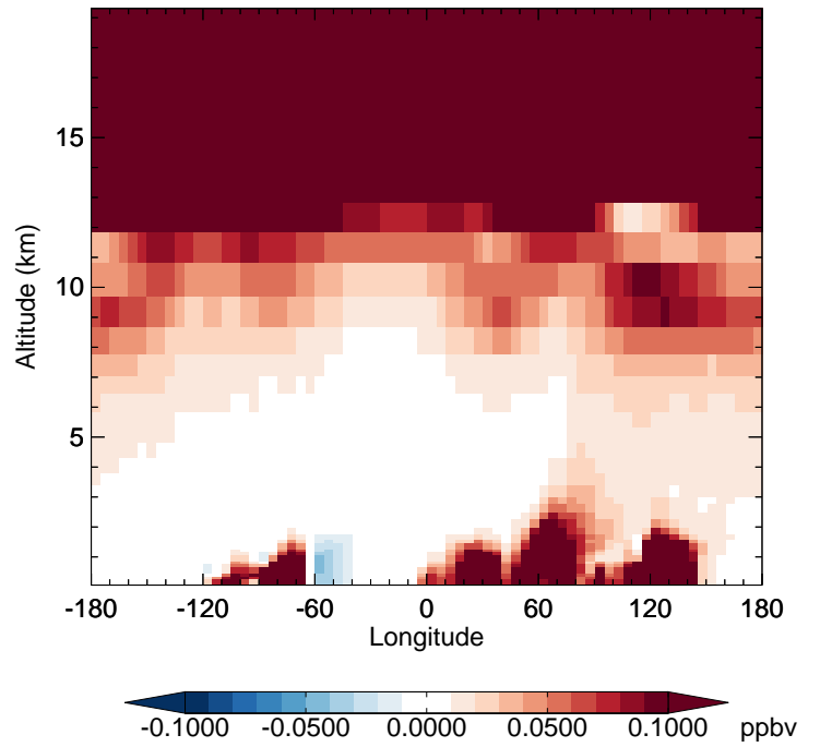
GC_12.0.0 - v11-02e-Run1 HNO 3 - Diff along 42N for Jan
