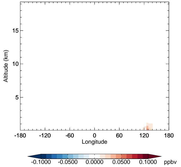
GC_12.0.0 - v11-02f-Run1 XYLE - Diff along 42N for Jan
