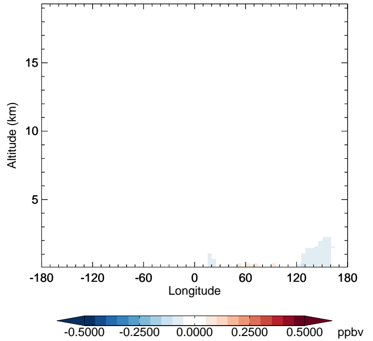
GC_12.0.0 - v11-02e-Run1 CH 2 O - Diff along 42N for Jan
