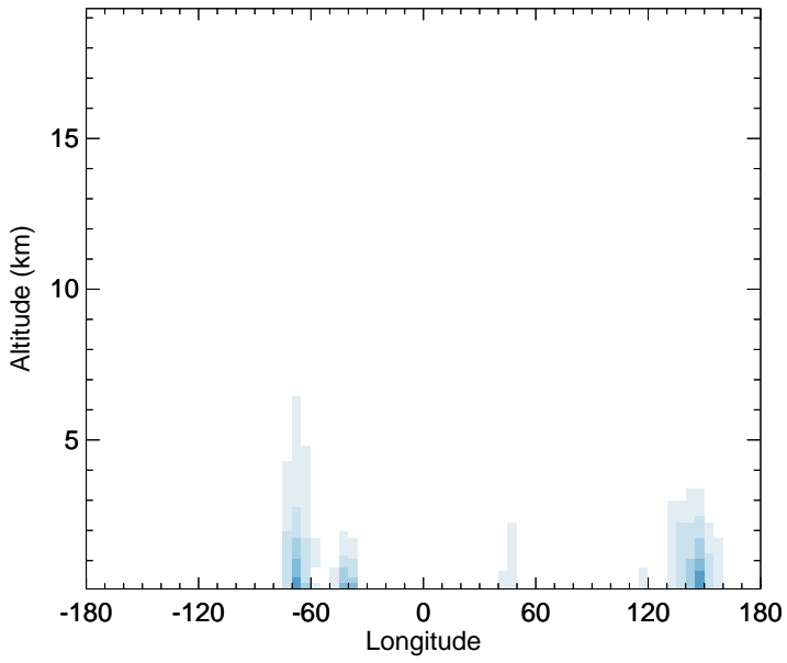
GC_12.0.0 - v11-02f-Run1 C3H8 - Diff along 15S for Jan
