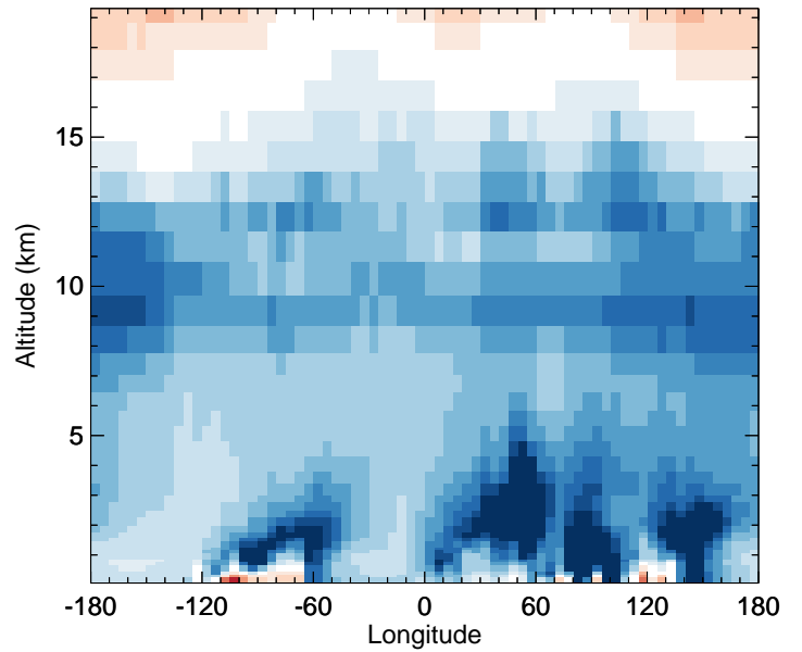
GC_12.0.0 - v11-02e-Run1 OH - Diff along 42N for Jan
