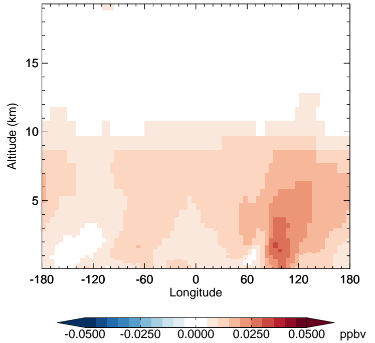
GC_12.0.0 - v11-02e-Run1 MP - Diff along 42N for Jan
