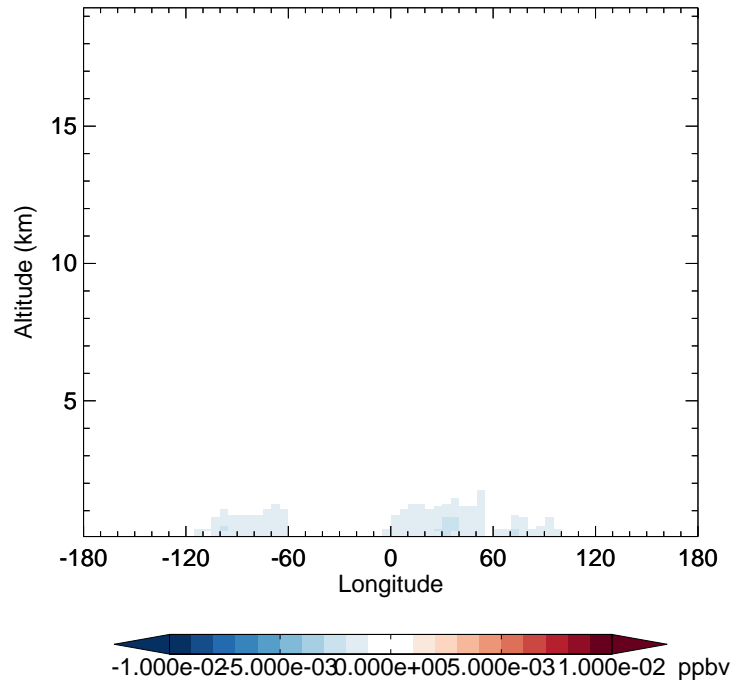
GC_12.0.0 - v11-02e-Run1 NO3 - Diff along 42N for Jan
