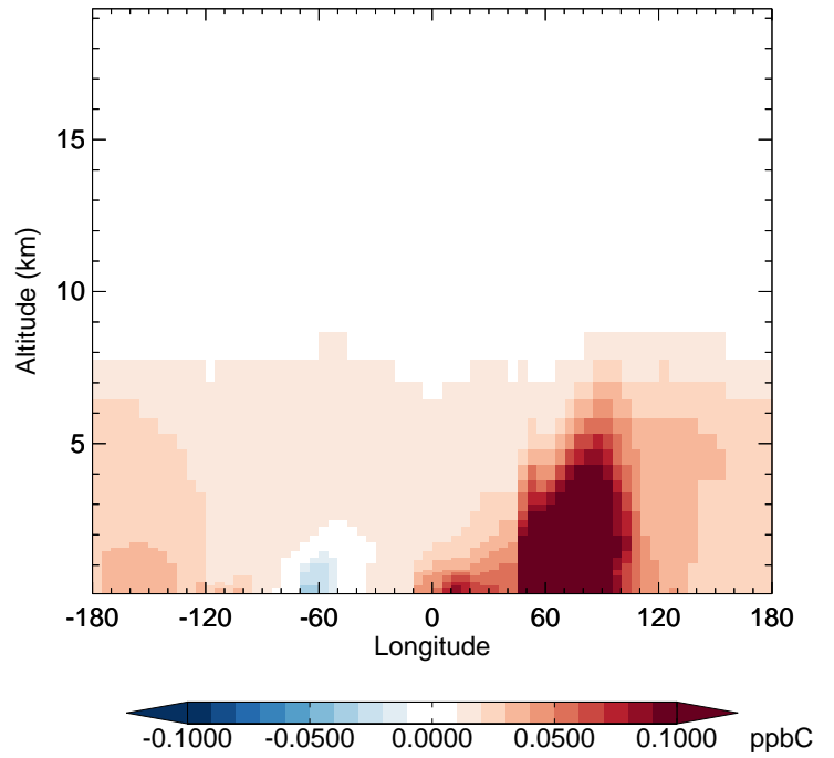
GC_12.0.0 - v11-02e-Run1 MEK - Diff along 42N for Jan
