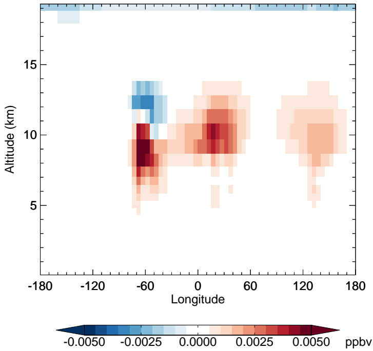
GC_12.0.0 - v11-02e-Run1 HNO 4 - Diff along 15S for Jan
