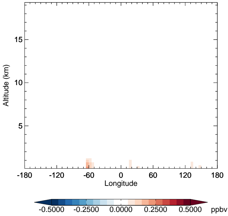
GC_12.0.0 - v11-02f-Run1 CH 2 O - Diff along 15S for Jan
