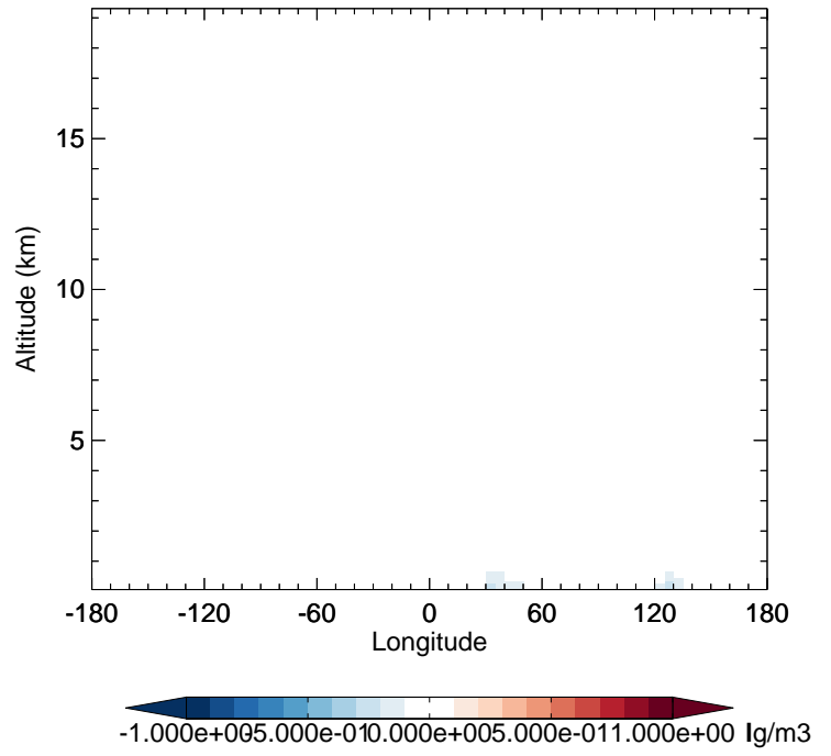
GC_12.0.0 - v11-02f-Run1 OCPO - Diff along 42N for Jan
