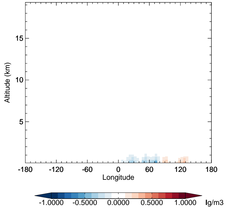
GC_12.0.0 - v11-02e-Run1 OCPI - Diff along 42N for Jan
