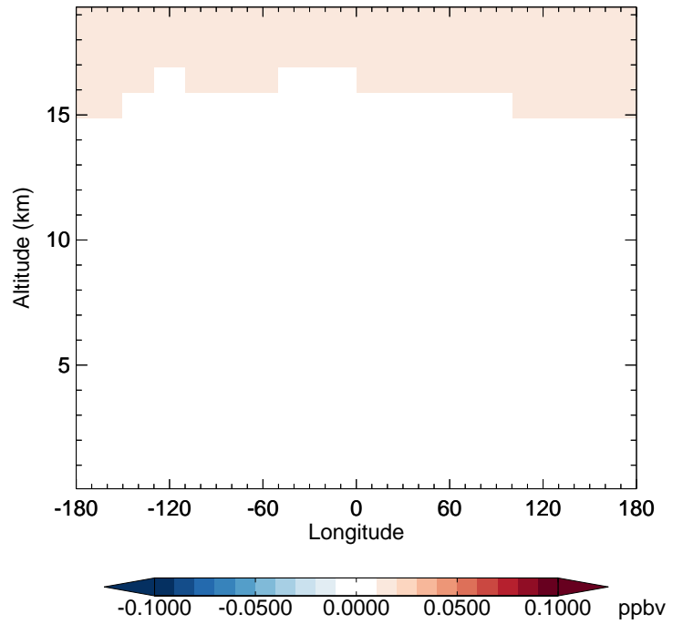
GC_12.0.0 - v11-02e-Run1 CFC12 - Diff along 42N for Jan
