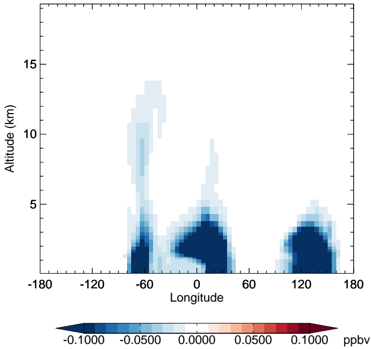
GC_12.0.0 - v11-02e-Run1 SOAIE - Diff along 15S for Jan
