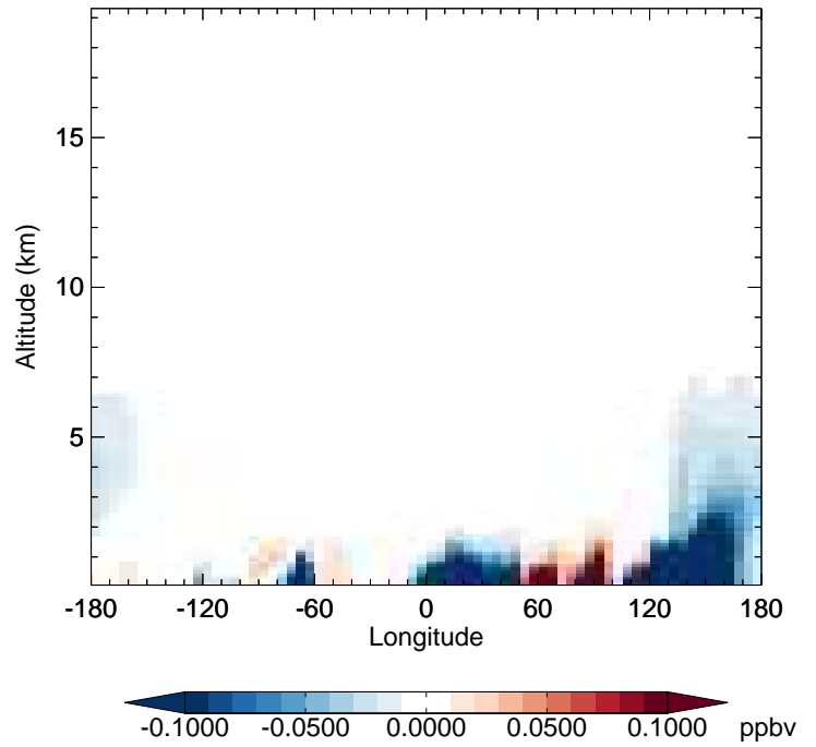
GC_12.0.0 - v11-02e-Run1 XYLE - Diff along 42N for Jan
