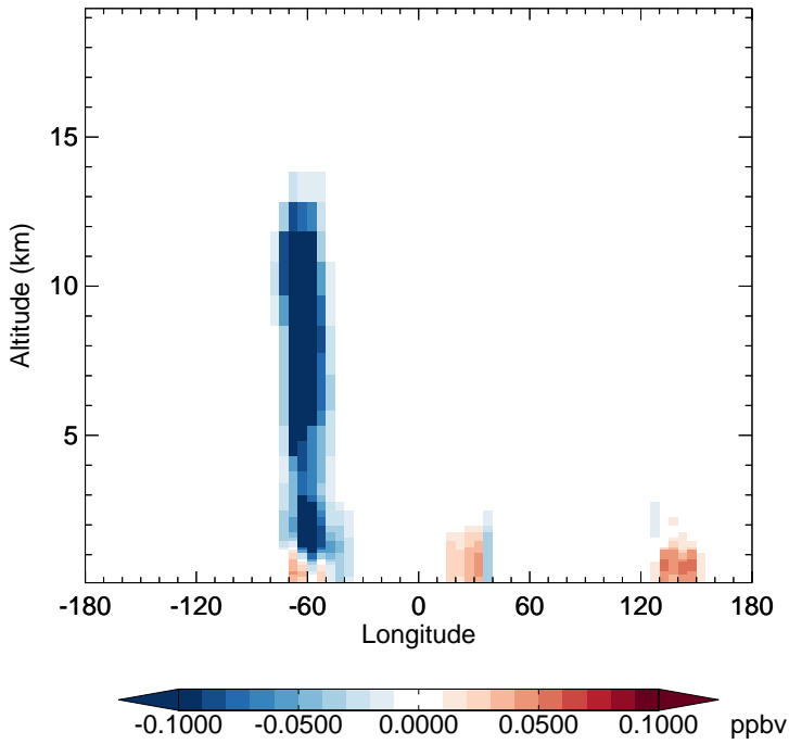
GC_12.0.0 - v11-02e-Run1 IEPOXA - Diff along 15S for Jan
