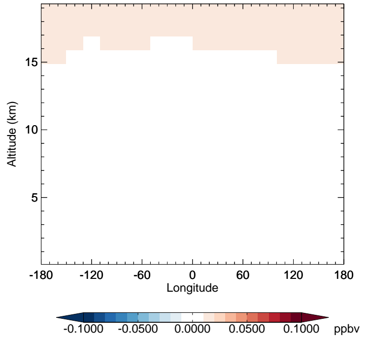
GC_12.0.0 - v11-02f-Run1 CFC12 - Diff along 42N for Jan
