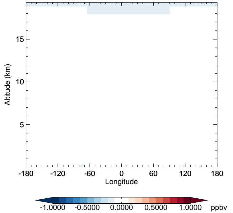
GC_12.0.0 - v11-02e-Run1 NO - Diff along 42N for Jan
