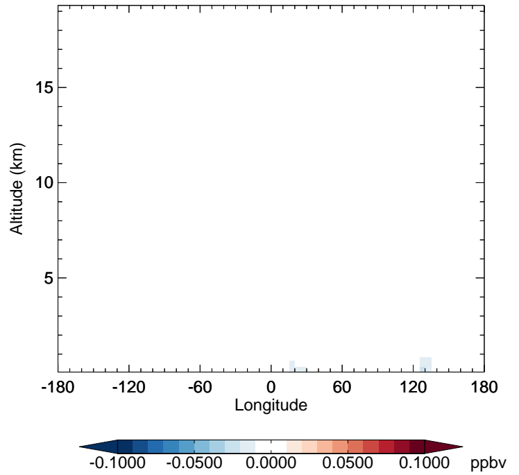
GC_12.0.0 - v11-02e-Run1 SOAGX - Diff along 42N for Jan
