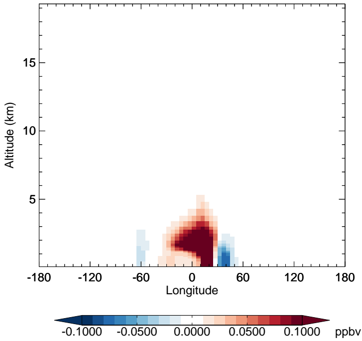
GC_12.0.0 - v11-02f-Run1 SOAIE - Diff along 15S for Jan
