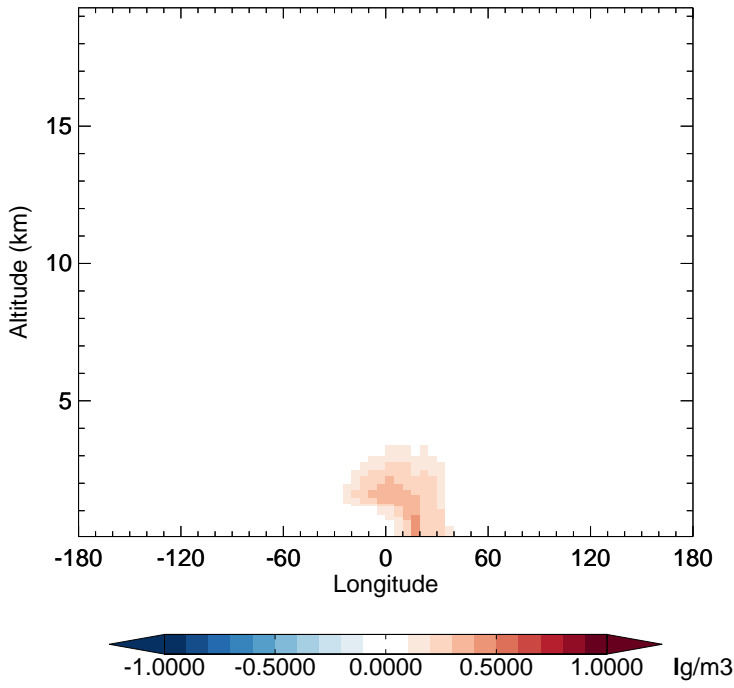
GC_12.0.0 - v11-02f-Run1 SO4 - Diff along 15S for Jan
