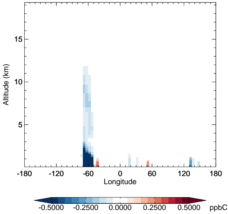
GC_12.0.0 - v11-02f-Run1 ISOP - Diff along 15S for Jan
