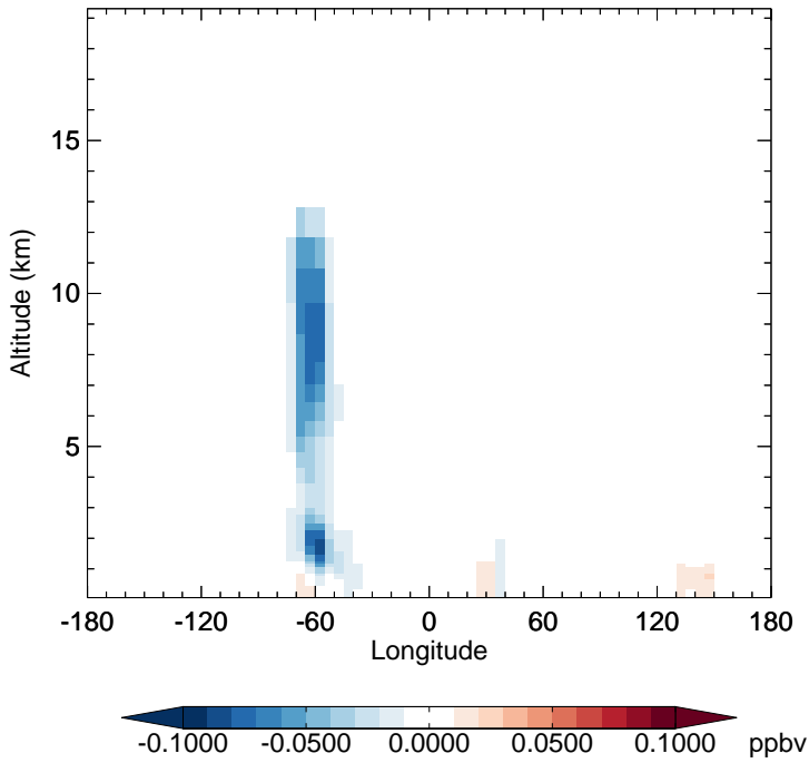
GC_12.0.0 - v11-02e-Run1 IEPOXB - Diff along 15S for Jan
