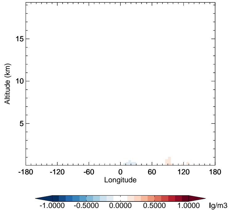
GC_12.0.0 - v11-02e-Run1 BCPI - Diff along 42N for Jan
