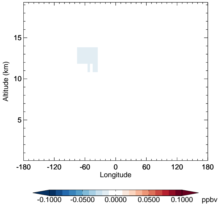
GC_12.0.0 - v11-02e-Run1 MPN - Diff along 15S for Jan
