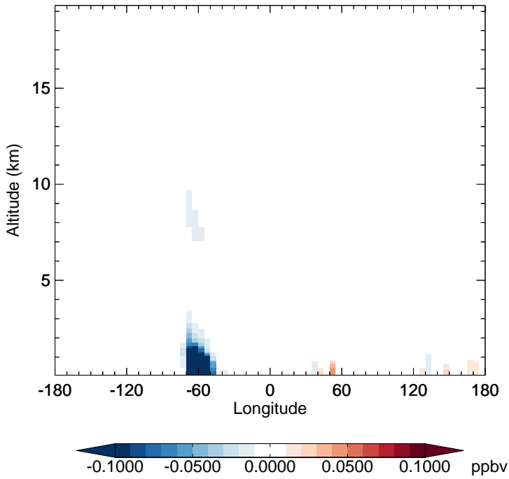
GC_12.0.0 - v11-02e-Run1 MTPA - Diff along 15S for Jan
