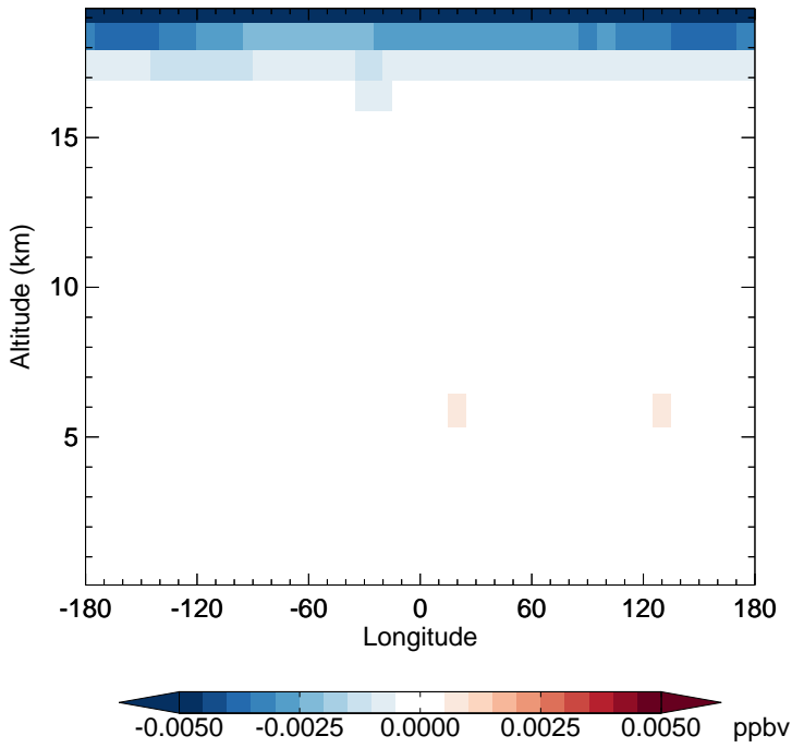
GC_12.0.0 - v11-02f-Run1 N2O5 - Diff along 15S for Jan
