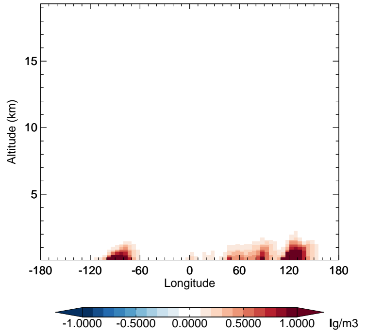
GC_12.0.0 - v11-02e-Run1 NIT - Diff along 42N for Jan
