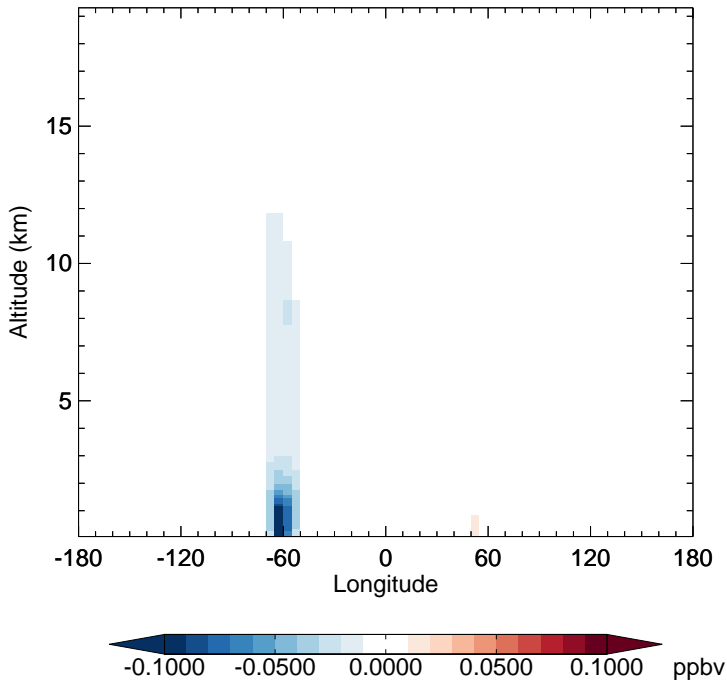
GC_12.0.0 - v11-02f-Run1 EOH - Diff along 15S for Jan
