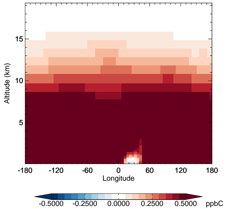
GC_12.0.0 - v11-02e-Run1 C2H6 - Diff along 42N for Jan
