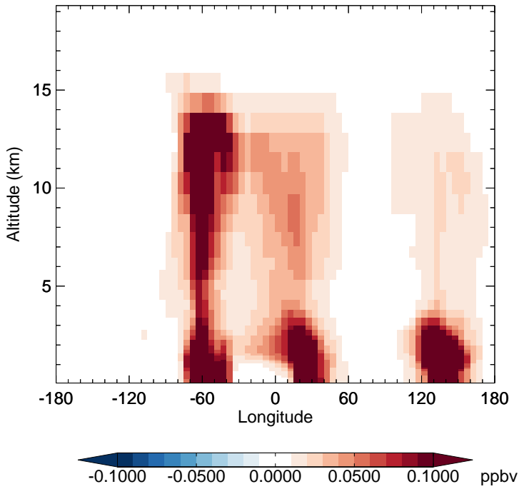
GC_12.0.0 - v11-02e-Run1 HCOOH - Diff along 15S for Jan
