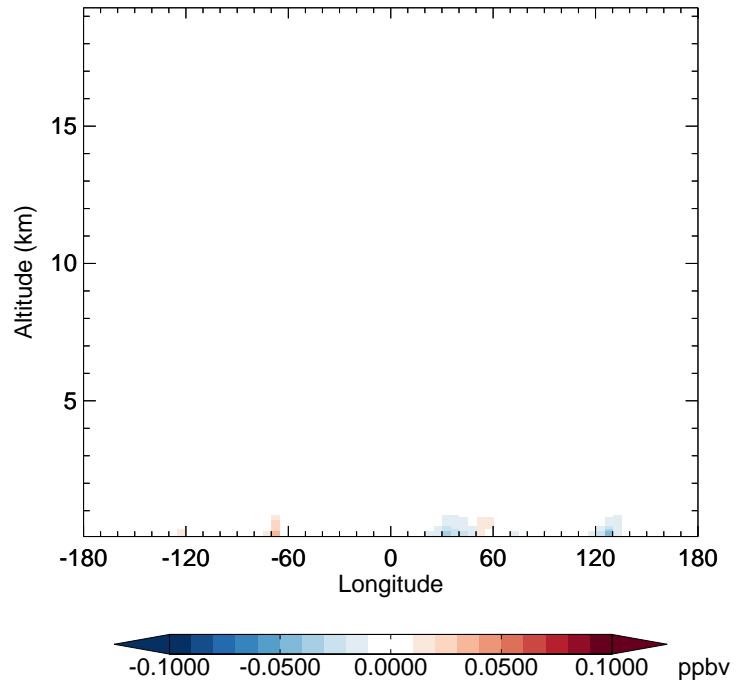
GC_12.0.0 - v11-02f-Run1 SOAP - Diff along 42N for Jan
