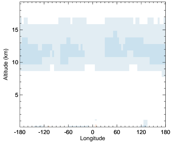
GC_12.0.0 - v11-02f-Run1 OH - Diff along 42N for Jan
