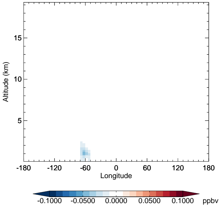
GC_12.0.0 - v11-02f-Run1 RIPA - Diff along 15S for Jan
