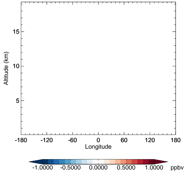
GC_12.0.0 - v11-02e-Run1 HNO 2 - Diff along 42N for Jan
