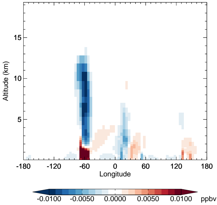
GC_12.0.0 - v11-02f-Run1 MAP - Diff along 15S for Jan
