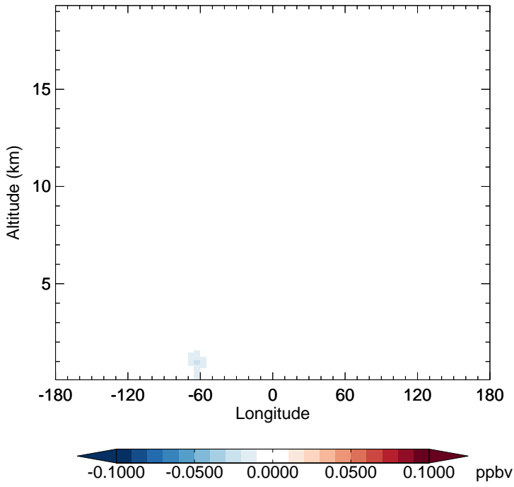
GC_12.0.0 - v11-02f-Run1 RIPB - Diff along 15S for Jan
