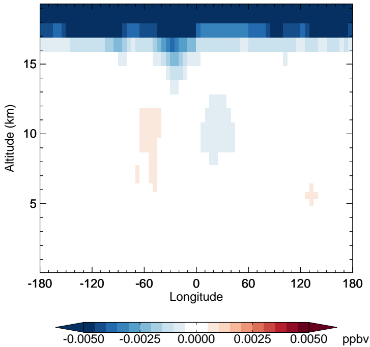
GC_12.0.0 - v11-02e-Run1 N2O5 - Diff along 15S for Jan
