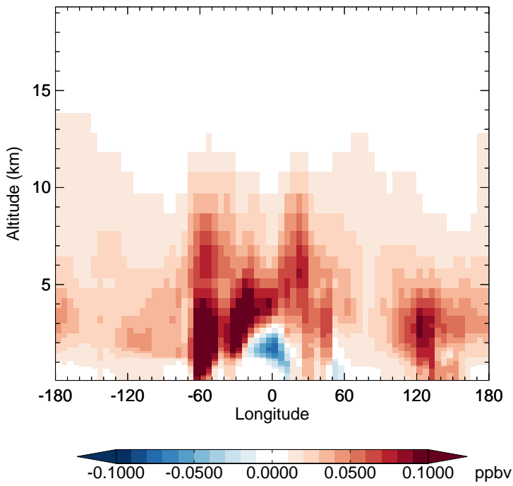
GC_12.0.0 - v11-02f-Run1 H2O2 - Diff along 15S for Jan
