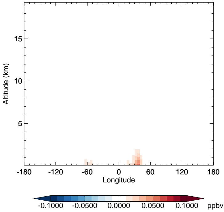
GC_12.0.0 - v11-02f-Run1 TOLU - Diff along 15S for Jan
