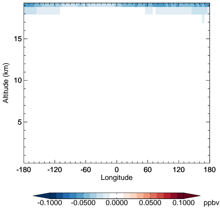
GC_12.0.0 - v11-02f-Run1 H2O - Diff along 15S for Jan
