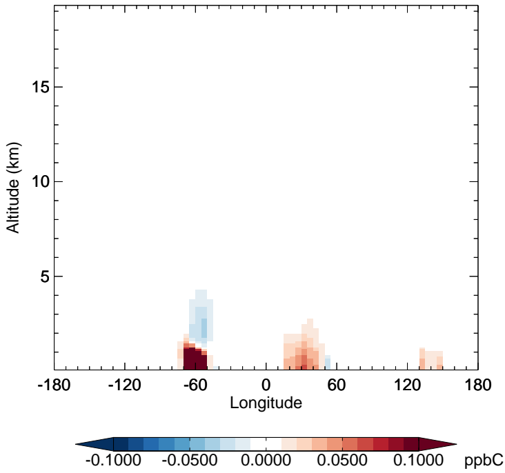
GC_12.0.0 - v11-02f-Run1 MEK - Diff along 15S for Jan
