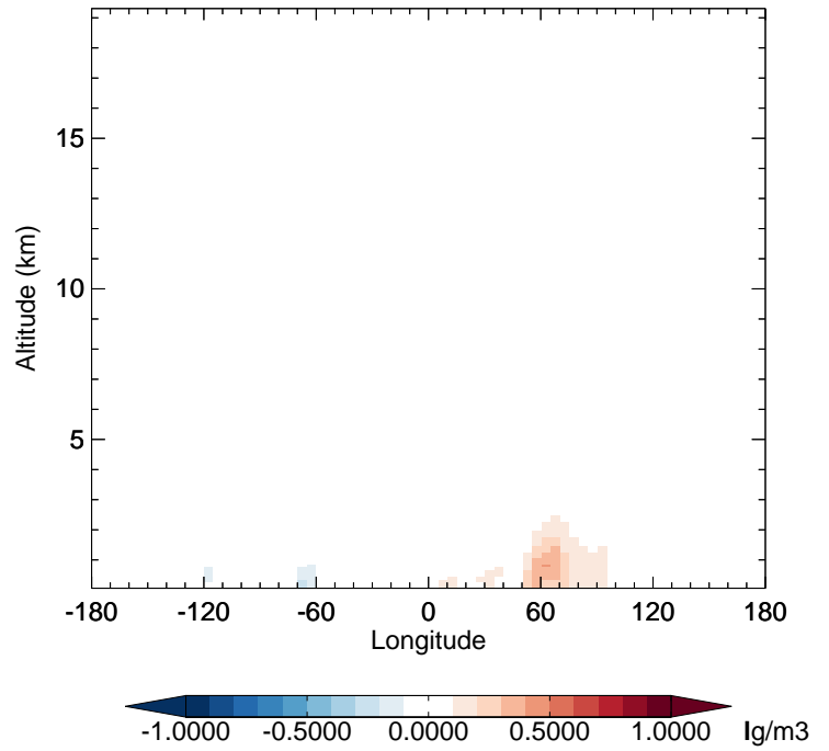
GC_12.0.0 - v11-02e-Run1 SOAS - Diff along 42N for Jan
