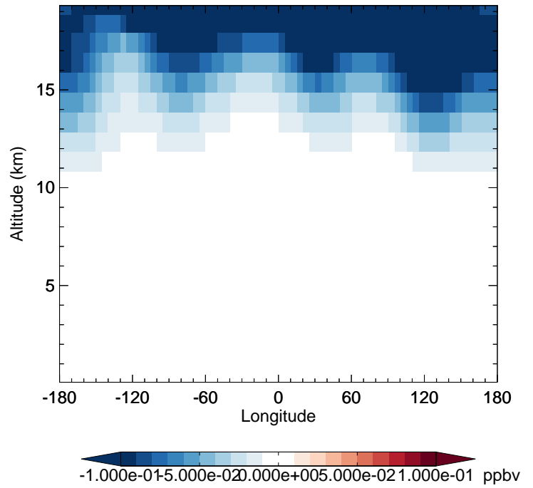
GC_12.0.0 - v11-02e-Run1 CINO3 - Diff along 42N for Jan
