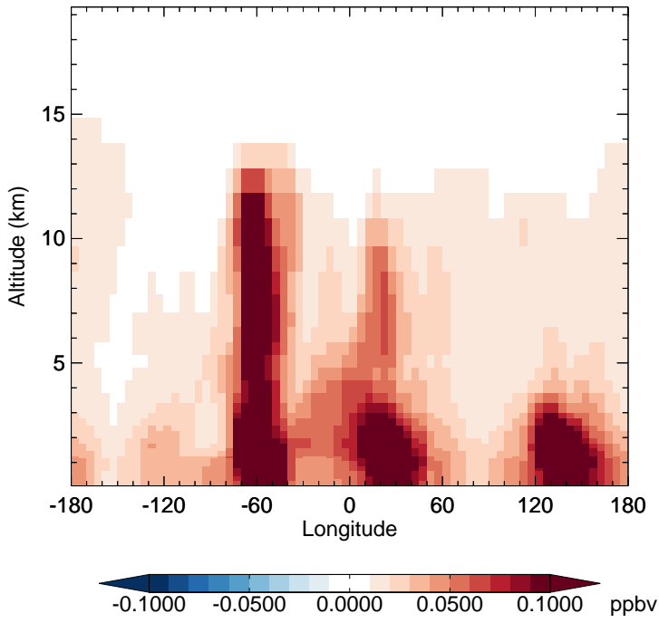
GC_12.0.0 - v11-02f-Run1 ACTA - Diff along 15S for Jan
