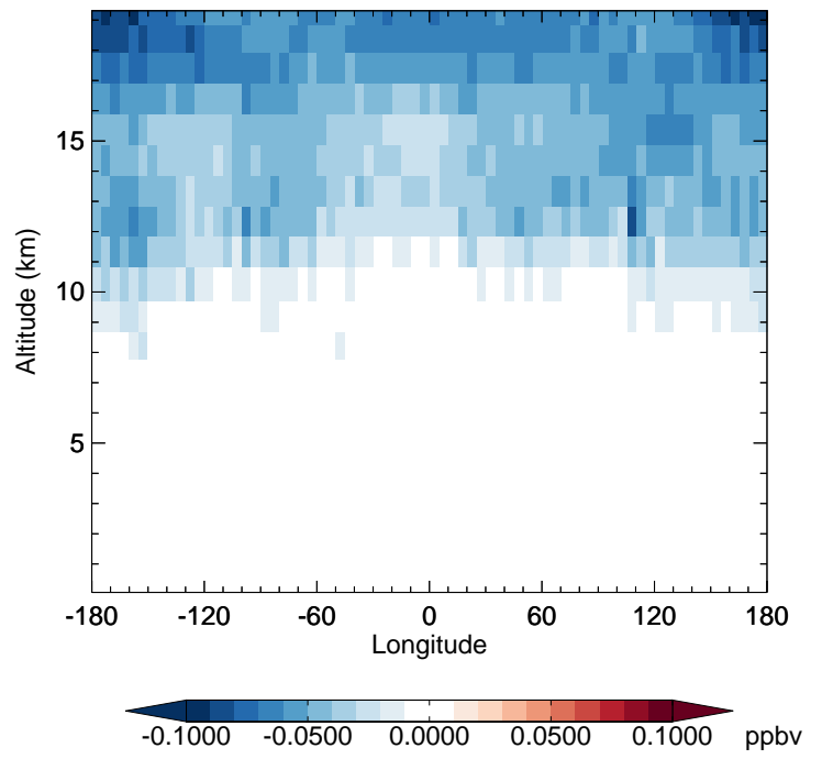
GC_12.0.0 - v11-02f-Run1 H2O - Diff along 42N for Jan
