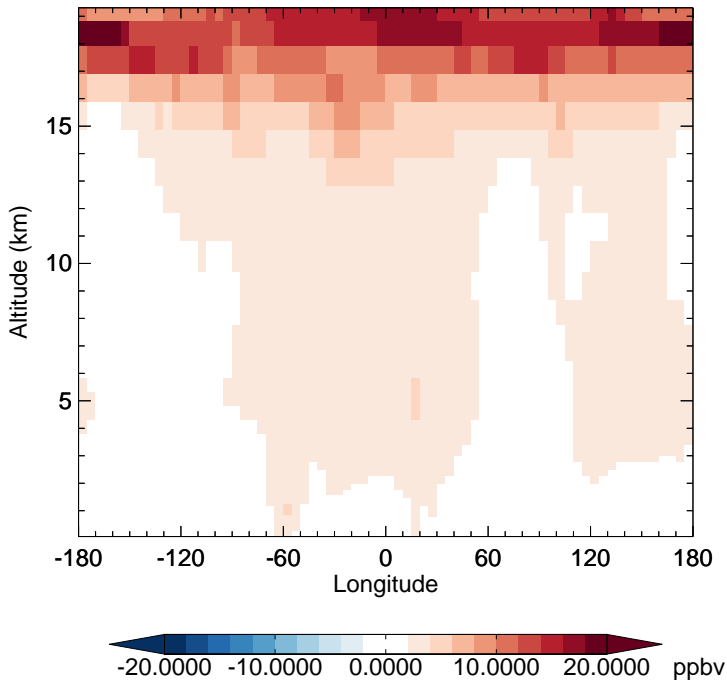
GC_12.0.0 - v11-02f-Run1 O3 - Diff along 15S for Jan
