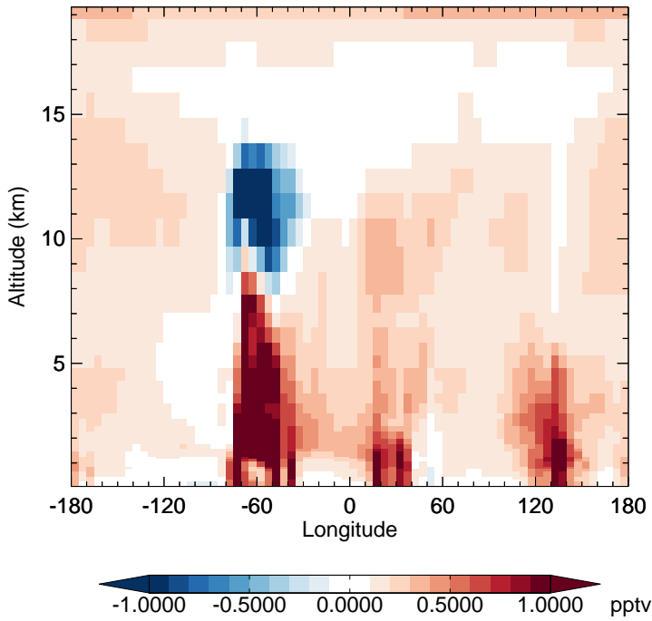
GC_12.0.0 - v11-02e-Run1 HO2 - Diff along 15S for Jan
