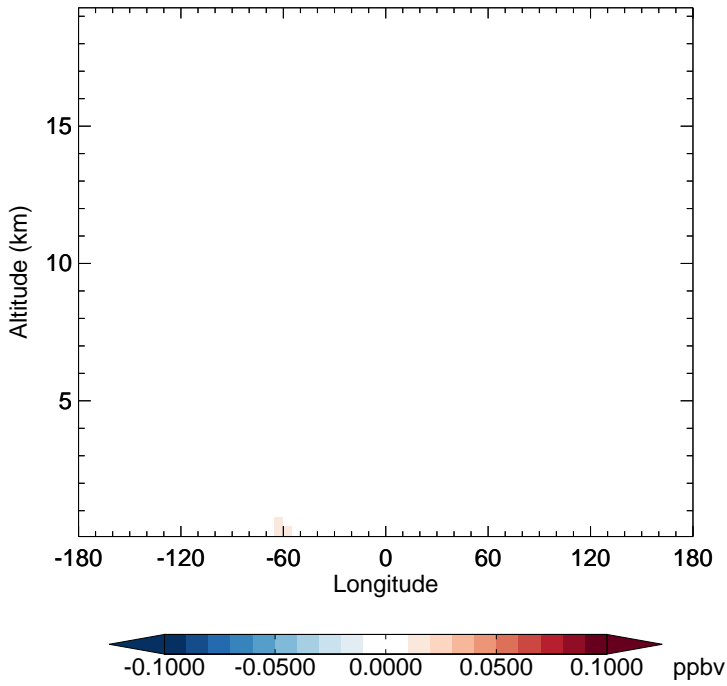
GC_12.0.0 - v11-02f-Run1 ISO3 - Diff along 15S for Jan
