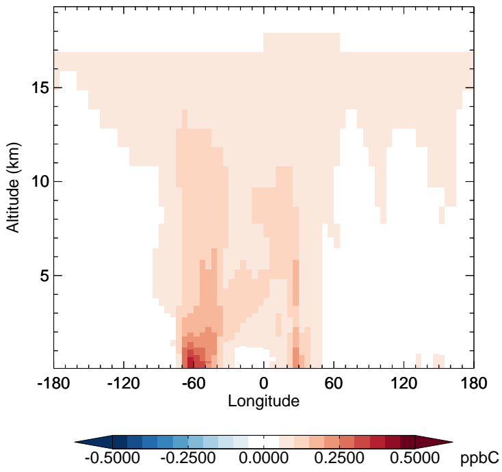
GC_12.0.0 - v11-02f-Run1 C2H6 - Diff along 15S for Jan
