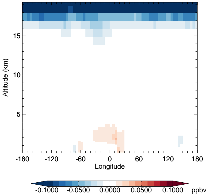
GC_12.0.0 - v11-02f-Run1 HNO 3 - Diff along 15S for Jan
