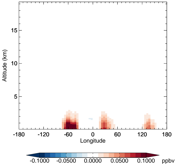
GC_12.0.0 - v11-02e-Run1 INDIOL - Diff along 15S for Jan
