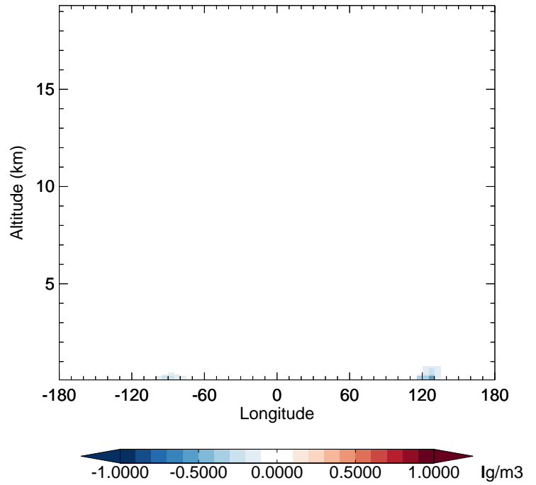
GC_12.0.0 - v11-02e-Run1 NH3 - Diff along 42N for Jan
