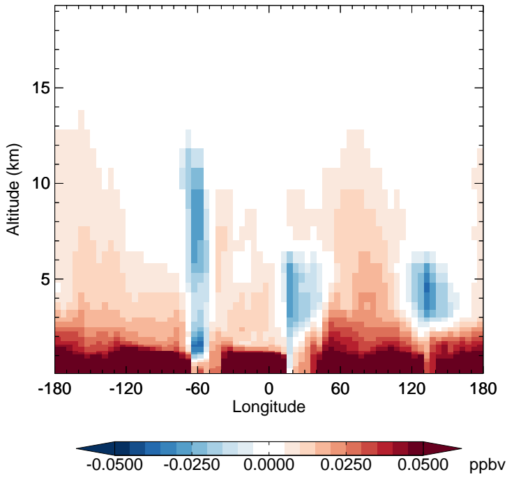
GC_12.0.0 - v11-02f-Run1 MP - Diff along 15S for Jan
