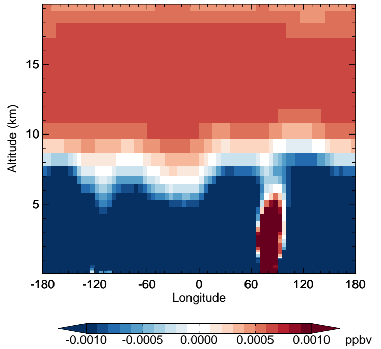
GC_12.0.0 - v11-02e-Run1 PPN - Diff along 42N for Jan
