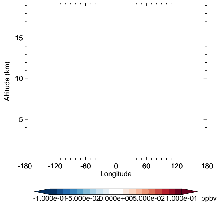
GC_12.0.0 - v11-02f-Run1 ISOA1 - Diff along 42N for Jan
