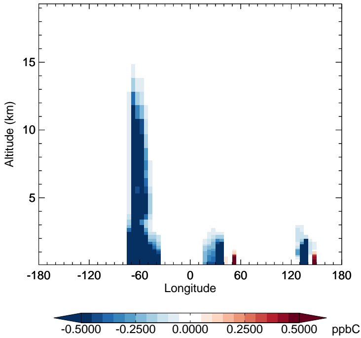
GC_12.0.0 - v11-02e-Run1 ISOP - Diff along 15S for Jan
