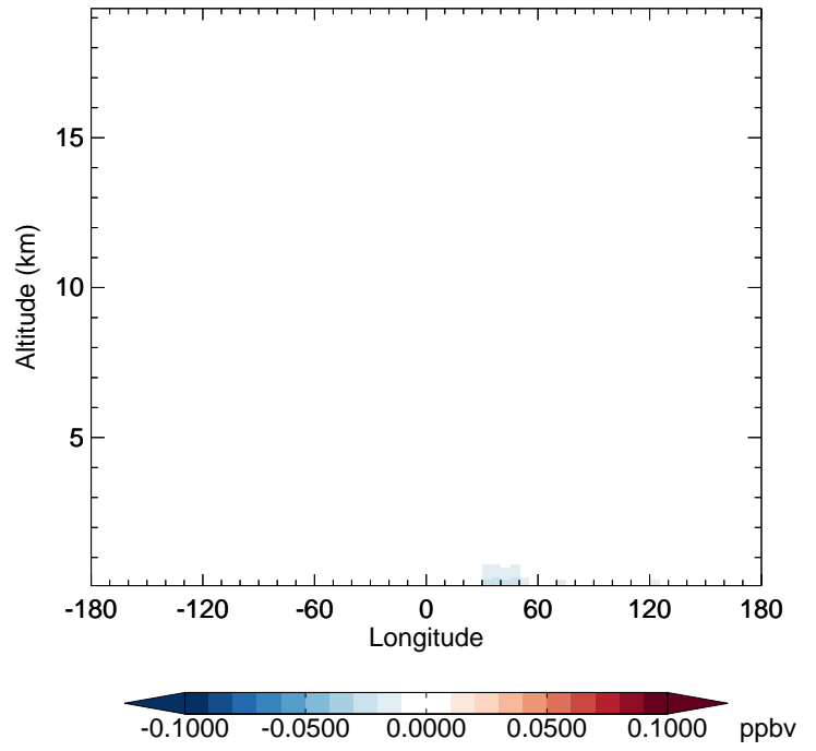
GC_12.0.0 - v11-02f-Run1 TOLU - Diff along 42N for Jan
