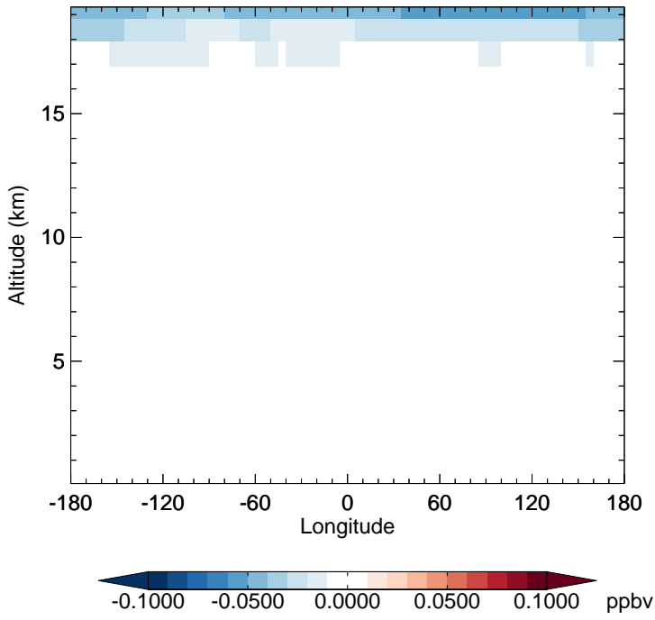
GC_12.0.0 - v11-02f-Run1 HCl - Diff along 15S for Jan
