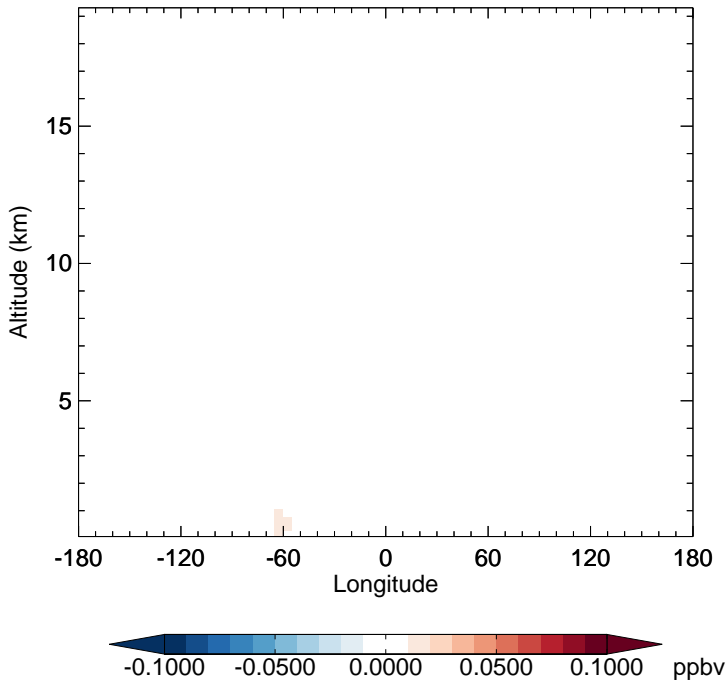
GC_12.0.0 - v11-02f-Run1 IMAE - Diff along 15S for Jan
