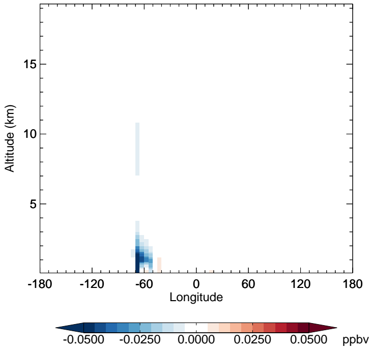
GC_12.0.0 - v11-02f-Run1 MACR - Diff along 15S for Jan
