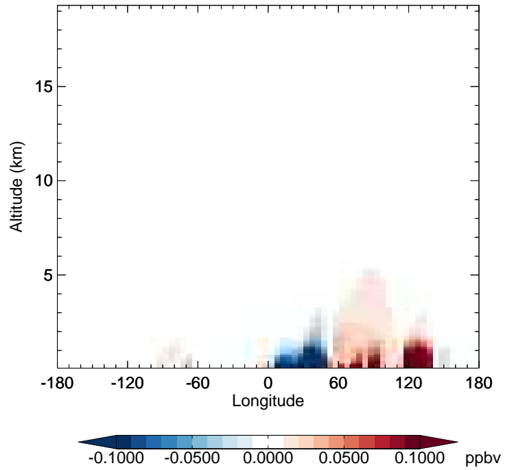
GC_12.0.0 - v11-02e-Run1 EOH - Diff along 42N for Jan
