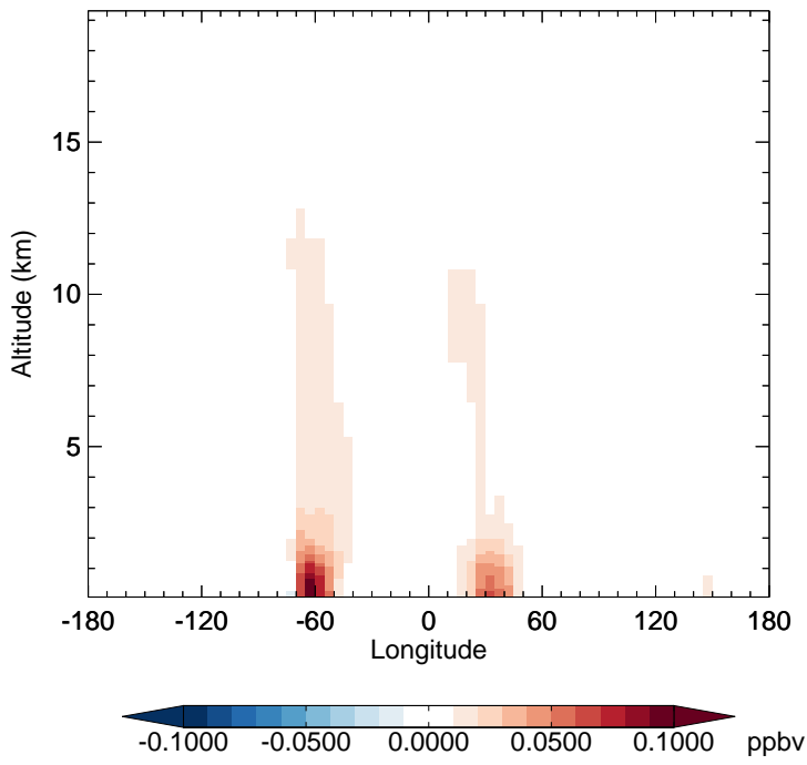
GC_12.0.0 - v11-02f-Run1 BENZ - Diff along 15S for Jan
