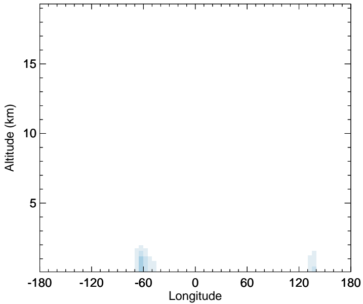
GC_12.0.0 - v11-02e-Run1 MOBA - Diff along 15S for Jan
