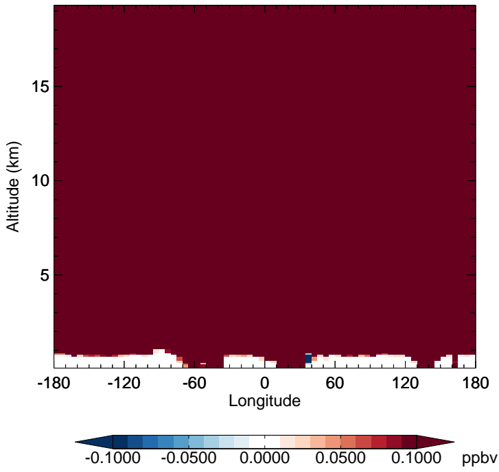
GC_12.0.0 - v11-02f-Run1 CH4 - Diff along 15S for Jan
