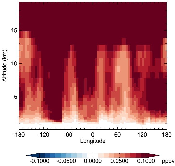
GC_12.0.0 - v11-02f-Run1 N2O - Diff along 15S for Jan
