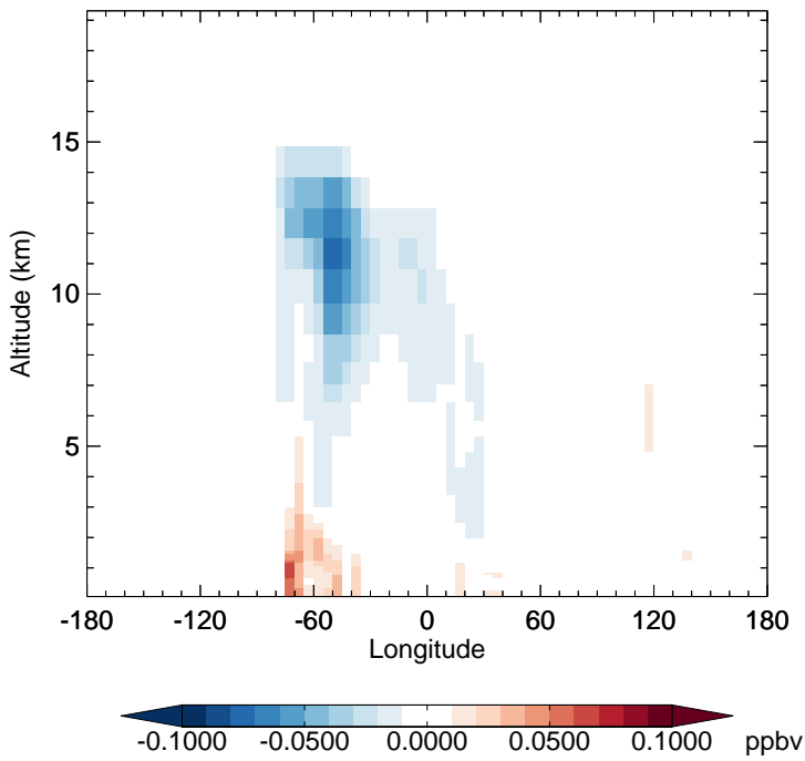
GC_12.0.0 - v11-02e-Run1 PAN - Diff along 15S for Jan
