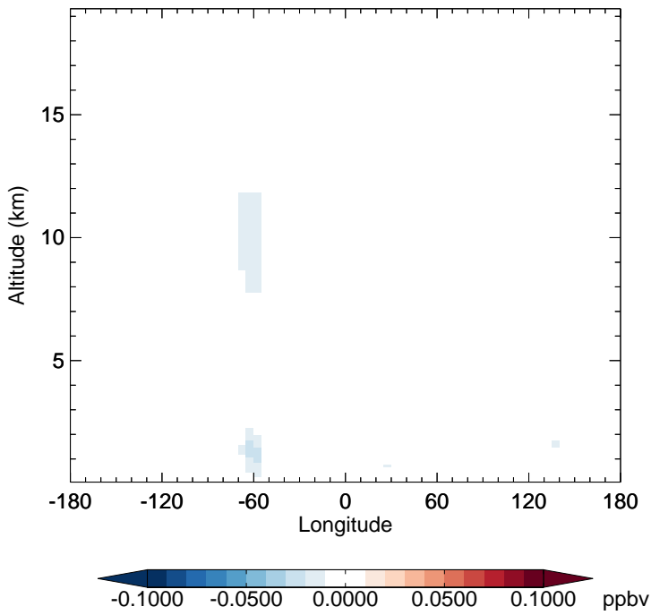
GC_12.0.0 - v11-02e-Run1 ISOA1 - Diff along 15S for Jan
