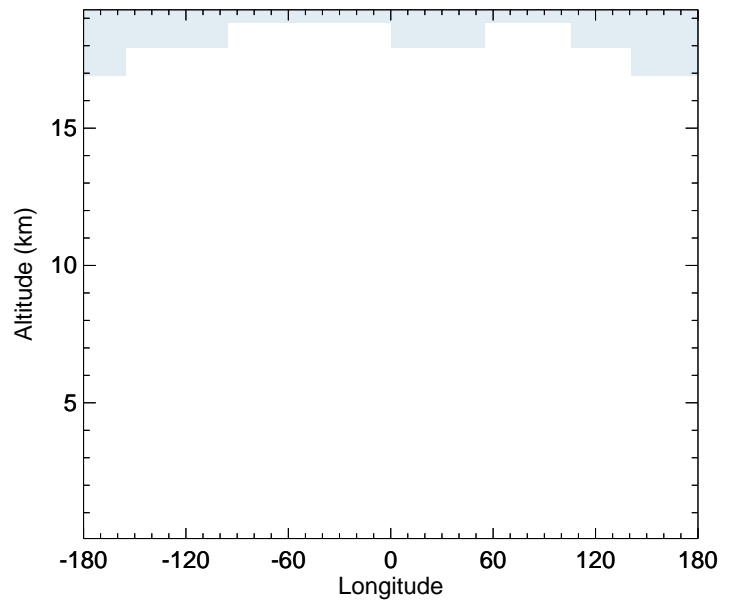
GC_12.0.0 - v11-02f-Run1 BrNO3 - Diff along 42N for Jan
