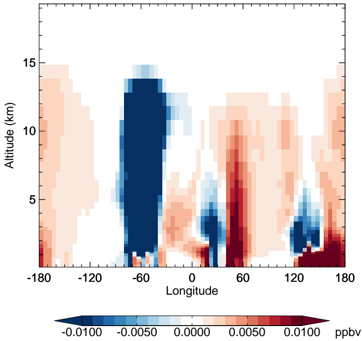
GC_12.0.0 - v11-02e-Run1 MAP - Diff along 15S for Jan
