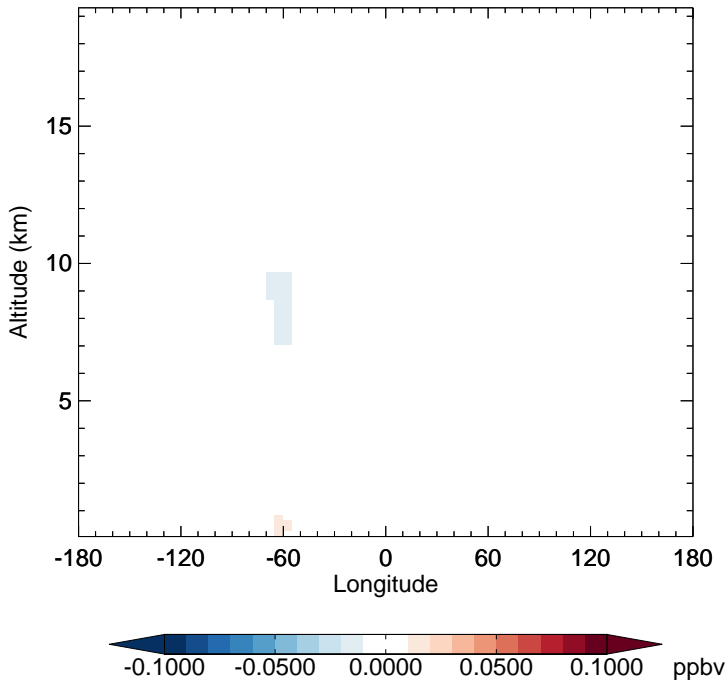
GC_12.0.0 - v11-02f-Run1 IEPOXB - Diff along 15S for Jan
