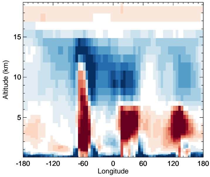
GC_12.0.0 - v11-02f-Run1 OH - Diff along 15S for Jan
