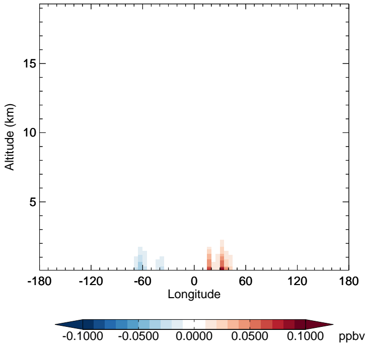
GC_12.0.0 - v11-02e-Run1 SOAP - Diff along 15S for Jan
