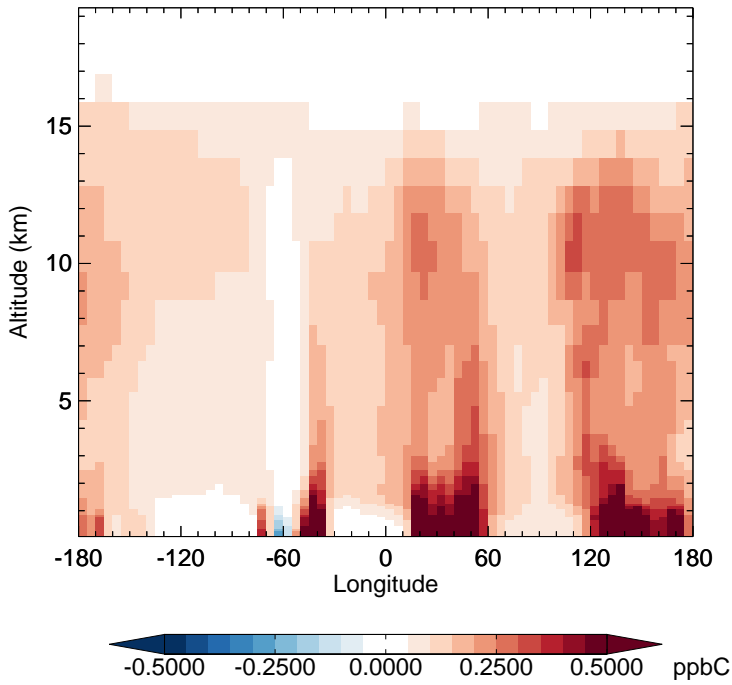
GC_12.0.0 - v11-02e-Run1 ACET - Diff along 15S for Jan
