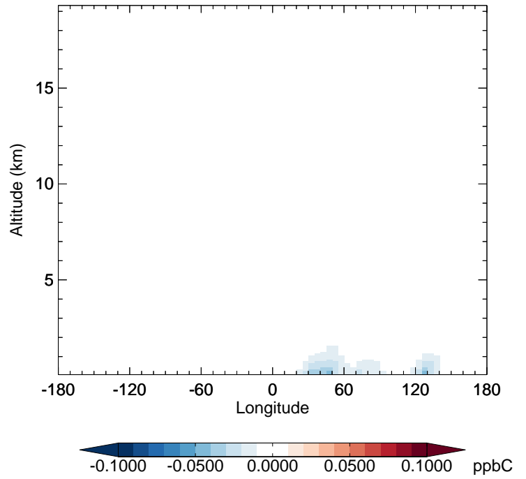
GC_12.0.0 - v11-02f-Run1 MEK - Diff along 42N for Jan
