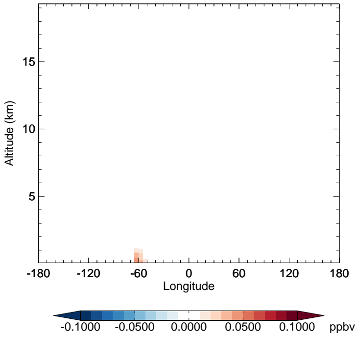
GC_12.0.0 - v11-02f-Run1 TSOA2 - Diff along 15S for Jan
