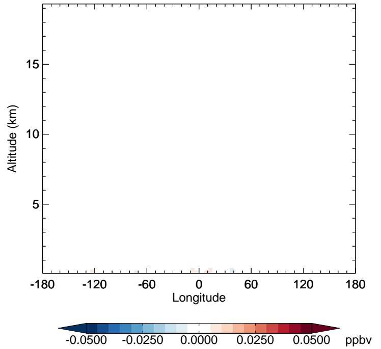
GC_12.0.0 - v11-02e-Run1 RCHO - Diff along 42N for Jan
