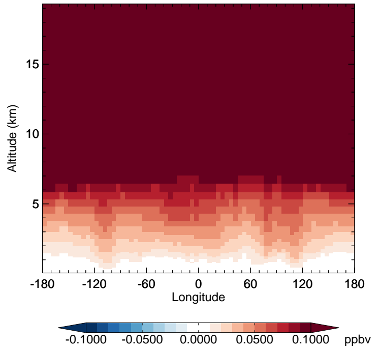
GC_12.0.0 - v11-02f-Run1 N2O - Diff along 42N for Jan
