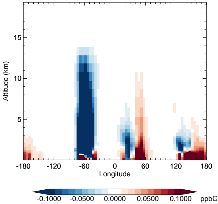
GC_12.0.0 - v11-02e-Run1 MEK - Diff along 15S for Jan
