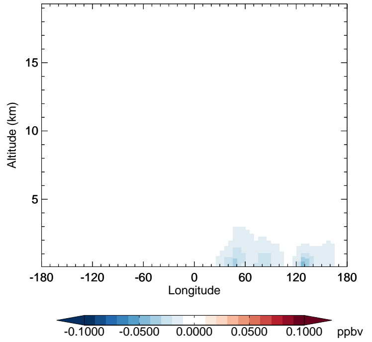
GC_12.0.0 - v11-02f-Run1 PAN - Diff along 42N for Jan
