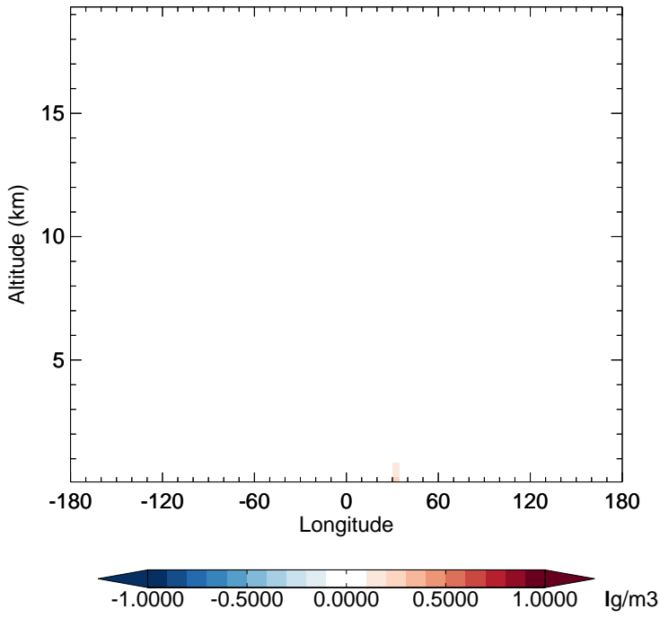
GC_12.0.0 - v11-02f-Run1 SO 2 - Diff along 15S for Jan
