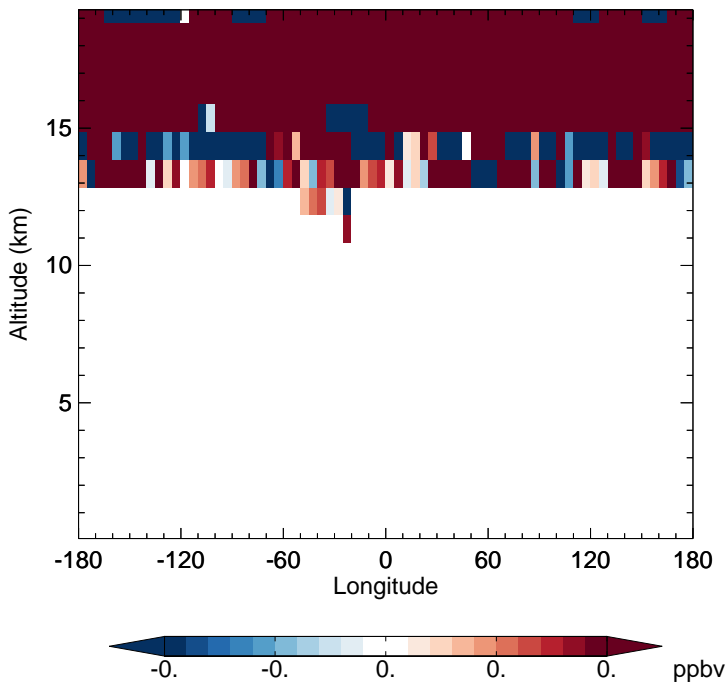
GC_12.0.0 - v11-02e-Run1 H2O - Diff along 15S for Jan
