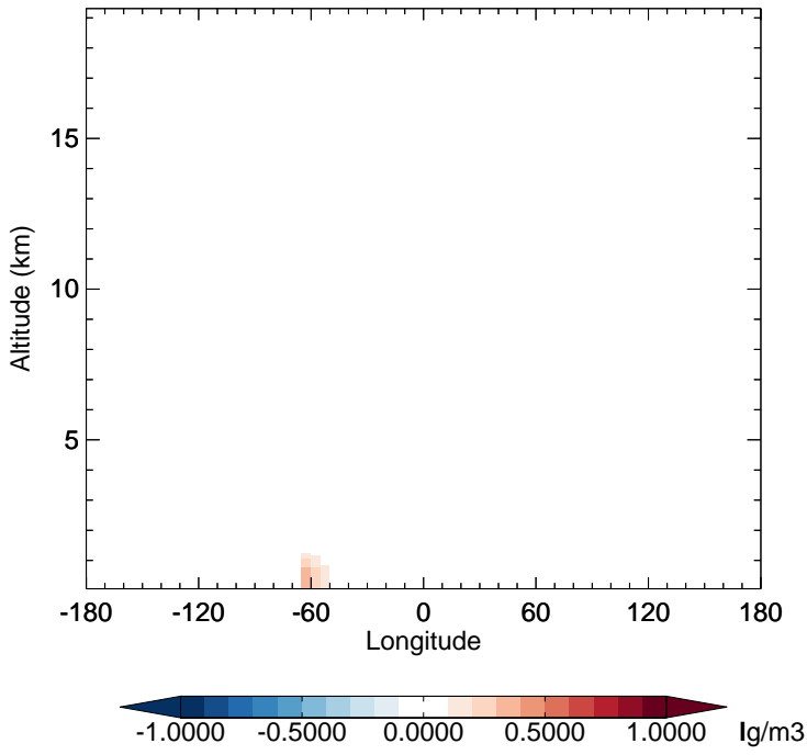
GC_12.0.0 - v11-02f-Run1 OCPI - Diff along 15S for Jan
