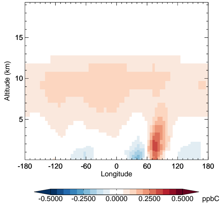
GC_12.0.0 - v11-02e-Run1 ACET - Diff along 42N for Jan
