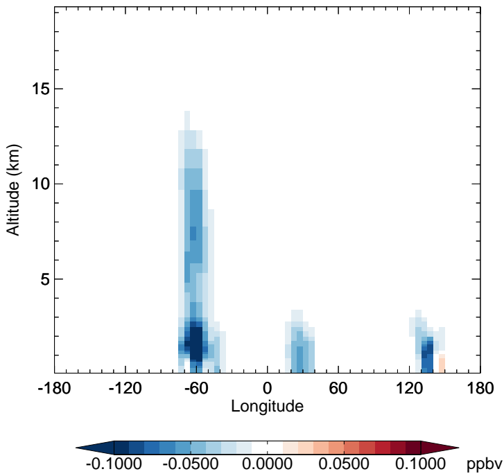
GC_12.0.0 - v11-02e-Run1 GLYC - Diff along 15S for Jan
