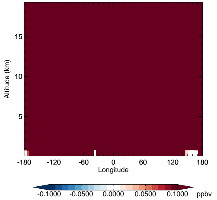
GC_12.0.0 - v11-02f-Run1 CH4 - Diff along 42N for Jan
