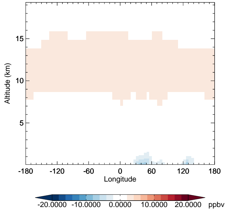
GC_12.0.0 - v11-02f-Run1 CO - Diff along 42N for Jan
