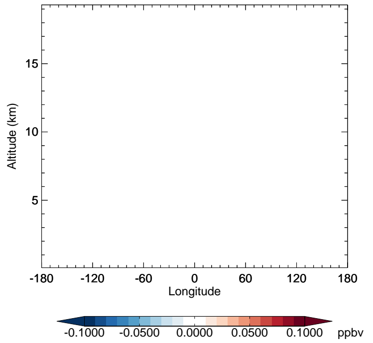
GC_12.0.0 - v11-02f-Run1 GLYX - Diff along 42N for Jan
