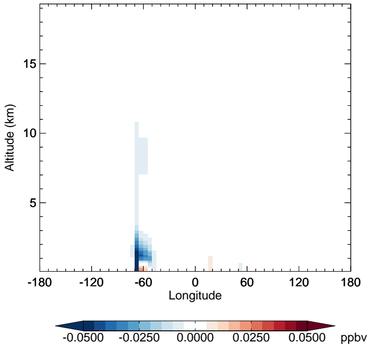
GC_12.0.0 - v11-02f-Run1 MVK - Diff along 15S for Jan
