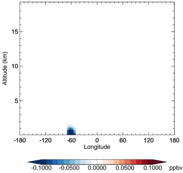
GC_12.0.0 - v11-02f-Run1 MTPA - Diff along 15S for Jan
