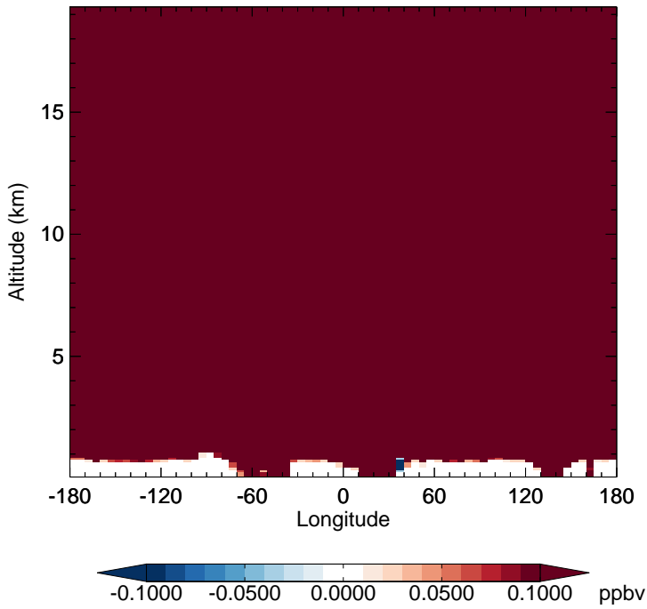
GC_12.0.0 - v11-02e-Run1 CH4 - Diff along 15S for Jan
