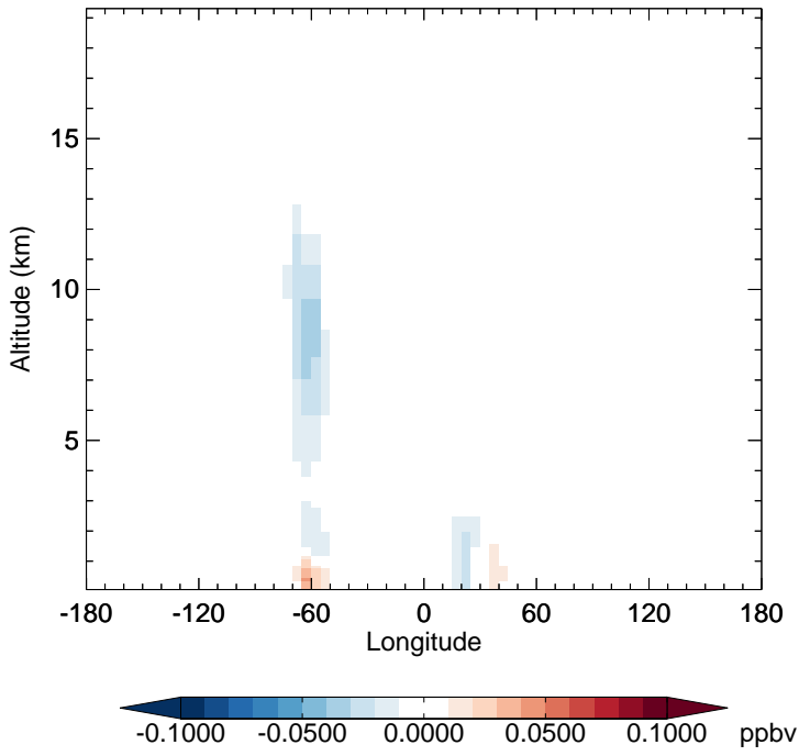
GC_12.0.0 - v11-02f-Run1 IEPOXA - Diff along 15S for Jan
