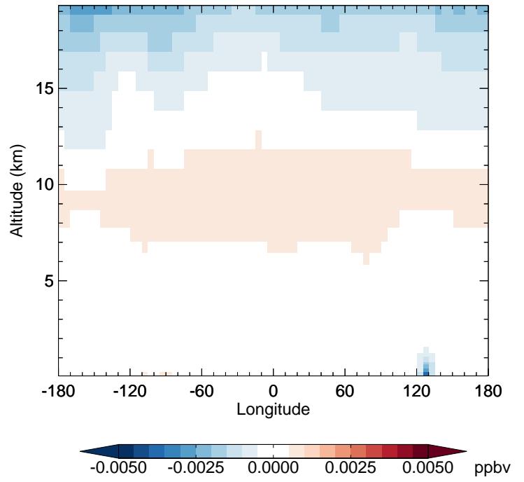
GC_12.0.0 - v11-02f-Run1 HNO 4 - Diff along 42N for Jan
