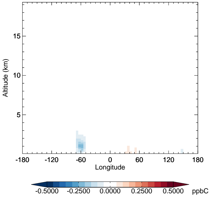
GC_12.0.0 - v11-02f-Run1 ALD2 - Diff along 15S for Jan
