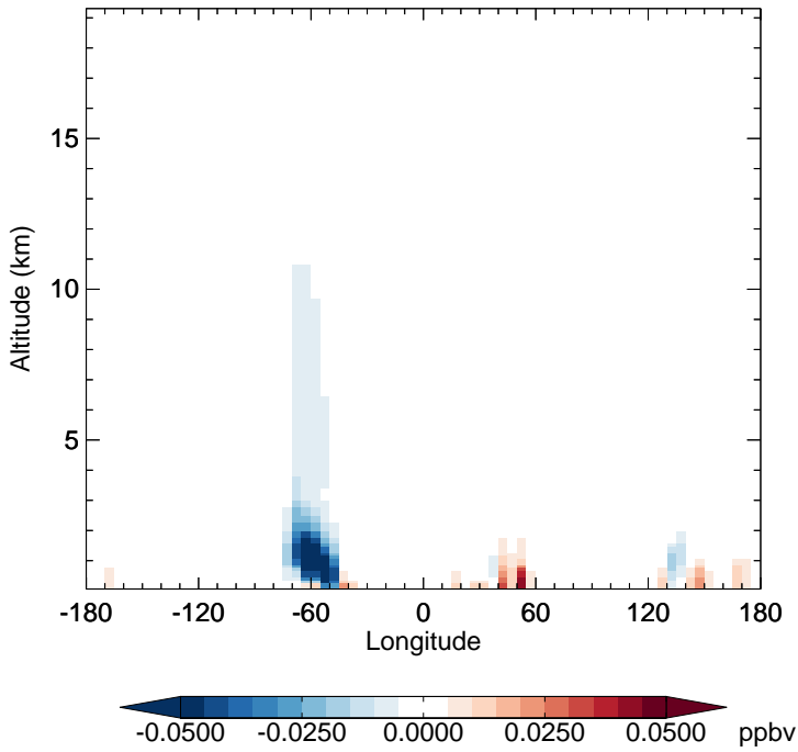
GC_12.0.0 - v11-02e-Run1 RCHO - Diff along 15S for Jan
