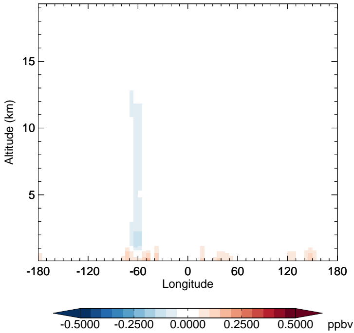
GC_12.0.0 - v11-02e-Run1 CH 2 O - Diff along 15S for Jan
