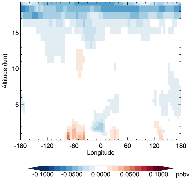
GC_12.0.0 - v11-02e-Run1 HNO 3 - Diff along 15S for Jan
