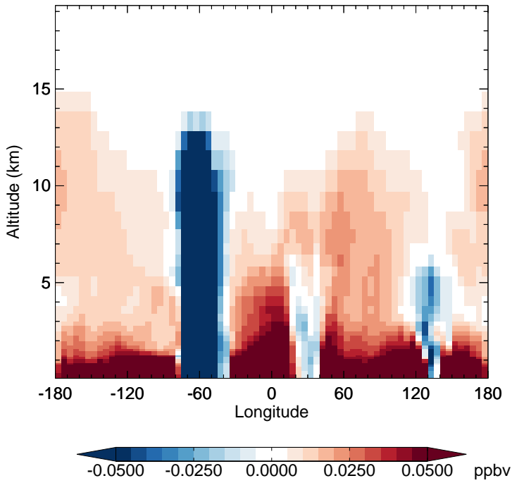
GC_12.0.0 - v11-02e-Run1 MP - Diff along 15S for Jan
