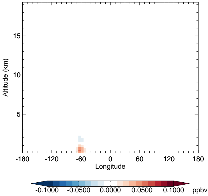
GC_12.0.0 - v11-02f-Run1 GLYC - Diff along 15S for Jan
