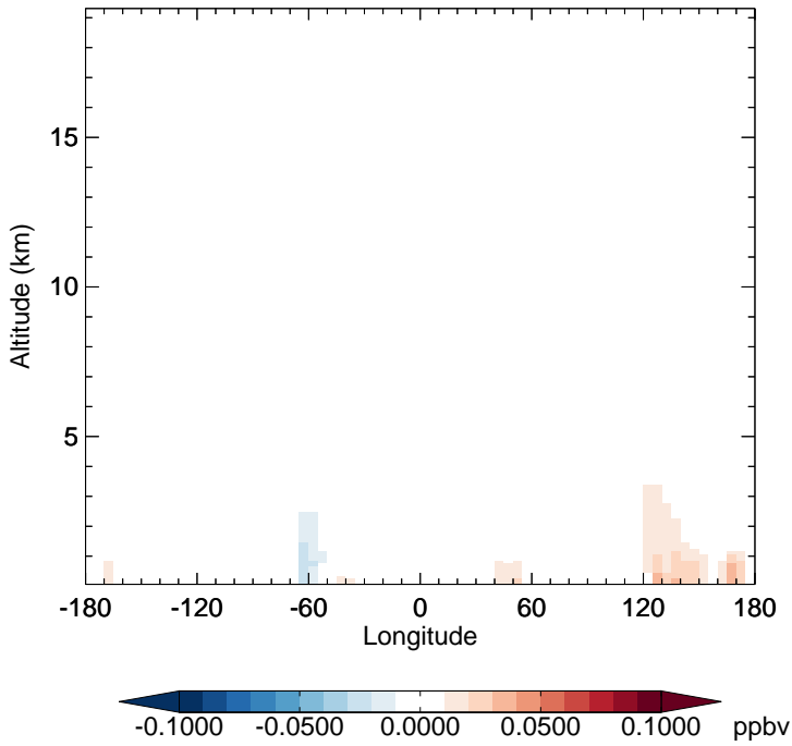
GC_12.0.0 - v11-02e-Run1 TSOG2 - Diff along 15S for Jan
