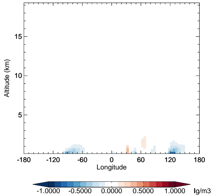
GC_12.0.0 - v11-02e-Run1 SO4 - Diff along 42N for Jan
