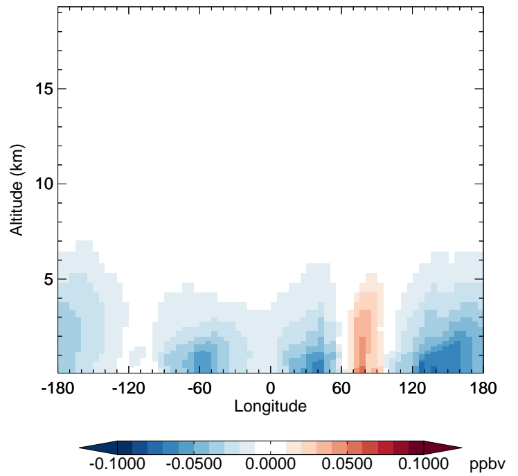
GC_12.0.0 - v11-02e-Run1 PAN - Diff along 42N for Jan
