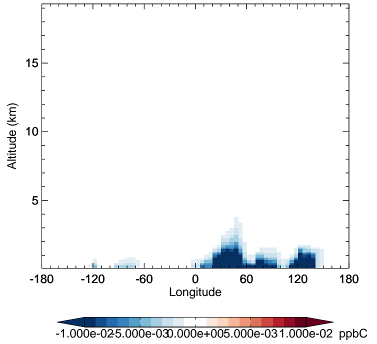
GC_12.0.0 - v11-02f-Run1 PRPE - Diff along 42N for Jan
