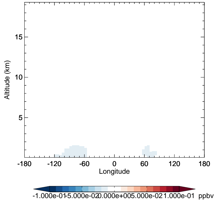
GC_12.0.0 - v11-02e-Run1 IONITA - Diff along 42N for Jan
