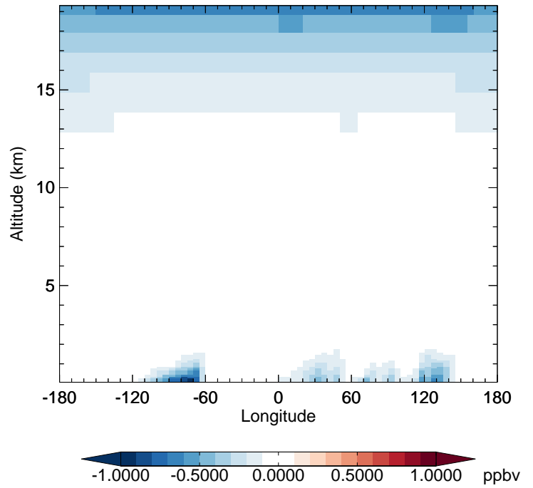
GC_12.0.0 - v11-02e-Run1 NO2 - Diff along 42N for Jan
