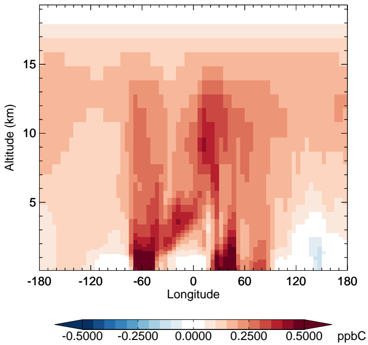
GC_12.0.0 - v11-02e-Run1 C2H6 - Diff along 15S for Jan
