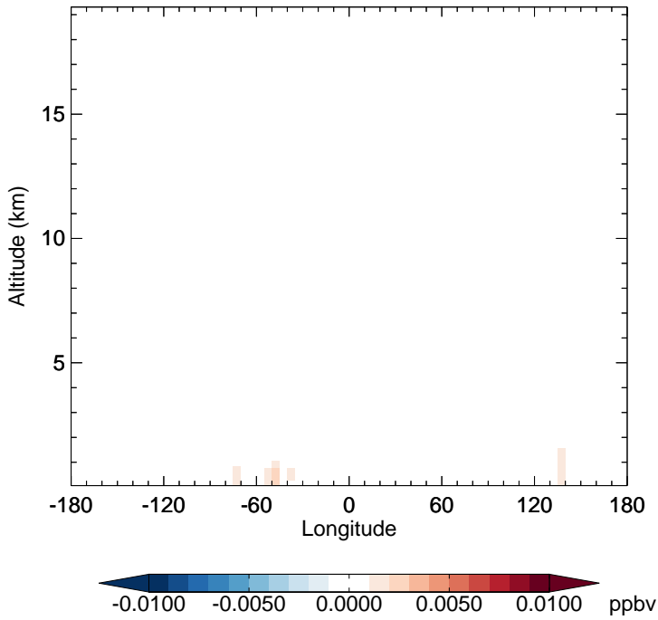
GC_12.0.0 - v11-02e-Run1 MVKN - Diff along 15S for Jan
