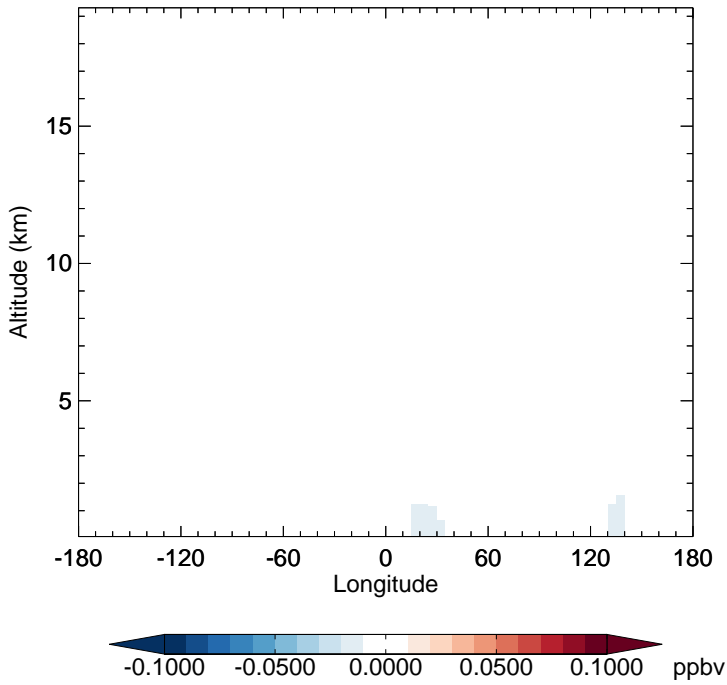
GC_12.0.0 - v11-02e-Run1 SOAGX - Diff along 15S for Jan
