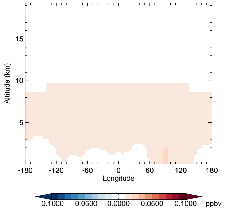
GC_12.0.0 - v11-02e-Run1 ACTA - Diff along 42N for Jan
