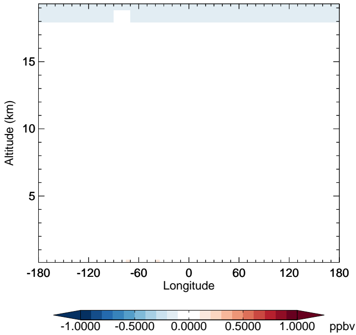
GC_12.0.0 - v11-02e-Run1 NO2 - Diff along 15S for Jan
