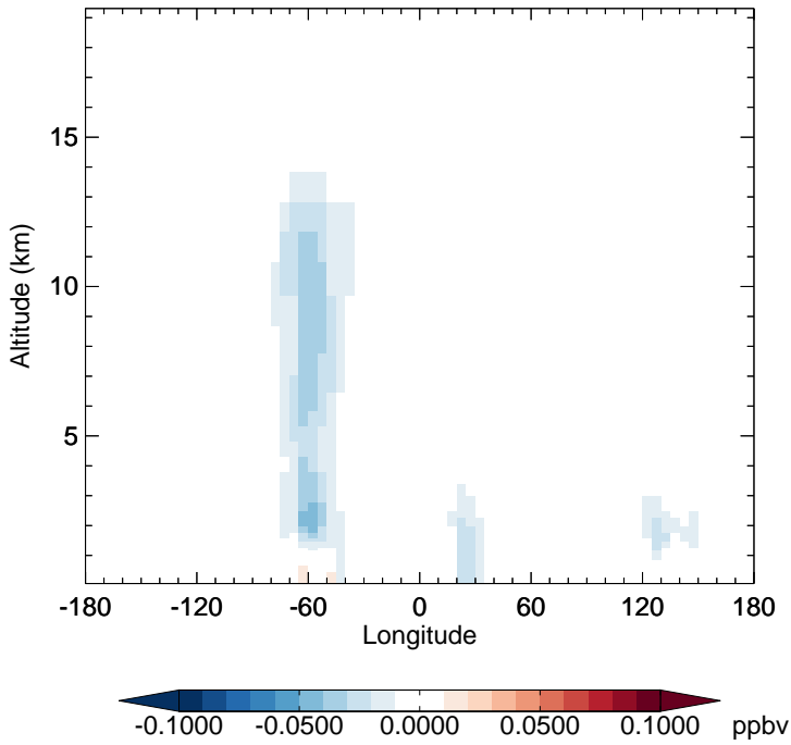
GC_12.0.0 - v11-02e-Run1 IMAE - Diff along 15S for Jan
