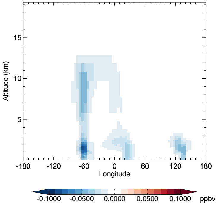
GC_12.0.0 - v11-02e-Run1 ISO3 - Diff along 15S for Jan
