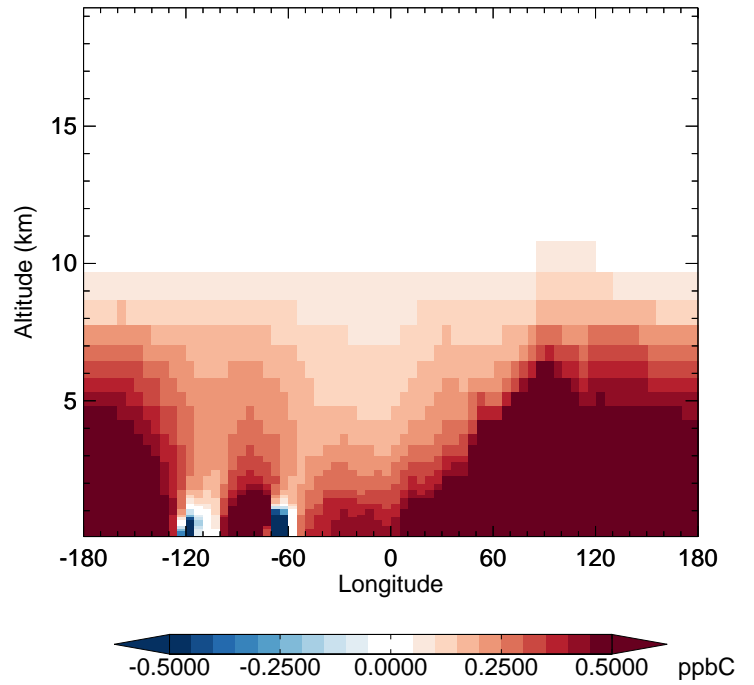
GC_12.0.0 - v11-02e-Run1 ALK4 - Diff along 42N for Jan
