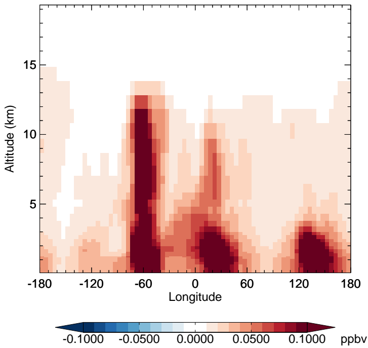
GC_12.0.0 - v11-02e-Run1 ACTA - Diff along 15S for Jan
