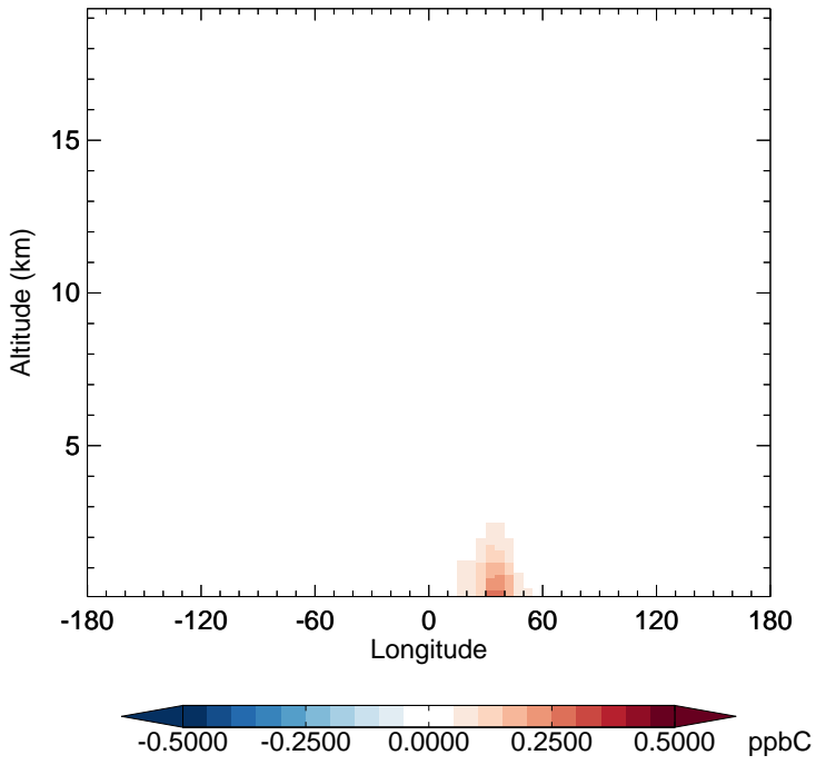
GC_12.0.0 - v11-02f-Run1 ALK4 - Diff along 15S for Jan
