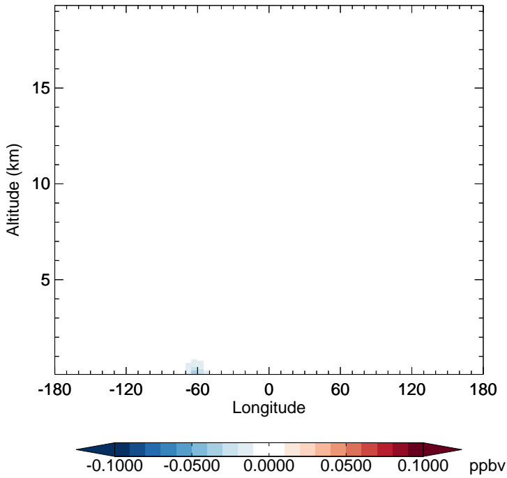
GC_12.0.0 - v11-02e-Run1 LIMO - Diff along 15S for Jan
