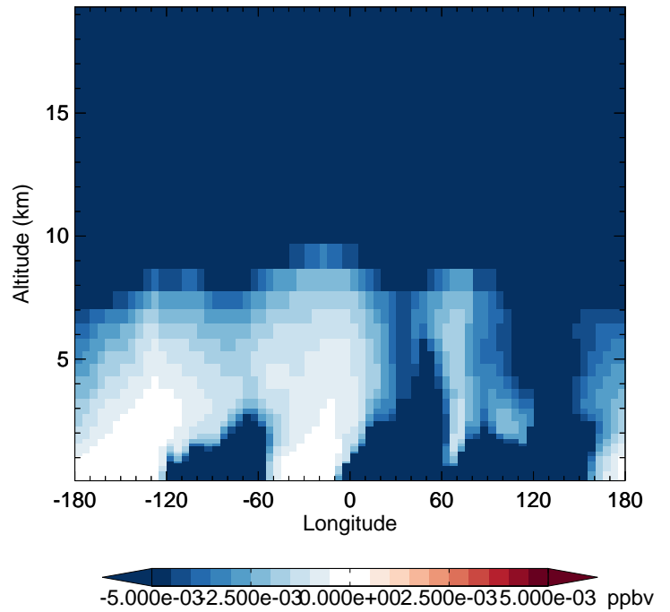
GC_12.0.0 - v11-02e-Run1 N2O5 - Diff along 42N for Jan
