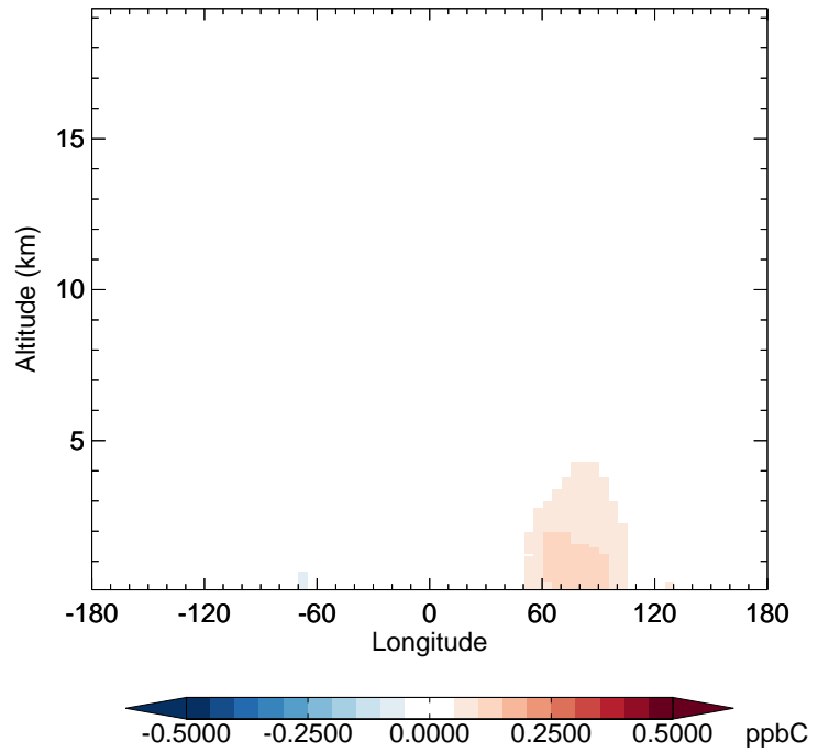
GC_12.0.0 - v11-02e-Run1 ALD2 - Diff along 42N for Jan
