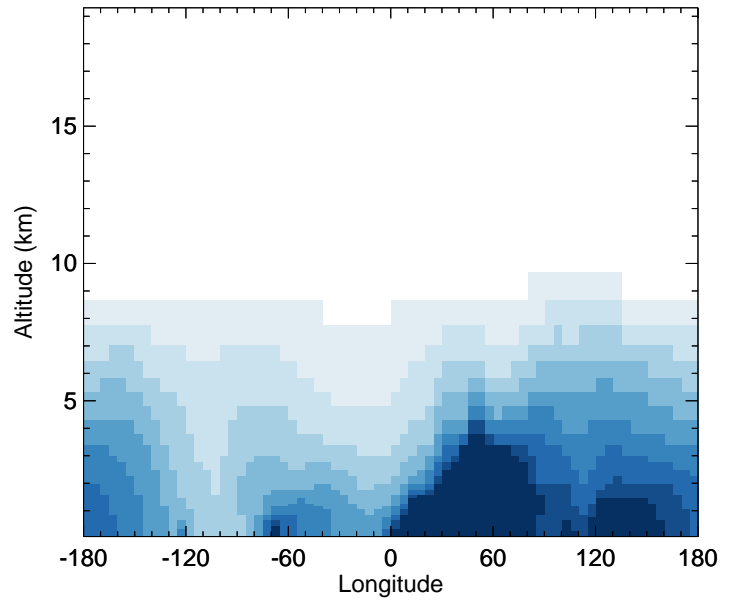
GC_12.0.0 - v11-02e-Run1 C3H8 - Diff along 42N for Jan
