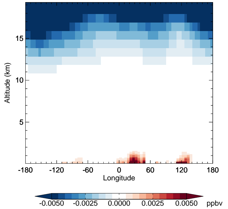
GC_12.0.0 - v11-02f-Run1 N2O5 - Diff along 42N for Jan
