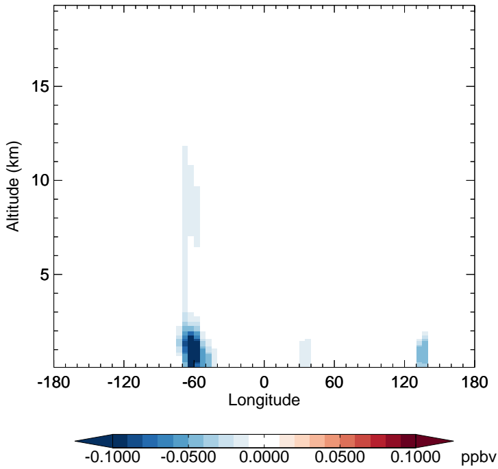
GC_12.0.0 - v11-02e-Run1 RIPB - Diff along 15S for Jan
