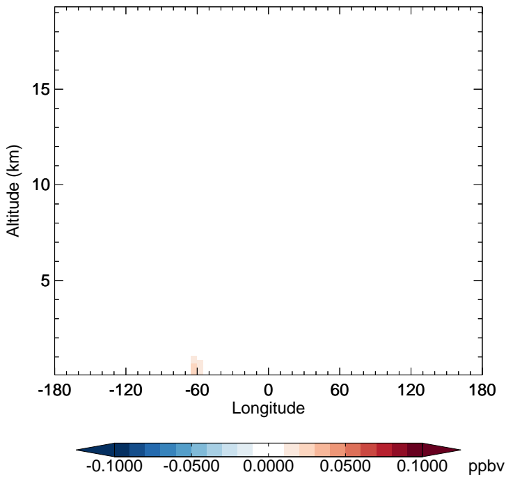
GC_12.0.0 - v11-02f-Run1 ISOA1 - Diff along 15S for Jan
