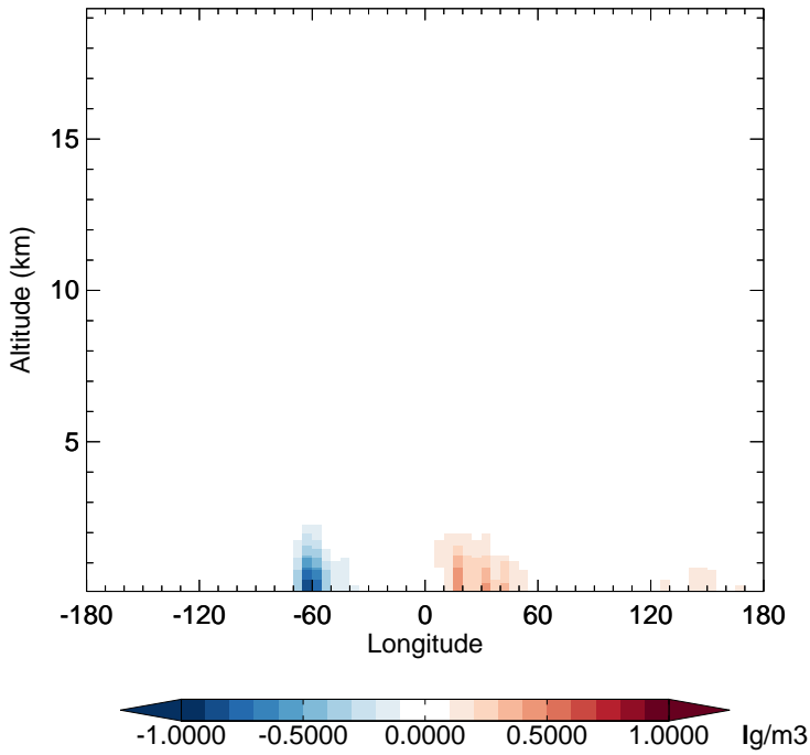
GC_12.0.0 - v11-02e-Run1 SOAS - Diff along 15S for Jan
