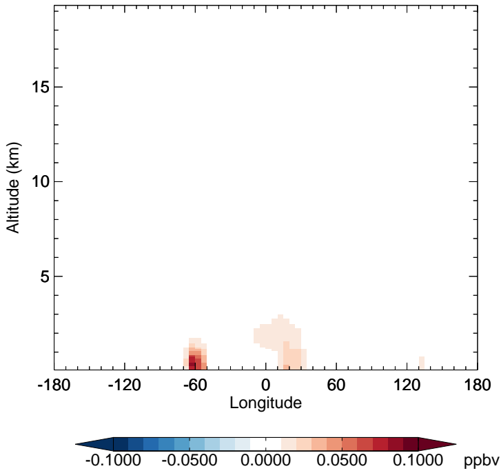
GC_12.0.0 - v11-02f-Run1 INDIOL - Diff along 15S for Jan
