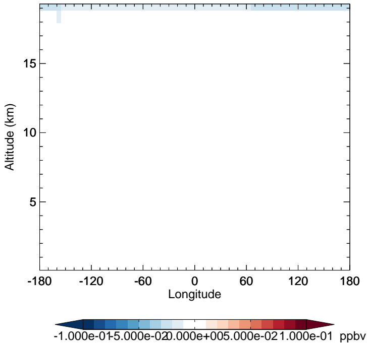
GC_12.0.0 - v11-02e-Run1 CINO3 - Diff along 15S for Jan
