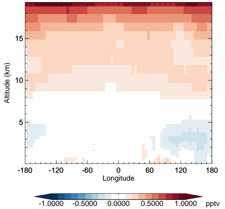
GC_12.0.0 - v11-02e-Run1 HO2 - Diff along 42N for Jan
