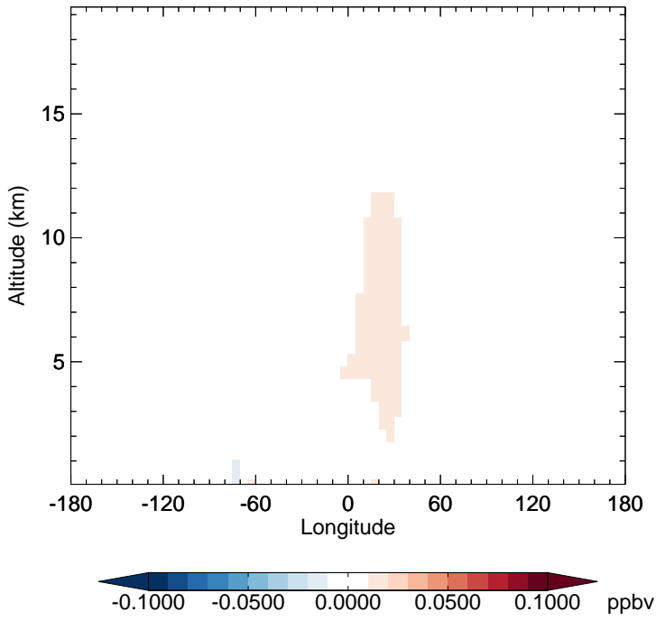
GC_12.0.0 - v11-02f-Run1 PAN - Diff along 15S for Jan
