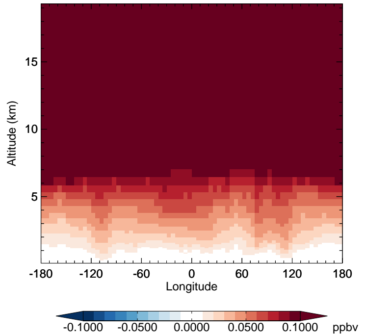
GC_12.0.0 - v11-02e-Run1 N2O - Diff along 42N for Jan
