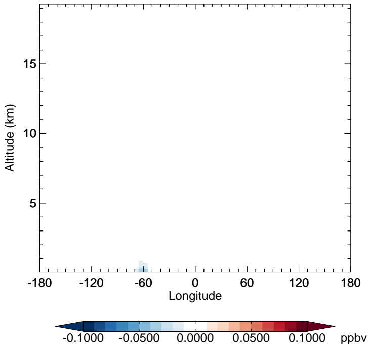
GC_12.0.0 - v11-02e-Run1 MTPO - Diff along 15S for Jan
