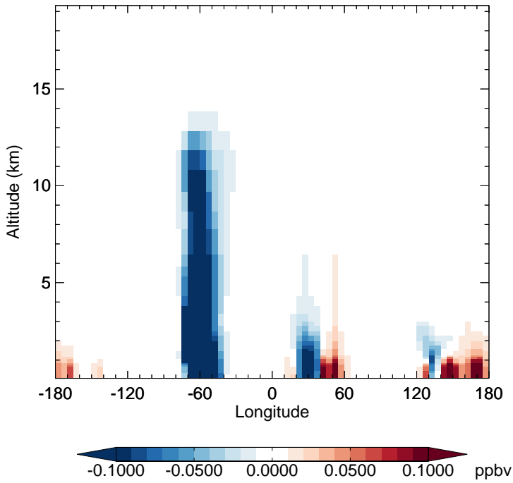
GC_12.0.0 - v11-02e-Run1 EOH - Diff along 15S for Jan
