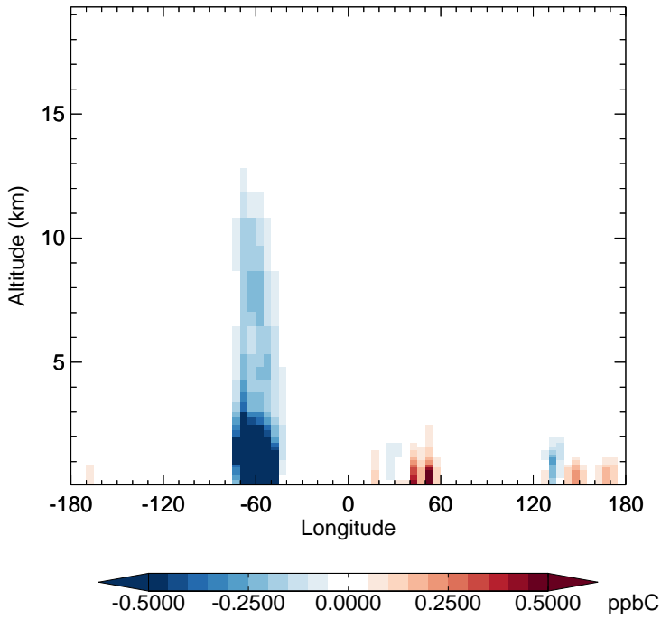
GC_12.0.0 - v11-02e-Run1 ALD2 - Diff along 15S for Jan
