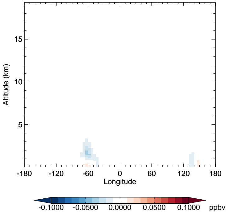
GC_12.0.0 - v11-02e-Run1 MGLY - Diff along 15S for Jan
