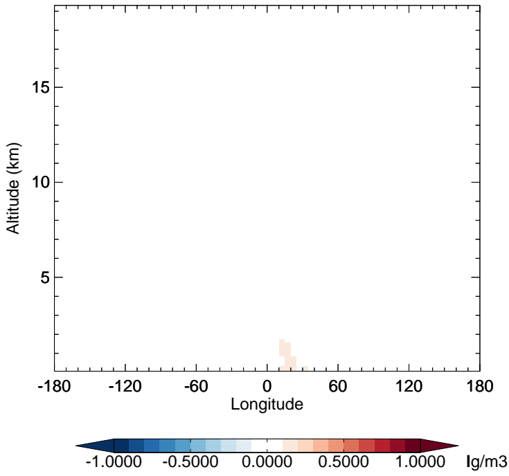
GC_12.0.0 - v11-02f-Run1 NH4 - Diff along 15S for Jan
