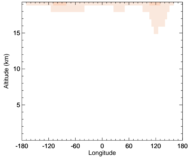
GC_12.0.0 - v11-02e-Run1 ClO - Diff along 42N for Jan
