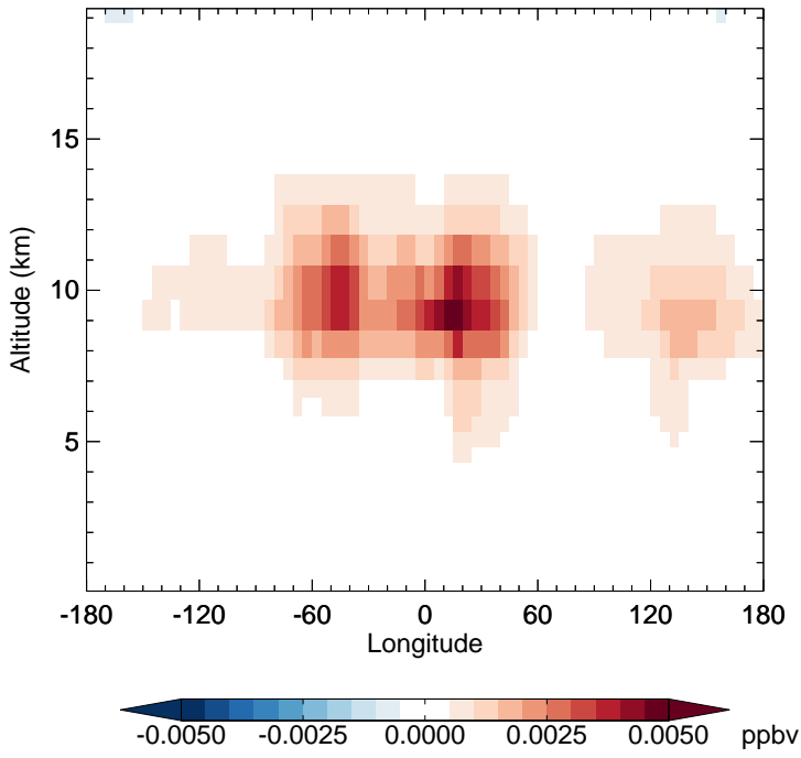
GC_12.0.0 - v11-02f-Run1 HNO 4 - Diff along 15S for Jan
