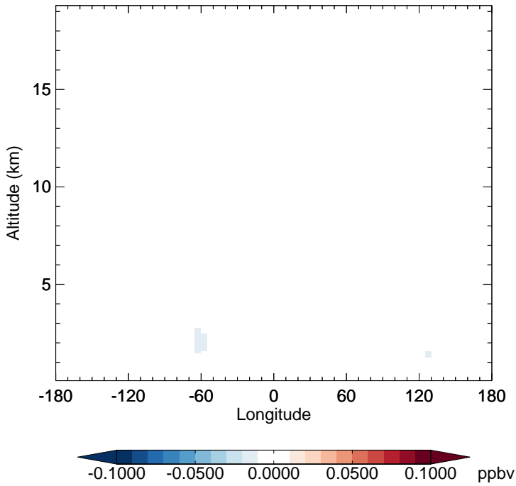
GC_12.0.0 - v11-02e-Run1 ISOG1 - Diff along 15S for Jan
