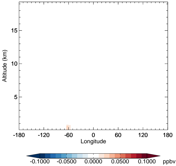
GC_12.0.0 - v11-02f-Run1 IPMN - Diff along 15S for Jan
