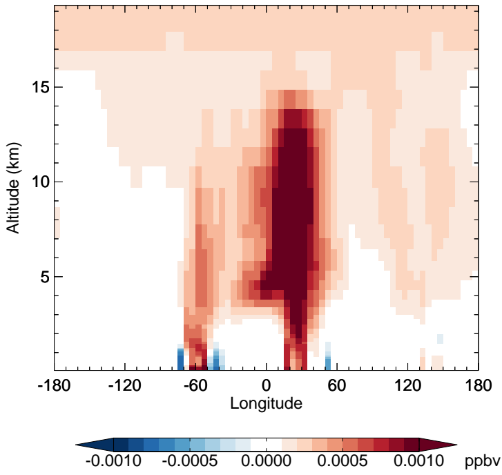
GC_12.0.0 - v11-02f-Run1 PPN - Diff along 15S for Jan
