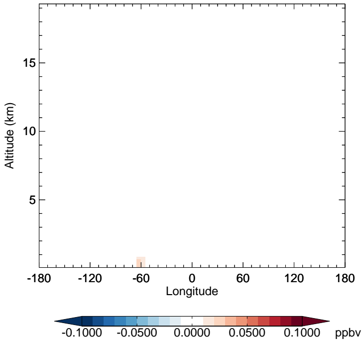
GC_12.0.0 - v11-02f-Run1 MGLY - Diff along 15S for Jan
