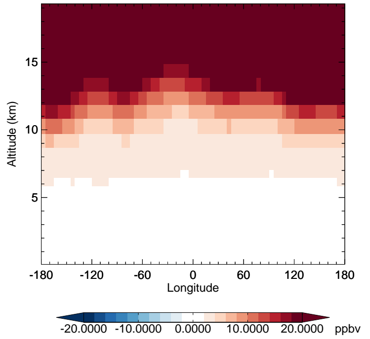
GC_12.0.0 - v11-02f-Run1 O3 - Diff along 42N for Jan
