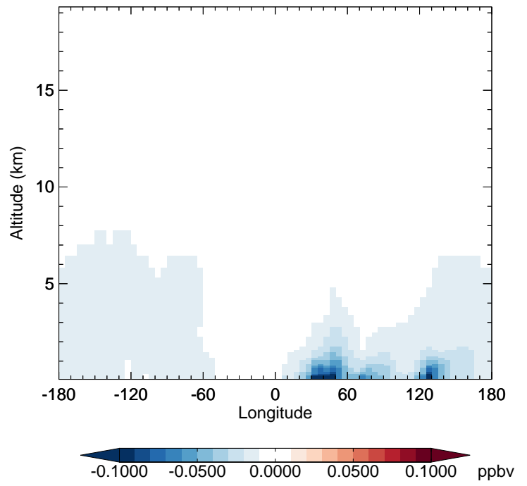
GC_12.0.0 - v11-02f-Run1 BENZ - Diff along 42N for Jan
