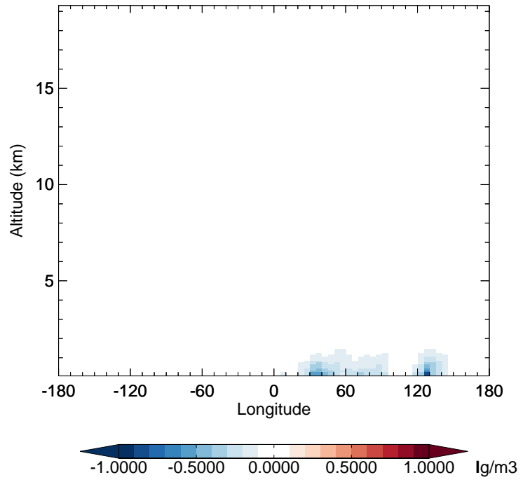
GC_12.0.0 - v11-02f-Run1 OCPI - Diff along 42N for Jan
