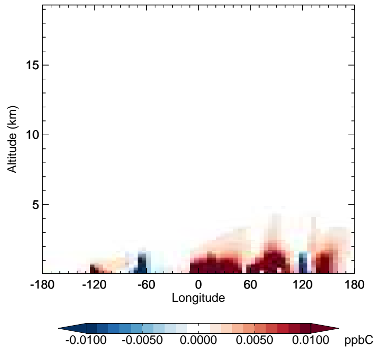
GC_12.0.0 - v11-02e-Run1 PRPE - Diff along 42N for Jan
