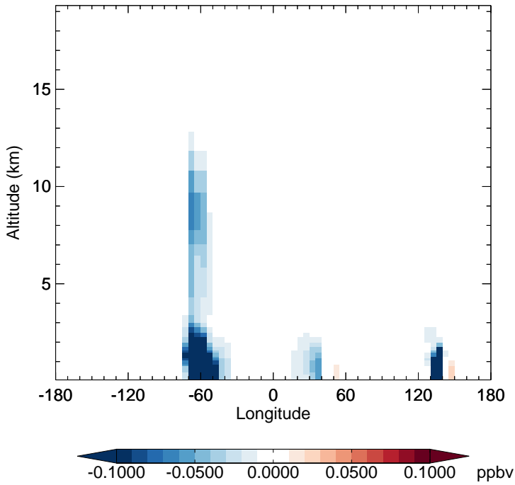
GC_12.0.0 - v11-02e-Run1 RIPA - Diff along 15S for Jan
