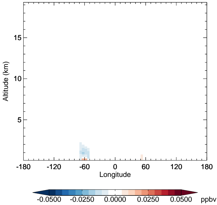
GC_12.0.0 - v11-02f-Run1 RCHO - Diff along 15S for Jan
