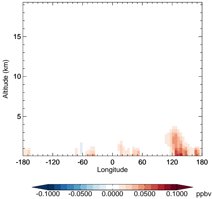
GC_12.0.0 - v11-02e-Run1 TSOG3 - Diff along 15S for Jan
