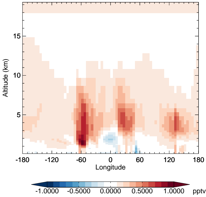
GC_12.0.0 - v11-02f-Run1 HO2 - Diff along 15S for Jan
