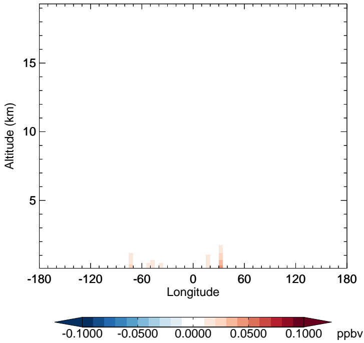
GC_12.0.0 - v11-02f-Run1 SOAP - Diff along 15S for Jan
