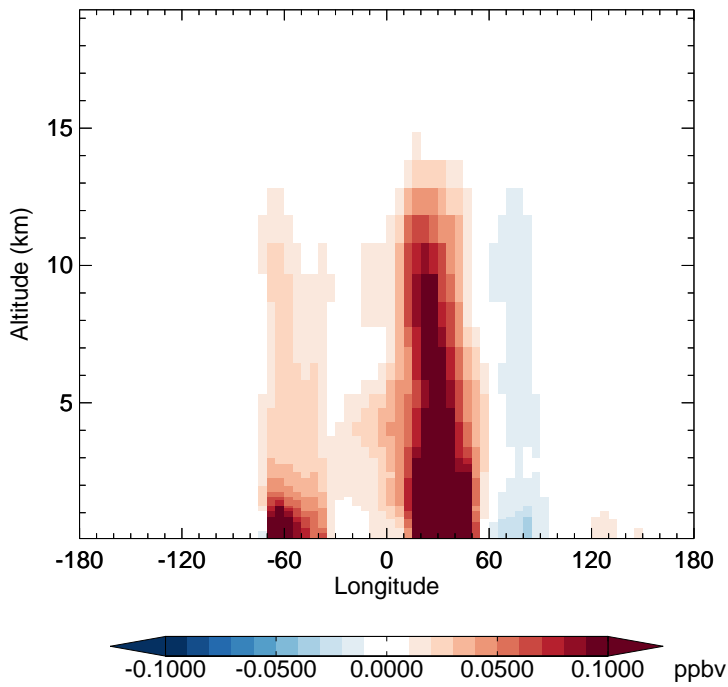
GC_12.0.0 - v11-02e-Run1 BENZ - Diff along 15S for Jan
