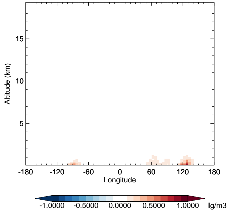
GC_12.0.0 - v11-02e-Run1 NH4 - Diff along 42N for Jan
