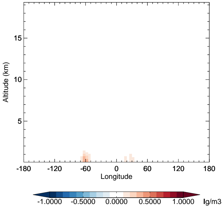
GC_12.0.0 - v11-02e-Run1 OCPI - Diff along 15S for Jan
