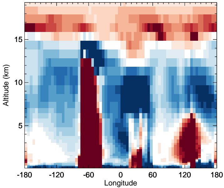
GC_12.0.0 - v11-02e-Run1 OH - Diff along 15S for Jan
