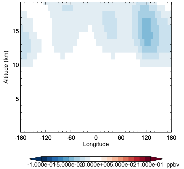
GC_12.0.0 - v11-02e-Run1 MPN - Diff along 42N for Jan
