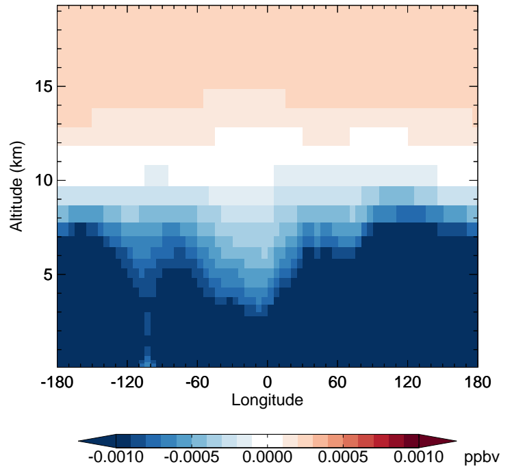
GC_12.0.0 - v11-02f-Run1 PPN - Diff along 42N for Jan
