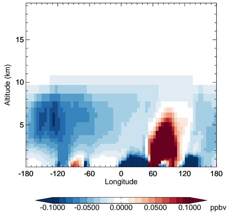
GC_12.0.0 - v11-02e-Run1 BENZ - Diff along 42N for Jan
