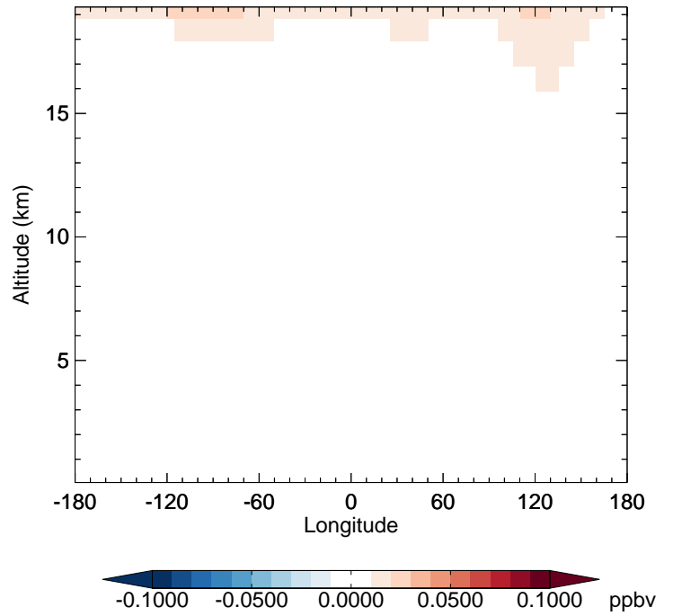
GC_12.0.0 - v11-02e-Run1 HOCl - Diff along 42N for Jan
