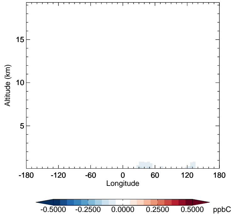
GC_12.0.0 - v11-02f-Run1 ALD2 - Diff along 42N for Jan
