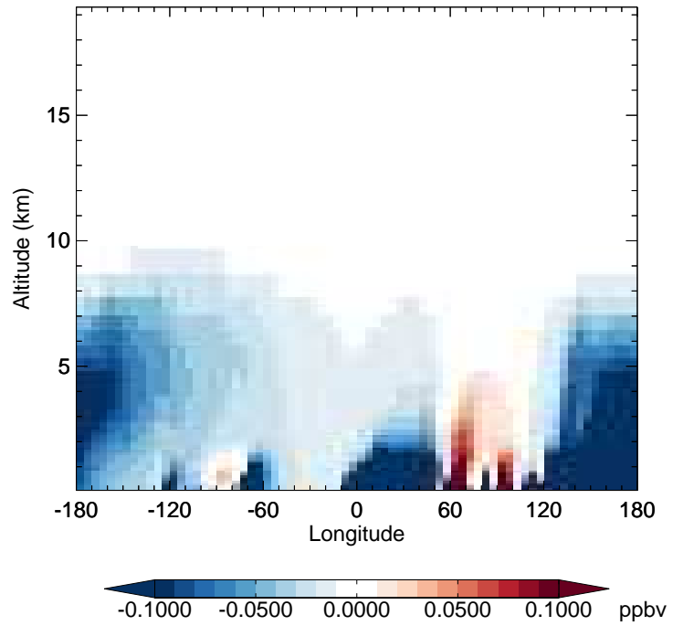
GC_12.0.0 - v11-02e-Run1 TOLU - Diff along 42N for Jan
