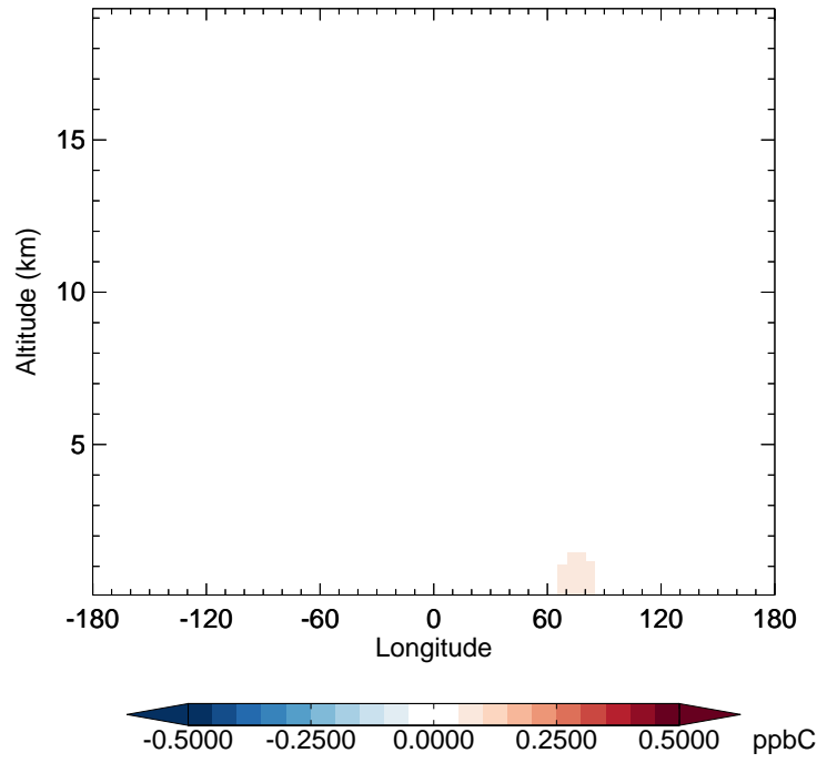
GC_12.0.0 - v11-02f-Run1 ALK4 - Diff along 42N for Jan
