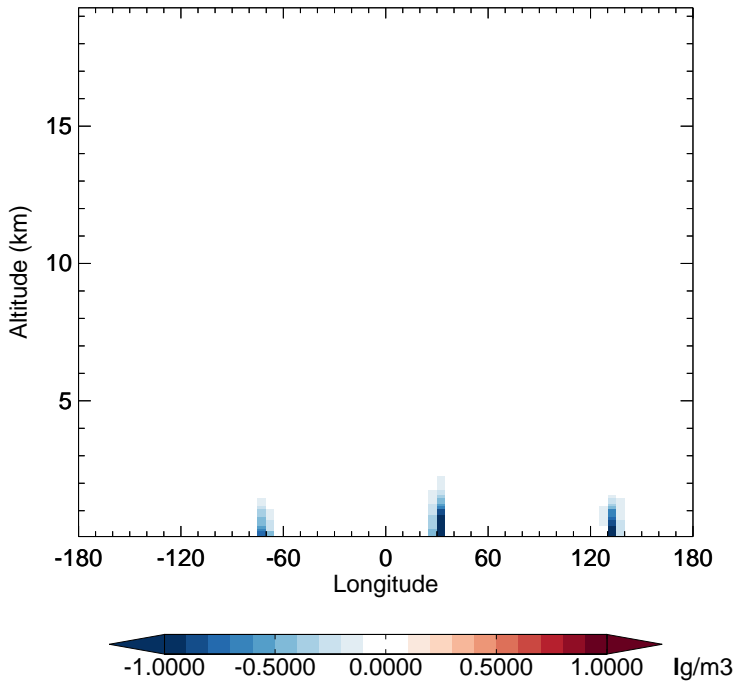
GC_12.0.0 - v11-02e-Run1 SO 2 - Diff along 15S for Jan
