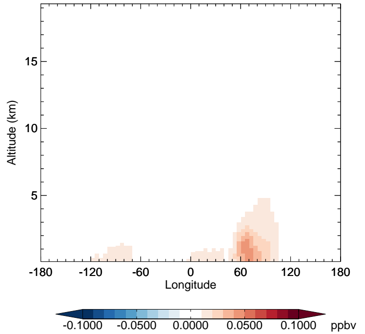
GC_12.0.0 - v11-02e-Run1 INDIOL - Diff along 42N for Jan
