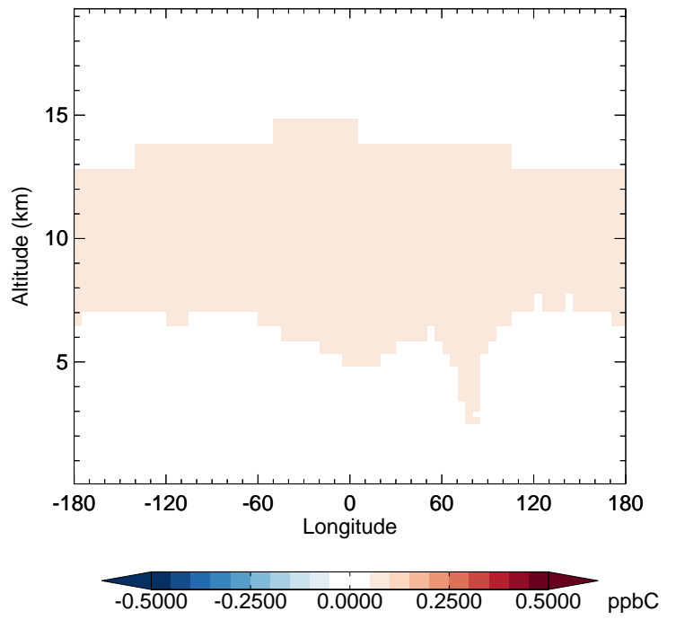
GC_12.0.0 - v11-02f-Run1 C2H6 - Diff along 42N for Jan
