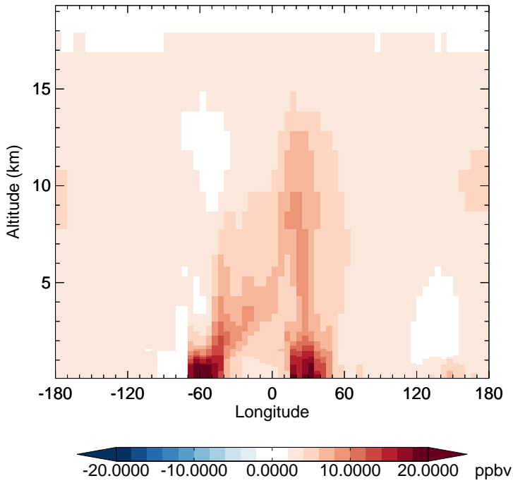
GC_12.0.0 - v11-02e-Run1 CO - Diff along 15S for Jan
