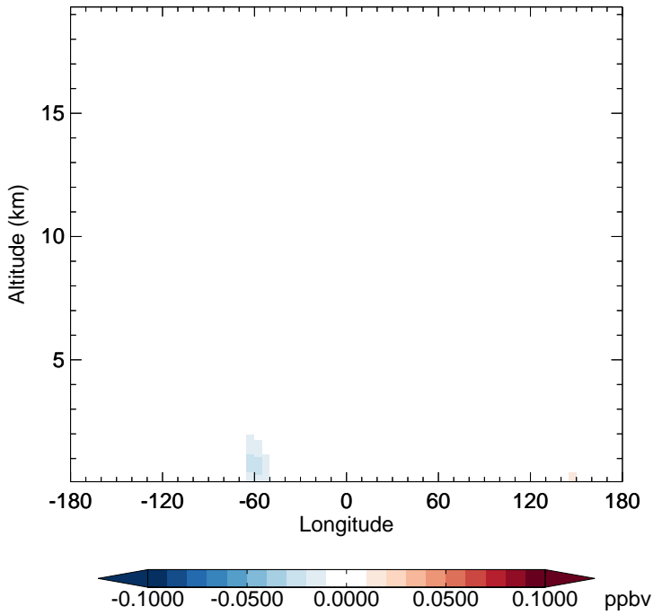
GC_12.0.0 - v11-02e-Run1 TSOA0 - Diff along 15S for Jan
