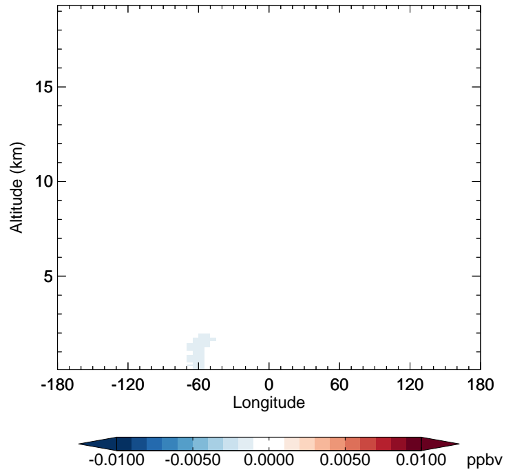
GC_12.0.0 - v11-02e-Run1 R4N2 - Diff along 42N for Jan
