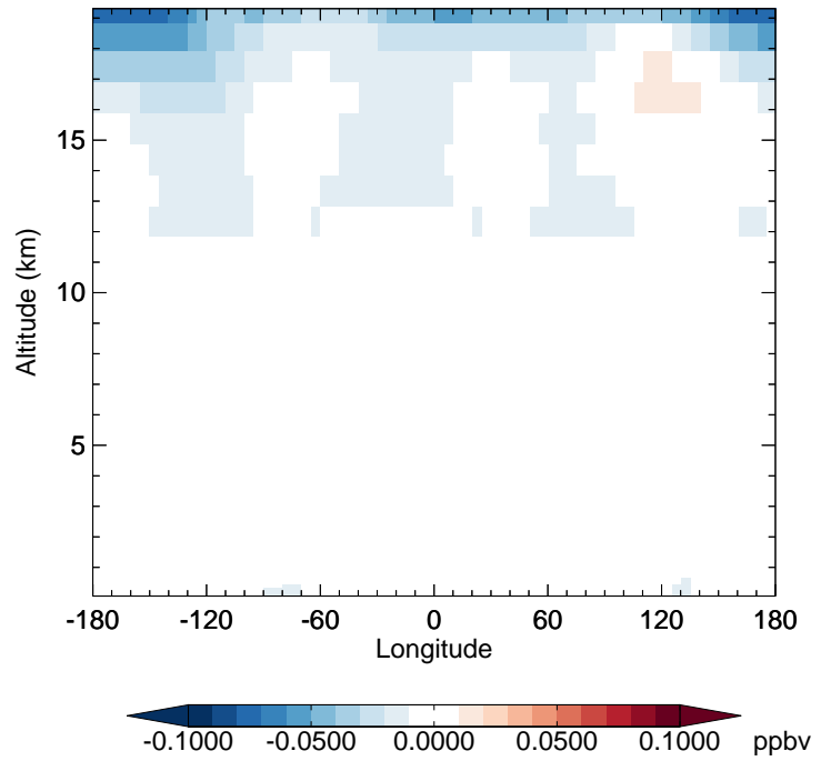
GC_12.0.0 - v11-02e-Run1 HCl - Diff along 42N for Jan
