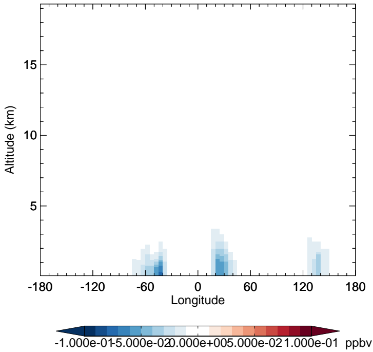
GC_12.0.0 - v11-02e-Run1 IONITA - Diff along 15S for Jan
