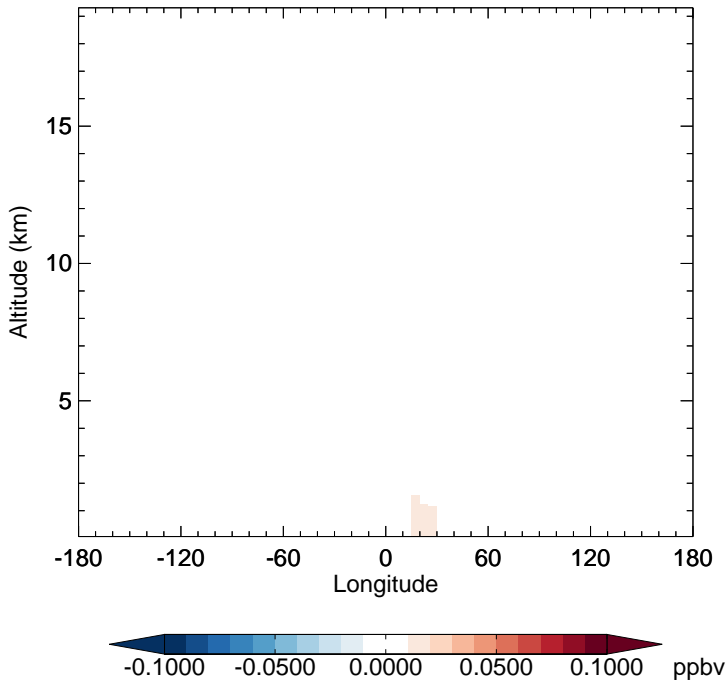
GC_12.0.0 - v11-02f-Run1 SOAGX - Diff along 15S for Jan
