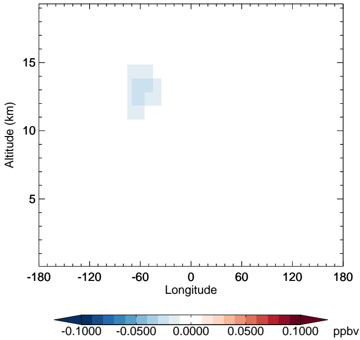
GC_12.0.0 - v11-02e-Run1 ISOA3 - Diff along 15S for Jan
