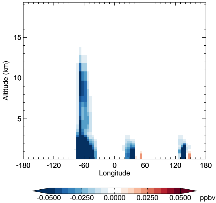
GC_12.0.0 - v11-02e-Run1 MACR - Diff along 15S for Jan
