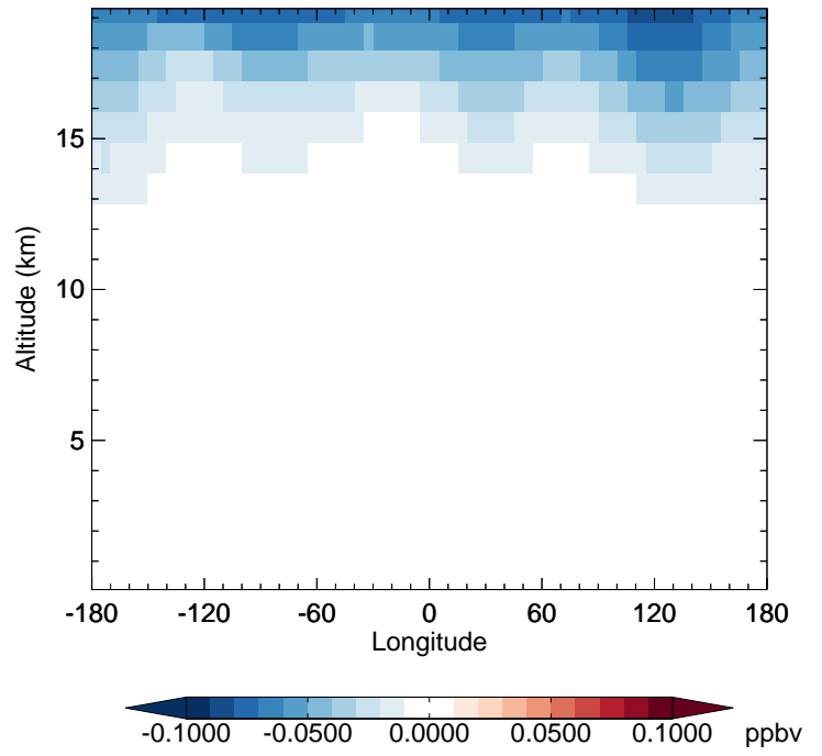
GC_12.0.0 - v11-02f-Run1 CINO3 - Diff along 42N for Jan
