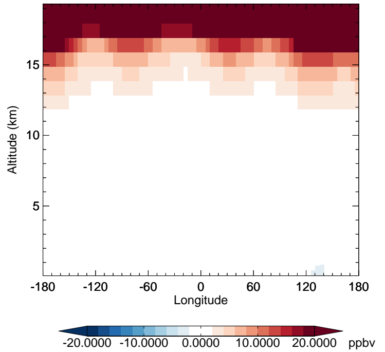
GC_12.0.0 - v11-02e-Run1 O3 - Diff along 42N for Jan
