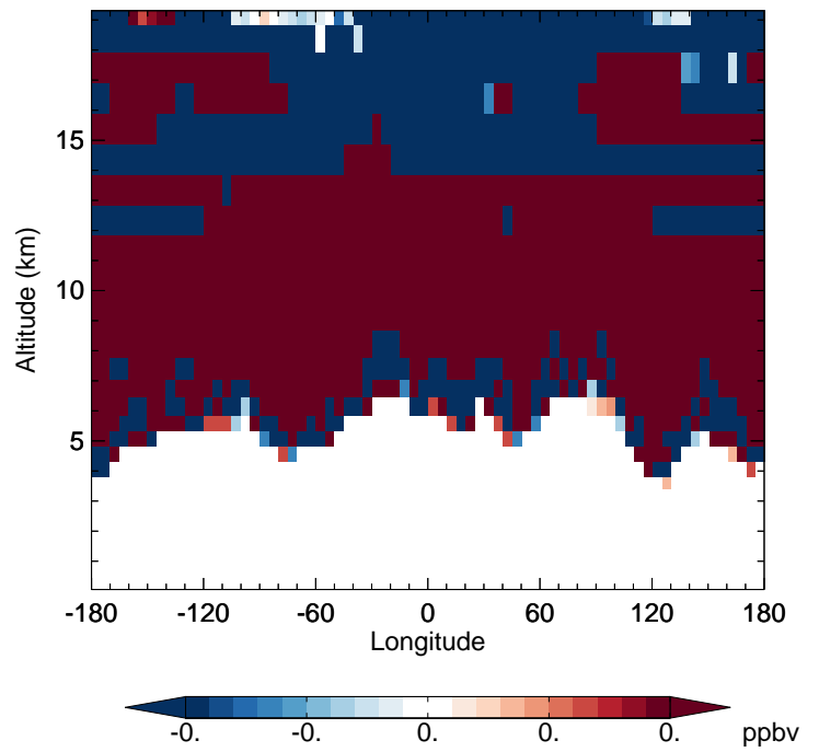
GC_12.0.0 - v11-02e-Run1 H2O - Diff along 42N for Jan
