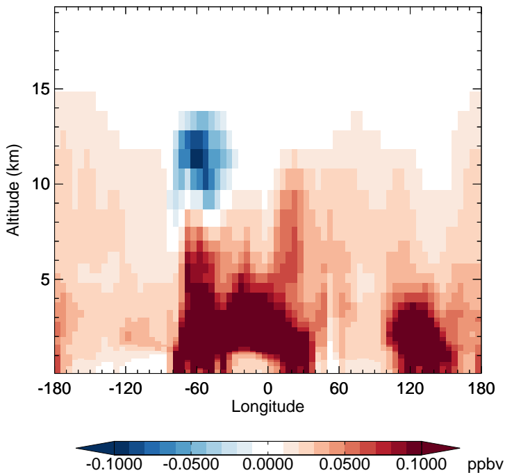
GC_12.0.0 - v11-02e-Run1 H2O2 - Diff along 15S for Jan
