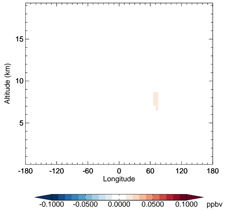
GC_12.0.0 - v11-02f-Run1 H2O2 - Diff along 42N for Jan
