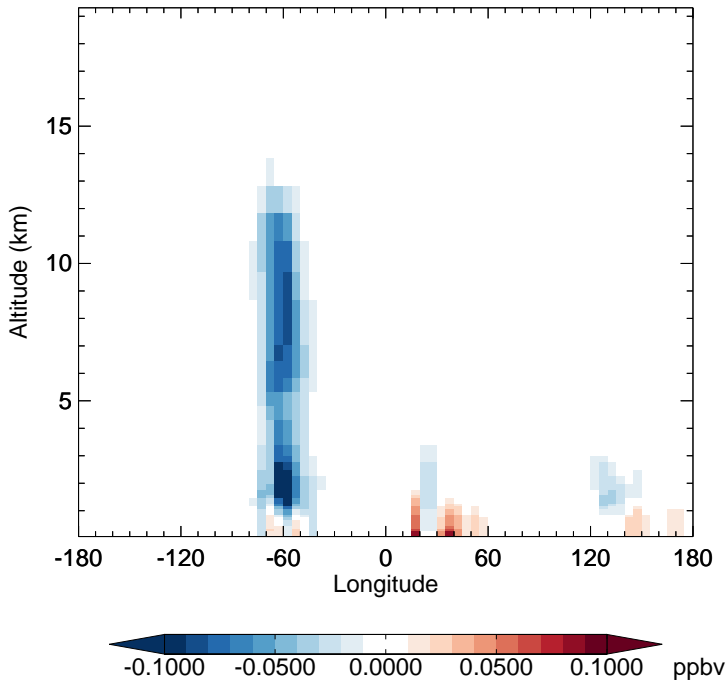
GC_12.0.0 - v11-02e-Run1 HAC - Diff along 15S for Jan
