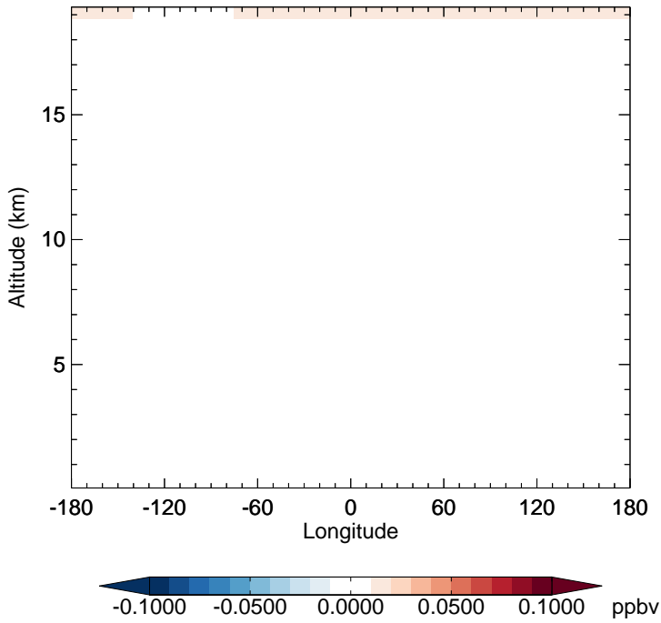
GC_12.0.0 - v11-02e-Run1 CFC12 - Diff along 15S for Jan
