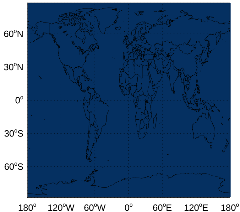
v11-02a - v11-01-public-Run0 Br2 biogenic emissions for Apr
